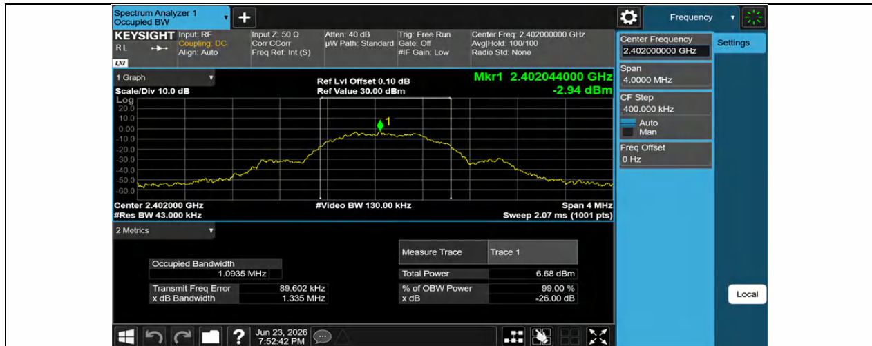
BLE_1M-Ant1-2402
