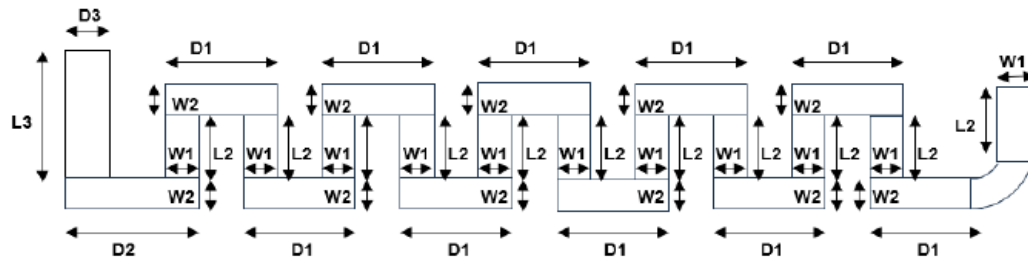
Antenna Dimensions
