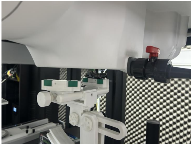
Next-to-mouth Front (dist. 10mm)
