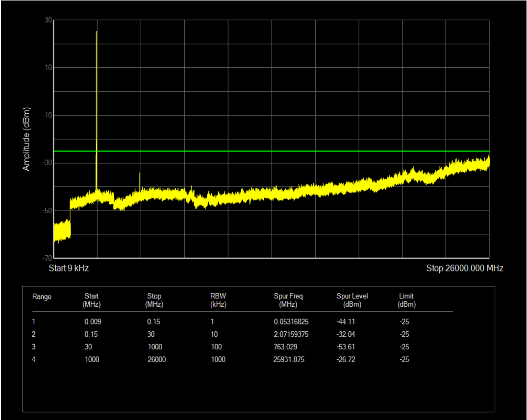
Band7 QPSK BW=10MHz Channel=21400 RB Size=1 Position=#Mid
