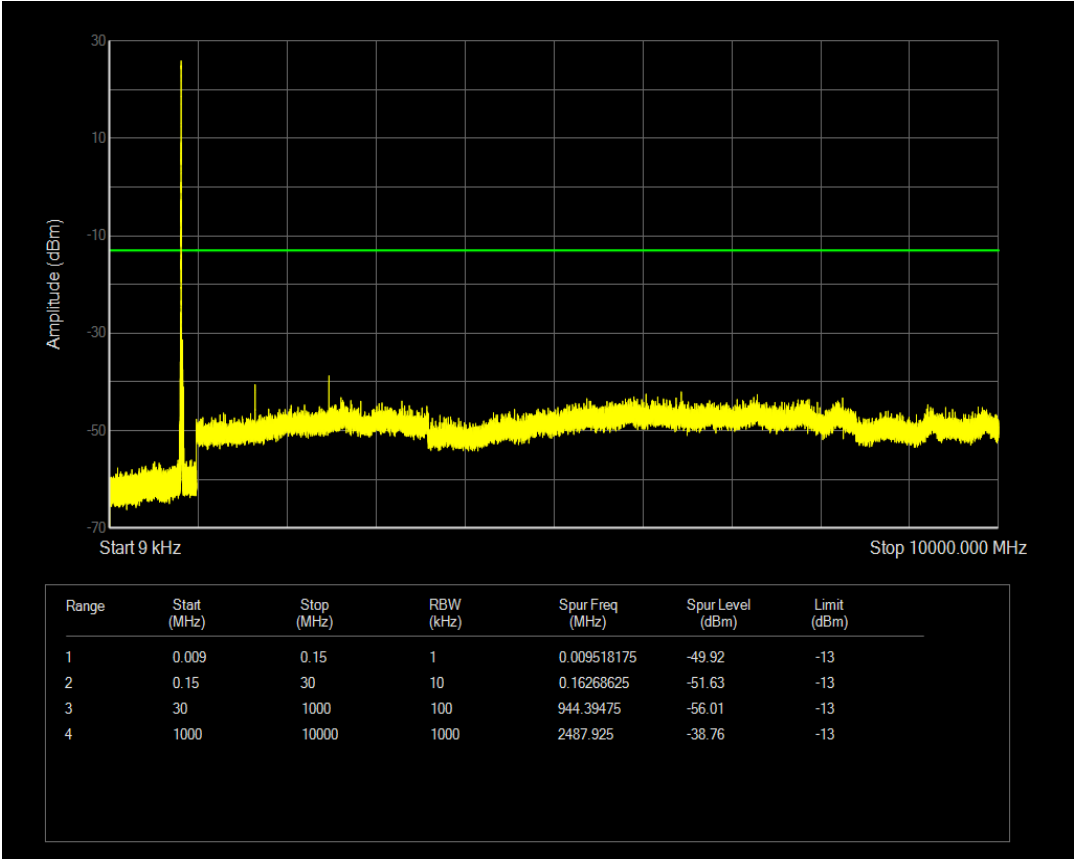
Band5 QAM16 BW=10MHz Channel=20450 RB Size=1 Position=#Mid
