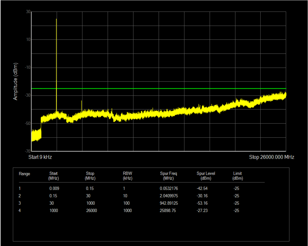
Band7 QAM16 BW=5MHz Channel=21425 RB Size=1 Position=#Mid
