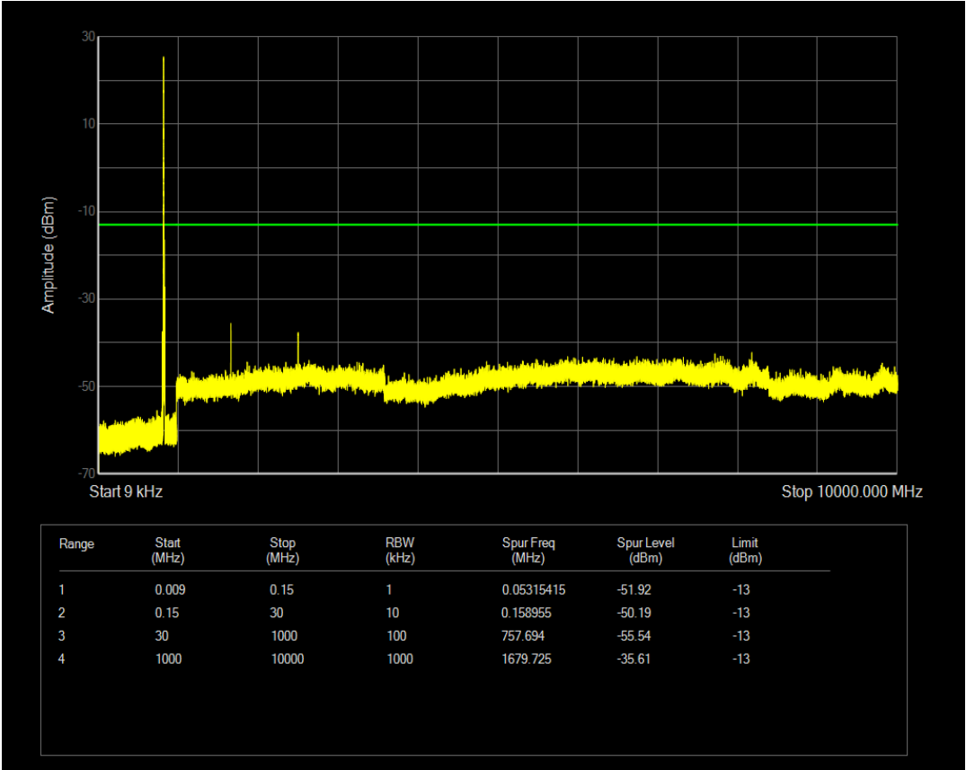
Band5 QPSK BW=10MHz Channel=20600 RB Size=1 Position=#Mid
