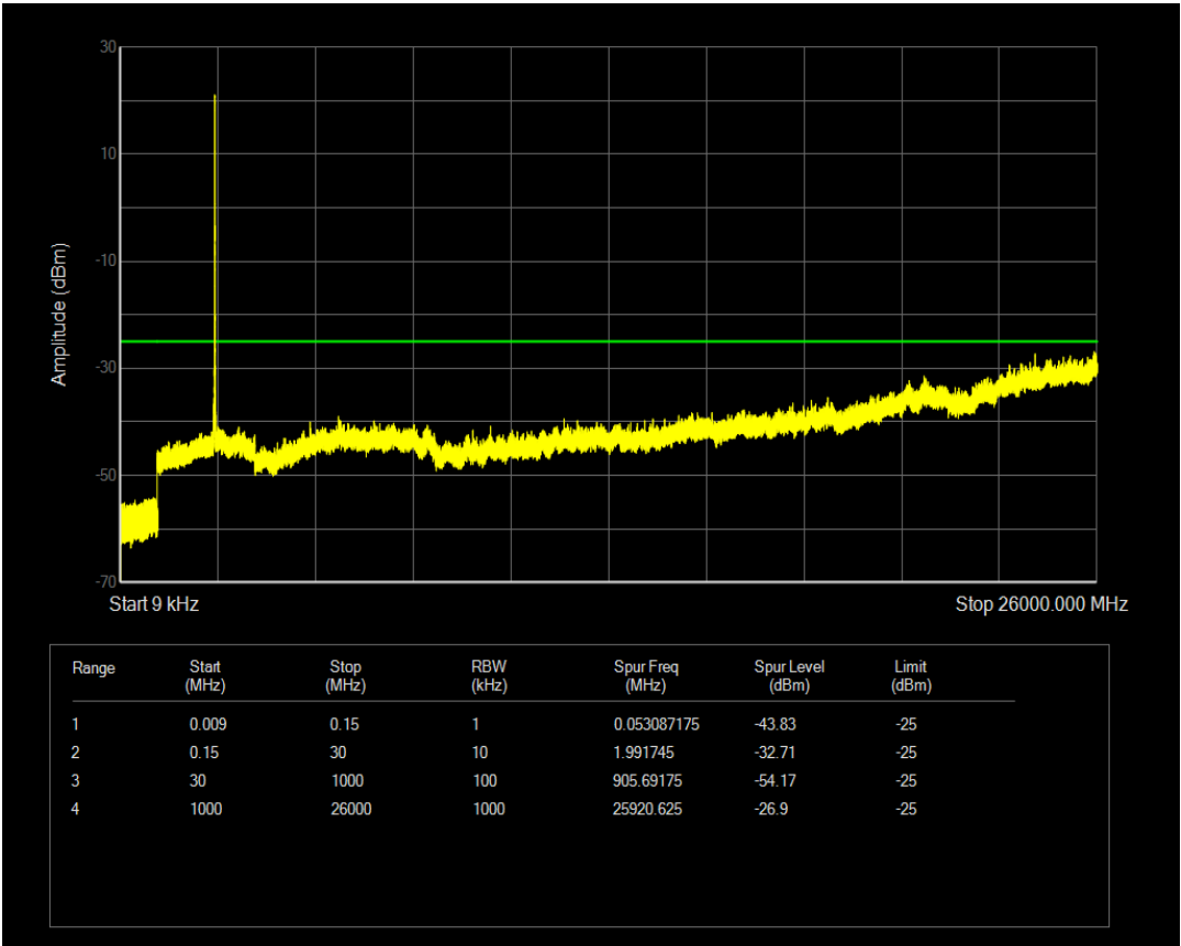
Band7 QPSK BW=10MHz Channel=21100 RB Size=25 Position=#0
