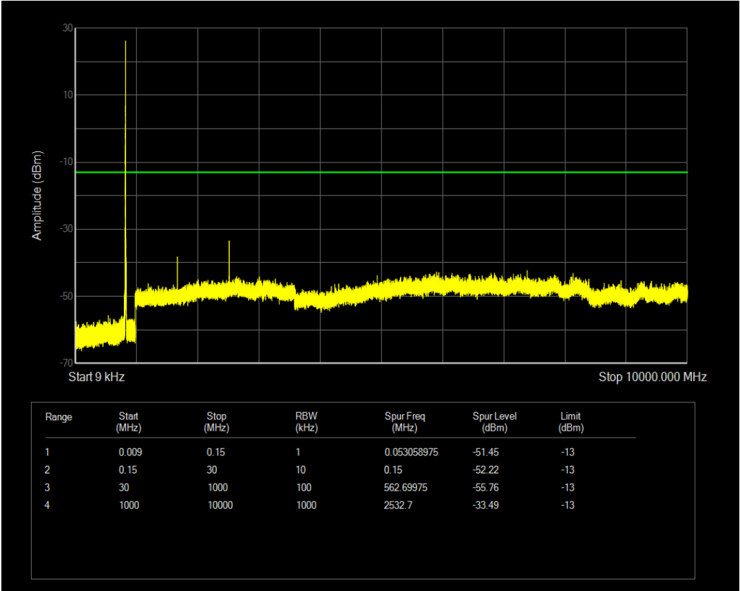
Band5 QAM16 BW=10MHz Channel=20600 RB Size=1 Position=#Mid
