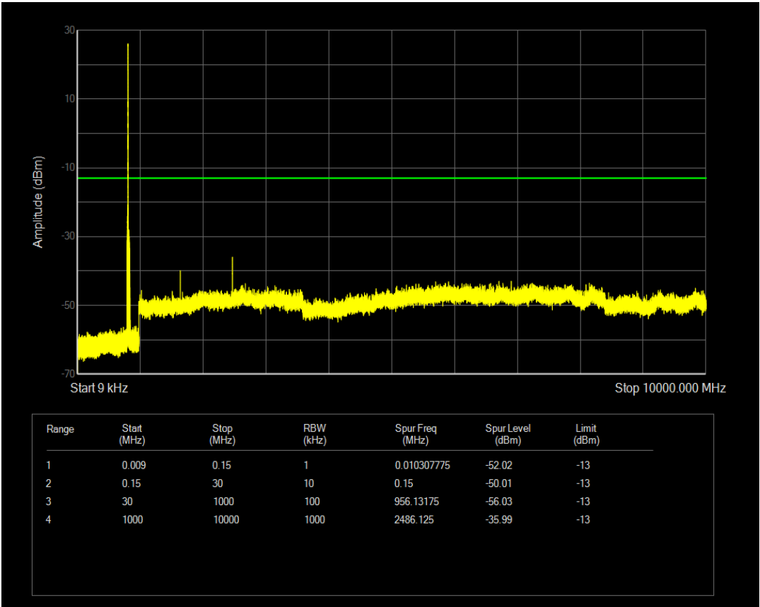
Band5 QAM16 BW=5MHz Channel=20425 RB Size=12 Position=#0
