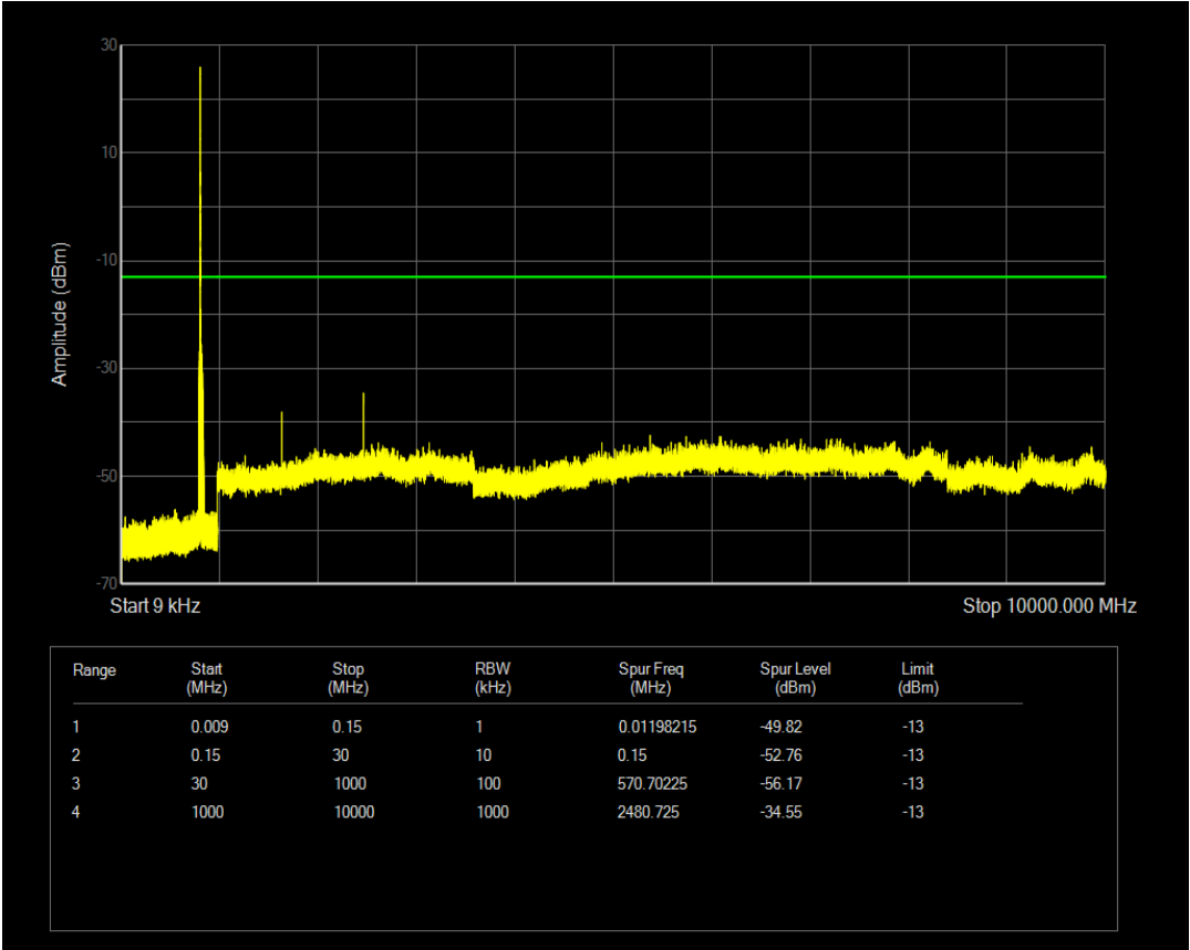
Band5 QAM16 BW=5MHz Channel=20425 RB Size=1 Position=#Mid
