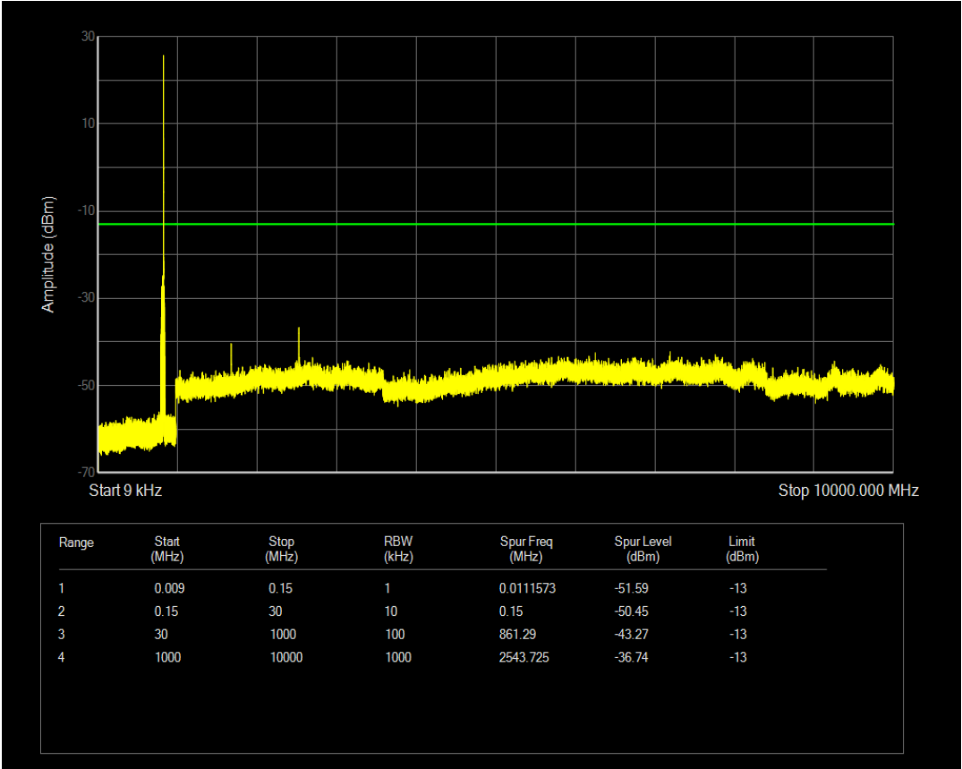
Band5 QAM16 BW=3MHz Channel=20635 RB Size=1 Position=#Mid
