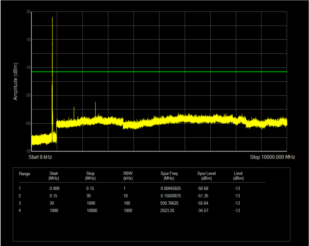
Band5 QPSK BW=10MHz Channel=20525 RB Size=25 Position=#0
