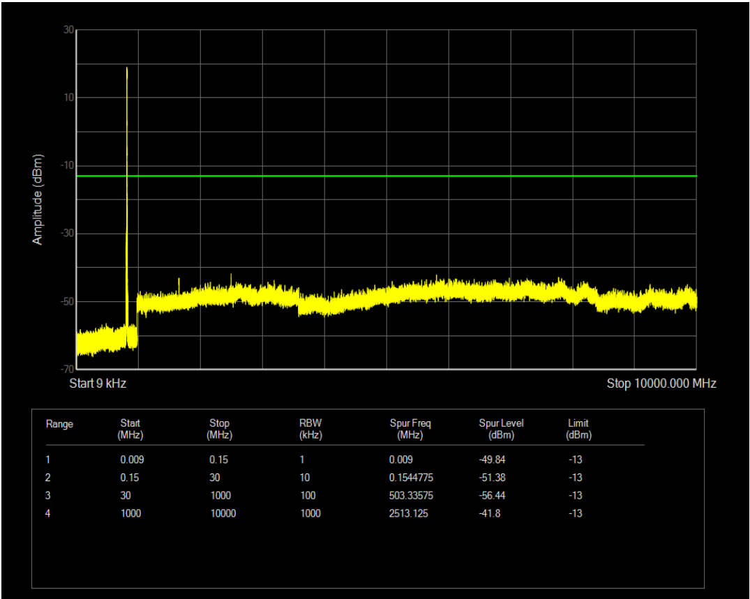
Band5 QPSK BW=5MHz Channel=20525 RB Size=12 Position=#Max
