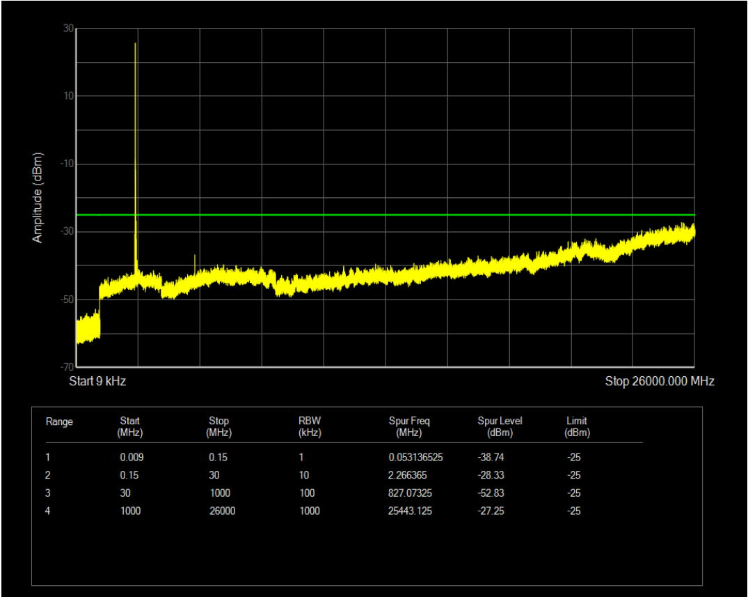
Band7 QAM16 BW=5MHz Channel=20775 RB Size=1 Position=#Mid
