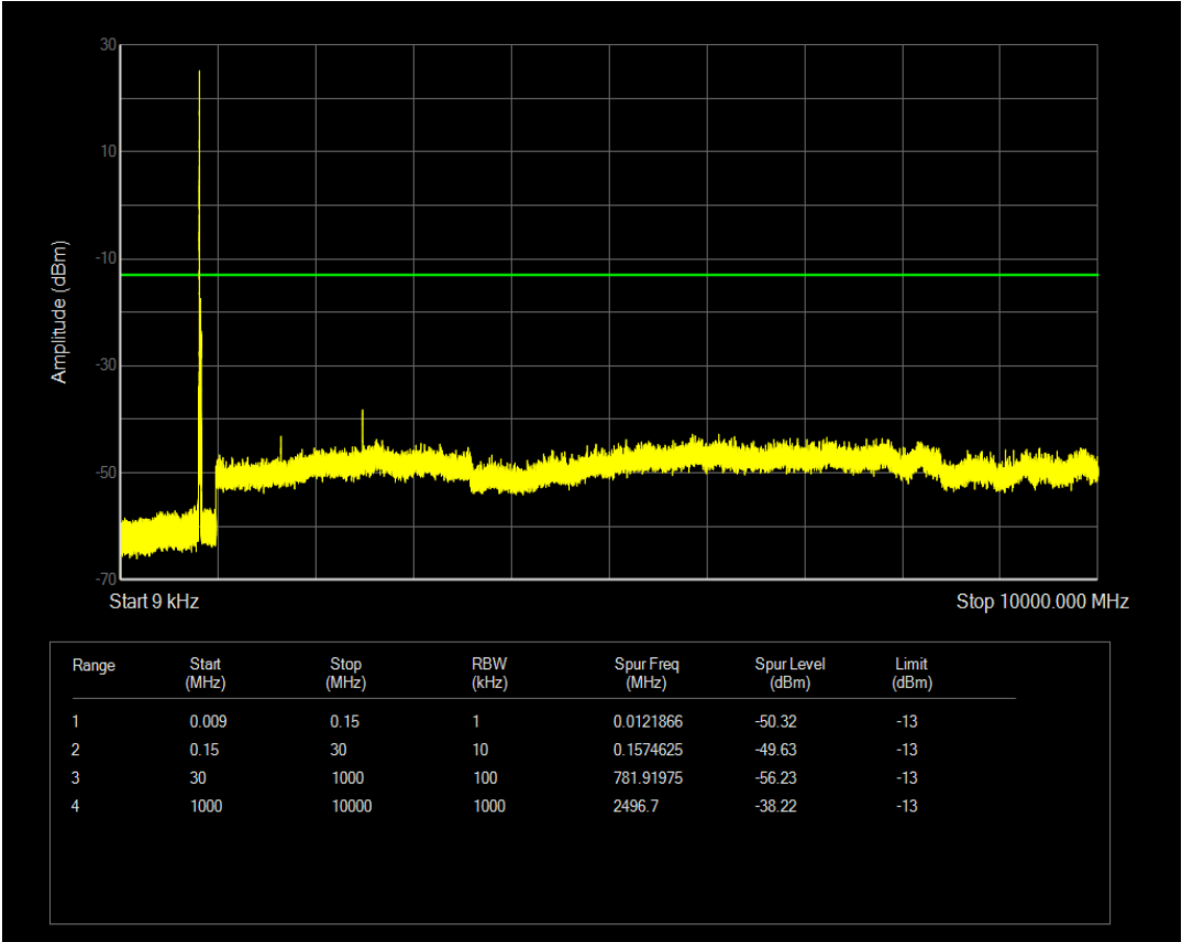
Band5 QAM16 BW=10MHz Channel=20525 RB Size=1 Position=#Max
