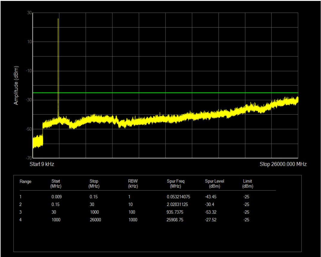
Band7 QAM16 BW=10MHz Channel=20800 RB Size=1 Position=#Mid
