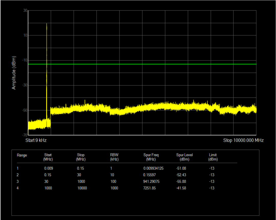
Band5 QAM16 BW=5MHz Channel=20525 RB Size=12 Position=#0
