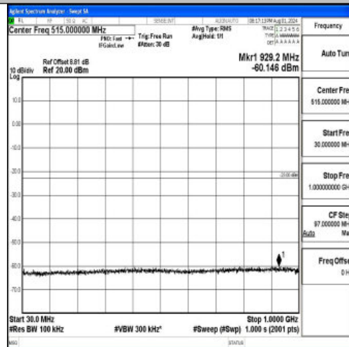
Band2-1.4MHz-QPSK-18607-1RB#0-30~1000-PASS
