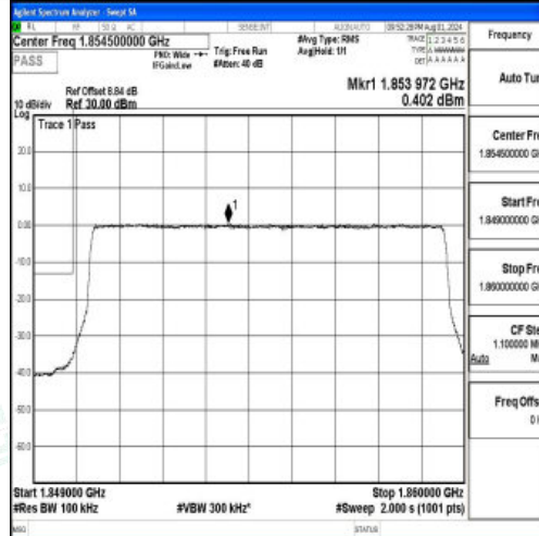
Band2-10MHz-16QAM-18650-50RB#0-PASS
