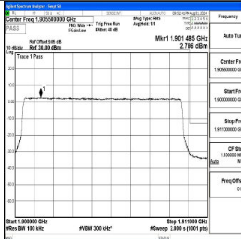
Band2-10MHz-QPSK-19150-50RB#0-PASS
