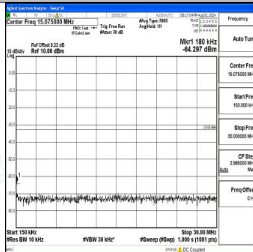
Band2-1.4MHz-QPSK-18607-1RB#0-0.15~30-PASS
