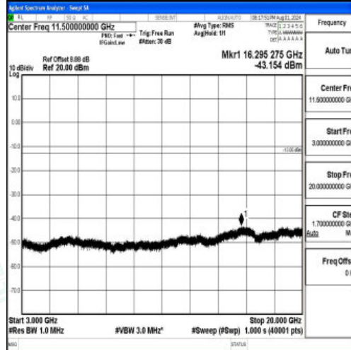
Band2-1.4MHz-QPSK-18607-1RB#0-3000~20000-PASS
