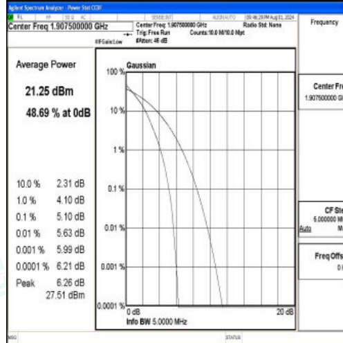
Band2-5MHz-QPSK-19175-25RB#0-PASS
