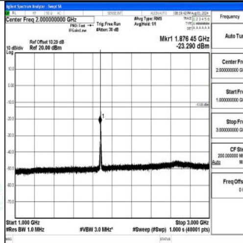
Band2-1.4MHz-QPSK-18900-1RB#0-1000~3000-PASS
