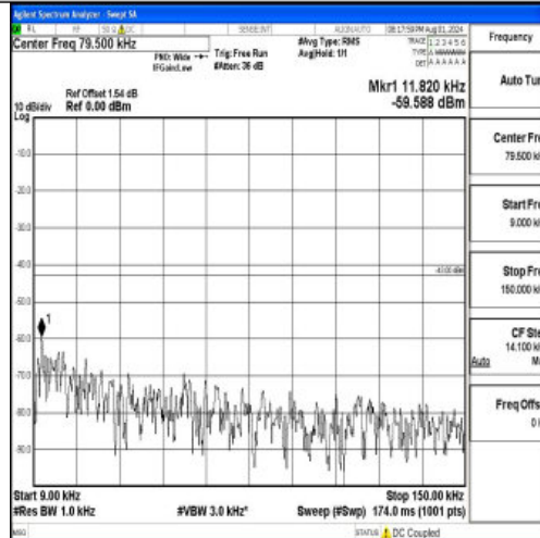
Band2-1.4MHz-16QAM-18607-1RB#0-0.009~0.15-PASS
