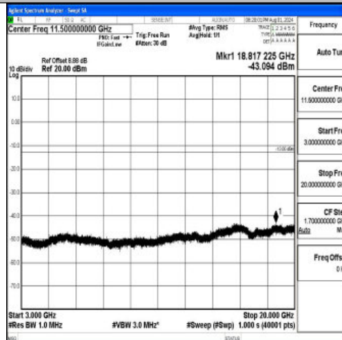
Band2-1.4MHz-QPSK-18900-1RB#0-3000~20000-PASS
