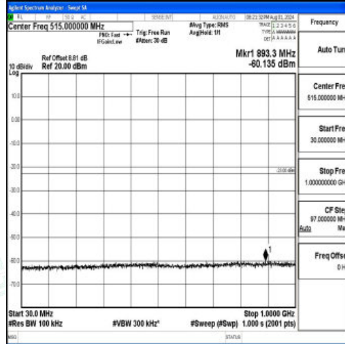
Band2-1.4MHz-QPSK-19193-1RB#0-30~1000-PASS
