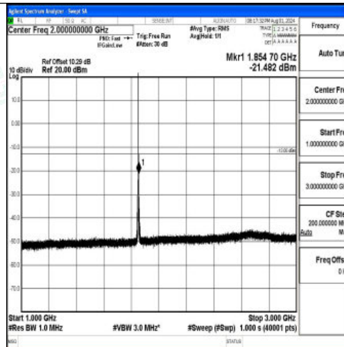
Band2-1.4MHz-QPSK-18607-1RB#0-1000~3000-PASS
