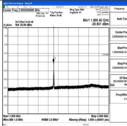
Band2-1.4MHz-QPSK-19193-1RB#0-1000~3000-PASS
