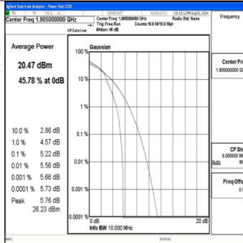
Band2-10MHz-16QAM-19150-1RB#0-PASS
