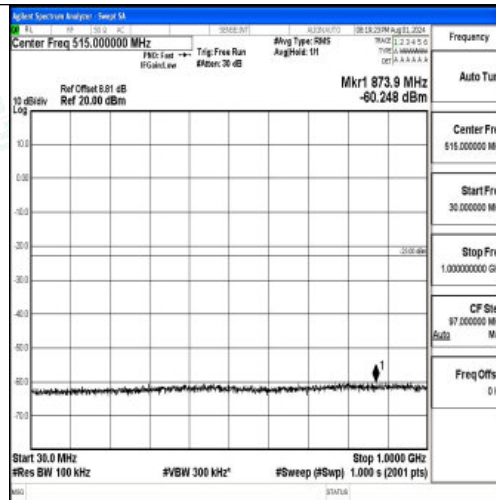
Band2-1.4MHz-QPSK-18900-1RB#0-30~1000-PASS
