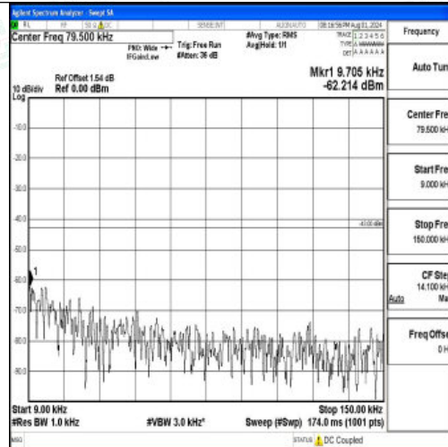
Band2-1.4MHz-QPSK-18607-1RB#0-0.009~0.15-PASS
