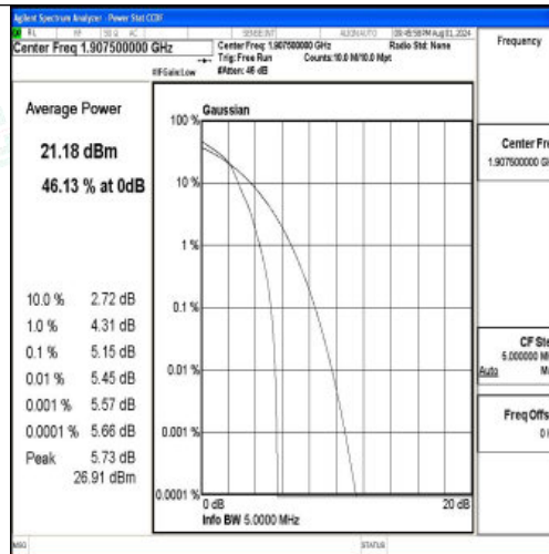
Band2-5MHz-16QAM-19175-1RB#0-PASS
