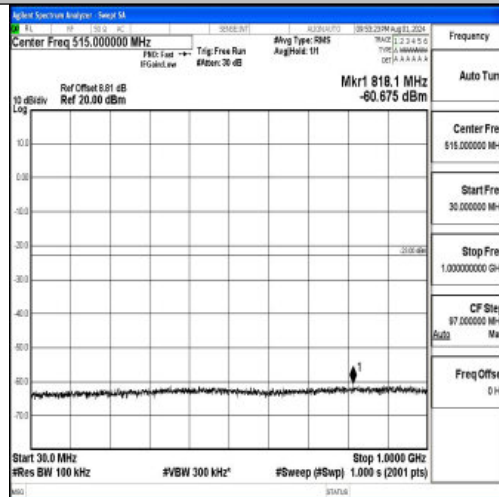
Band2-10MHz-QPSK-18650-1RB#0-30~1000-PASS
