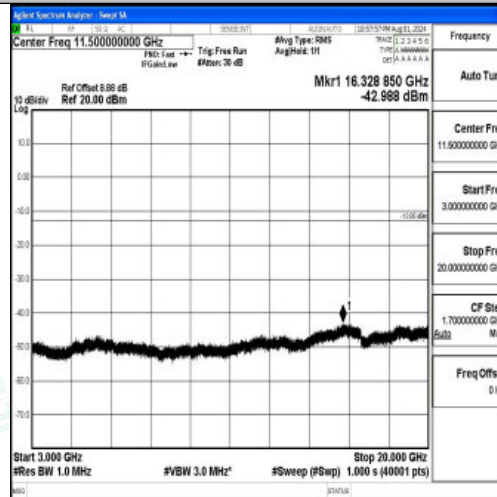
Band2-20MHz-QPSK-18700-1RB#0-3000~20000-PASS
