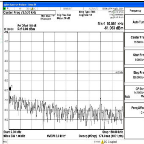
Band2-10MHz-16QAM-18900-1RB#0-0.009~0.15-PASS
