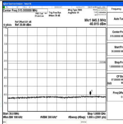
Band2-10MHz-QPSK-19150-1RB#0-30~1000-PASS
