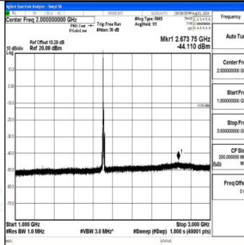
Band2-10MHz-16QAM-19150-1RB#0-1000~3000-PASS
