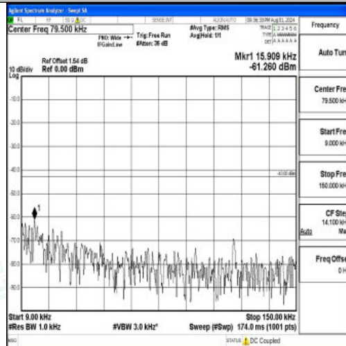
Band2-5MHz-16QAM-19175-1RB#0-0.009~0.15-PASS
