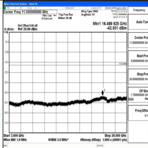
Band2-3MHz-QPSK-18615-1RB#0-3000~20000-PASS
