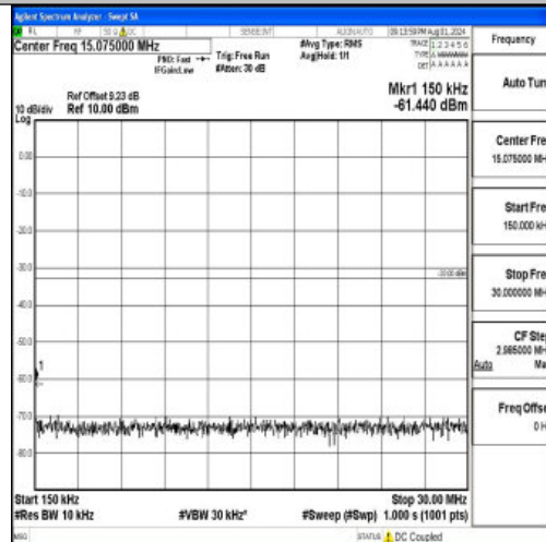
Band2-3MHz-16QAM-19185-1RB#0-0.15~30-PASS
