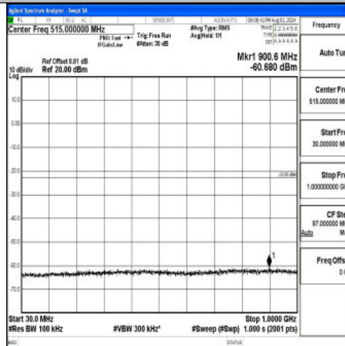
Band2-3MHz-QPSK-18615-1RB#0-30~1000-PASS
