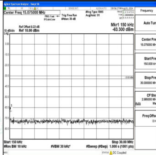
Band2-10MHz-16QAM-18900-1RB#0-0.15~30-PASS
