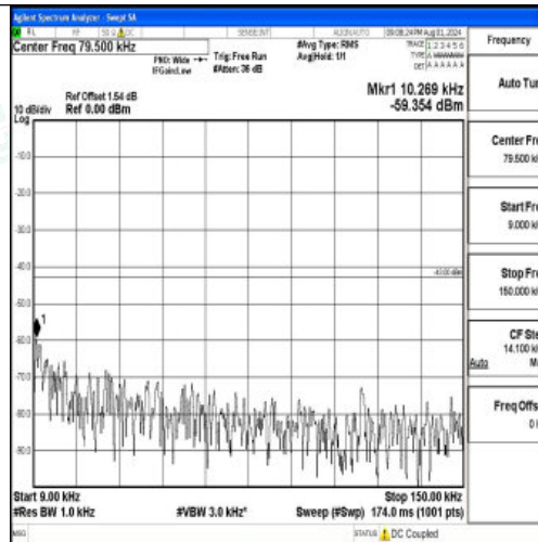
Band2-3MHz-QPSK-18615-1RB#0-0.009~0.15-PASS
