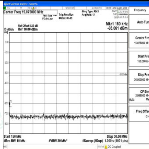
Band2-10MHz-QPSK-18650-1RB#0-0.15~30-PASS
