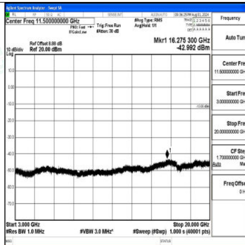
Band2-5MHz-QPSK-19175-1RB#0-3000~20000-PASS
