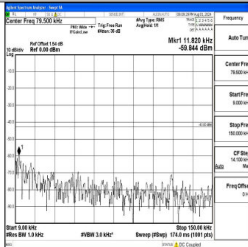
Band2-3MHz-16QAM-18615-1RB#0-0.009~0.15-PASS
