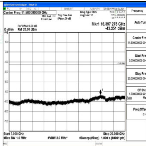
Band2-10MHz-16QAM-18650-1RB#0-3000~20000-PASS
