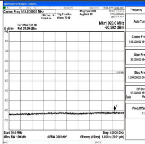
Band2-10MHz-16QAM-18900-1RB#0-30~1000-PASS
