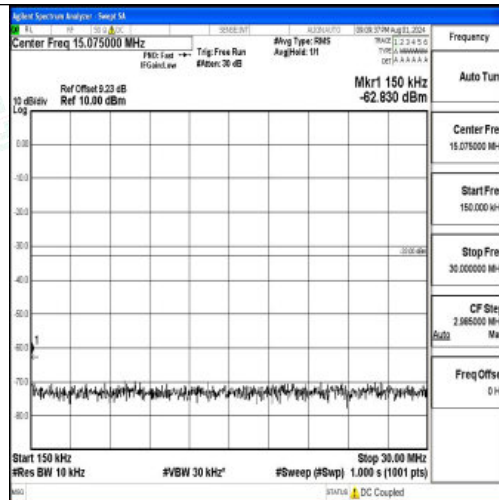
Band2-3MHz-16QAM-18615-1RB#0-0.15~30-PASS
