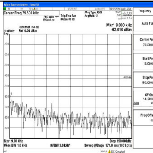
Band2-10MHz-QPSK-19150-1RB#0-0.009~0.15-PASS
