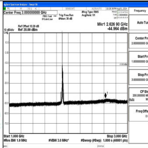
Band2-15MHz-16QAM-19125-1RB#0-1000~3000-PASS
