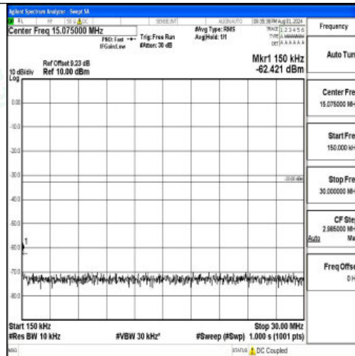
Band2-5MHz-QPSK-19175-1RB#0-0.15~30-PASS
