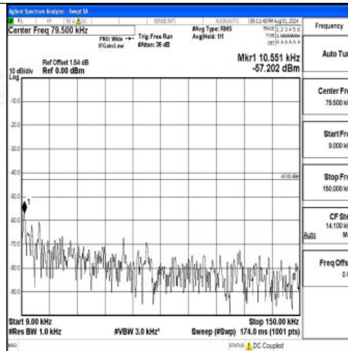
Band2-3MHz-16QAM-18900-1RB#0-0.009~0.15-PASS
