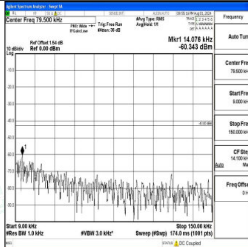
Band2-10MHz-QPSK-18900-1RB#0-0.009~0.15-PASS
