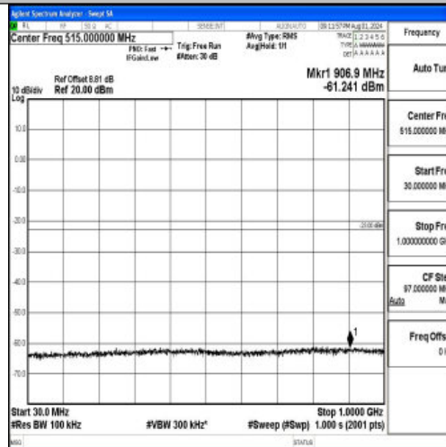
Band2-3MHz-16QAM-18900-1RB#0-30~1000-PASS
