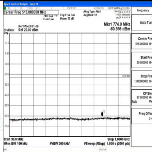
Band2-5MHz-QPSK-19175-1RB#0-30~1000-PASS
