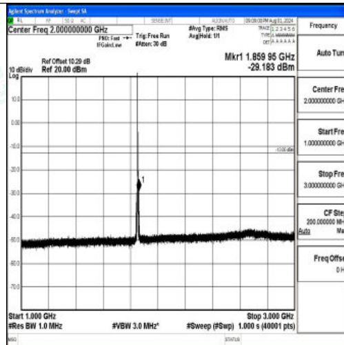
Band2-3MHz-QPSK-18615-1RB#0-1000~3000-PASS
