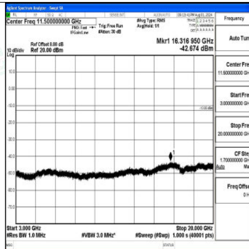
Band2-3MHz-QPSK-19185-1RB#0-3000~20000-PASS
