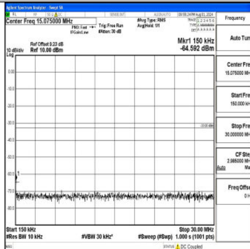
Band2-10MHz-QPSK-18900-1RB#0-0.15~30-PASS
