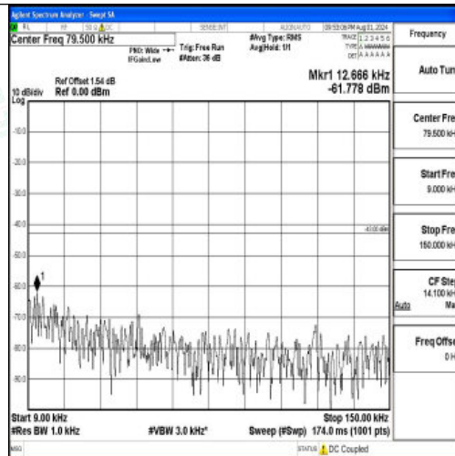
Band2-10MHz-QPSK-18650-1RB#0-0.009~0.15-PASS
