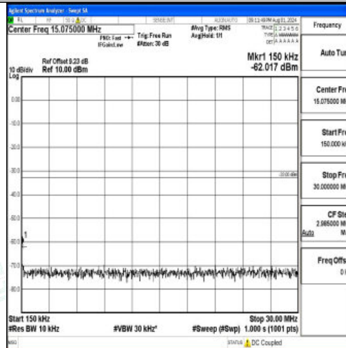
Band2-3MHz-16QAM-18900-1RB#0-0.15~30-PASS
