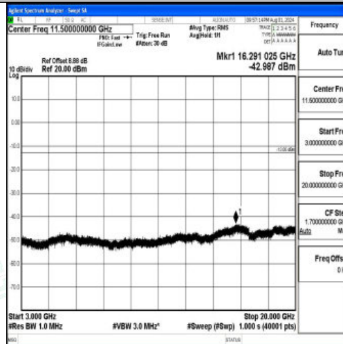
Band2-10MHz-16QAM-18900-1RB#0-3000~20000-PASS
