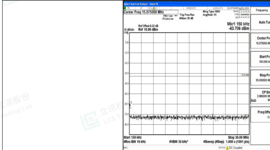
Band4-20MHz-16QAM-20175-1RB#0-0.15~30-PASS
