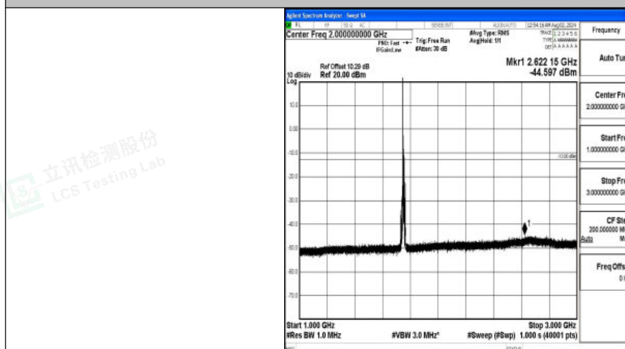
Band4-10MHz-QPSK-20350-1RB#0-1000~3000-PASS
