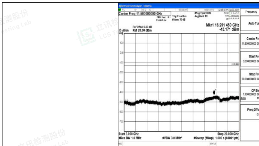
Band4-3MHz-QPSK-20385-1RB#0-3000~20000-PASS
