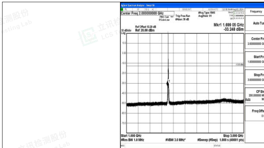
Band4-5MHz-QPSK-19975-1RB#0-1000~3000-PASS
