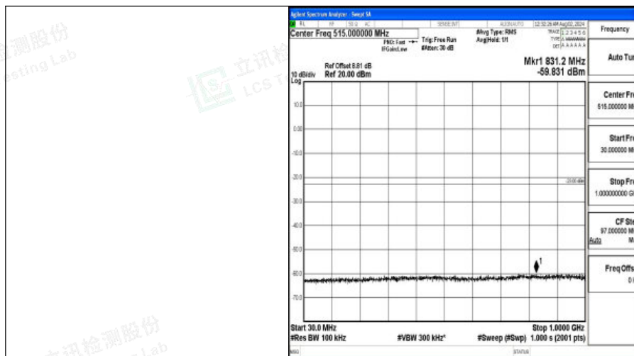
Band4-5MHz-QPSK-20175-1RB#0-30~1000-PASS
