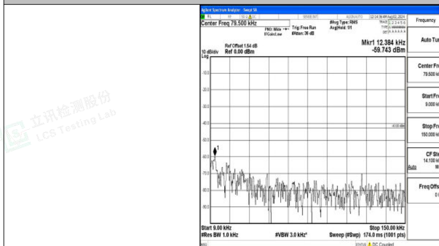
Band4-3MHz-QPSK-20385-1RB#0-0.009~0.15-PASS
