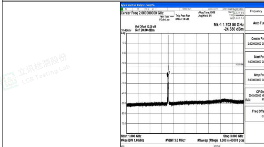
Band4-3MHz-16QAM-19965-1RB#0-1000~3000-PASS
