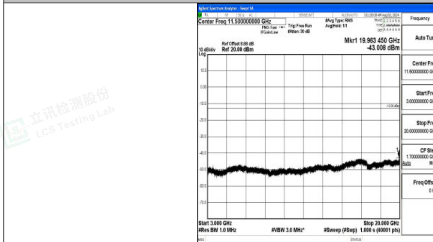
Band4-15MHz-16QAM-20325-1RB#0-3000~20000-PASS
