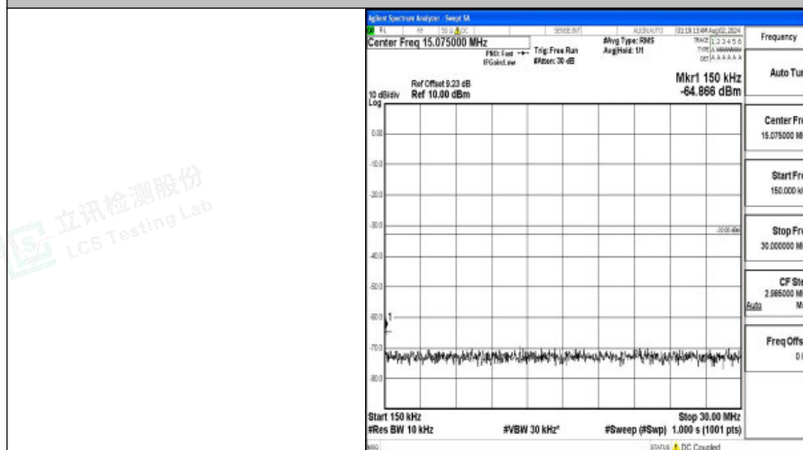
Band4-15MHz-16QAM-20325-1RB#0-0.15~30-PASS
