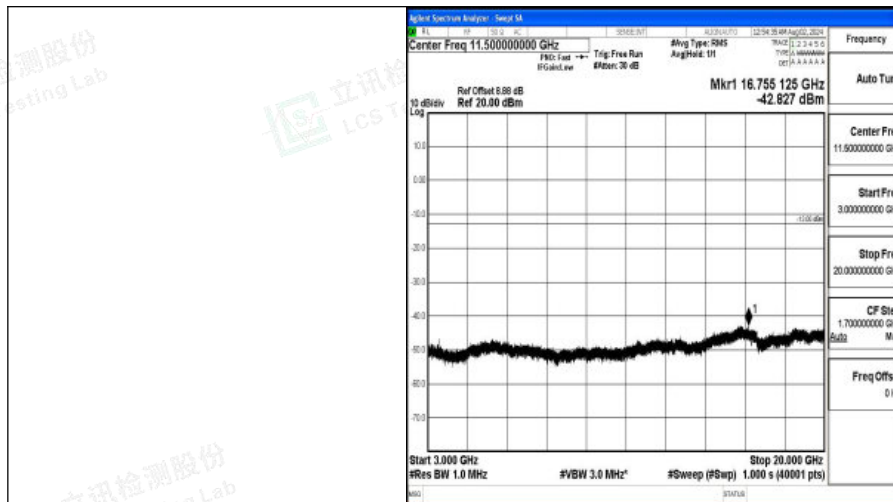
Band4-10MHz-QPSK-20350-1RB#0-3000~20000-PASS
