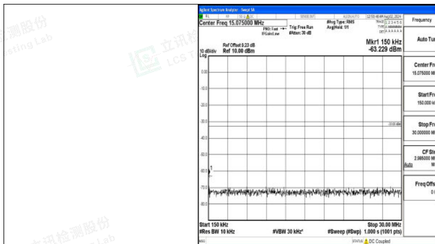
Band4-10MHz-QPSK-20350-1RB#0-0.15~30-PASS
