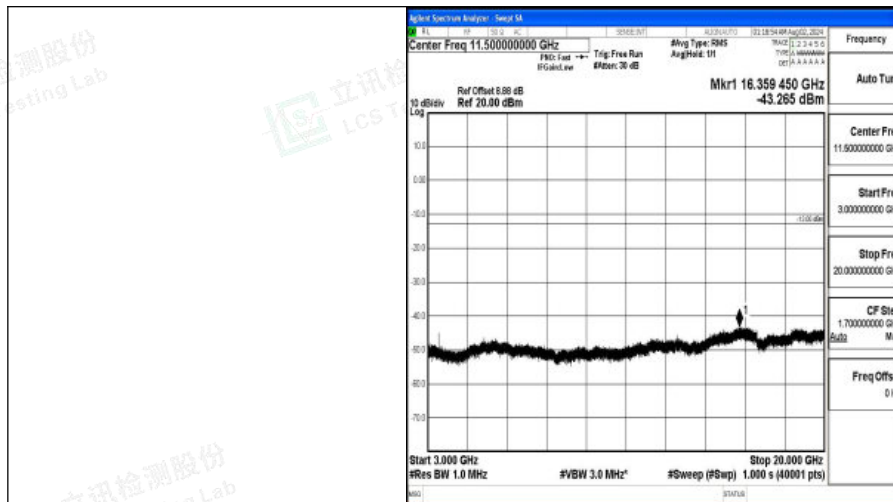
Band4-15MHz-QPSK-20325-1RB#0-3000~20000-PASS
