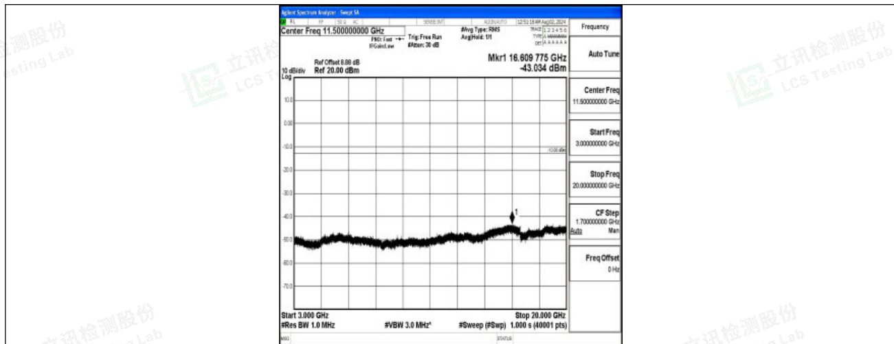
Band4-10MHz-16QAM-20000-1RB#0-3000~20000-PASS
