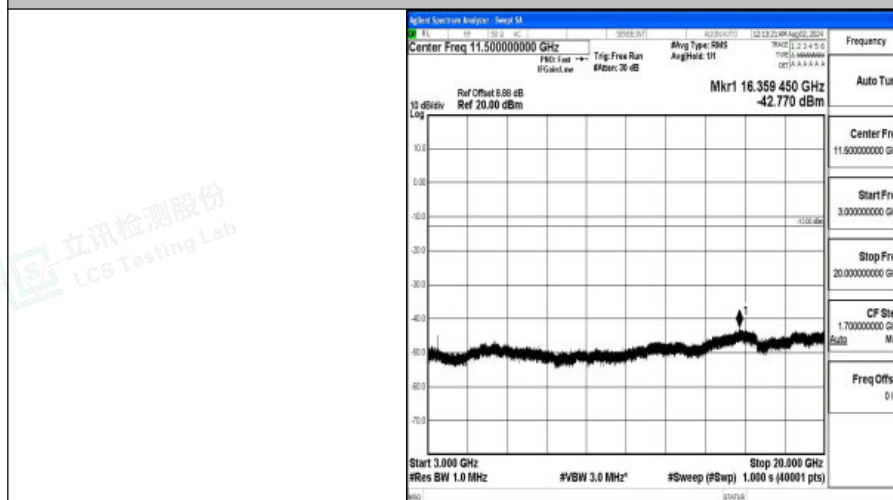
Band4-3MHz-QPSK-20175-1RB#0-3000~20000-PASS
