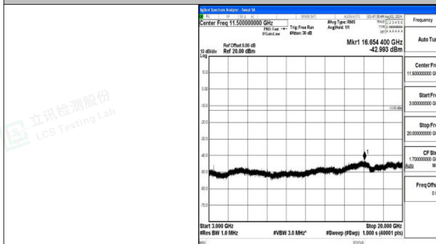
Band4-20MHz-QPSK-20175-1RB#0-3000~20000-PASS
