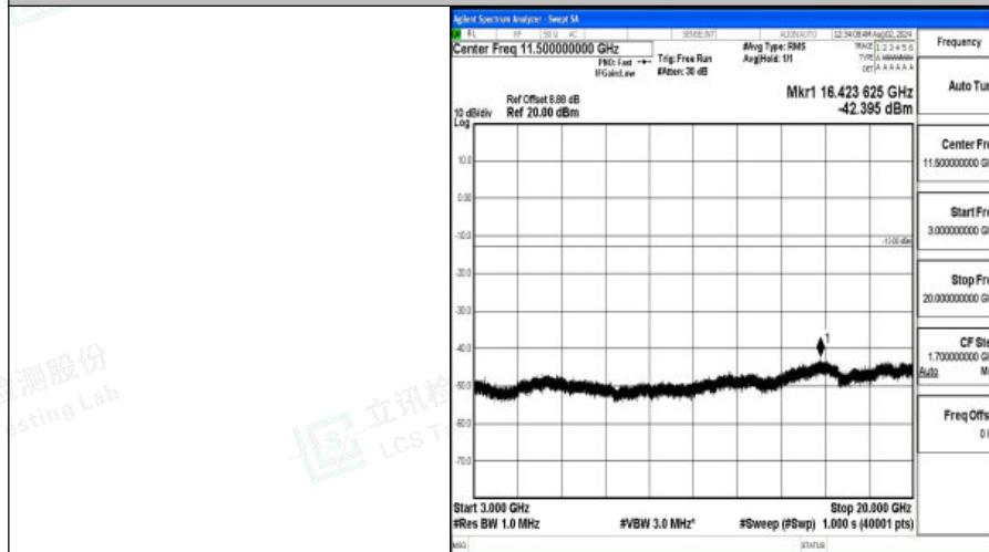
Band4-5MHz-16QAM-20175-1RB#0-3000~20000-PASS
