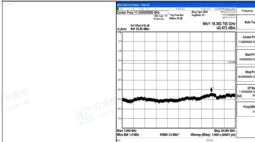
Band4-5MHz-QPSK-19975-1RB#0-3000~20000-PASS
