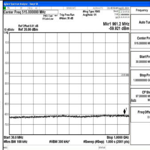
Band4-20MHz-16QAM-20050-1RB#0-30~1000-PASS
