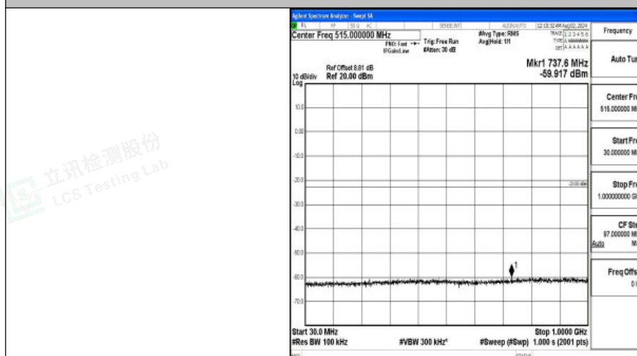
Band4-3MHz-QPSK-19965-1RB#0-30~1000-PASS
