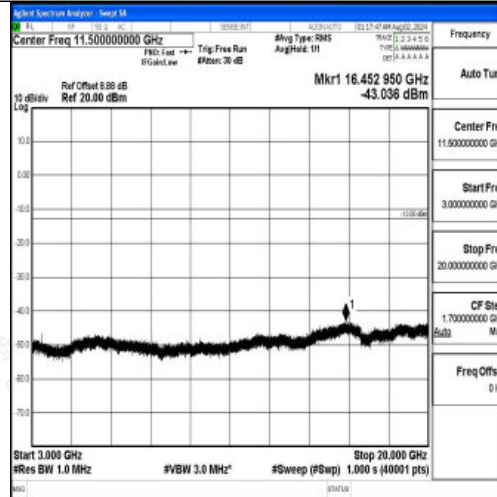
Band4-15MHz-16QAM-20175-1RB#0-3000~20000-PASS
