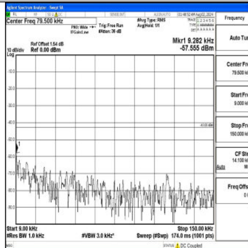
Band4-20MHz-QPSK-20300-1RB#0-0.009~0.15-PASS
