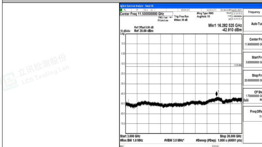
Band4-15MHz-QPSK-20175-1RB#0-3000~20000-PASS
