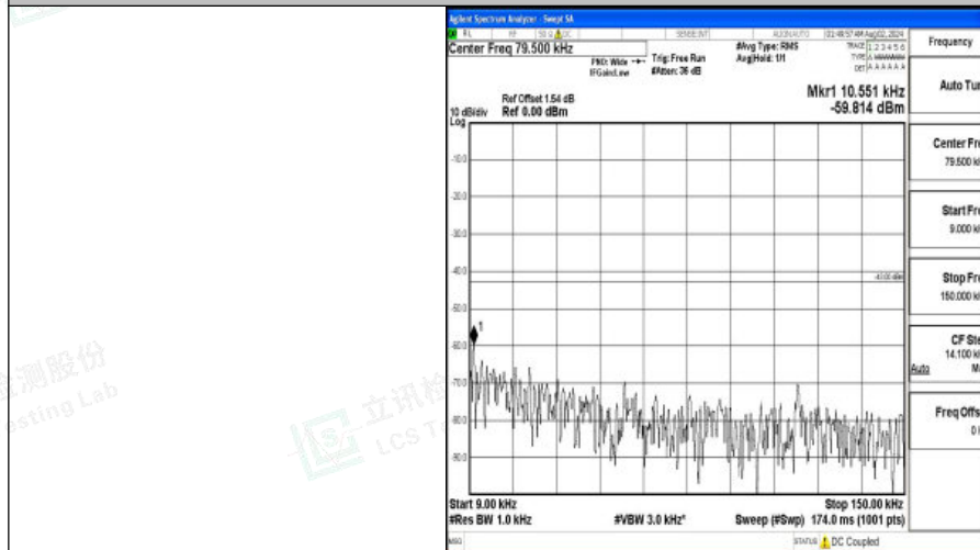
Band4-20MHz-16QAM-20300-1RB#0-0.009~0.15-PASS
