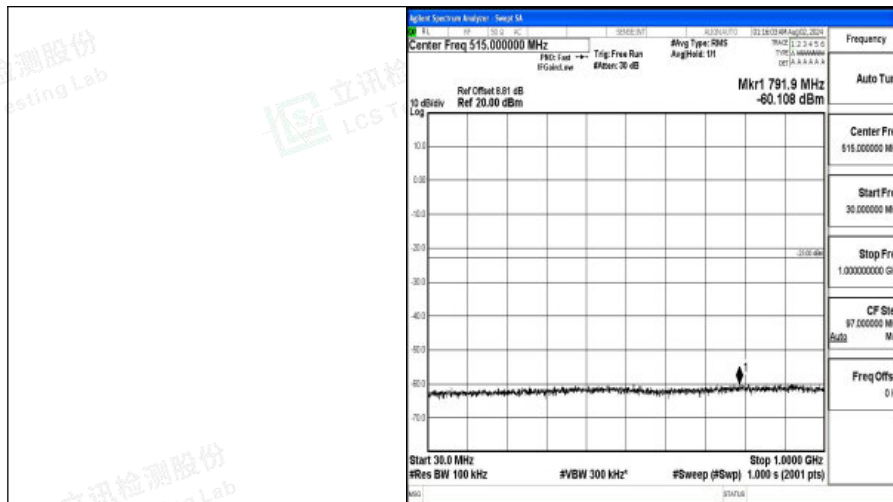
Band4-15MHz-QPSK-20175-1RB#0-30~1000-PASS
