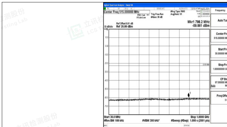
Band4-10MHz-QPSK-20175-1RB#0-30~1000-PASS
