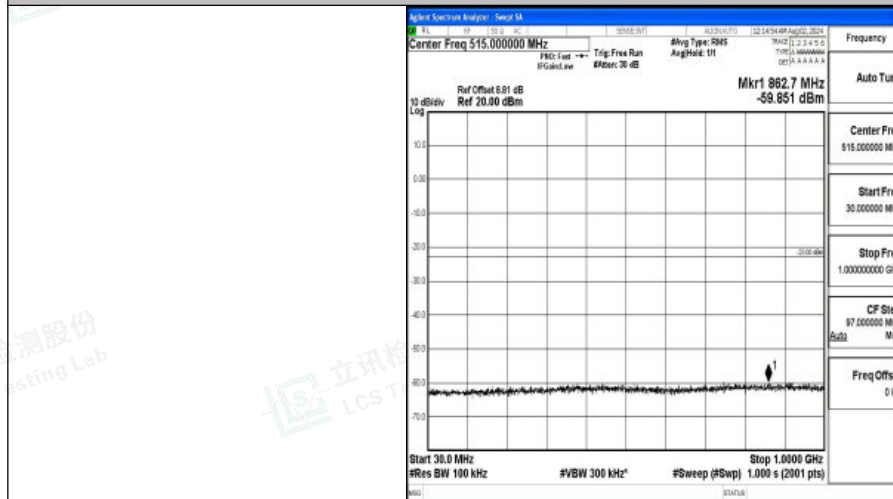
Band4-3MHz-QPSK-20385-1RB#0-30~1000-PASS
