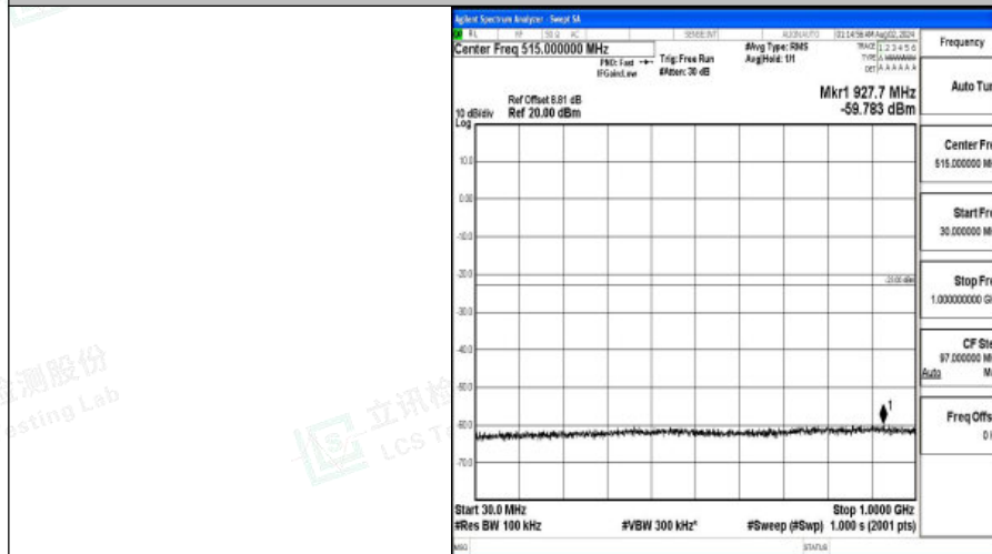
Band4-15MHz-16QAM-20025-1RB#0-30~1000-PASS
