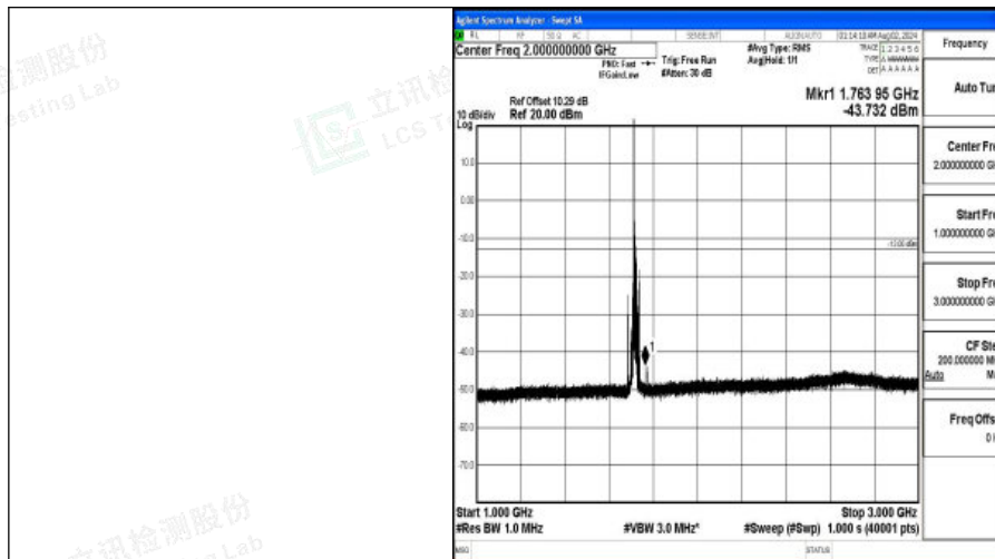
Band4-15MHz-QPSK-20025-1RB#0-1000~3000-PASS
