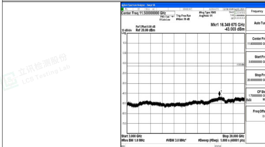
Band4-5MHz-16QAM-20375-1RB#0-3000~20000-PASS
