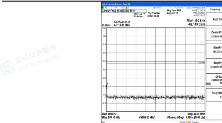
Band4-3MHz-QPSK-20175-1RB#0-0.15~30-PASS
