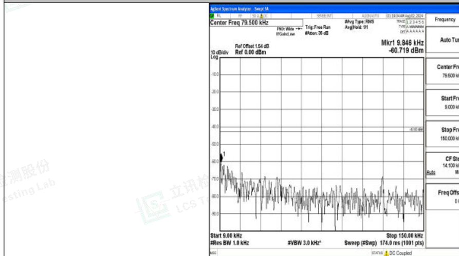
Band4-15MHz-16QAM-20325-1RB#0-0.009~0.15-PASS
