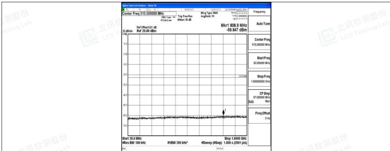
Band4-3MHz-16QAM-20385-1RB#0-30~1000-PASS
