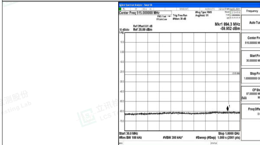
Band4-3MHz-16QAM-19965-1RB#0-30~1000-PASS
