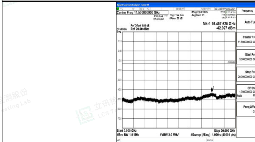
Band4-3MHz-QPSK-19965-1RB#0-3000~20000-PASS
