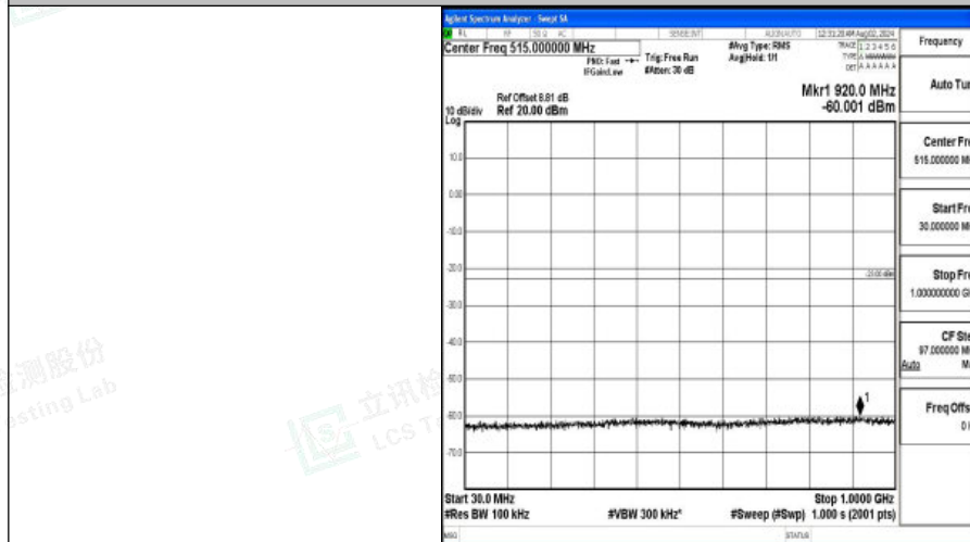
Band4-5MHz-16QAM-19975-1RB#0-30~1000-PASS
