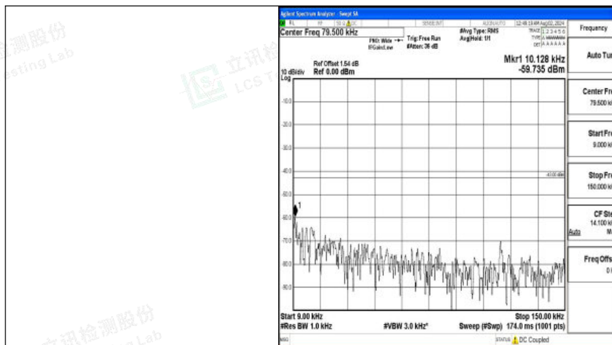
Band4-10MHz-QPSK-20000-1RB#0-0.009~0.15-PASS
