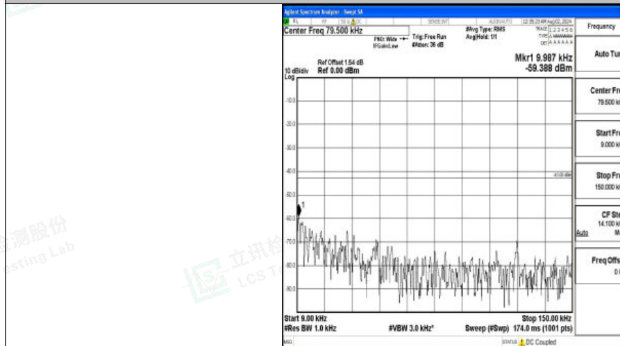
Band4-5MHz-16QAM-20375-1RB#0-0.009~0.15-PASS
