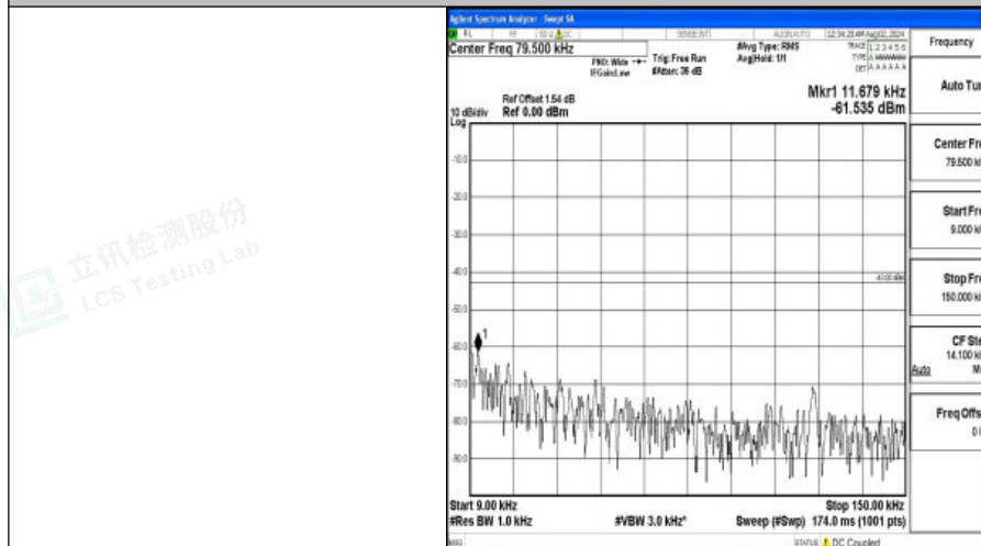
Band4-5MHz-QPSK-20375-1RB#0-0.009~0.15-PASS
