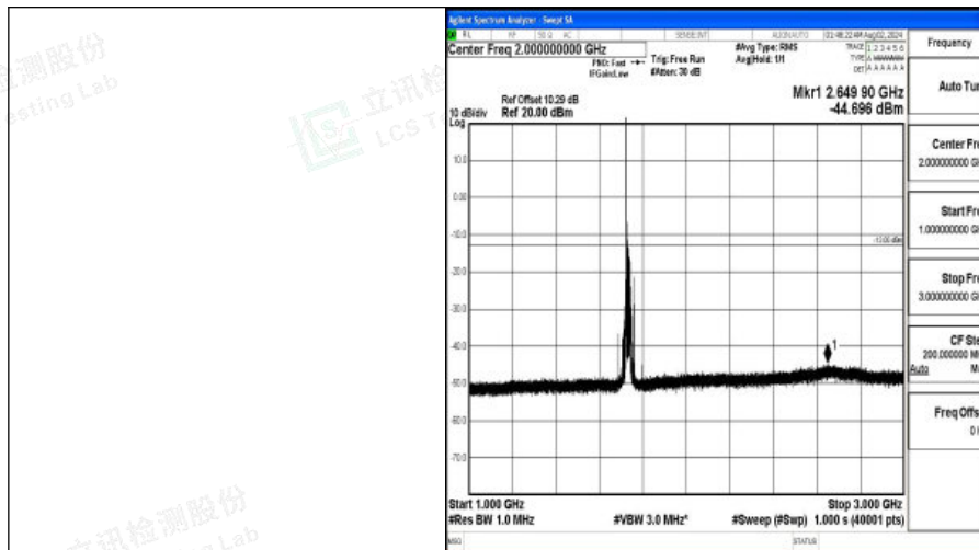
Band4-20MHz-16QAM-20175-1RB#0-1000~3000-PASS
