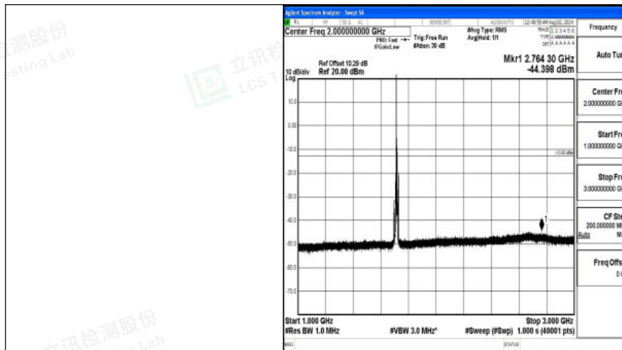
Band4-10MHz-QPSK-20000-1RB#0-1000~3000-PASS
