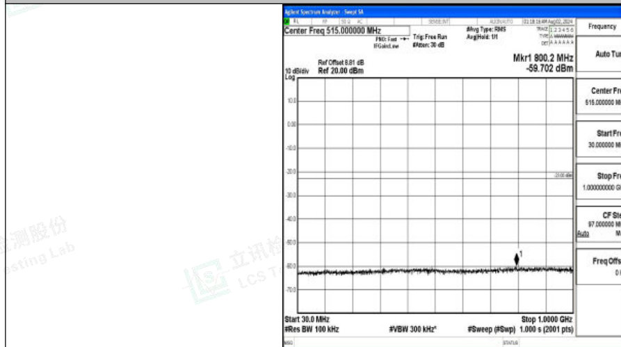
Band4-15MHz-QPSK-20325-1RB#0-30~1000-PASS
