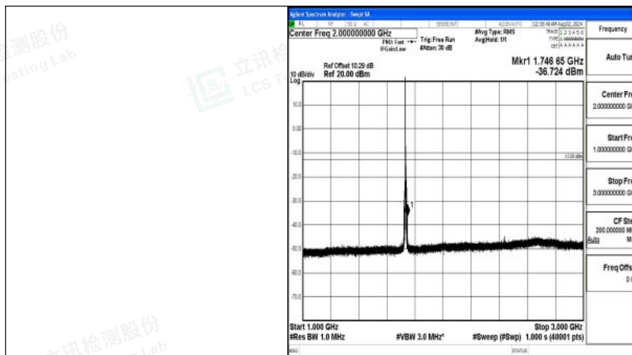
Band4-5MHz-16QAM-20175-1RB#0-1000~3000-PASS
