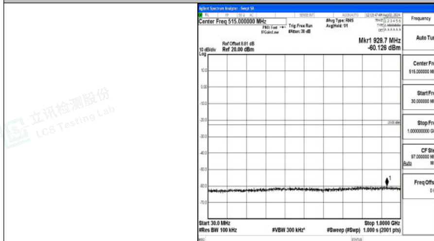
Band4-3MHz-16QAM-20175-1RB#0-30~1000-PASS
