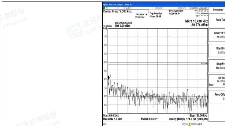
Band4-3MHz-QPSK-19965-1RB#0-0.009~0.15-PASS
