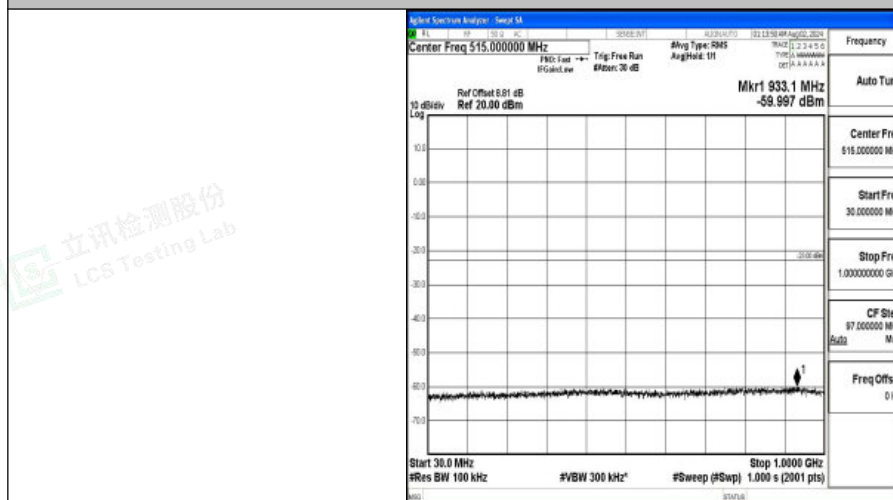
Band4-15MHz-QPSK-20025-1RB#0-30~1000-PASS
