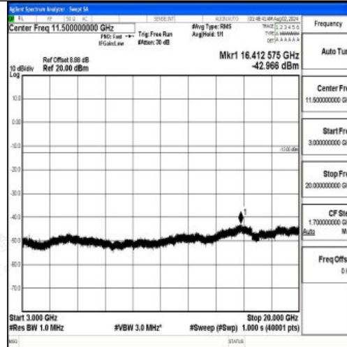
Band4-20MHz-16QAM-20175-1RB#0-3000~20000-PASS
