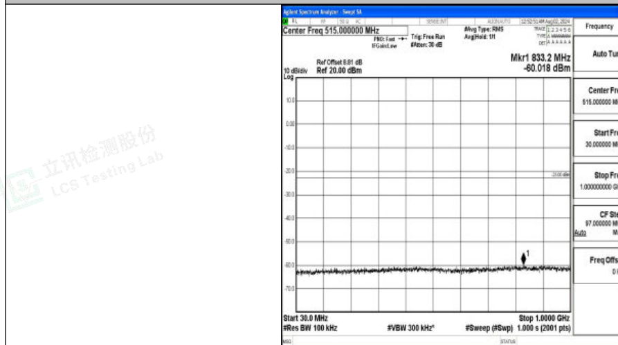
Band4-10MHz-16QAM-20175-1RB#0-30~1000-PASS
