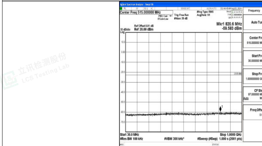
Band4-20MHz-QPSK-20050-1RB#0-30~1000-PASS
