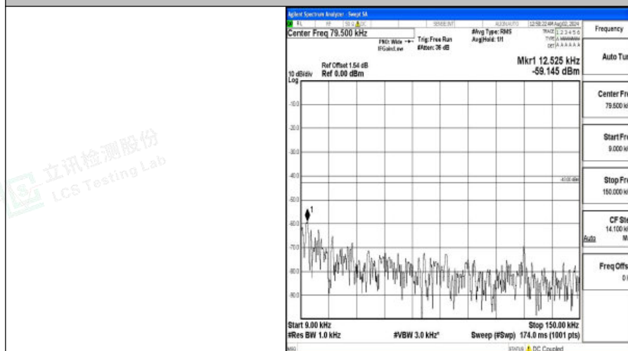
Band4-10MHz-16QAM-20000-1RB#0-0.009~0.15-PASS
