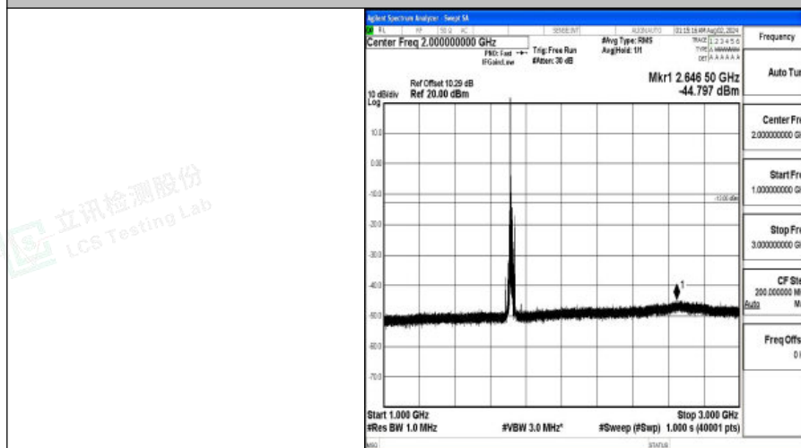
Band4-15MHz-16QAM-20025-1RB#0-1000~3000-PASS
