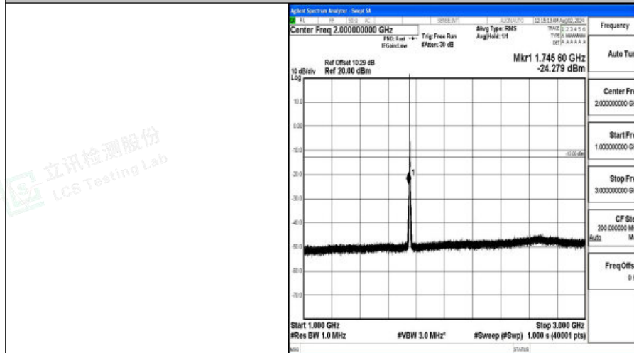
Band4-3MHz-QPSK-20385-1RB#0-1000~3000-PASS
