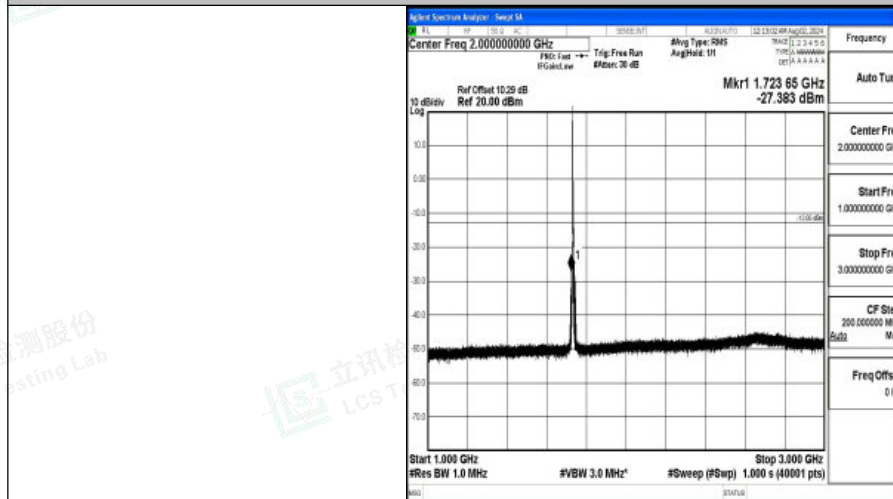
Band4-3MHz-QPSK-20175-1RB#0-1000~3000-PASS
