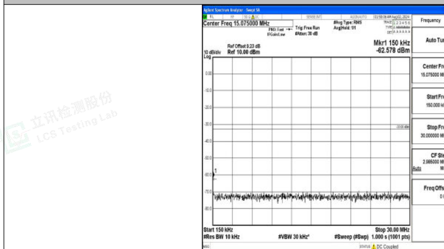
Band4-20MHz-16QAM-20300-1RB#0-0.15~30-PASS
