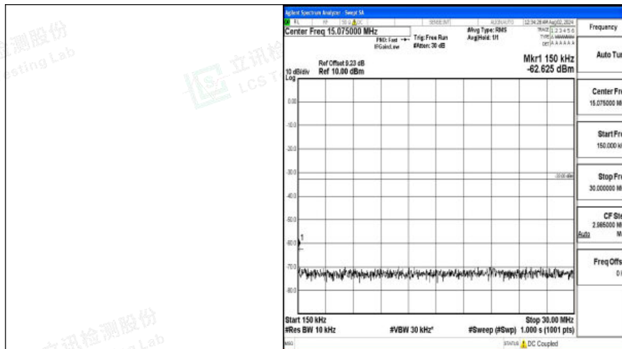
Band4-5MHz-QPSK-20375-1RB#0-0.15~30-PASS
