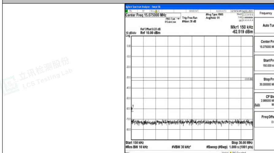
Band4-10MHz-16QAM-20350-1RB#0-0.15~30-PASS
