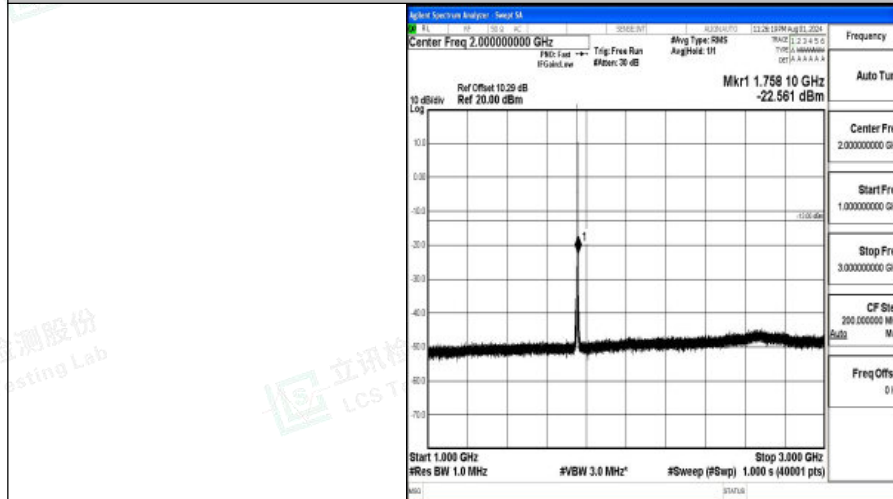
Band4-1.4MHz-16QAM-20393-1RB#0-1000~3000-PASS
