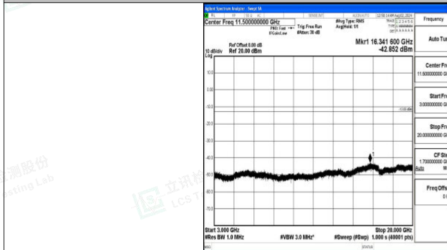
Band4-10MHz-QPSK-20000-1RB#0-3000~20000-PASS
