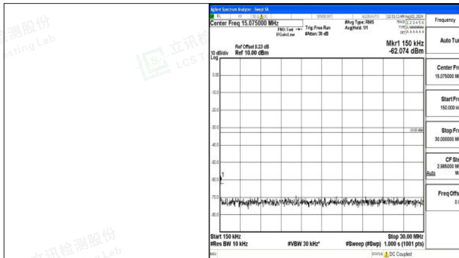
Band4-5MHz-16QAM-19975-1RB#0-0.15~30-PASS
