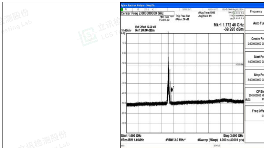
Band4-20MHz-QPSK-20050-1RB#0-1000~3000-PASS
