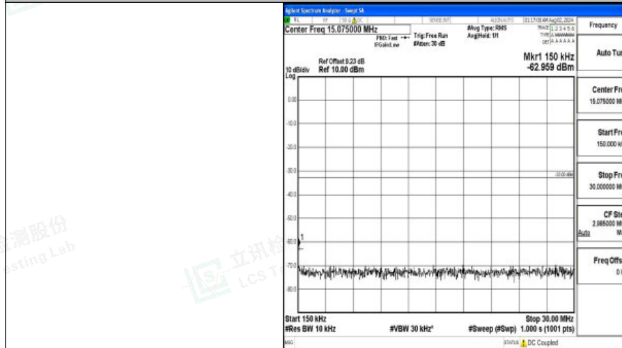
Band4-15MHz-16QAM-20175-1RB#0-0.15~30-PASS
