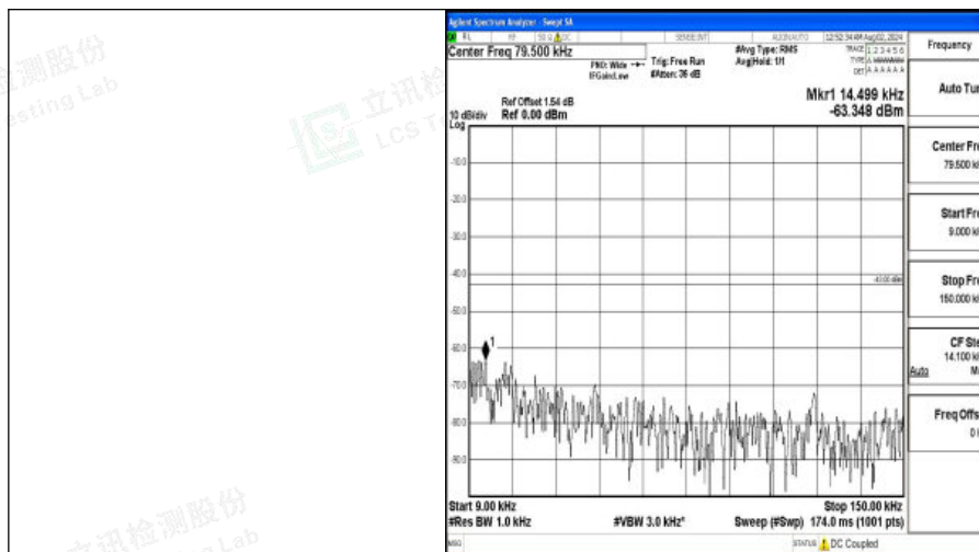
Band4-10MHz-16QAM-20175-1RB#0-0.009~0.15-PASS
