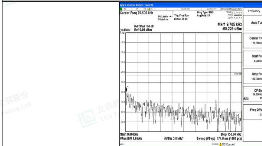
Band4-10MHz-16QAM-20350-1RB#0-0.009~0.15-PASS
