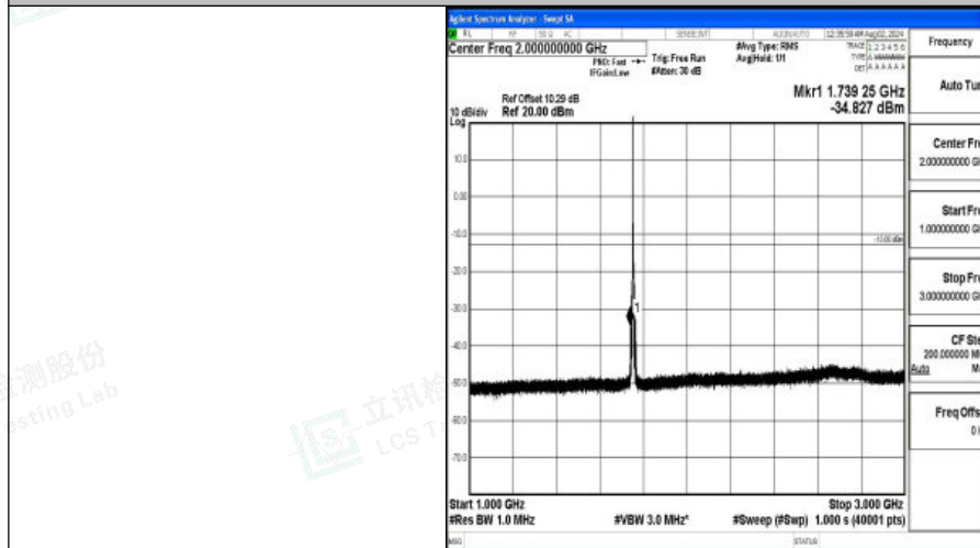
Band4-5MHz-16QAM-20375-1RB#0-1000~3000-PASS
