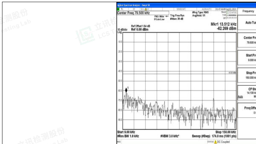
Band4-20MHz-16QAM-20175-1RB#0-0.009~0.15-PASS
