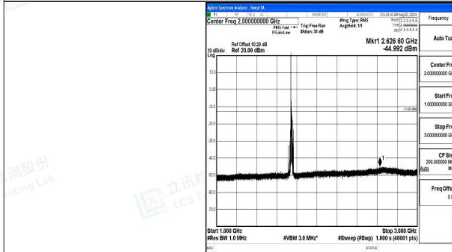
Band4-15MHz-16QAM-20325-1RB#0-1000~3000-PASS
