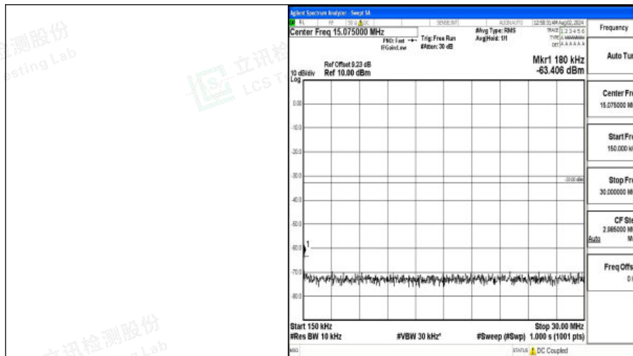
Band4-10MHz-16QAM-20000-1RB#0-0.15~30-PASS
