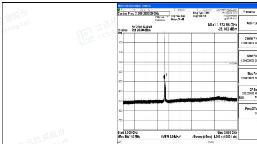
Band4-3MHz-16QAM-20175-1RB#0-1000~3000-PASS
