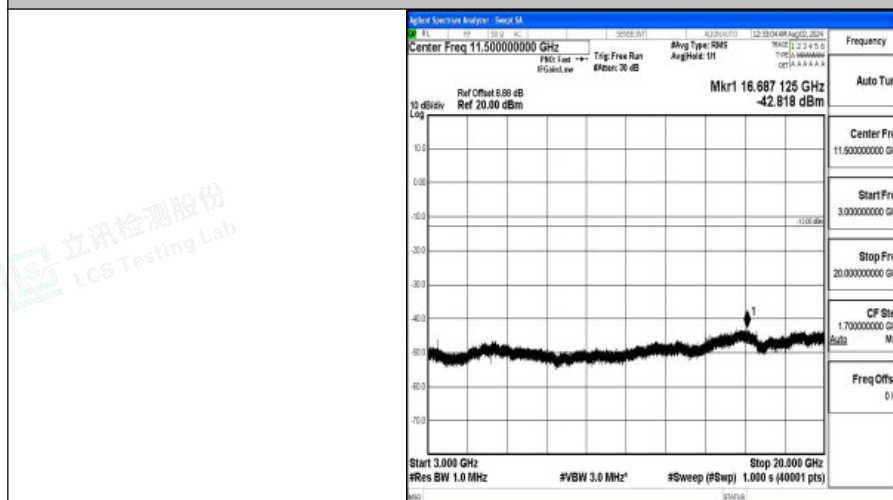
Band4-5MHz-QPSK-20175-1RB#0-3000~20000-PASS
