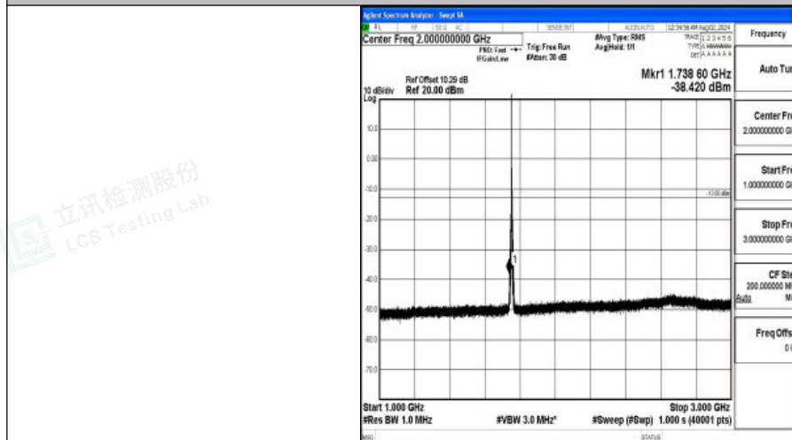
Band4-5MHz-QPSK-20375-1RB#0-1000~3000-PASS
