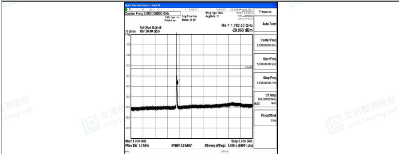
Band4-3MHz-16QAM-20385-1RB#0-1000~3000-PASS
