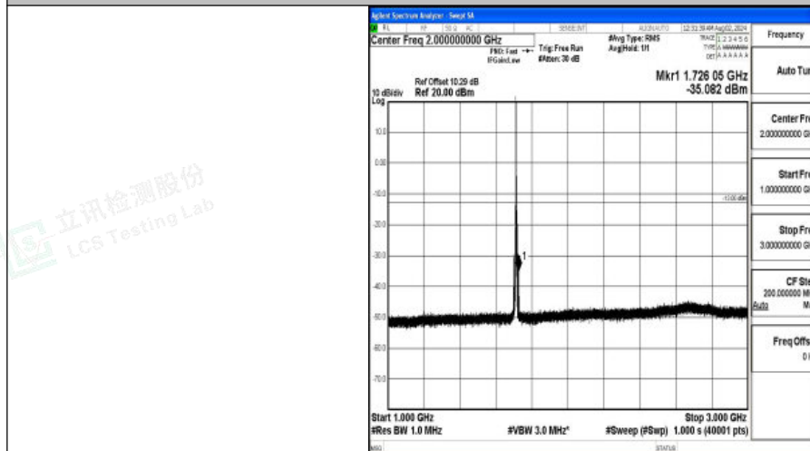
Band4-5MHz-16QAM-19975-1RB#0-1000~3000-PASS
