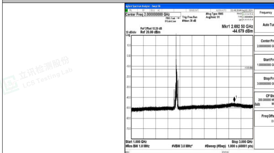
Band4-20MHz-QPSK-20300-1RB#0-1000~3000-PASS
