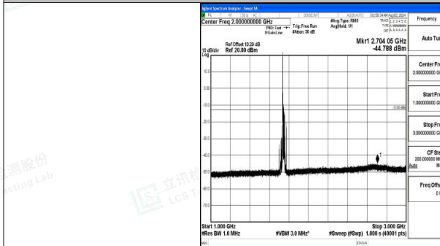
Band4-20MHz-16QAM-20300-1RB#0-1000~3000-PASS
