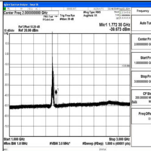
Band4-20MHz-16QAM-20050-1RB#0-1000~3000-PASS
