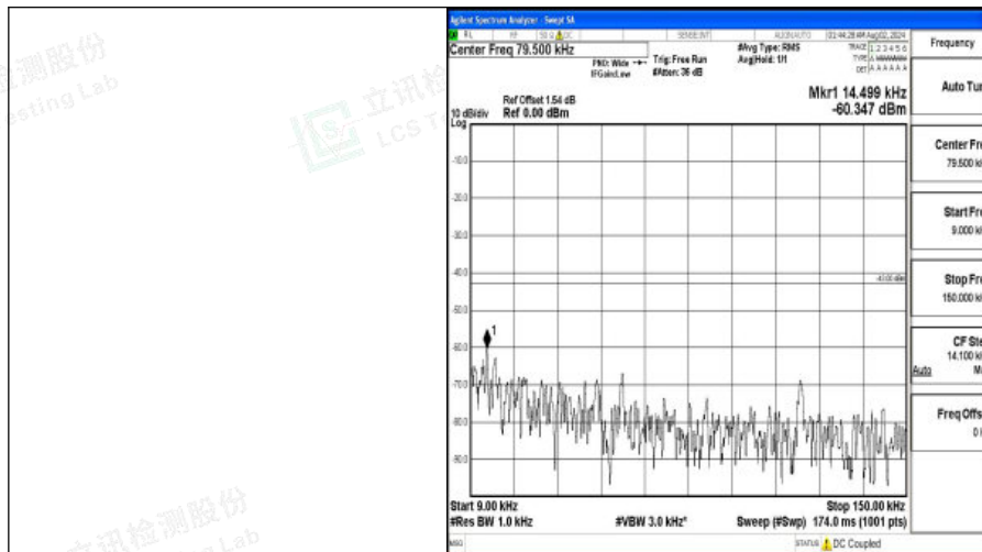
Band4-20MHz-QPSK-20050-1RB#0-0.009~0.15-PASS
