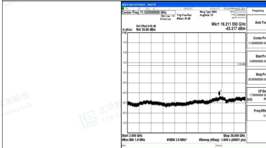
Band4-15MHz-QPSK-20025-1RB#0-3000~20000-PASS
