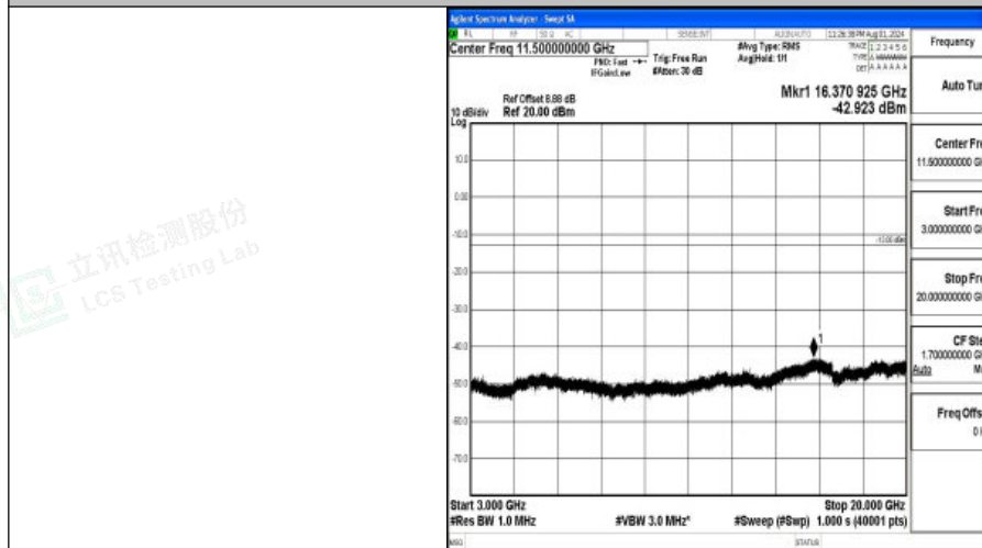
Band4-1.4MHz-16QAM-20393-1RB#0-3000~20000-PASS
