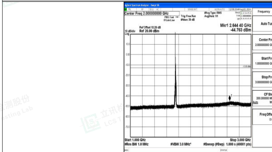
Band4-10MHz-16QAM-20350-1RB#0-1000~3000-PASS
