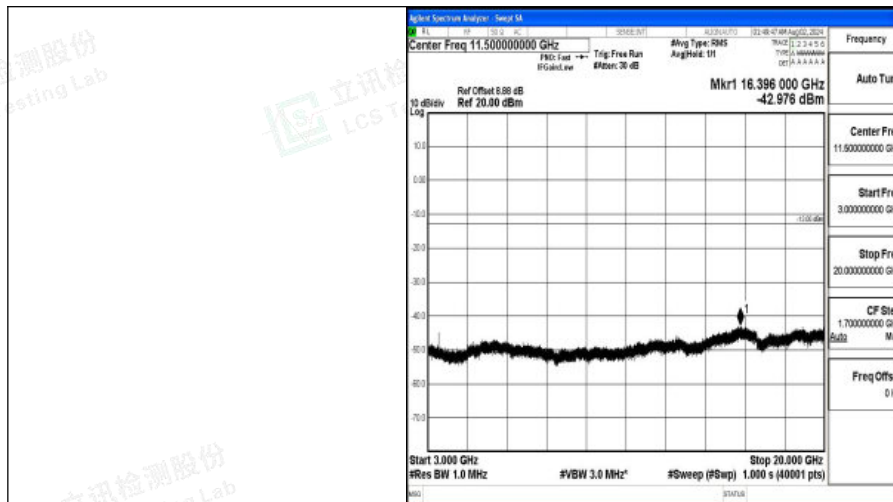
Band4-20MHz-QPSK-20300-1RB#0-3000~20000-PASS
