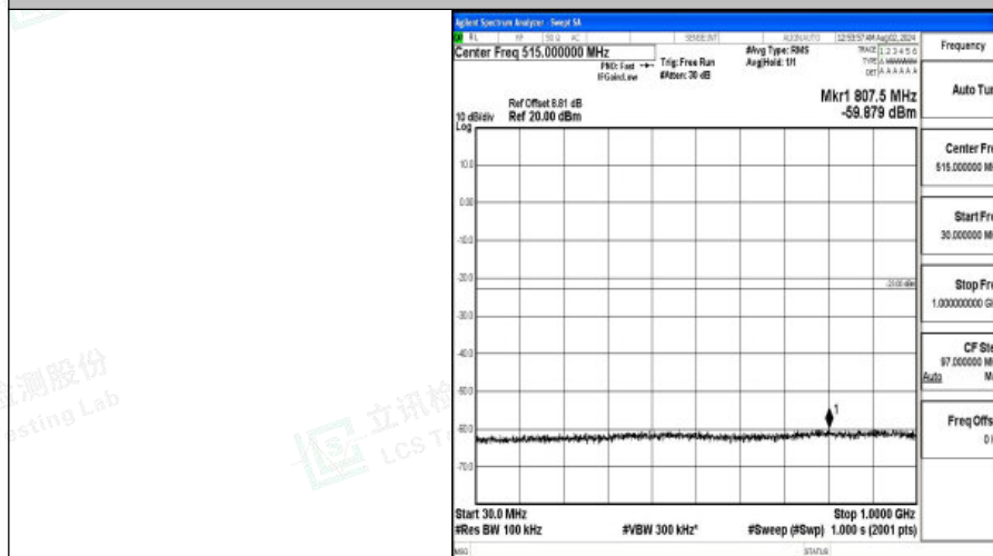
Band4-10MHz-QPSK-20350-1RB#0-30~1000-PASS
