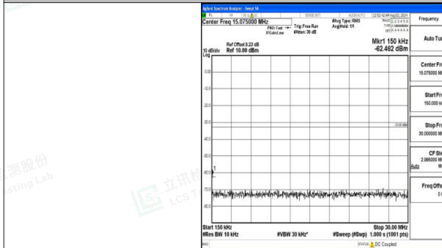
Band4-10MHz-16QAM-20175-1RB#0-0.15~30-PASS
