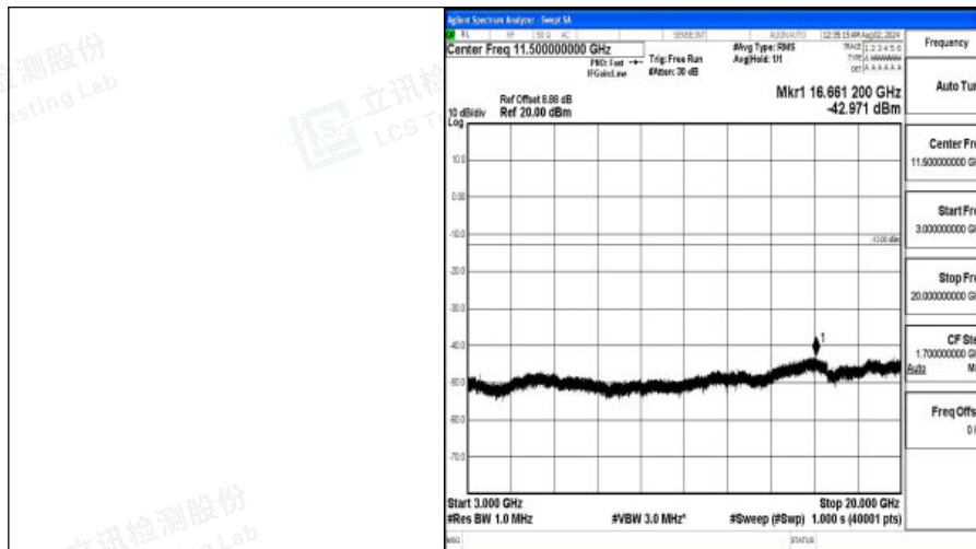
Band4-5MHz-QPSK-20375-1RB#0-3000~20000-PASS
