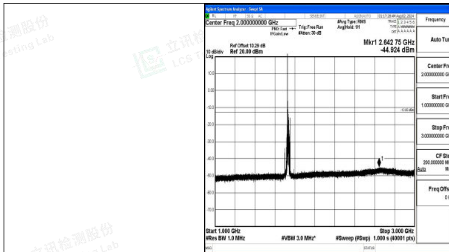
Band4-15MHz-16QAM-20175-1RB#0-1000~3000-PASS
