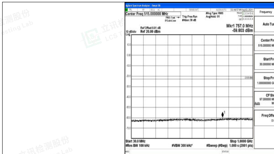
Band4-20MHz-QPSK-20175-1RB#0-30~1000-PASS
