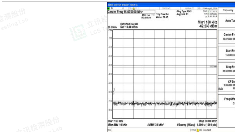
Band4-3MHz-16QAM-19965-1RB#0-0.15~30-PASS
