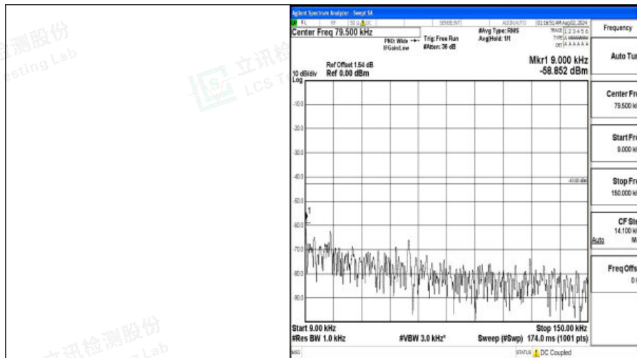
Band4-15MHz-16QAM-20175-1RB#0-0.009~0.15-PASS
