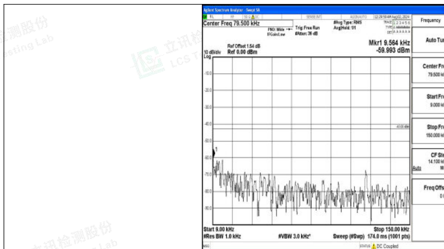
Band4-5MHz-QPSK-19975-1RB#0-0.009~0.15-PASS
