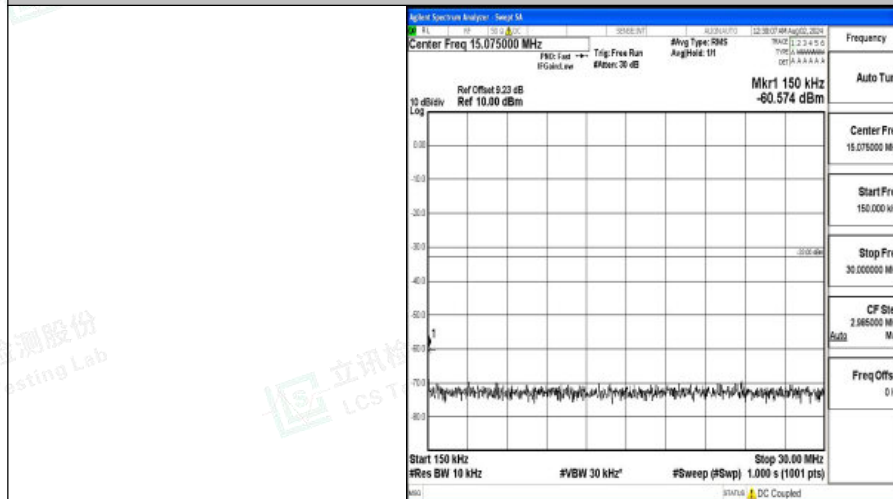
Band4-5MHz-QPSK-19975-1RB#0-0.15~30-PASS
