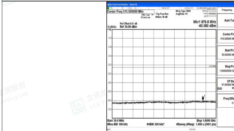
Band4-20MHz-QPSK-20300-1RB#0-30~1000-PASS
