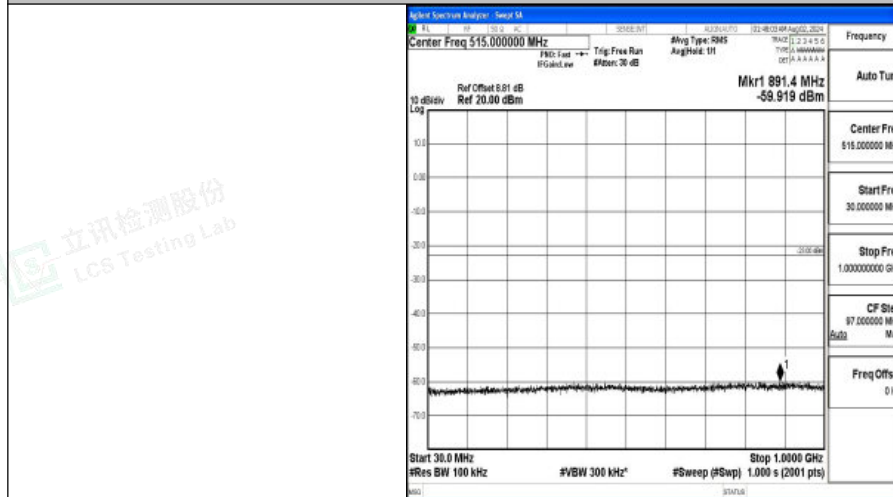
Band4-20MHz-16QAM-20175-1RB#0-30~1000-PASS
