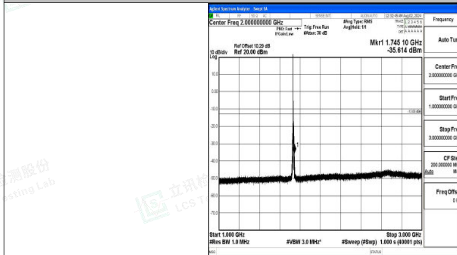
Band4-5MHz-QPSK-20175-1RB#0-1000~3000-PASS
