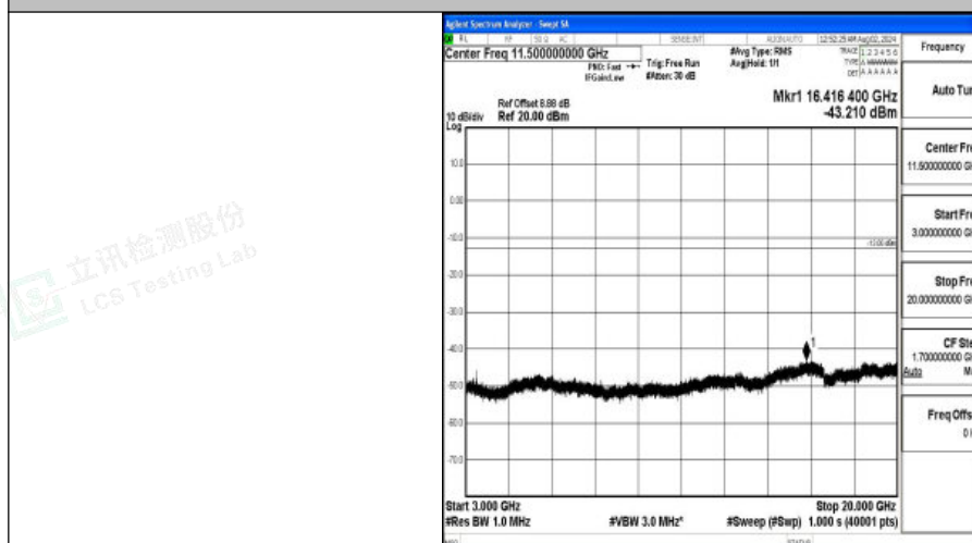
Band4-10MHz-QPSK-20175-1RB#0-3000~20000-PASS
