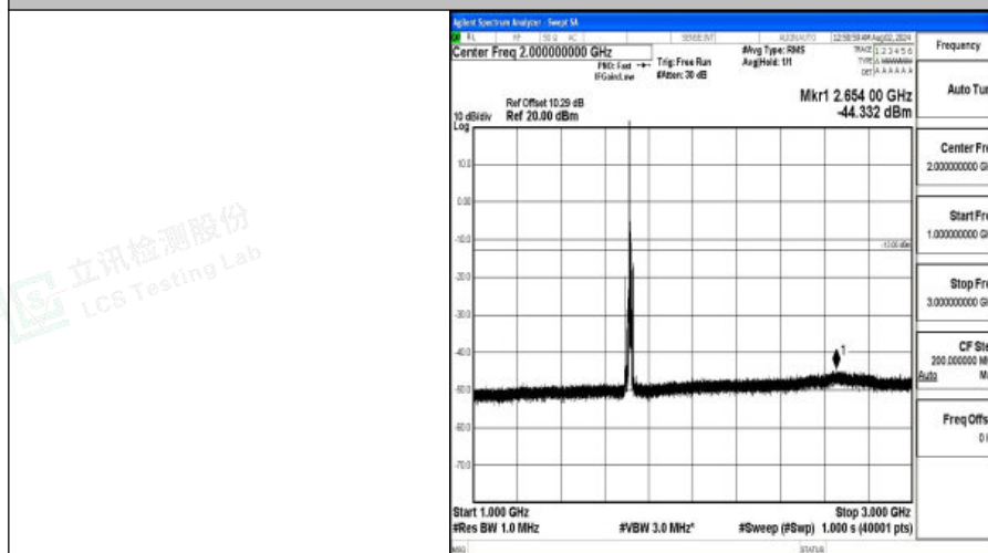
Band4-10MHz-16QAM-20000-1RB#0-1000~3000-PASS
