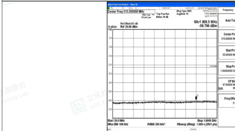
Band4-5MHz-QPSK-20375-1RB#0-30~1000-PASS
