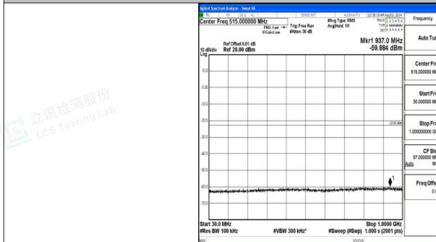
Band4-5MHz-QPSK-19975-1RB#0-30~1000-PASS
