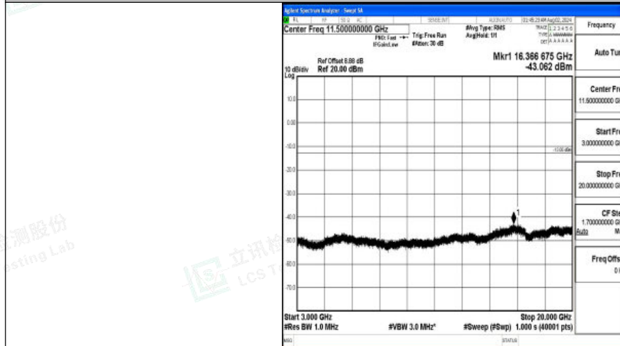
Band4-20MHz-QPSK-20050-1RB#0-3000~20000-PASS
