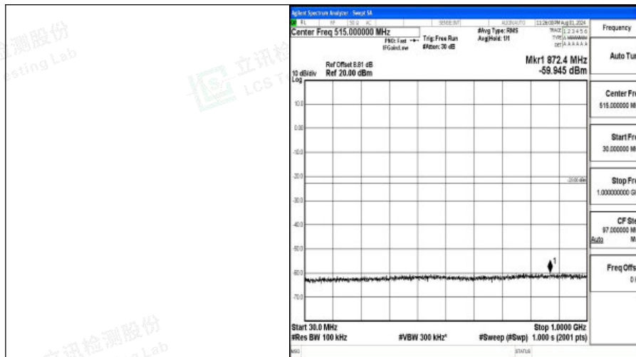
Band4-1.4MHz-16QAM-20393-1RB#0-30~1000-PASS
