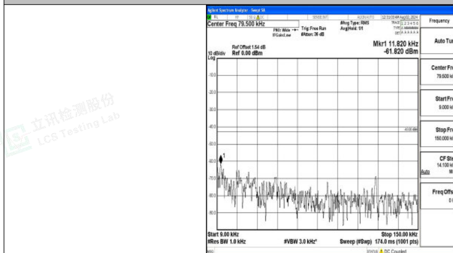
Band4-5MHz-16QAM-19975-1RB#0-0.009~0.15-PASS
