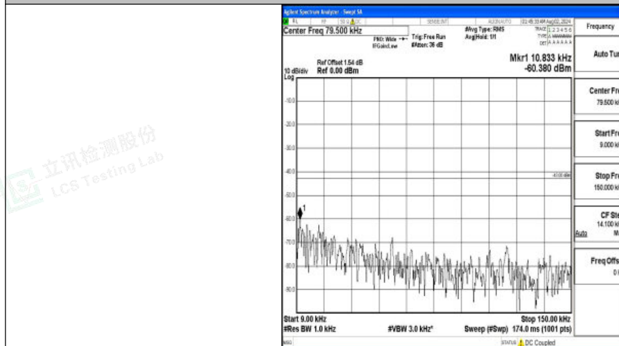
Band4-20MHz-16QAM-20050-1RB#0-0.009~0.15-PASS
