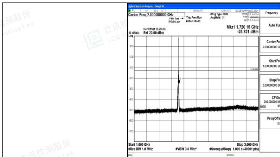
Band4-3MHz-QPSK-19965-1RB#0-1000~3000-PASS
