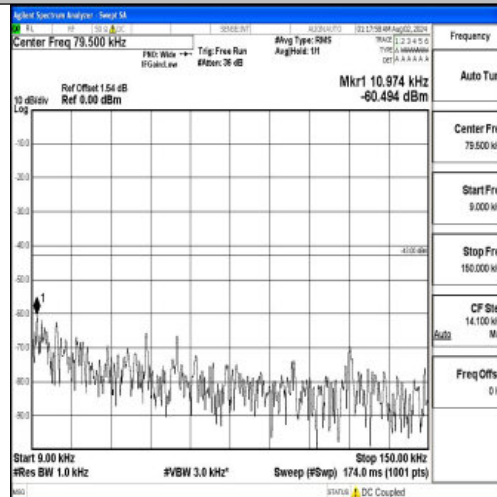
Band4-15MHz-QPSK-20325-1RB#0-0.009~0.15-PASS
