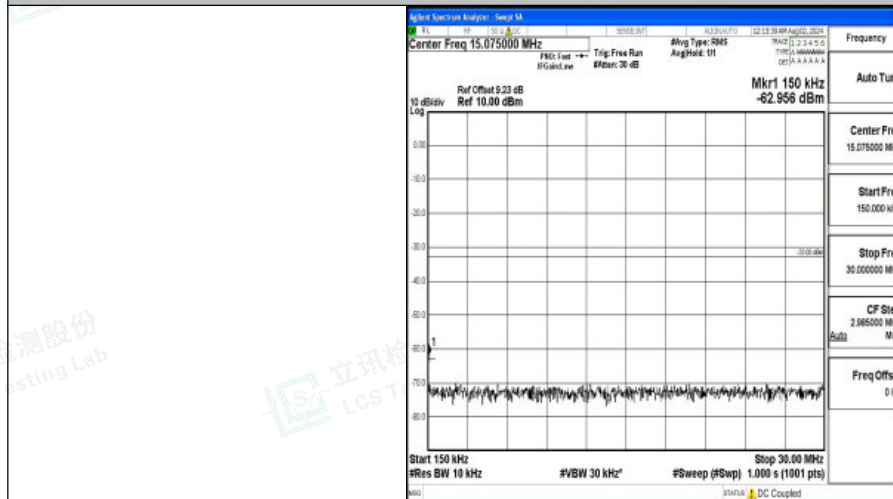
Band4-3MHz-16QAM-20175-1RB#0-0.15~30-PASS
