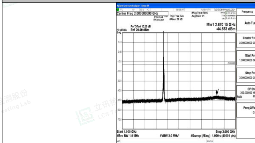
Band4-10MHz-QPSK-20175-1RB#0-1000~3000-PASS
