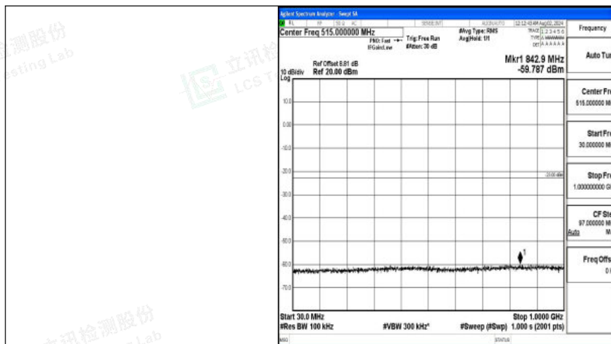
Band4-3MHz-QPSK-20175-1RB#0-30~1000-PASS
