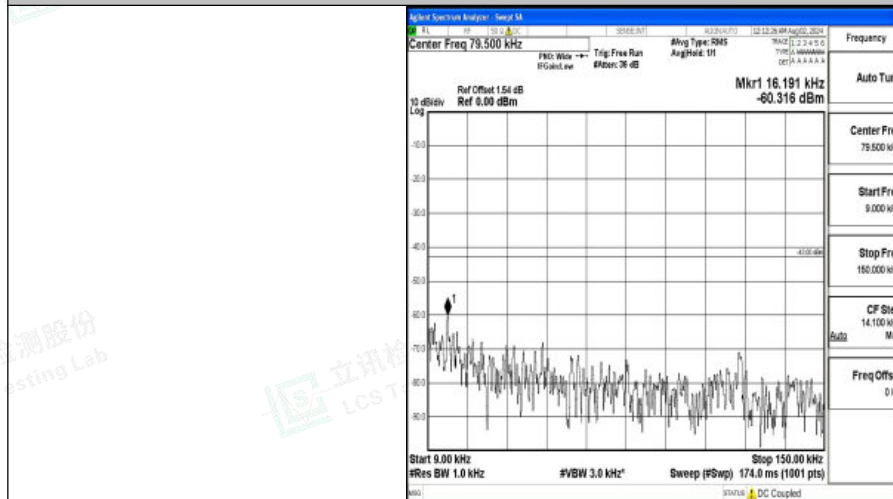
Band4-3MHz-QPSK-20175-1RB#0-0.009~0.15-PASS
