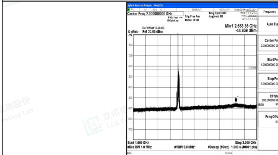
Band4-15MHz-QPSK-20175-1RB#0-1000~3000-PASS
