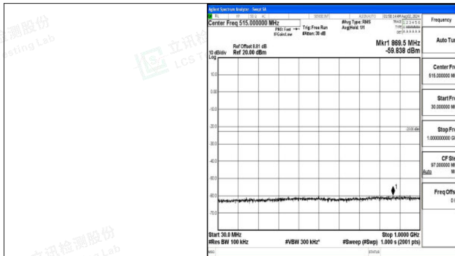
Band4-20MHz-16QAM-20300-1RB#0-30~1000-PASS
