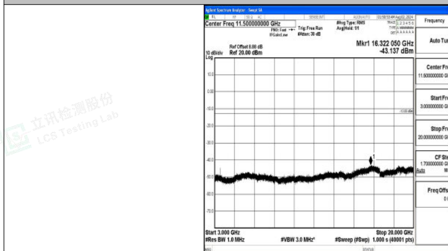
Band4-20MHz-16QAM-20300-1RB#0-3000~20000-PASS
