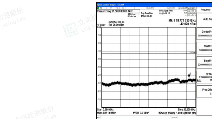
Band4-3MHz-16QAM-19965-1RB#0-3000~20000-PASS
