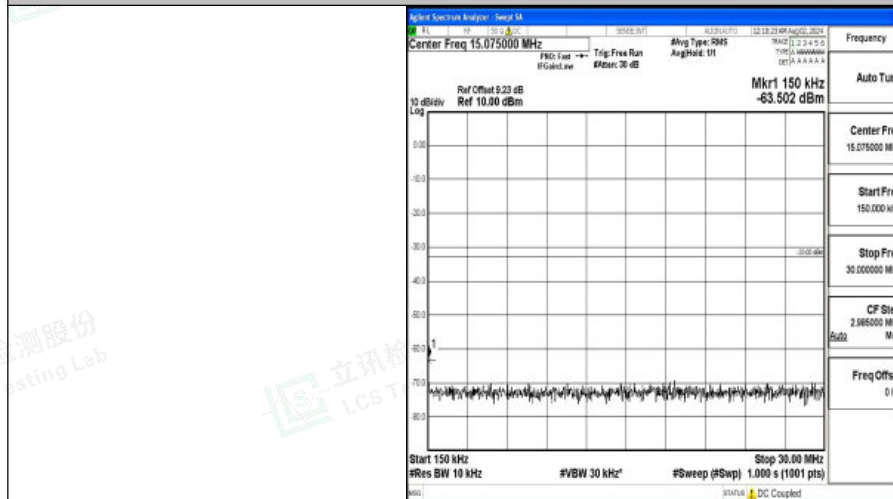
Band4-3MHz-QPSK-19965-1RB#0-0.15~30-PASS
