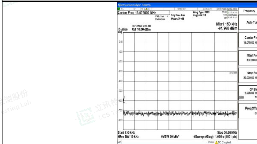
Band4-5MHz-16QAM-20175-1RB#0-0.15~30-PASS
