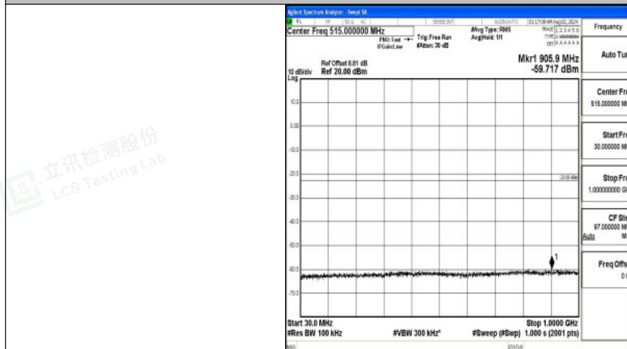
Band4-15MHz-16QAM-20175-1RB#0-30~1000-PASS
