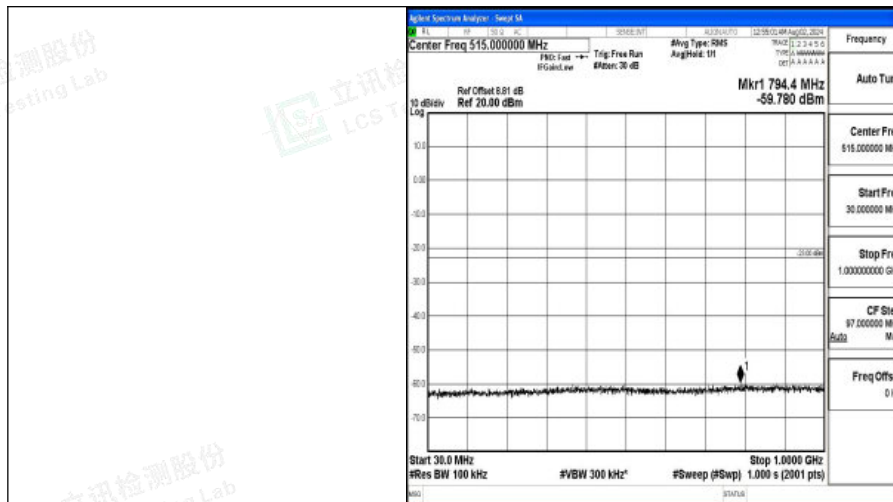
Band4-10MHz-16QAM-20350-1RB#0-30~1000-PASS
