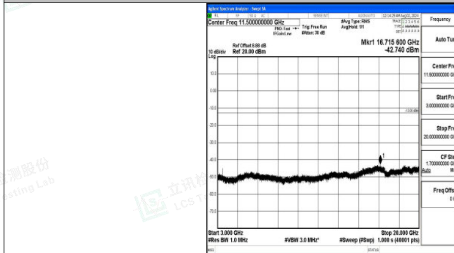
Band4-3MHz-16QAM-20175-1RB#0-3000~20000-PASS
