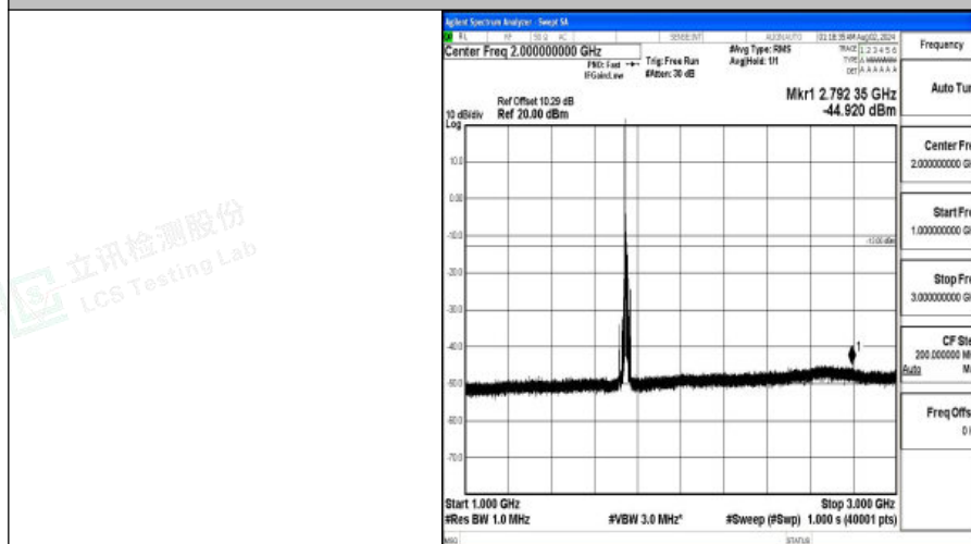
Band4-15MHz-QPSK-20325-1RB#0-1000~3000-PASS
