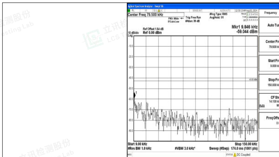
Band4-5MHz-16QAM-20175-1RB#0-0.009~0.15-PASS
