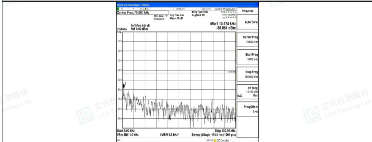
Band4-10MHz-QPSK-20175-1RB#0-0.009~0.15-PASS
