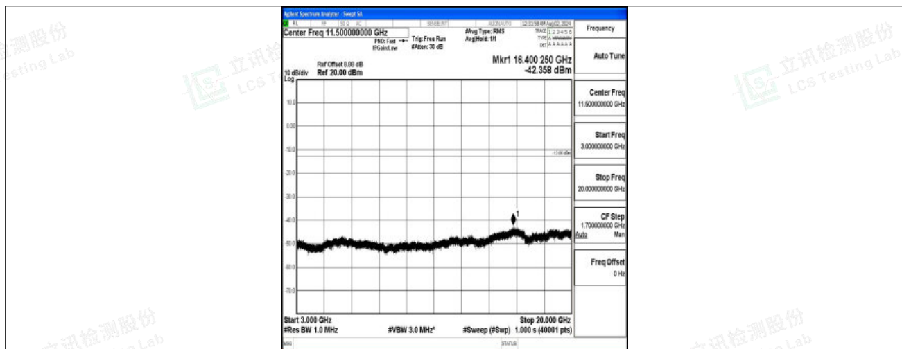
Band4-5MHz-16QAM-19975-1RB#0-3000~20000-PASS
