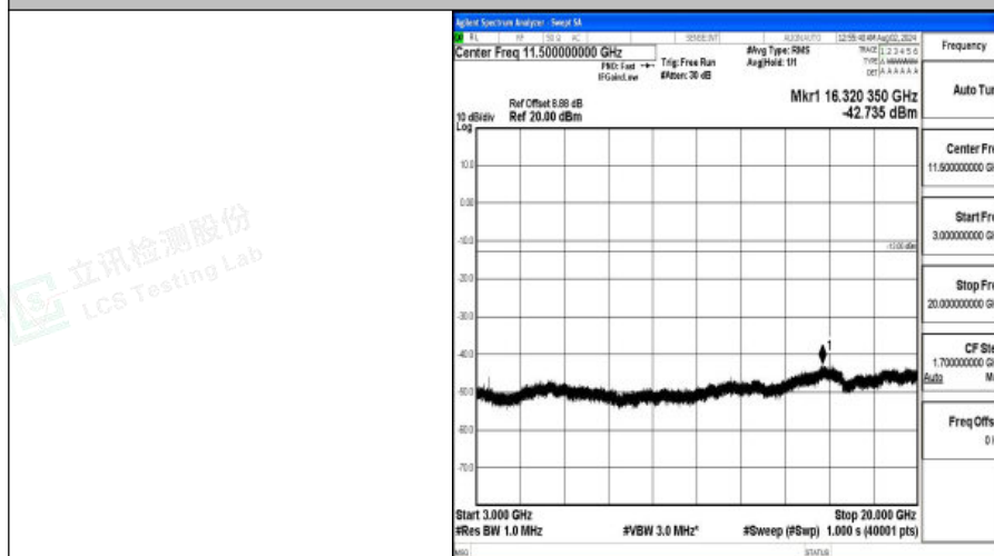
Band4-10MHz-16QAM-20350-1RB#0-3000~20000-PASS
