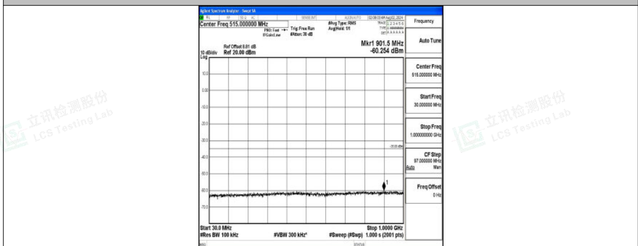
Band7-5MHz-16QAM-20775-1RB#0-30~1000-PASS
