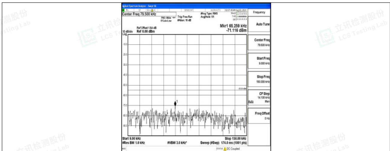
Band7-5MHz-16QAM-20775-1RB#0-0.009~0.15-PASS
