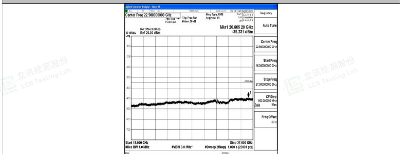
Band7-5MHz-QPSK-21100-1RB#0-18000~27000-PASS
