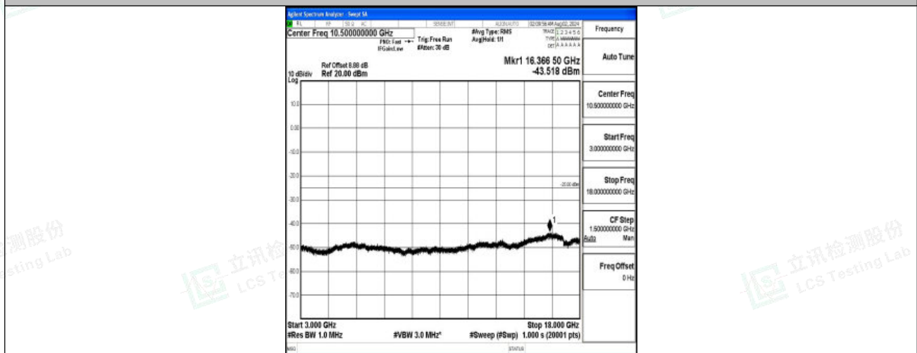
Band7-5MHz-QPSK-21100-1RB#0-3000~18000-PASS
