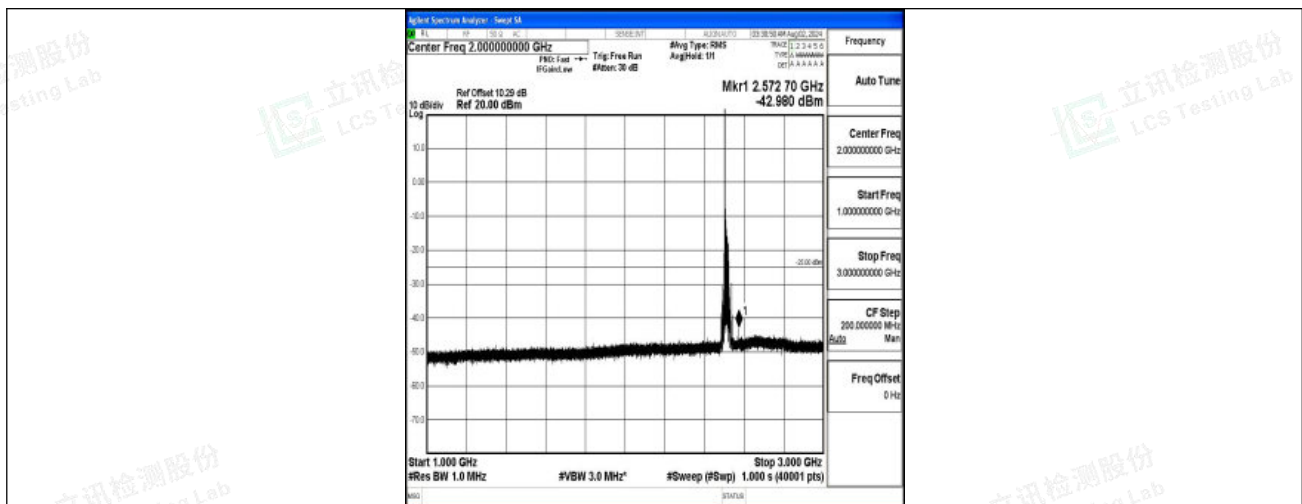
Band7-20MHz-16QAM-20850-1RB#0-1000~3000-PASS
