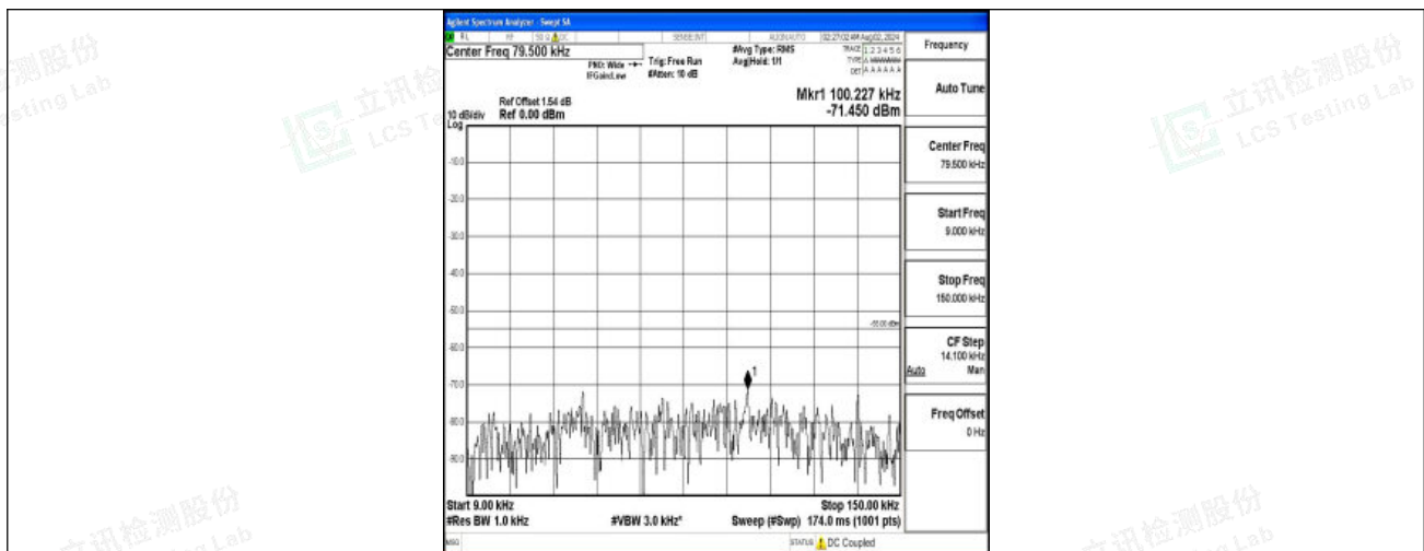
Band7-10MHz-QPSK-20800-1RB#0-0.009~0.15-PASS
