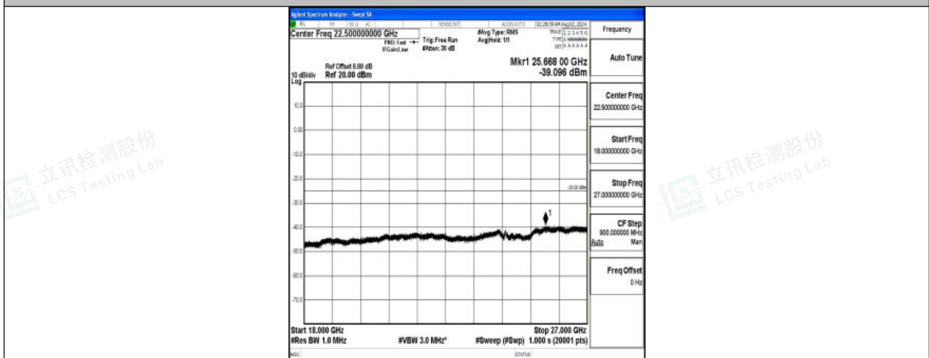
Band7-10MHz-QPSK-20800-1RB#0-18000~27000-PASS
