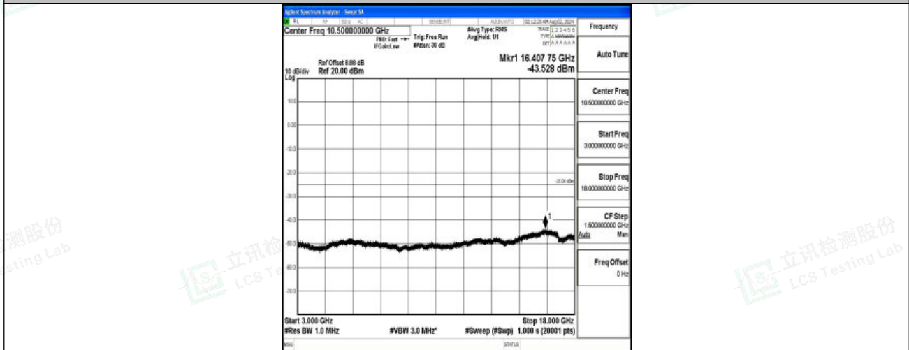
Band7-5MHz-QPSK-21425-1RB#0-3000~18000-PASS
