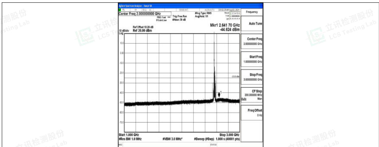
Band7-15MHz-16QAM-21375-1RB#0-1000~3000-PASS
