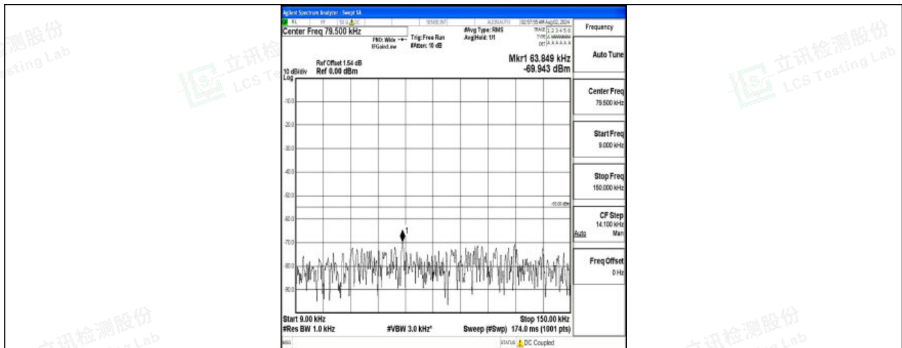
Band7-15MHz-QPSK-21100-1RB#0-0.009~0.15-PASS
