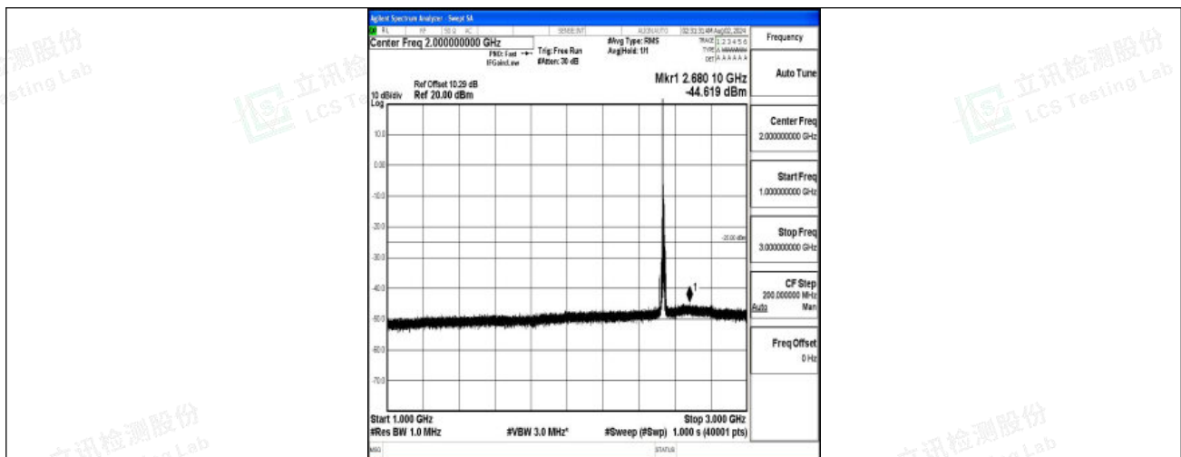
Band7-10MHz-16QAM-21100-1RB#0-1000~3000-PASS
