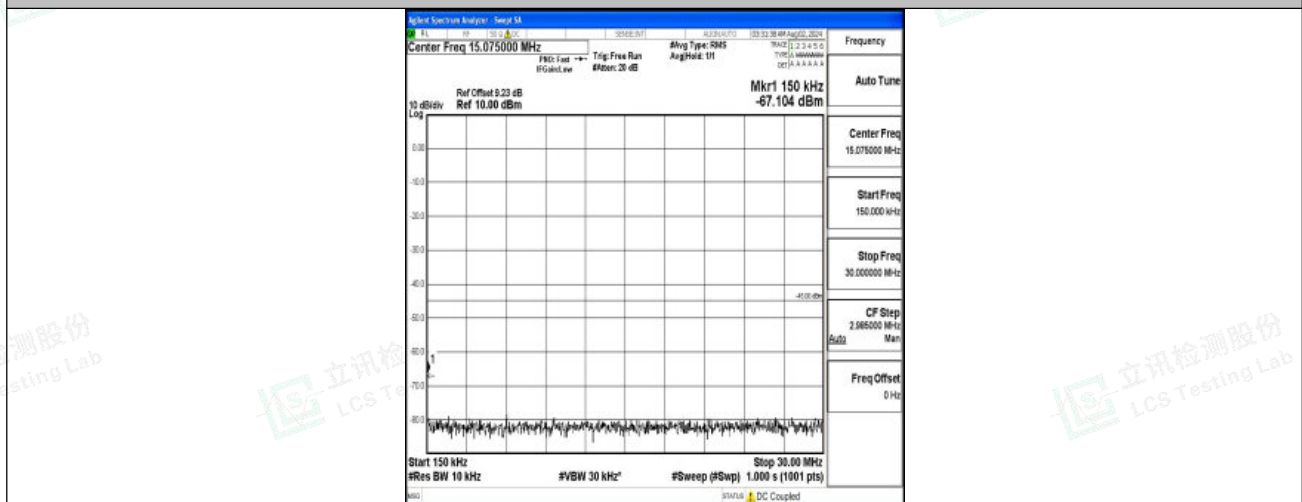
Band7-20MHz-QPSK-21100-1RB#0-0.15~30-PASS
