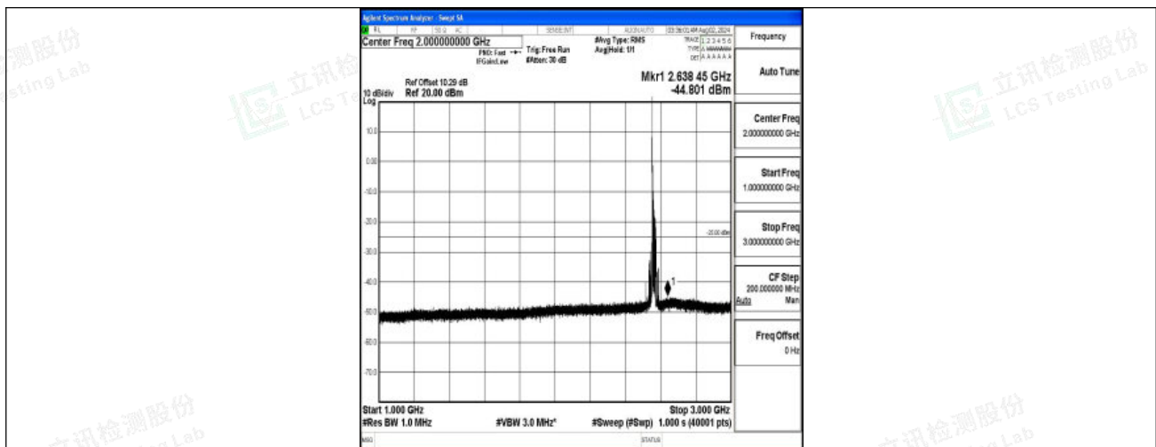
Band7-20MHz-16QAM-21350-1RB#0-1000~3000-PASS
