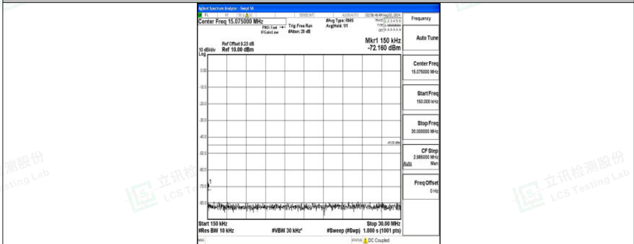
Band 7-15MHz-16QAM-20825-1RB#0-0.15~30-PASS
