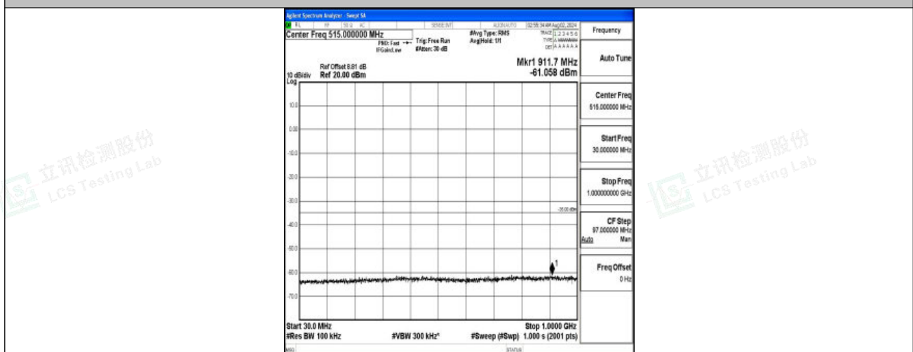
Band7-15MHz-QPSK-20825-1RB#0-30~1000-PASS
