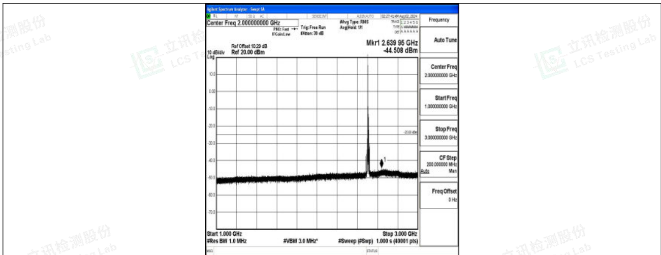
Band7-10MHz-QPSK-20800-1RB#0-1000~3000-PASS
