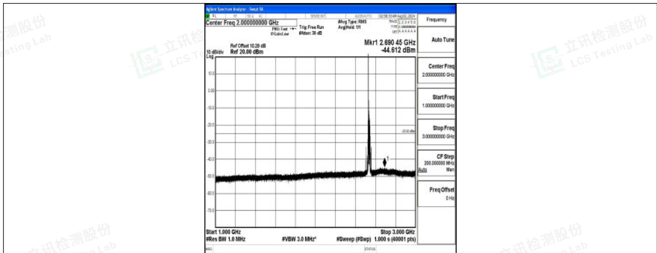
Band7-15MHz-QPSK-21100-1RB#0-1000~3000-PASS
