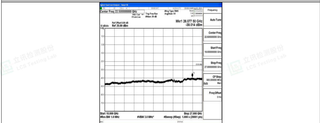
Band7-15MHz-16QAM-21100-1RB#0-18000~27000-PASS
