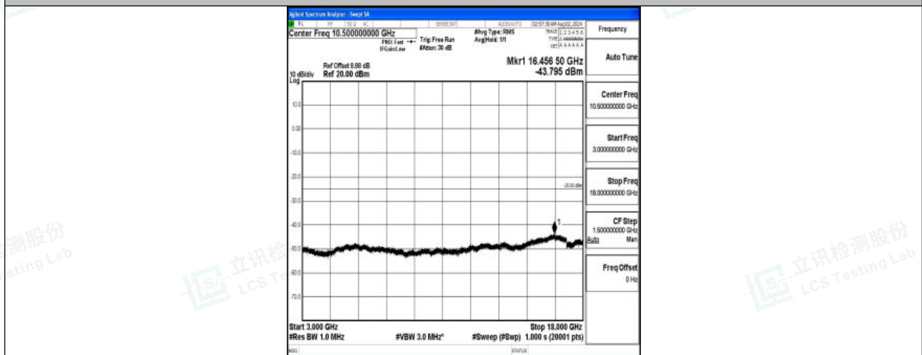
Band7-15MHz-16QAM-20825-1RB#0-3000~18000-PASS
