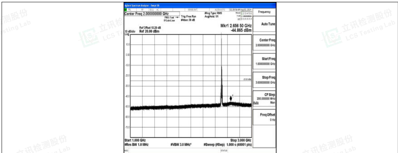
Band7-10MHz-16QAM-20800-1RB#0-1000~3000-PASS
