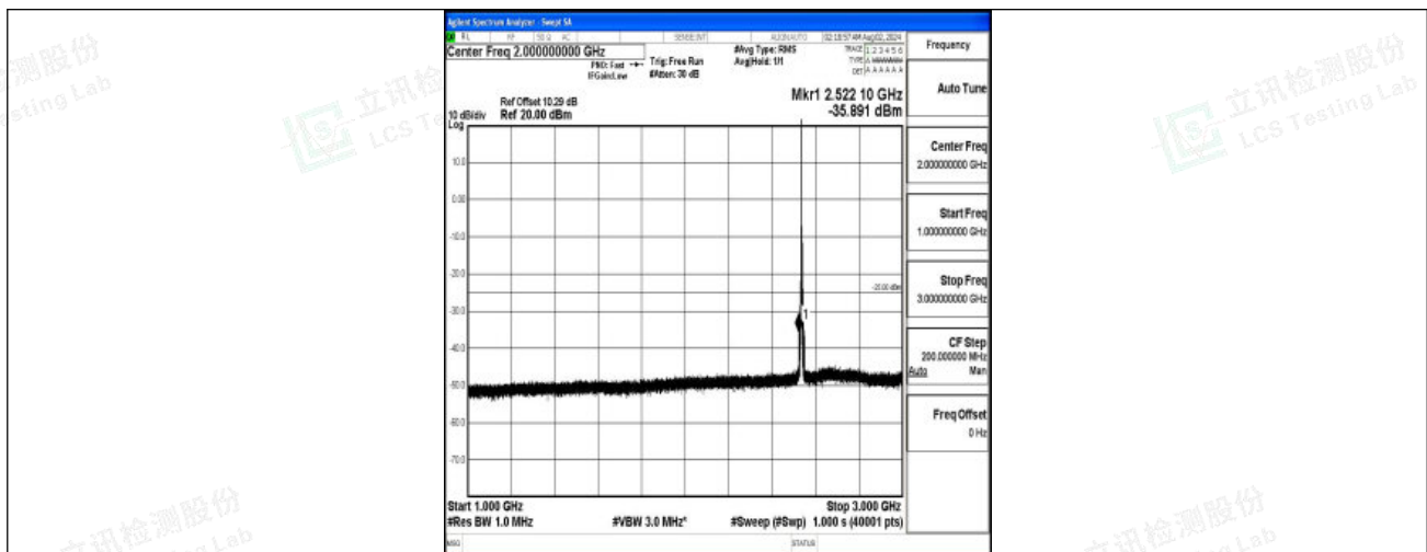
Band7-5MHz-16QAM-21100-1RB#0-1000~3000-PASS
