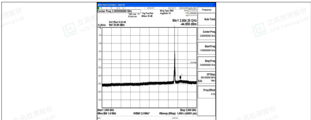
Band7-10MHz-QPSK-21100-1RB#0-1000~3000-PASS
