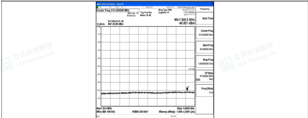
Band7-15MHz-16QAM-21100-1RB#0-30~1000-PASS
