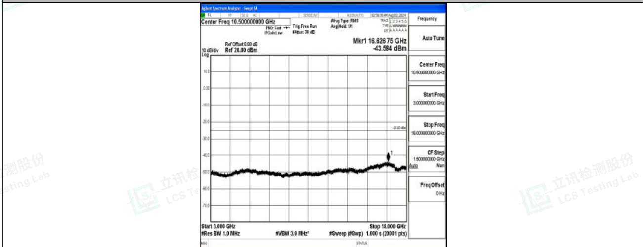
Band7-15MHz-QPSK-20825-1RB#0-3000~18000-PASS
