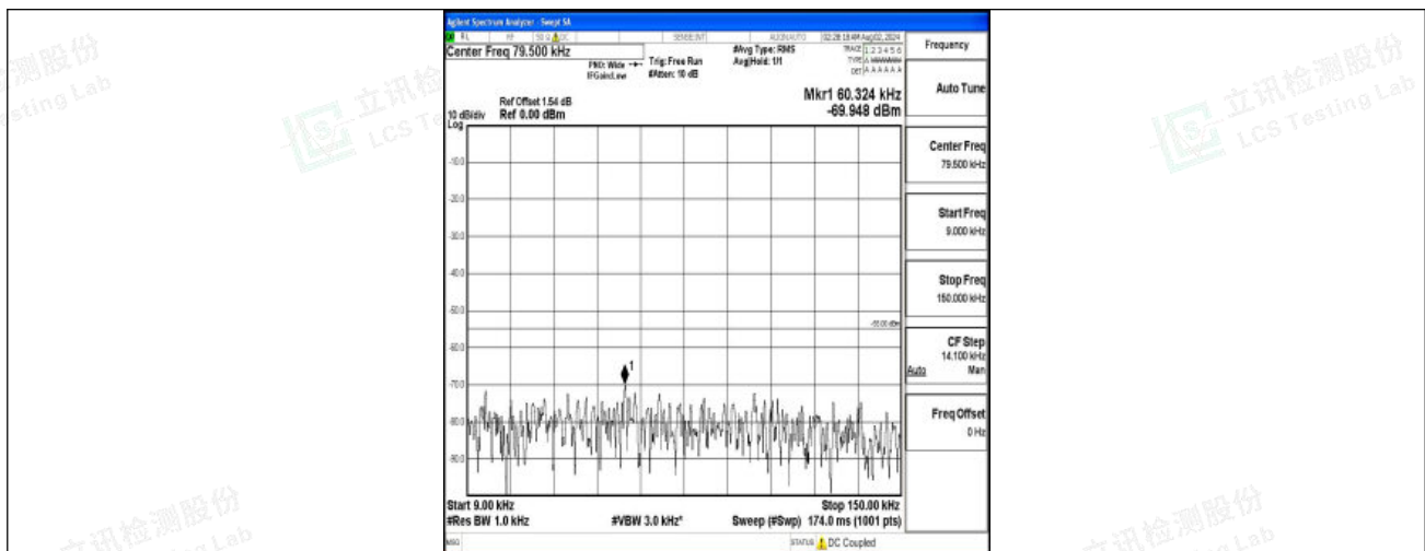
Band7-10MHz-16QAM-20800-1RB#0-0.009~0.15-PASS
