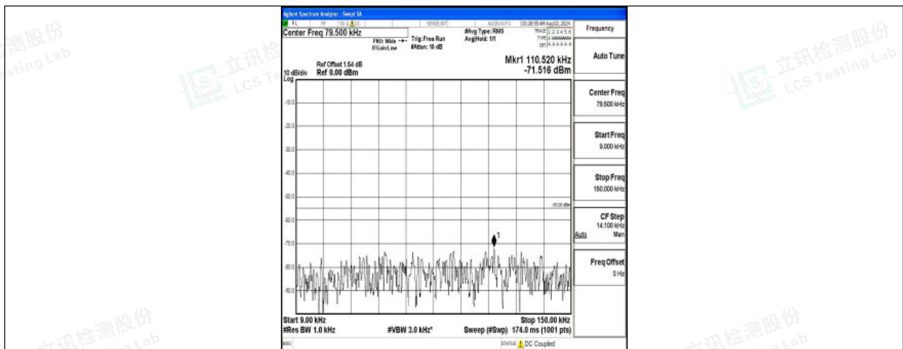
Band7-20MHz-QPSK-20850-1RB#0-0.009~0.15-PASS
