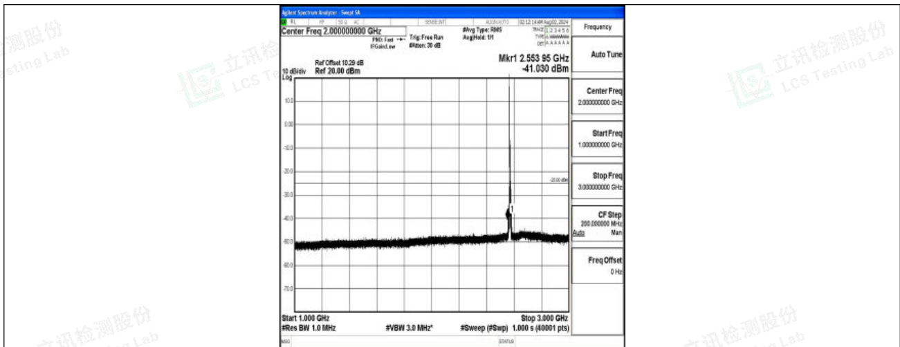
Band7-5MHz-QPSK-21425-1RB#0-1000~3000-PASS
