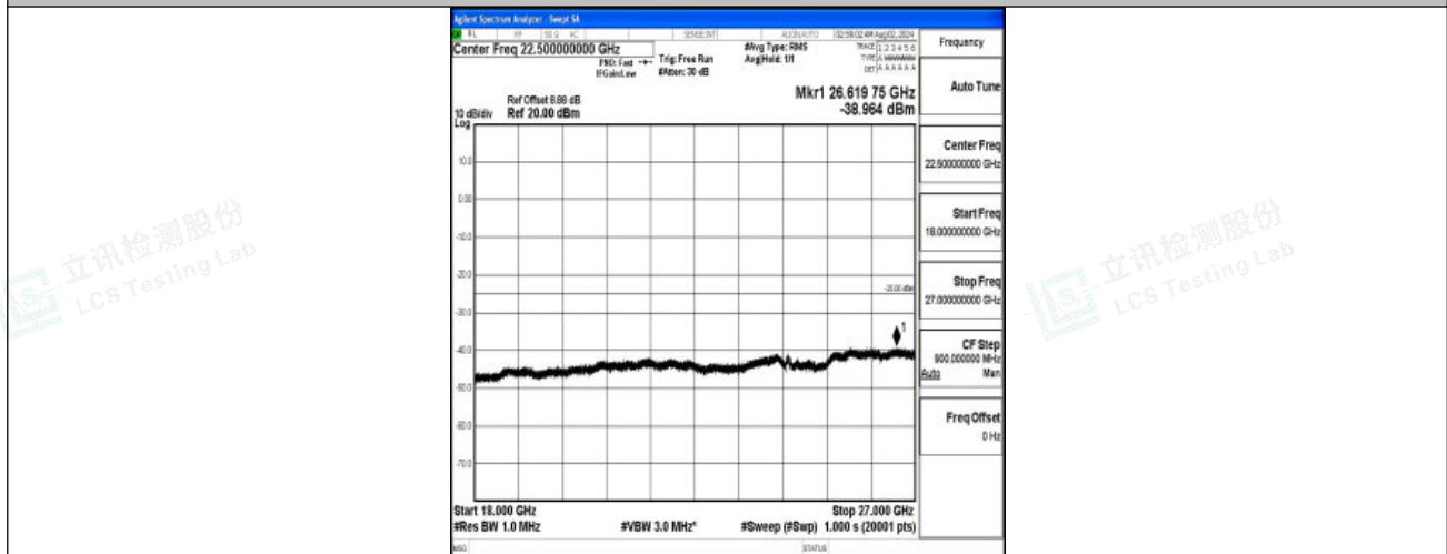
Band7-15MHz-QPSK-21100-1RB#0-18000~27000-PASS
