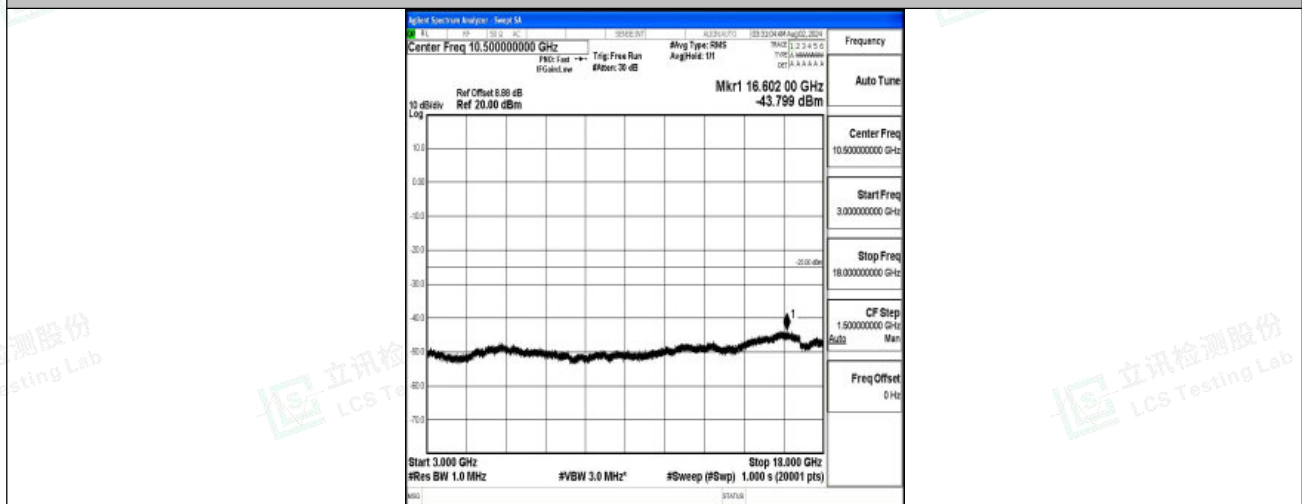
Band7-20MHz-16QAM-20850-1RB#0-3000~18000-PASS
