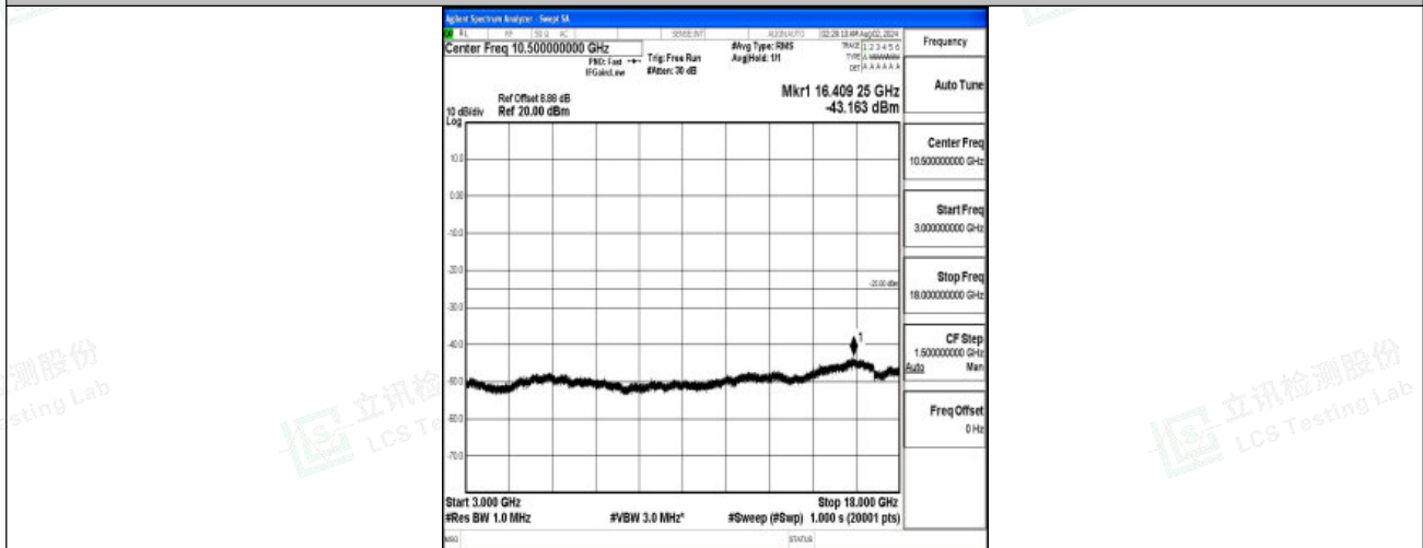
Band7-10MHz-16QAM-20800-1RB#0-3000~18000-PASS
