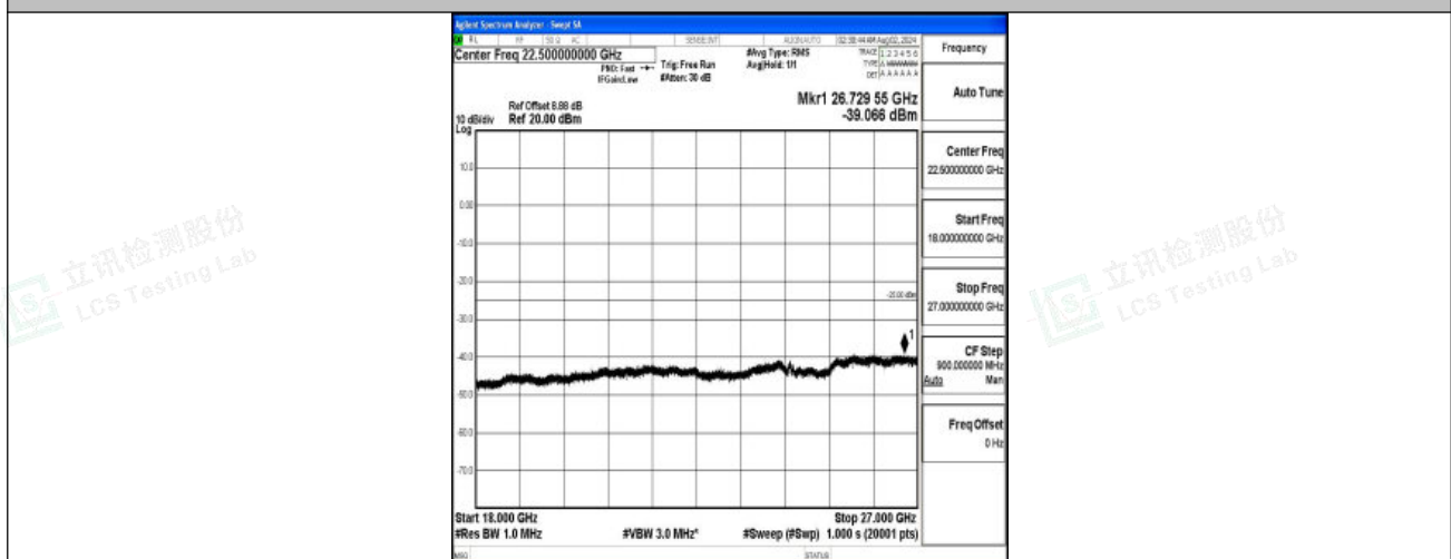
Band7-10MHz-QPSK-21100-1RB#0-18000~27000-PASS
