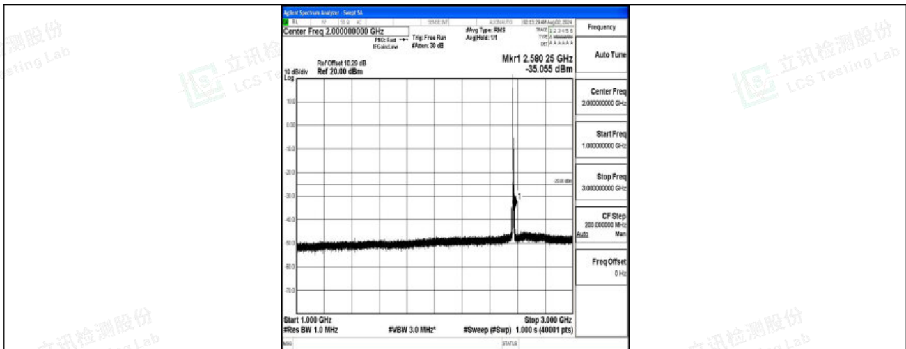
Band7-5MHz-16QAM-21425-1RB#0-1000~3000-PASS
