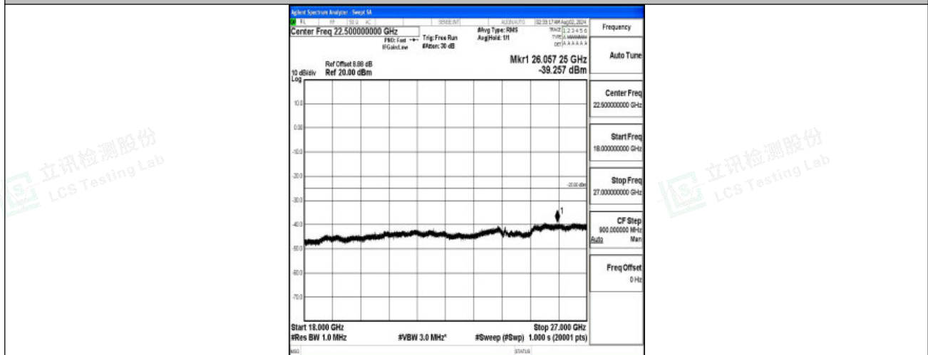
Band7-10MHz-QPSK-21400-1RB#0-18000~27000-PASS
