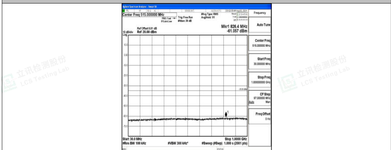
Band 7-15MHz-16QAM-21375-1RB#0-30~1000-PASS
