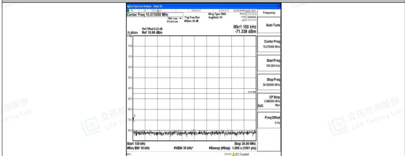
Band7-10MHz-16QAM-20800-1RB#0-0.15~30-PASS
