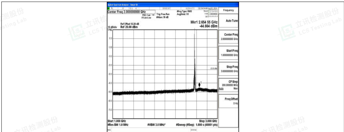
Band7-10MHz-16QAM-21400-1RB#0-1000~3000-PASS
