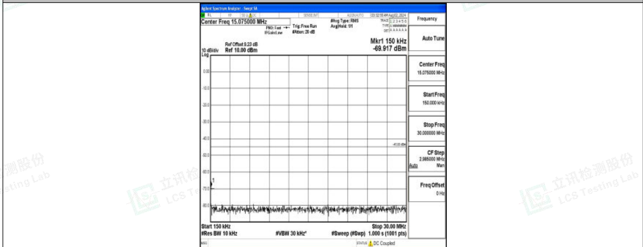
Band7-20MHz-16QAM-21100-1RB#0-0.15~30-PASS
