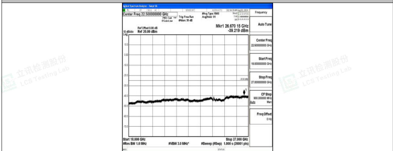
Band7-10MHz-16QAM-21400-1RB#0-18000~27000-PASS
