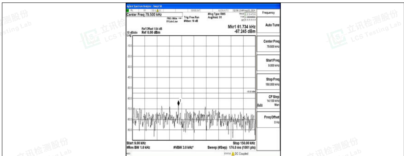
Band7-15MHz-16QAM-21100-1RB#0-0.009~0.15-PASS
