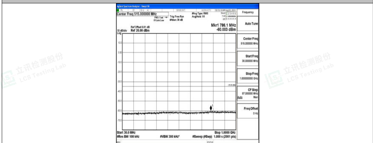
Band7-10MHz-16QAM-21100-1RB#0-30~1000-PASS
