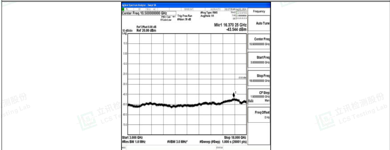
Band7-10MHz-QPSK-20800-1RB#0-3000~18000-PASS
