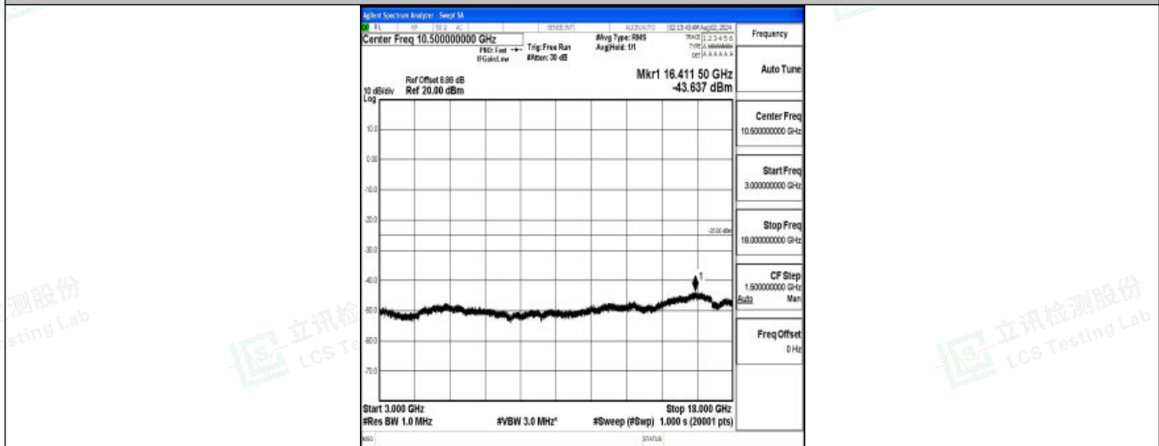
Band7-5MHz-16QAM-21425-1RB#0-3000~18000-PASS
