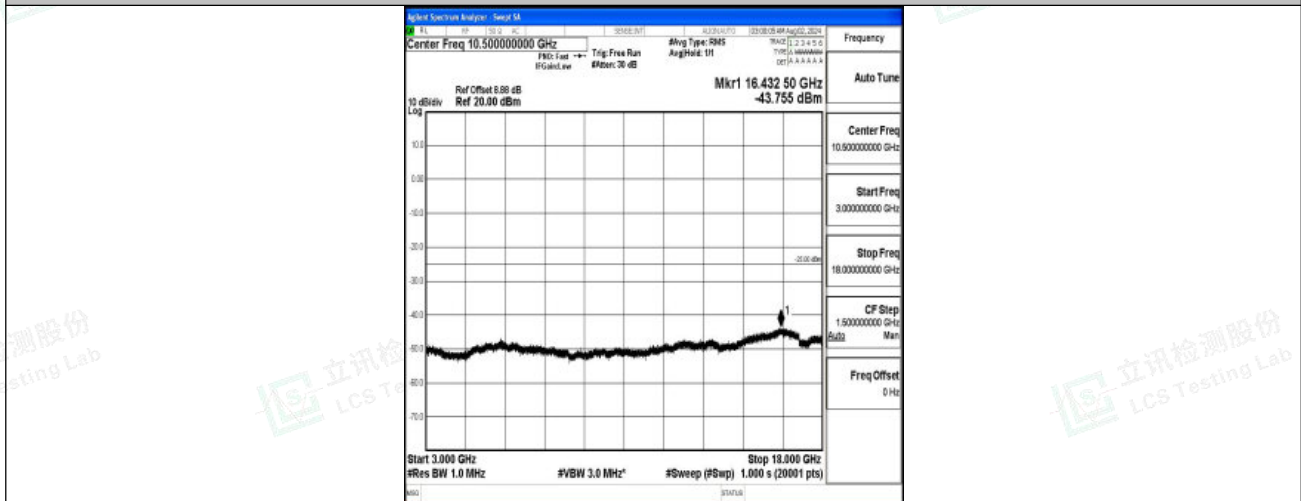
Band7-15MHz-16QAM-21100-1RB#0-3000~18000-PASS
