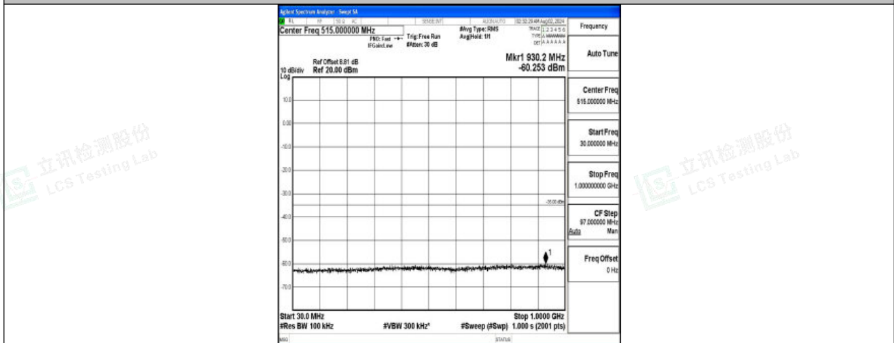
Band7-10MHz-QPSK-21400-1RB#0-30~1000-PASS
