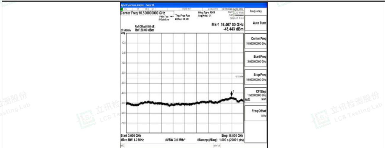
Band7-10MHz-QPSK-21400-1RB#0-3000~18000-PASS
