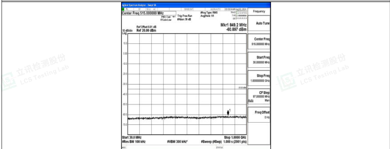
Band7-20MHz-16QAM-21100-1RB#0-30~1000-PASS
