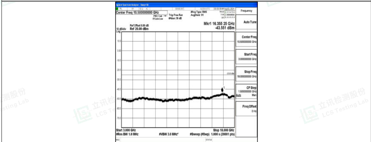
Band7-20MHz-16QAM-21100-1RB#0-3000~18000-PASS
