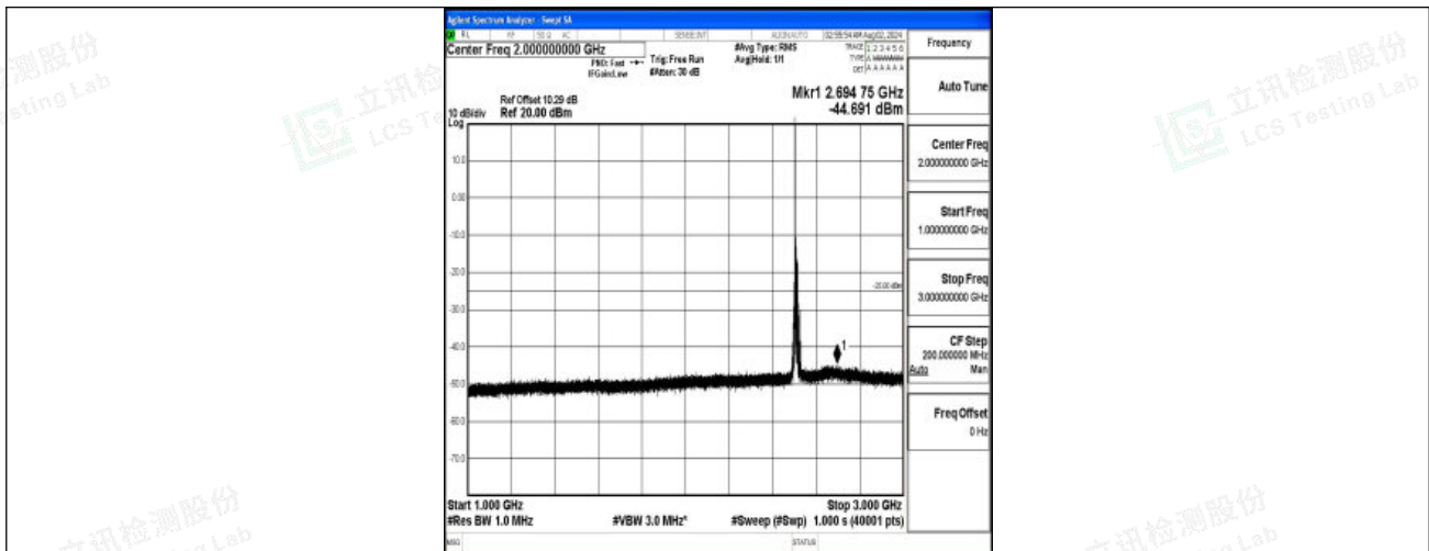
Band7-15MHz-QPSK-20825-1RB#0-1000~3000-PASS
