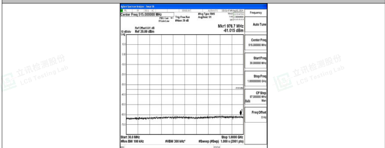
Band7-20MHz-QPSK-21100-1RB#0-30~1000-PASS
