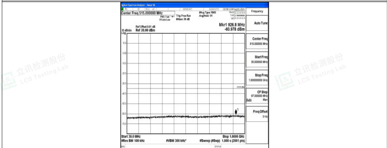
Band7-15MHz-QPSK-21100-1RB#0-30~1000-PASS
