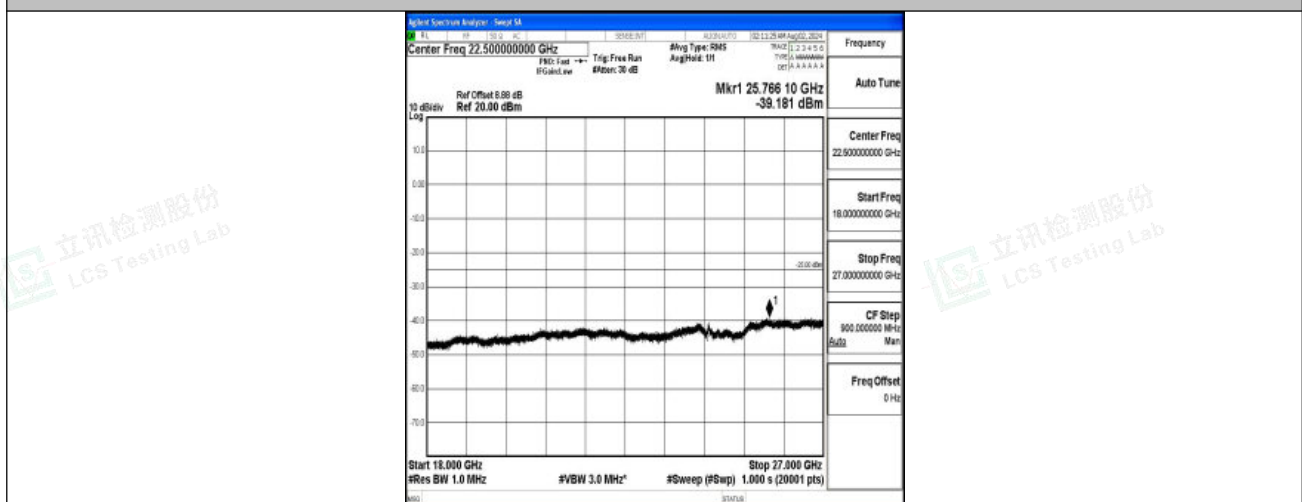
Band7-5MHz-16QAM-21100-1RB#0-18000~27000-PASS
