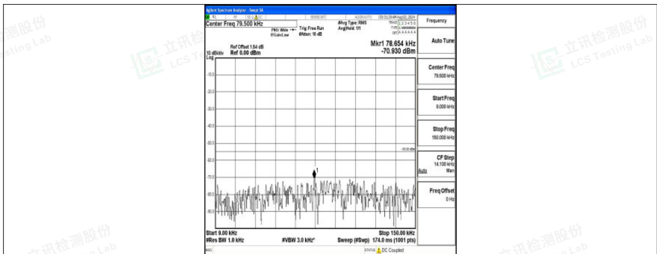
Band7-20MHz-QPSK-21100-1RB#0-0.009~0.15-PASS
