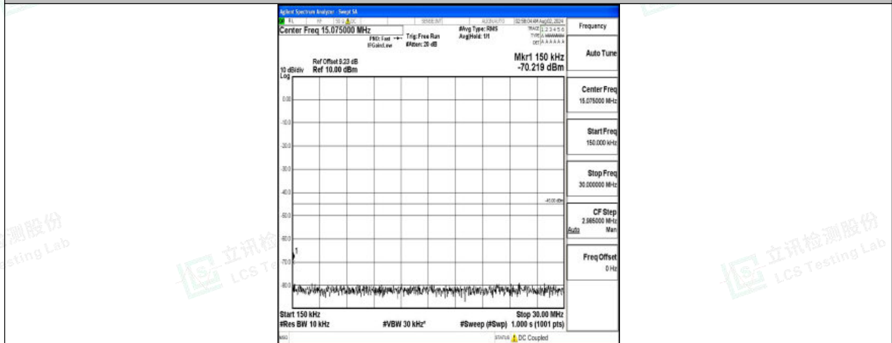
Band7-15MHz-QPSK-21100-1RB#0-0.15~30-PASS
