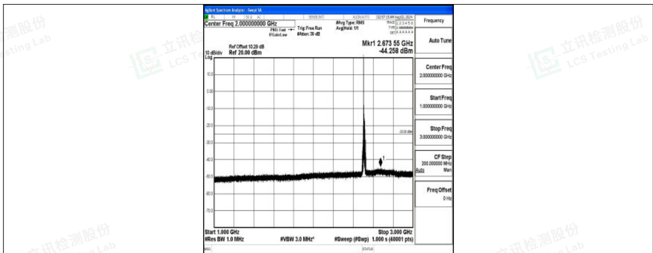
Band7-15MHz-16QAM-20825-1RB#0-1000~3000-PASS
