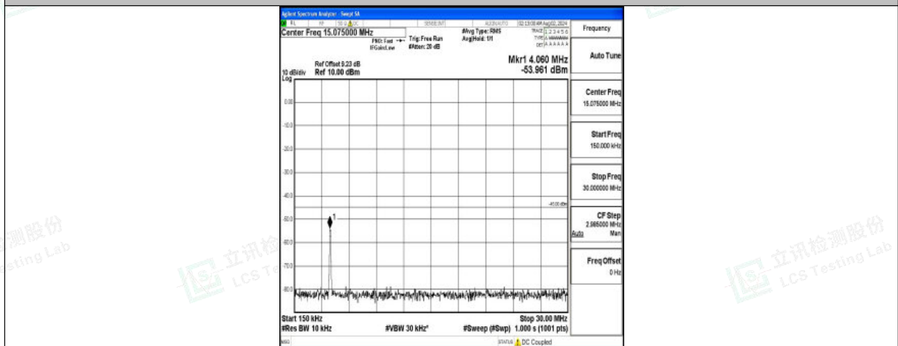
Band7-5MHz-16QAM-21425-1RB#0-0.15~30-PASS
