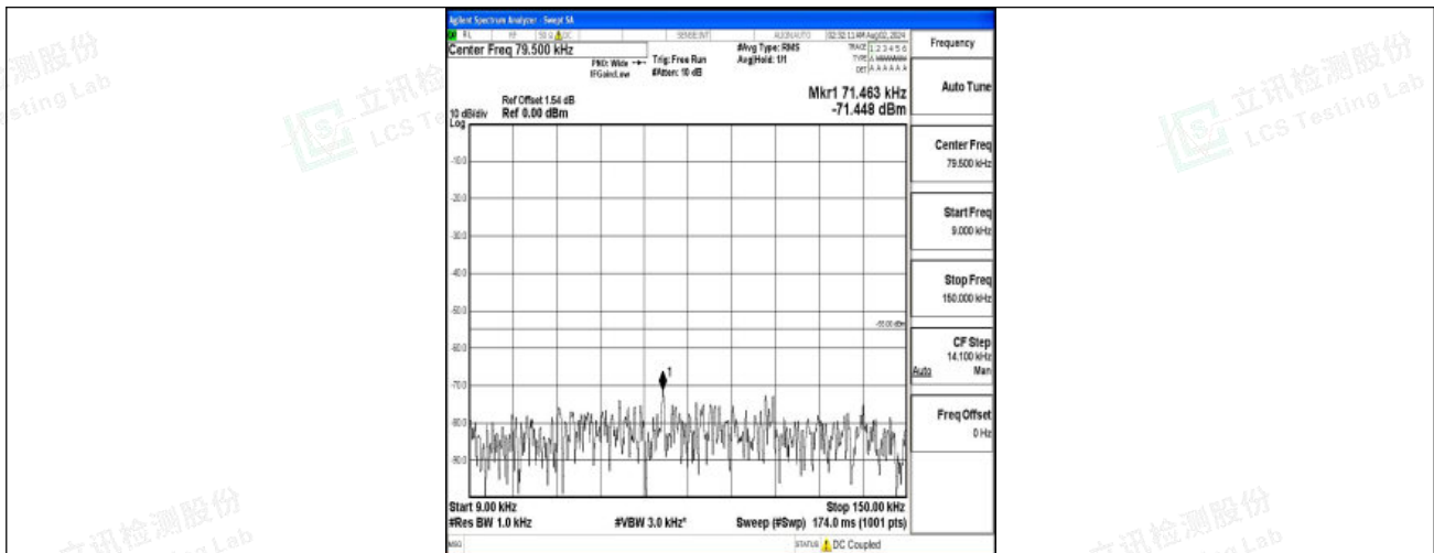
Band7-10MHz-QPSK-21400-1RB#0-0.009~0.15-PASS
