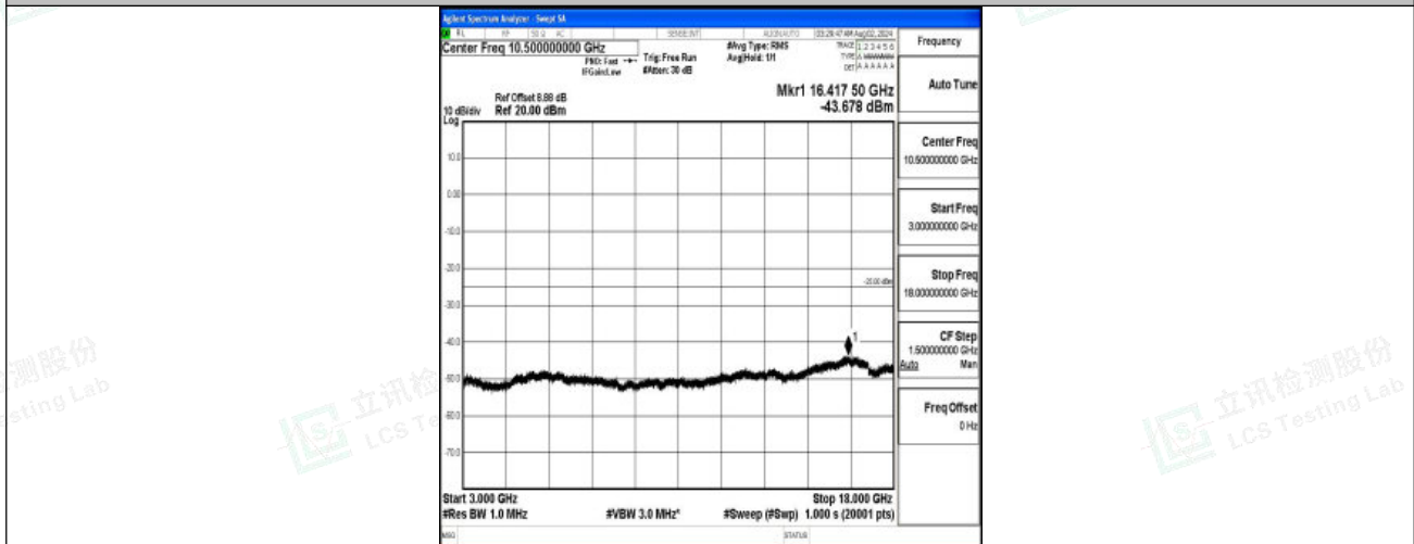
Band7-20MHz-QPSK-20850-1RB#0-3000~18000-PASS
