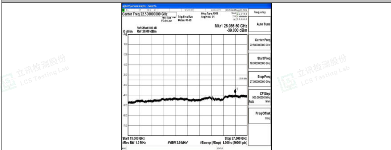
Band7-10MHz-16QAM-20800-1RB#0-18000~27000-PASS
