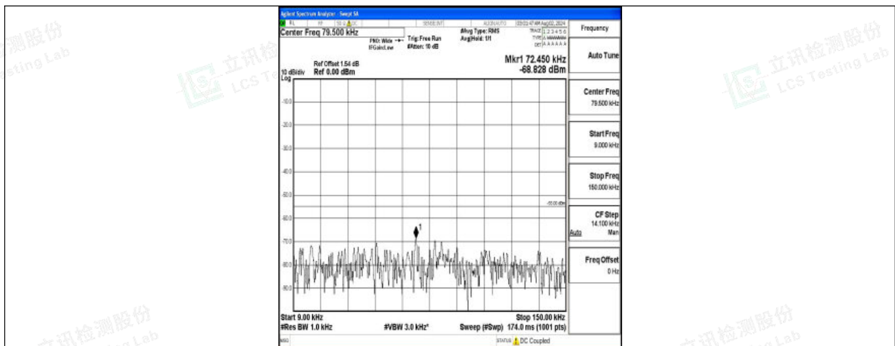
Band 7-15MHz-16QAM-21375-1RB#0-0.009~0.15-PASS
