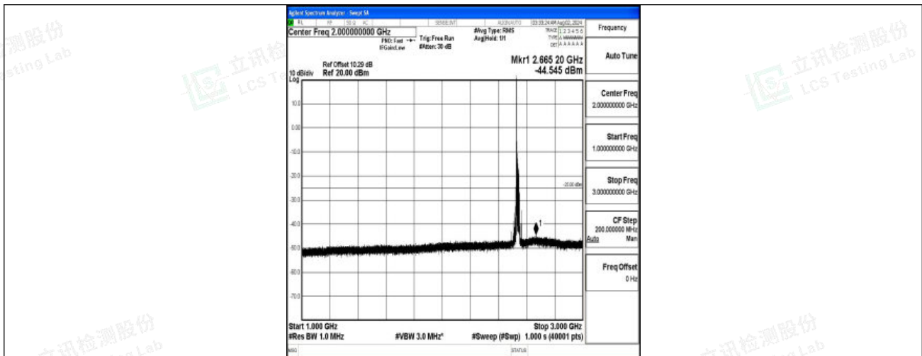
Band7-20MHz-16QAM-21100-1RB#0-1000~3000-PASS
