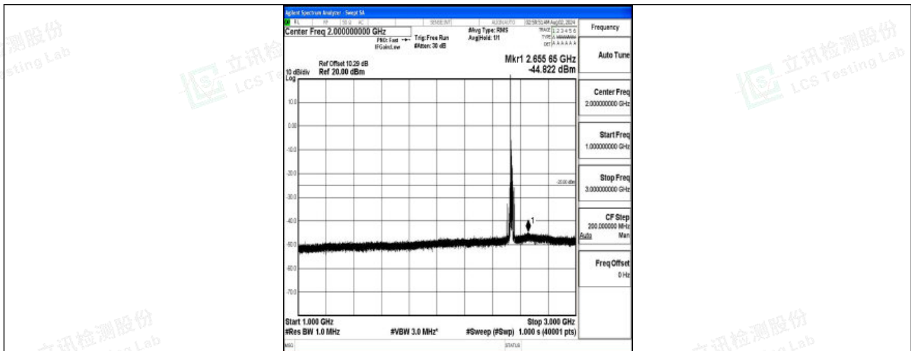
Band7-15MHz-16QAM-21100-1RB#0-1000~3000-PASS
