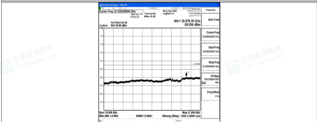
Band7-5MHz-16QAM-21425-1RB#0-18000~27000-PASS
