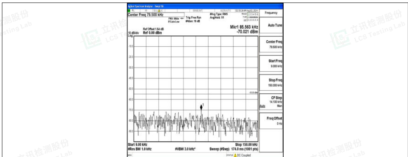
Band7-10MHz-16QAM-21400-1RB#0-0.009~0.15-PASS
