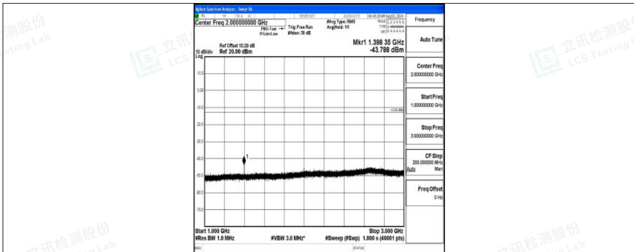
Band12-3MHz-16QAM-23025-1RB#0-1000~3000-PASS
