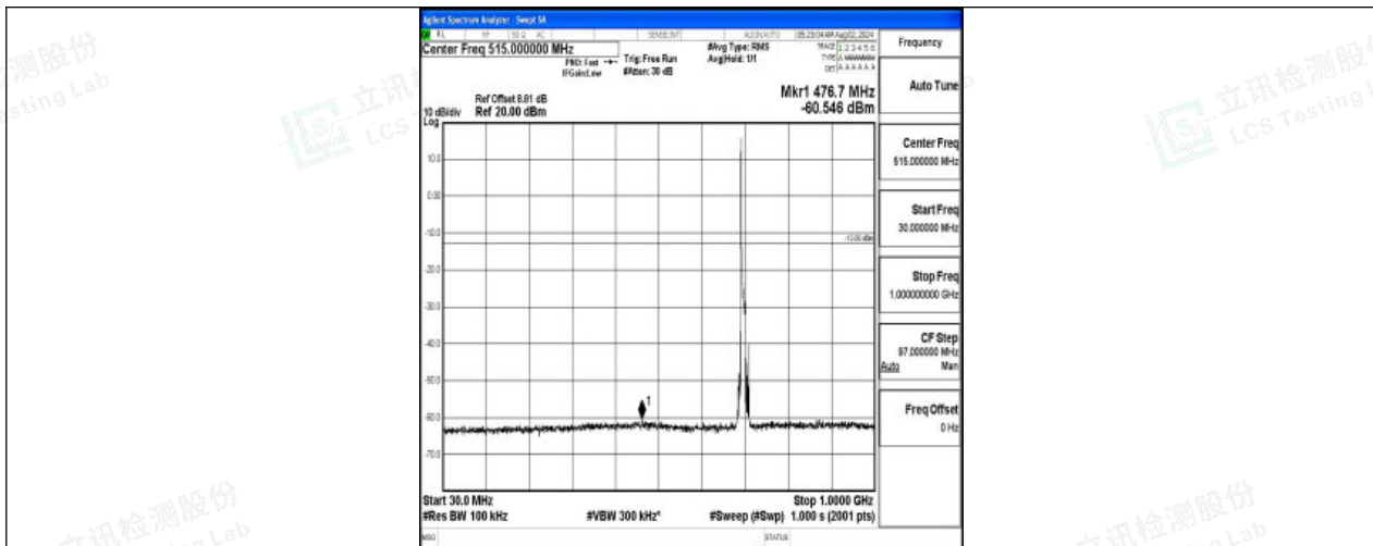
Band12-10MHz-QPSK-23060-1RB#0-30~1000-PASS
