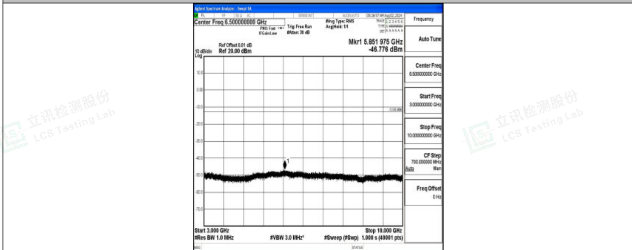
Band12-10MHz-16QAM-23095-1RB#0-3000~10000-PASS
