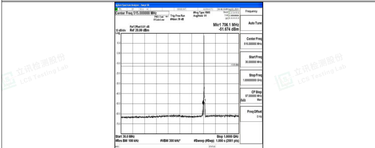
Band12-3MHz-QPSK-23165-1RB#0-30~1000-PASS
