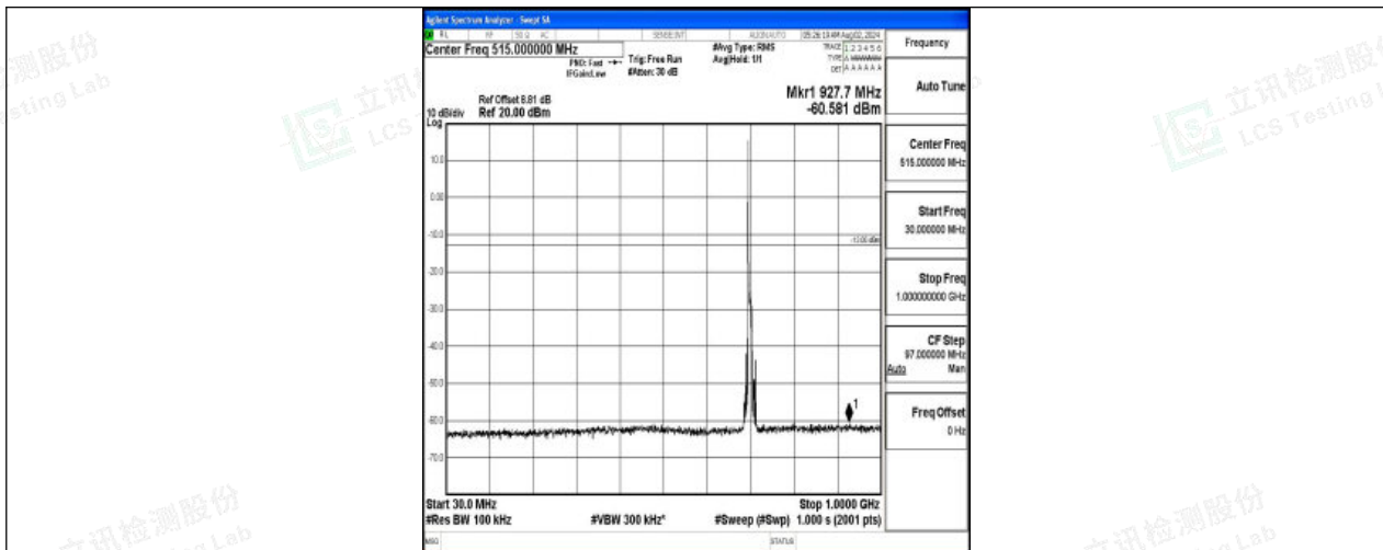
Band12-10MHz-16QAM-23095-1RB#0-30~1000-PASS
