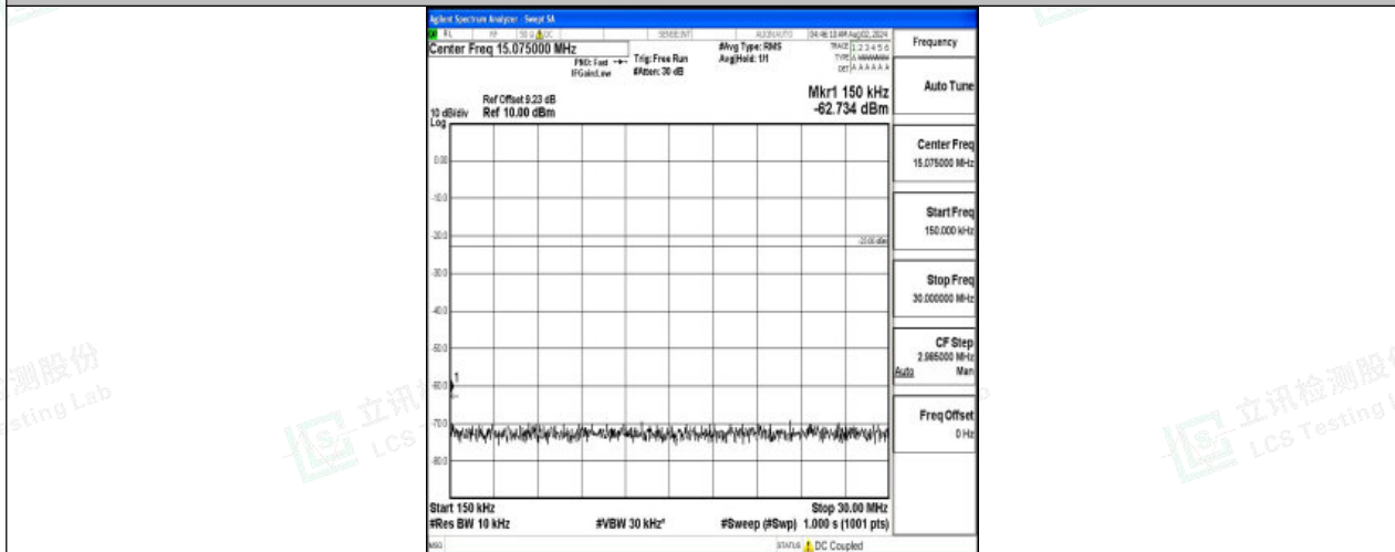
Band12-3MHz-QPSK-23165-1RB#0-0.15~30-PASS
