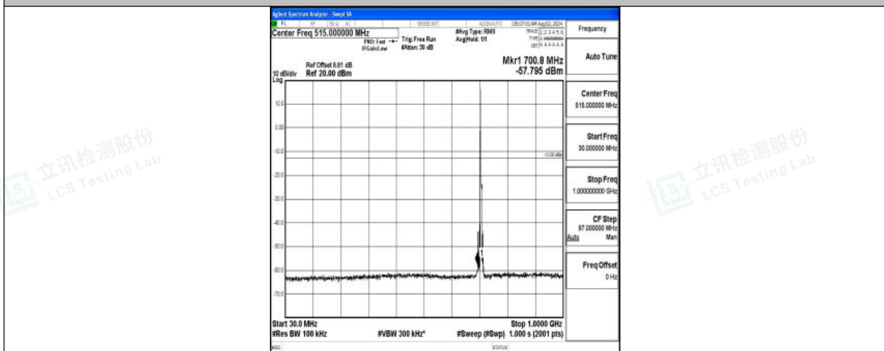
Band12-5MHz-QPSK-23155-1RB#0-30~1000-PASS
