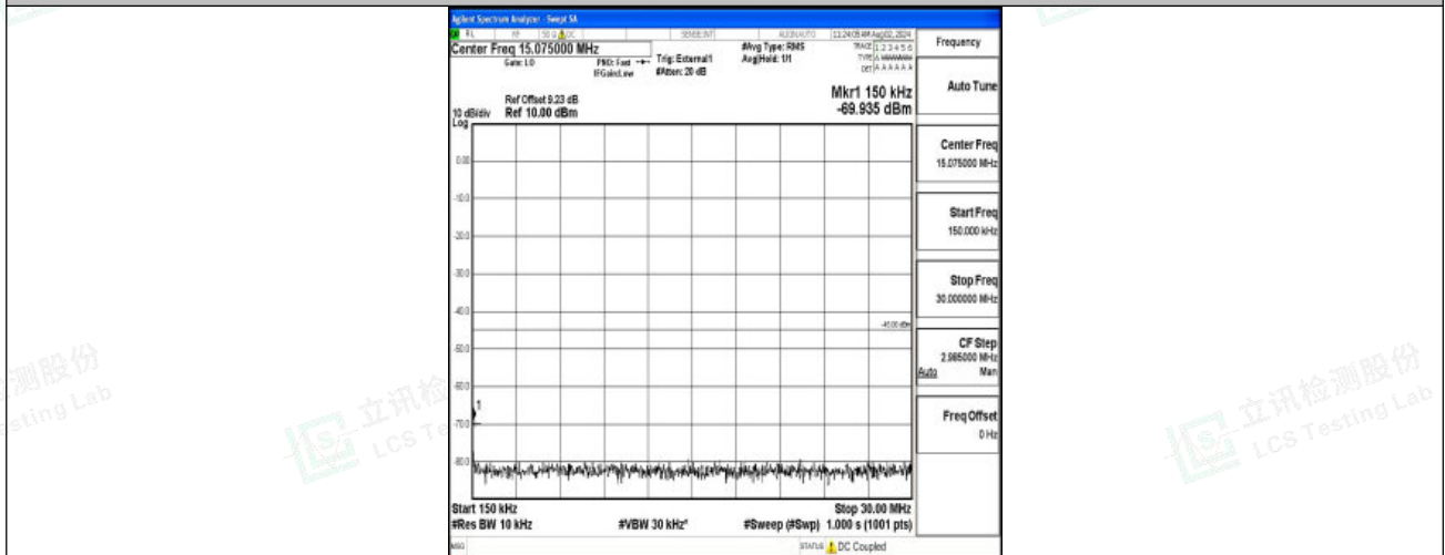
Band38-15MHz-16QAM-38175-1RB#0-0.15~30-PASS
