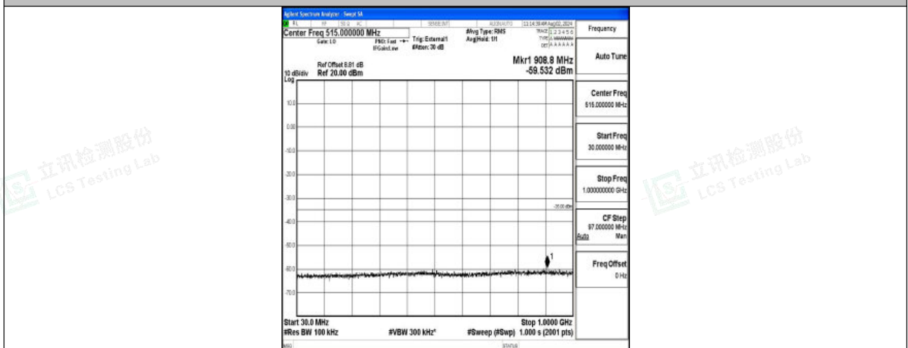
Band38-15MHz-16QAM-37825-1RB#0-30~1000-PASS
