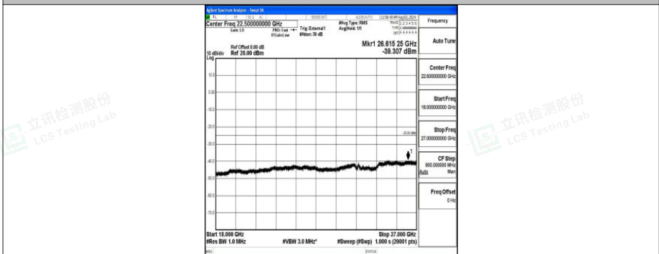
Band38-20MHz-16QAM-38150-1RB#0-18000~27000-PASS
