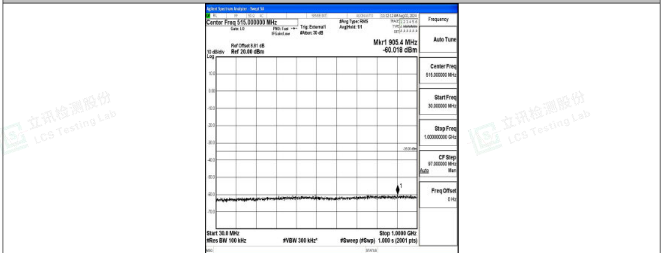
Band38-15MHz-QPSK-37825-1RB#0-30~1000-PASS
