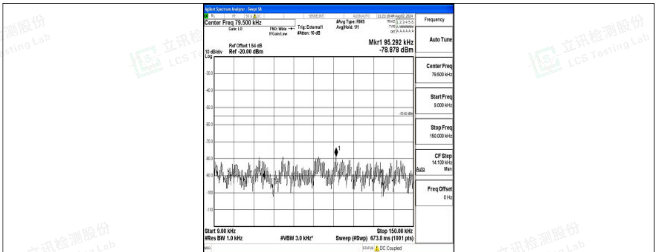
Band38-15MHz-QPSK-38175-1RB#0-0.009~0.15-PASS
