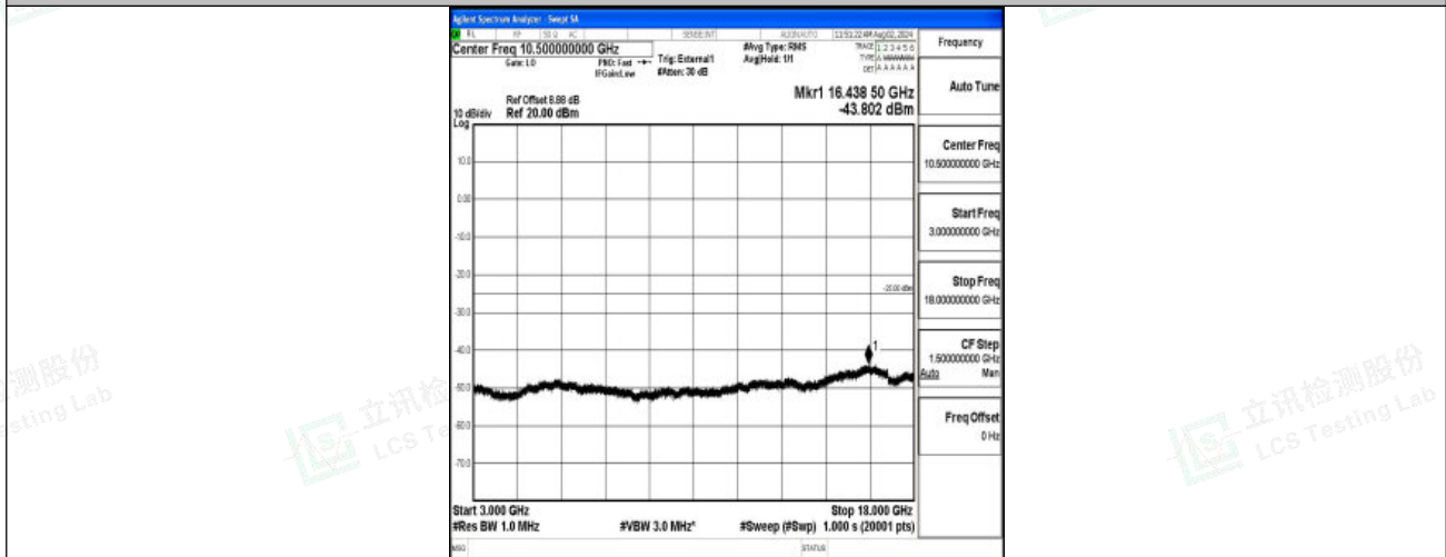
Band38-20MHz-16QAM-38000-1RB#0-3000~18000-PASS
