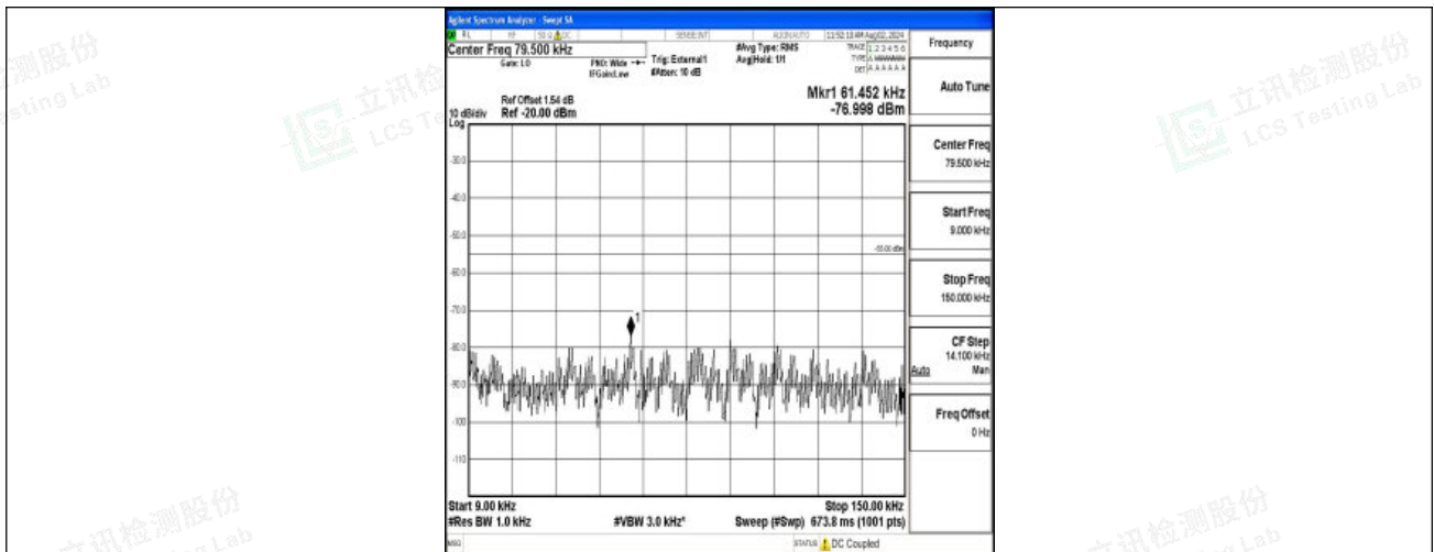
Band38-20MHz-QPSK-38150-1RB#0-0.009~0.15-PASS
