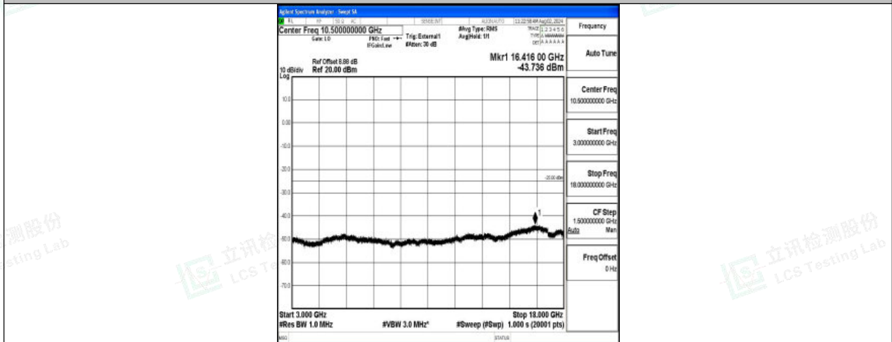
Band38-15MHz-QPSK-38175-1RB#0-3000~18000-PASS
