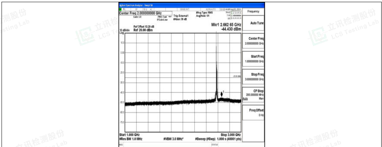
Band38-15MHz-QPSK-37825-1RB#0-1000~3000-PASS
