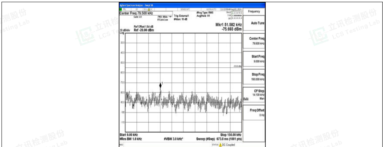
Band38-15MHz-16QAM-37825-1RB#0-0.009~0.15-PASS
