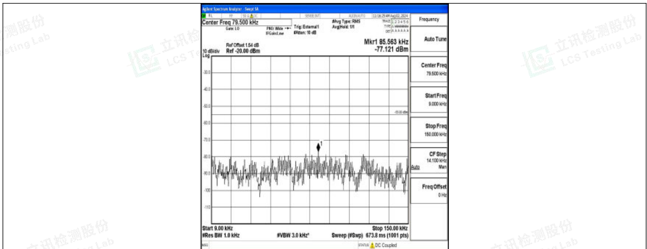
Band38-15MHz-QPSK-38000-1RB#0-0.009~0.15-PASS
