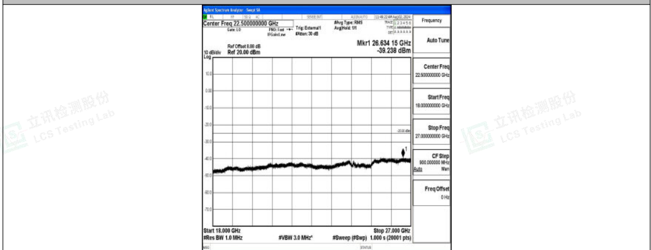
Band38-20MHz-QPSK-38000-1RB#0-18000~27000-PASS
