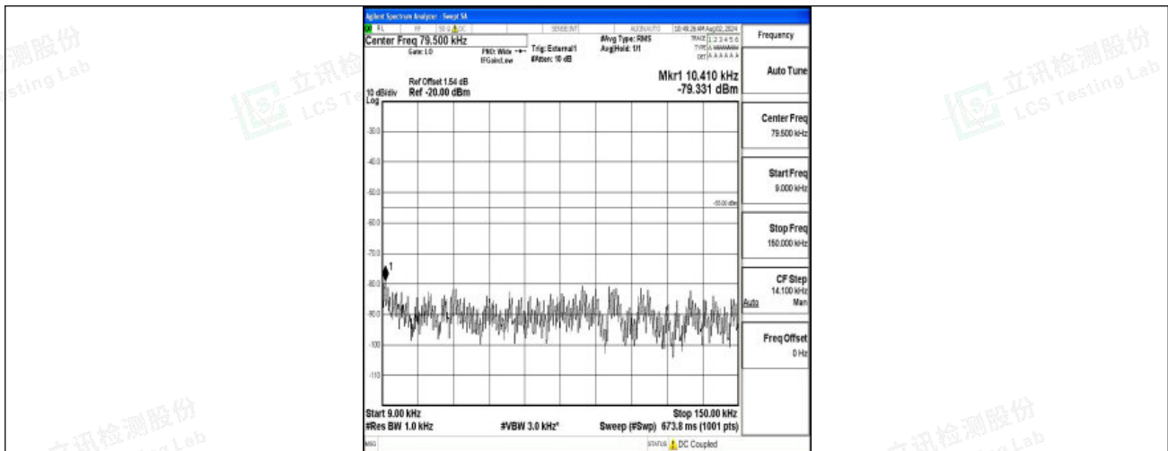
Band38-10MHz-QPSK-38200-1RB#0-0.009~0.15-PASS
