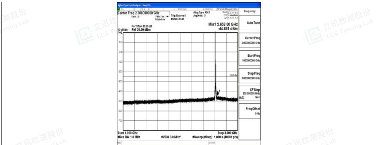
Band38-10MHz-QPSK-38200-1RB#0-1000~3000-PASS
