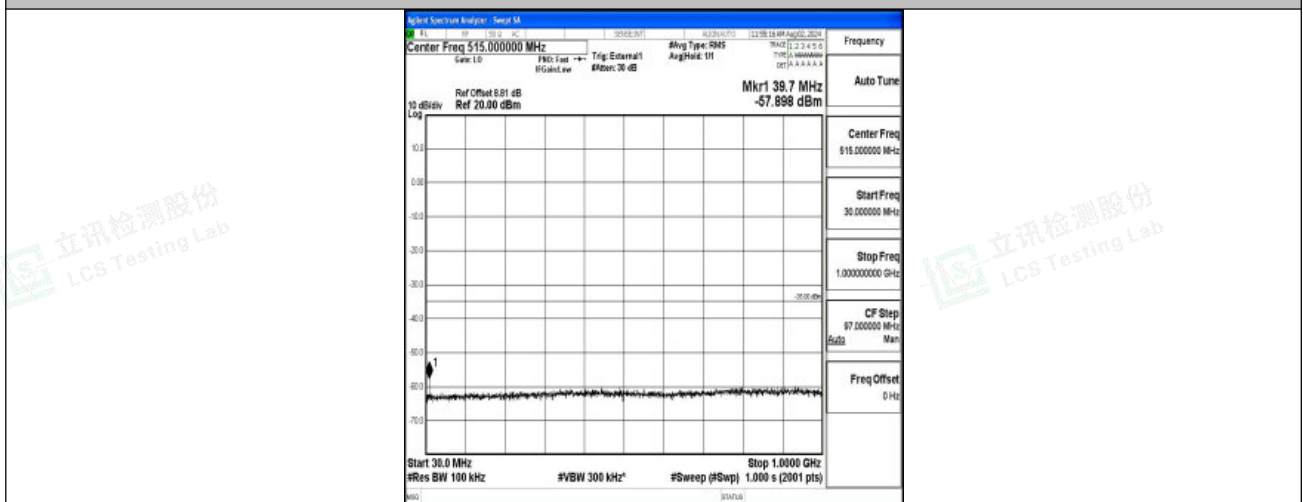
Band38-20MHz-16QAM-38150-1RB#0-30~1000-PASS
