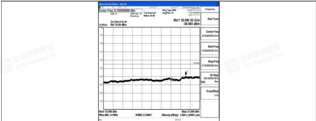
Band38-10MHz-16QAM-38200-1RB#0-18000~27000-PASS
