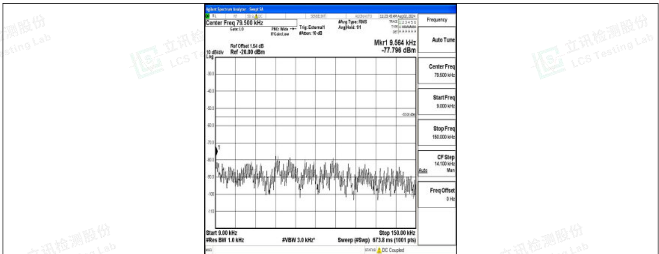
Band38-15MHz-16QAM-38175-1RB#0-0.009~0.15-PASS
