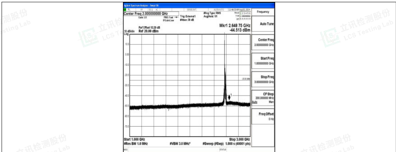
Band38-20MHz-16QAM-37850-1RB#0-1000~3000-PASS
