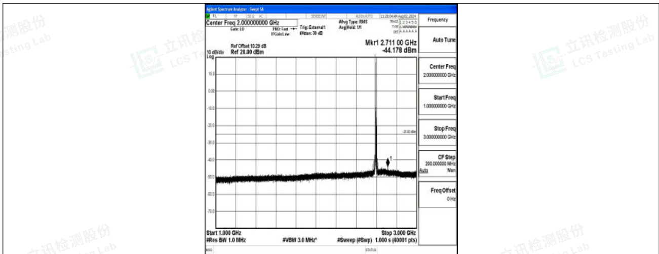
Band38-15MHz-16QAM-38000-1RB#0-1000~3000-PASS
