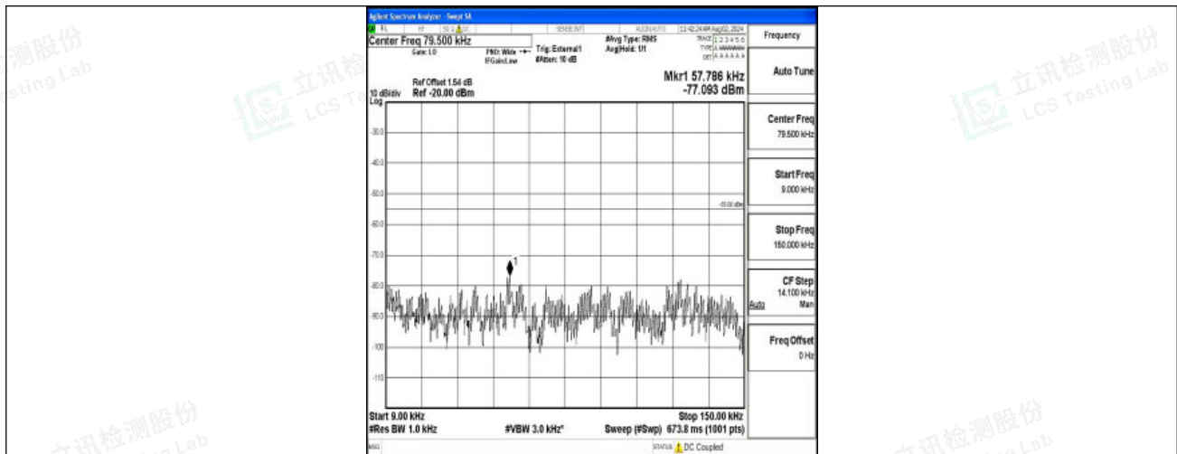
Band38-20MHz-QPSK-37850-1RB#0-0.009~0.15-PASS
