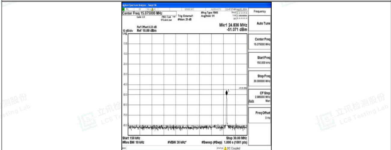
Band38-20MHz-QPSK-38000-1RB#0-0.15~30-PASS
