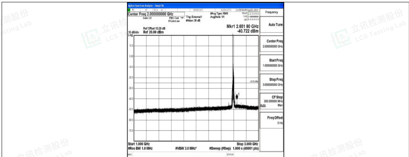
Band38-20MHz-16QAM-38000-1RB#0-1000~3000-PASS
