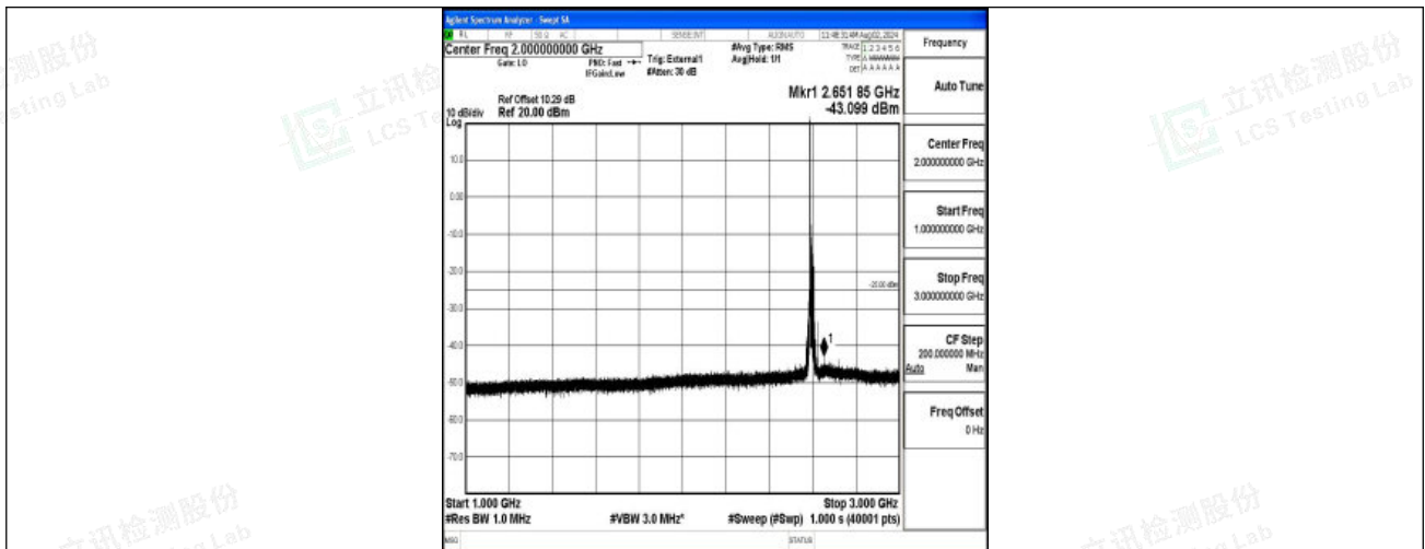
Band38-20MHz-QPSK-38000-1RB#0-1000~3000-PASS
