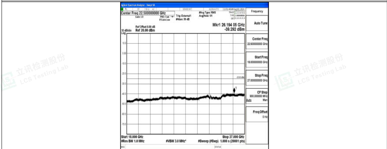
Band38-20MHz-16QAM-38000-1RB#0-18000~27000-PASS
