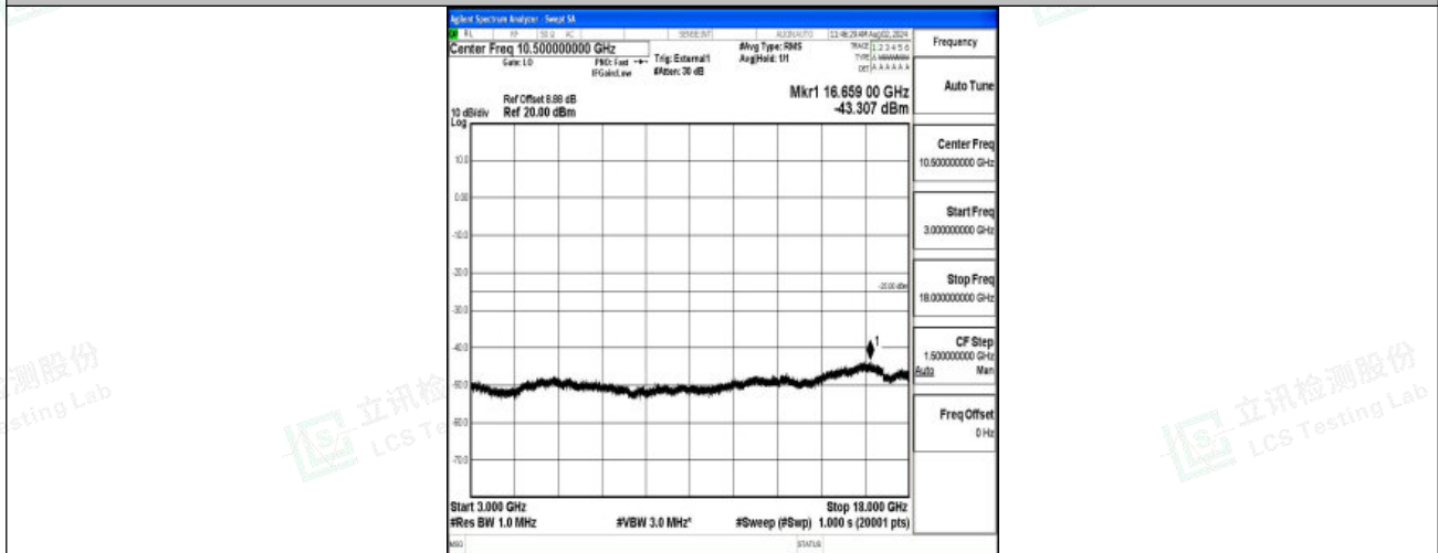
Band38-20MHz-16QAM-37850-1RB#0-3000~18000-PASS
