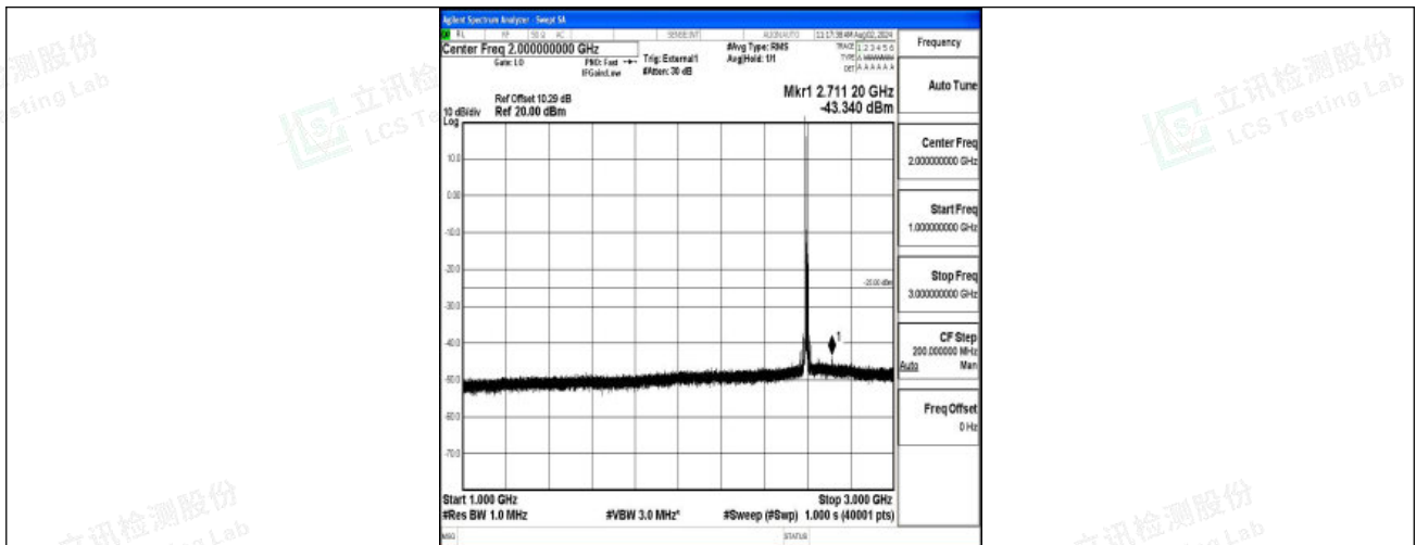
Band38-15MHz-QPSK-38000-1RB#0-1000~3000-PASS
