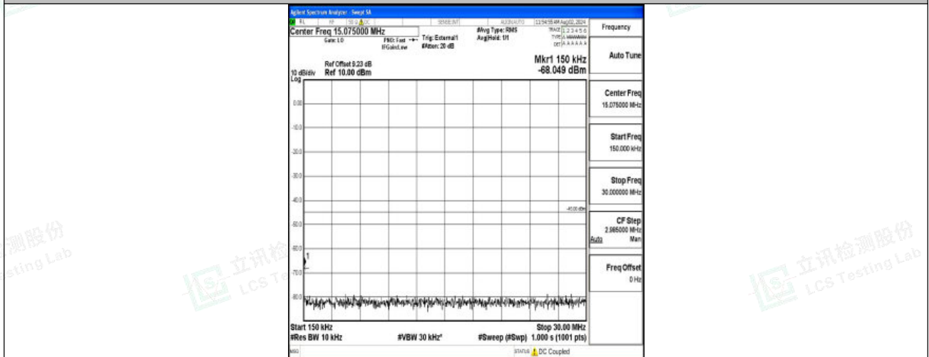
Band38-20MHz-16QAM-38150-1RB#0-0.15~30-PASS
