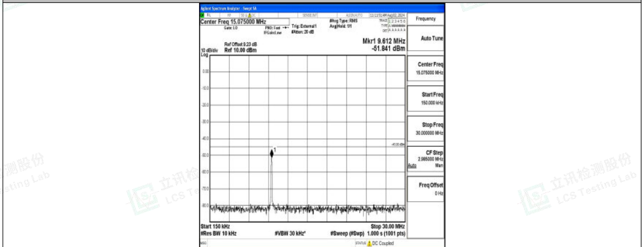
Band38-15MHz-QPSK-37825-1RB#0-0.15~30-PASS
