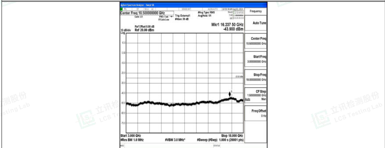
Band38-10MHz-16QAM-38200-1RB#0-3000~18000-PASS
