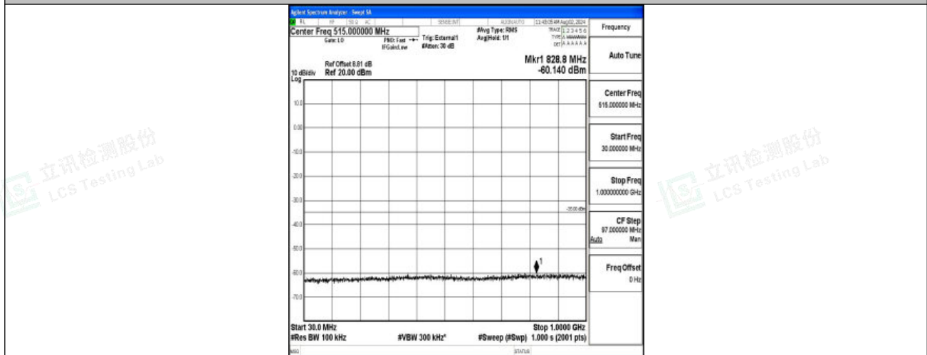
Band38-20MHz-QPSK-37850-1RB#0-30~1000-PASS
