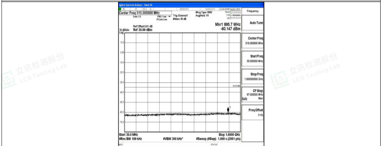
Band38-15MHz-16QAM-38175-1RB#0-30~1000-PASS
