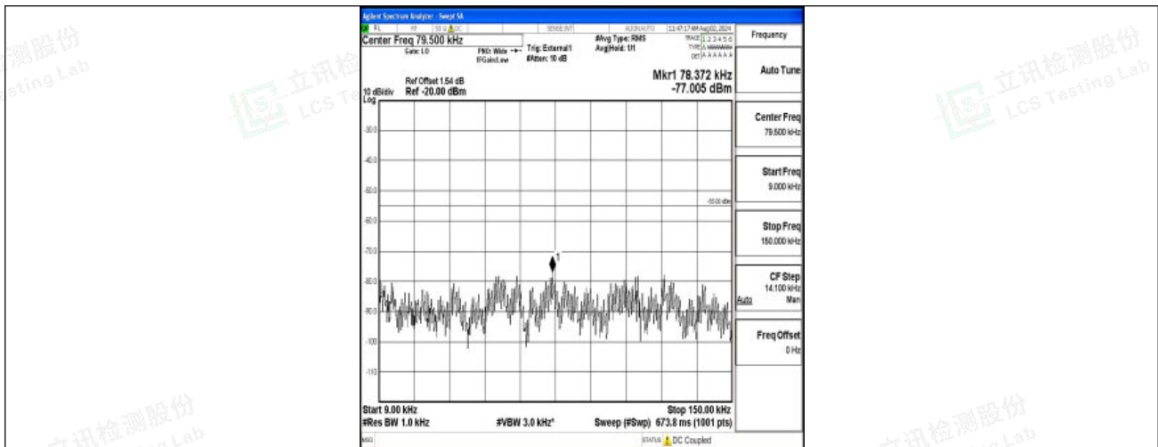
Band38-20MHz-QPSK-38000-1RB#0-0.009~0.15-PASS
