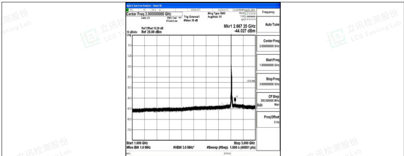
Band38-15MHz-16QAM-38175-1RB#0-1000~3000-PASS
