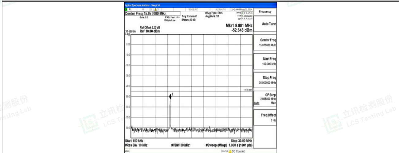
Band38-20MHz-QPSK-37850-1RB#0-0.15~30-PASS
