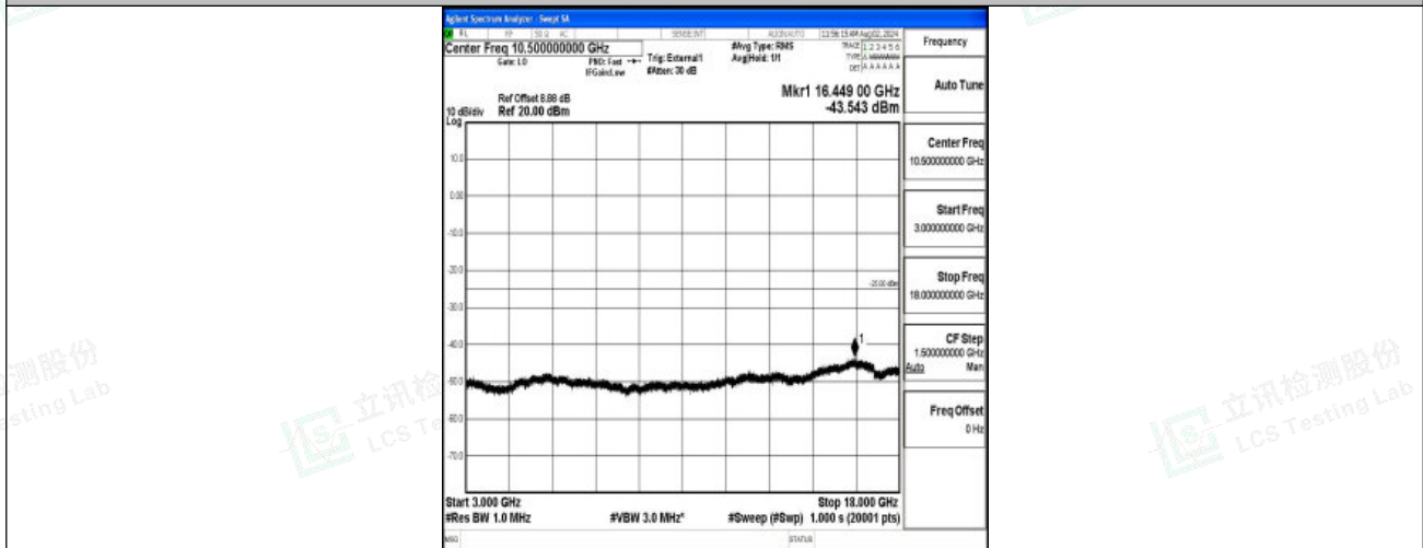
Band38-20MHz-16QAM-38150-1RB#0-3000~18000-PASS
