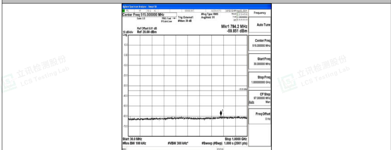
Band38-10MHz-16QAM-38200-1RB#0-30~1000-PASS
