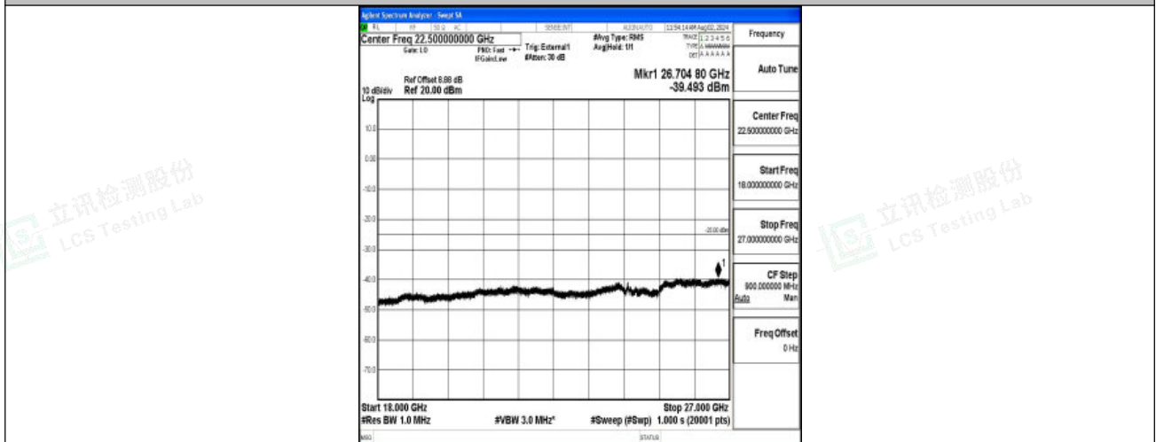
Band38-20MHz-QPSK-38150-1RB#0-18000~27000-PASS
