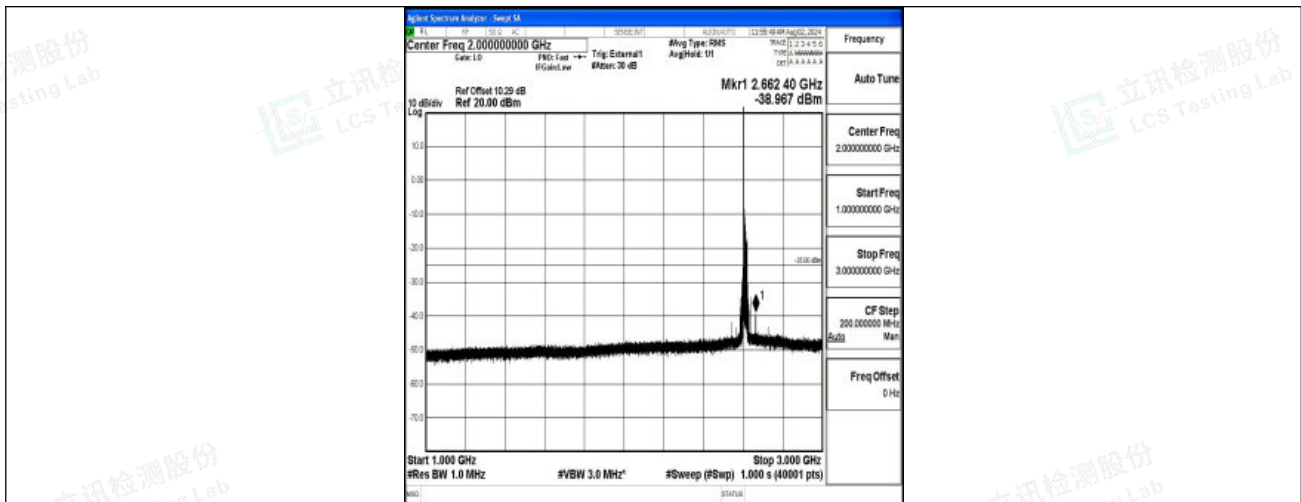
Band38-20MHz-16QAM-38150-1RB#0-1000~3000-PASS
