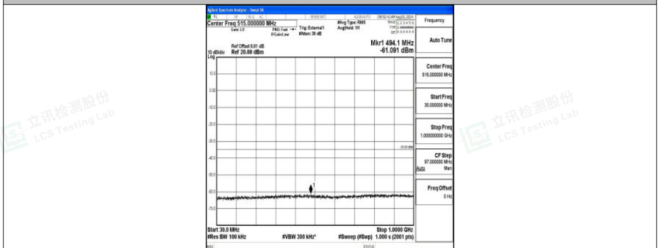
Band41-20MHz-16QAM-40620-1RB#0-30~1000-PASS
