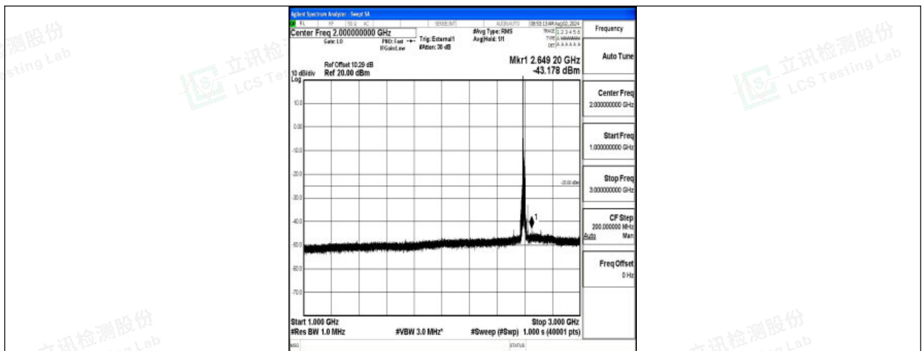
Band41-20MHz-16QAM-40620-1RB#0-1000~3000-PASS
