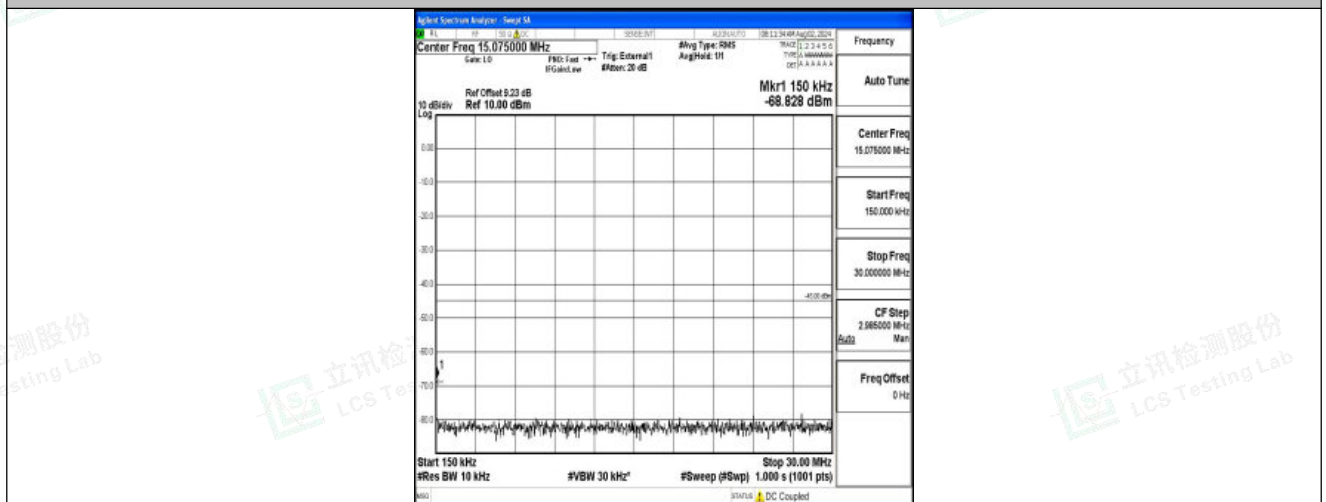
Band41-15MHz-16QAM-41515-1RB#0-0.15~30-PASS
