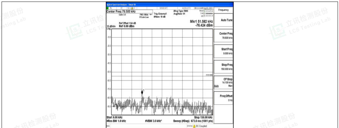
Band41-15MHz-16QAM-41515-1RB#0-0.009~0.15-PASS
