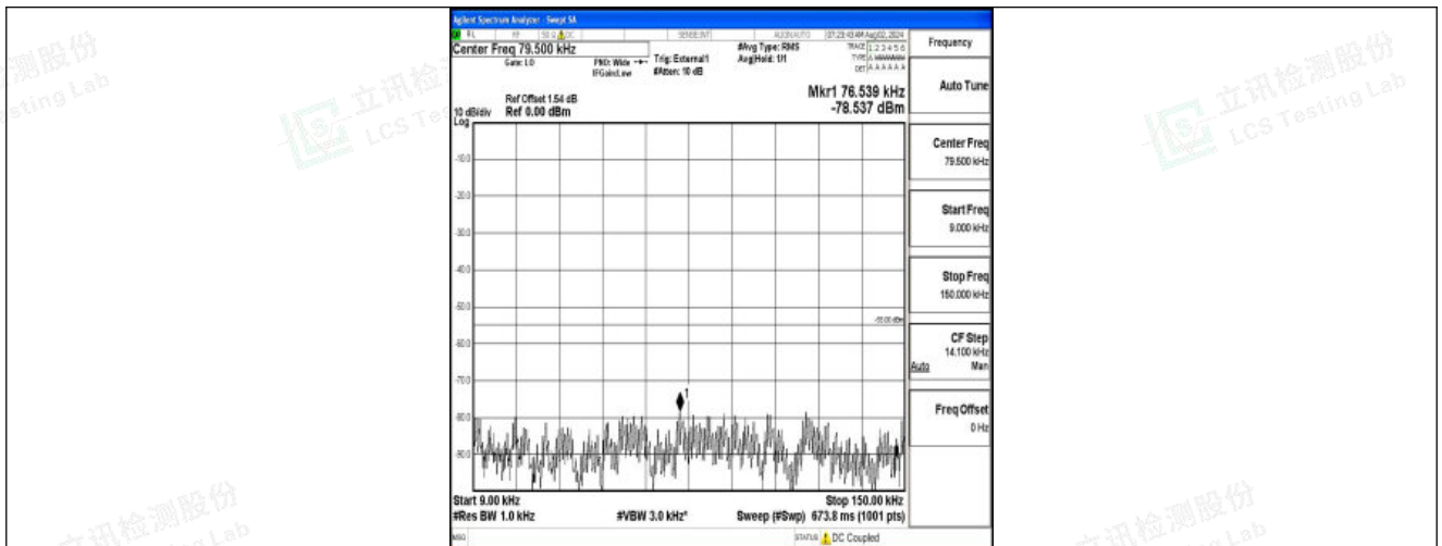
Band41-10MHz-QPSK-40620-1RB#0-0.009~0.15-PASS
