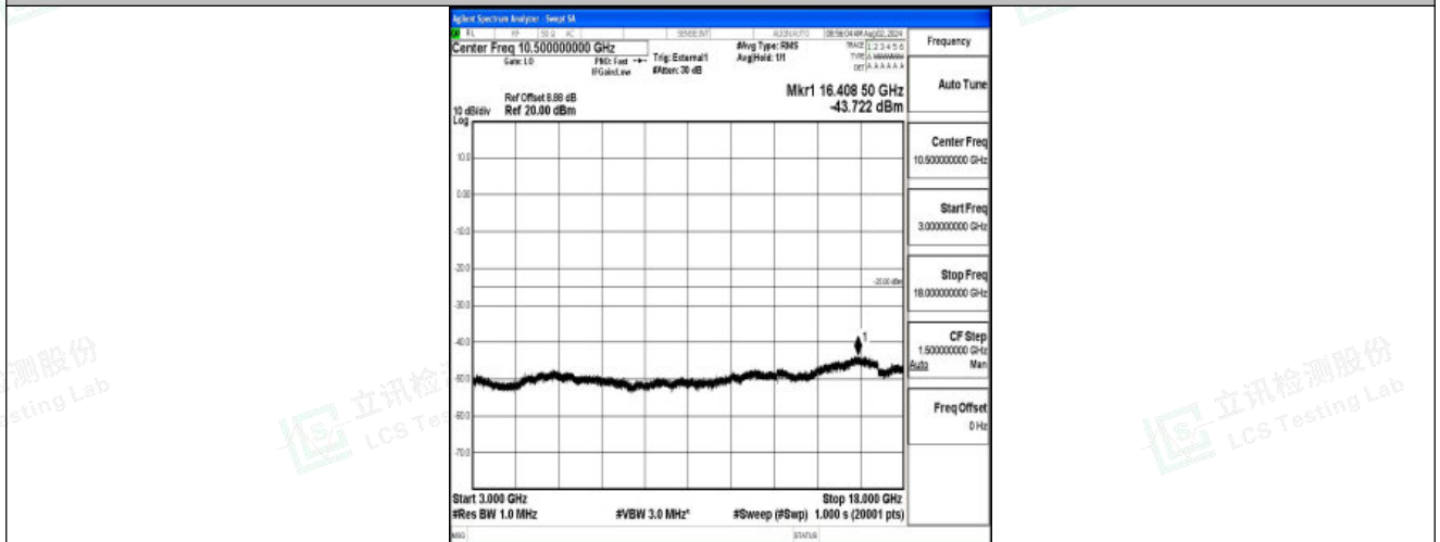
Band41-20MHz-QPSK-41490-1RB#0-3000~18000-PASS
