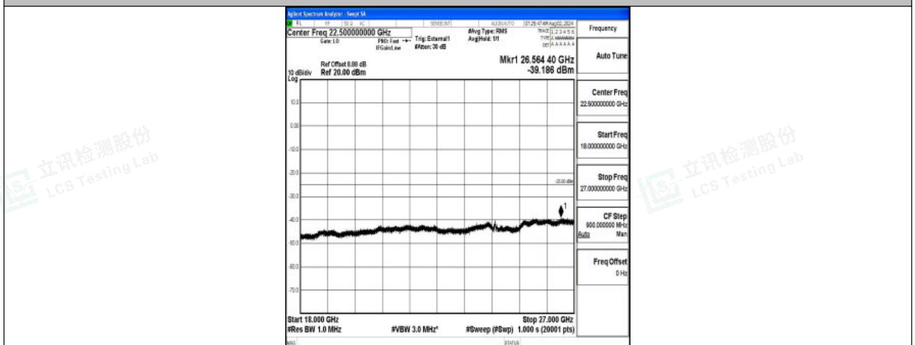
Band41-10MHz-QPSK-40620-1RB#0-18000~27000-PASS
