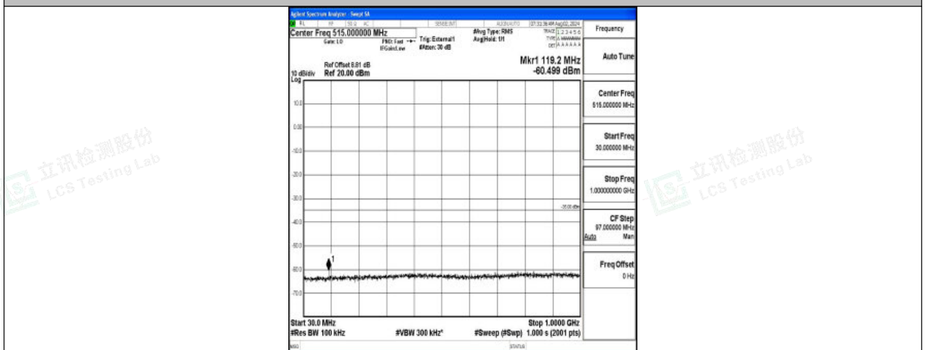
Band41-10MHz-16QAM-41540-1RB#0-30~1000-PASS
