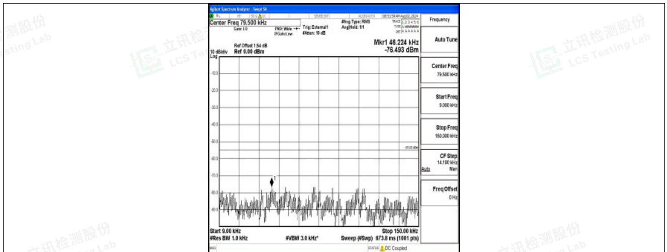
Band41-20MHz-16QAM-40620-1RB#0-0.009~0.15-PASS
