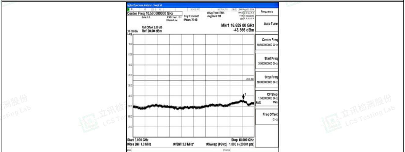
Band41-20MHz-QPSK-40620-1RB#0-3000~18000-PASS
