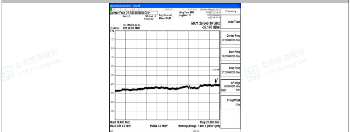
Band41-20MHz-16QAM-40620-1RB#0-18000~27000-PASS
