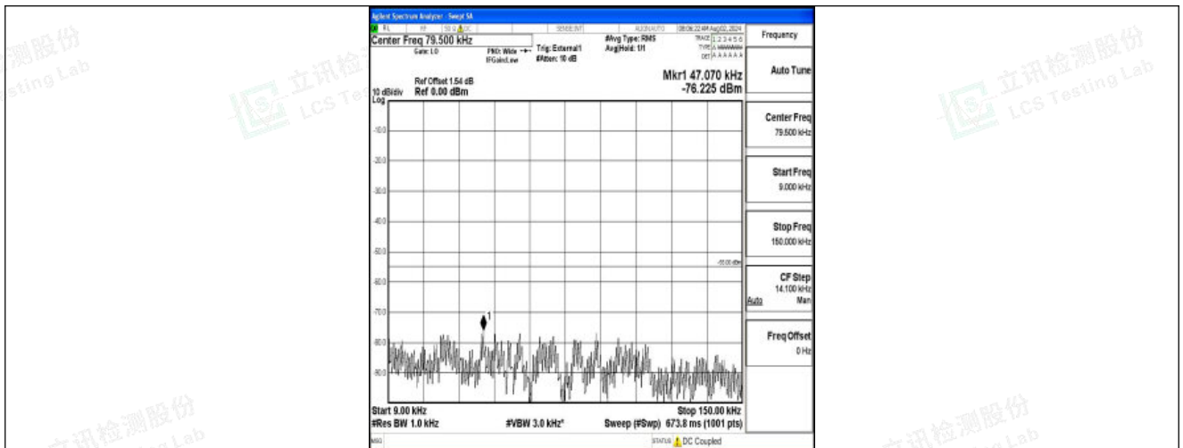
Band41-15MHz-16QAM-40620-1RB#0-0.009~0.15-PASS
