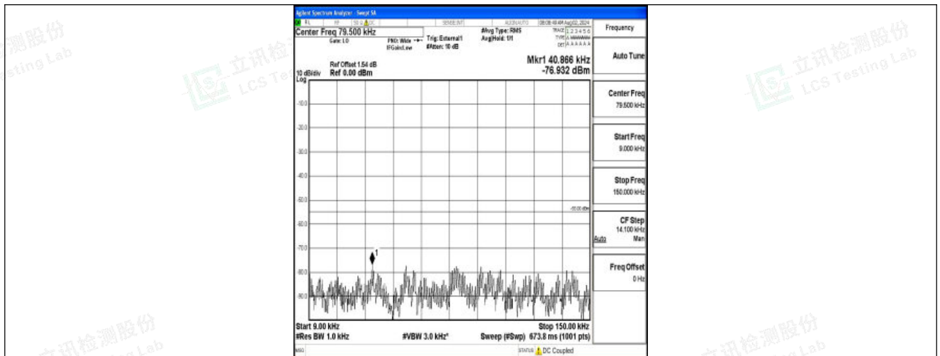
Band41-15MHz-QPSK-41515-1RB#0-0.009~0.15-PASS
