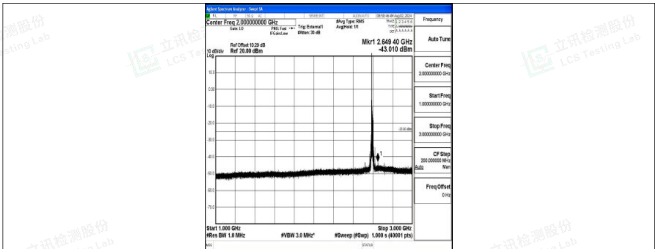
Band41-20MHz-QPSK-40620-1RB#0-1000~3000-PASS
