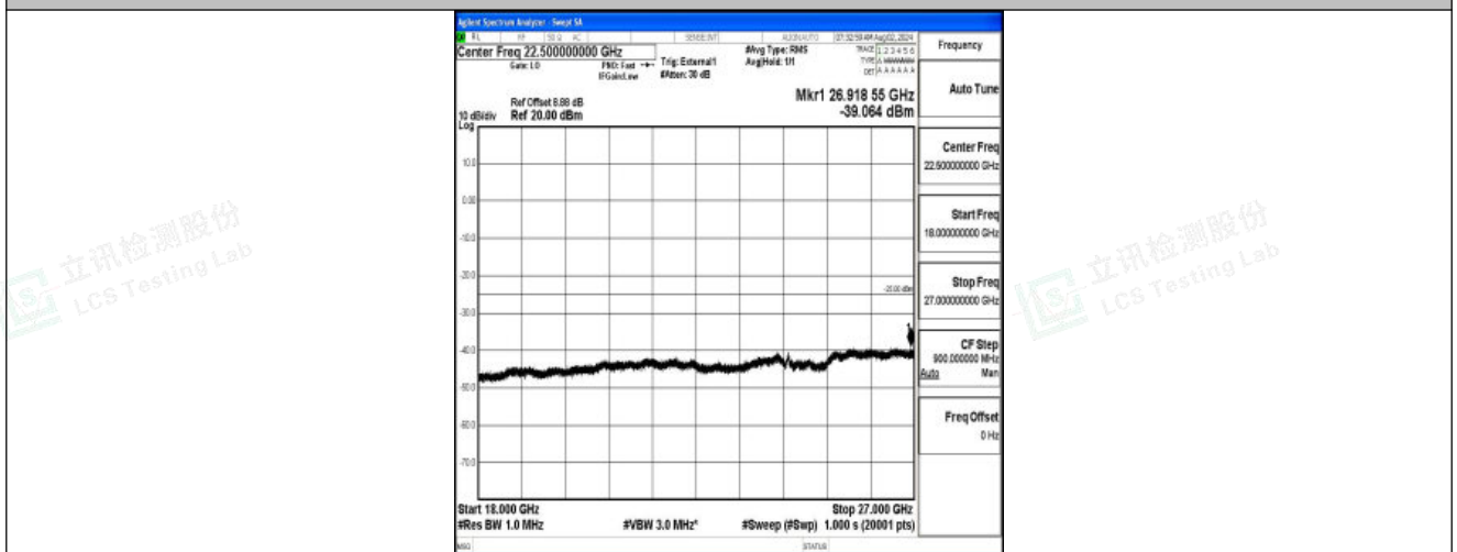
Band41-10MHz-16QAM-41540-1RB#0-18000~27000-PASS
