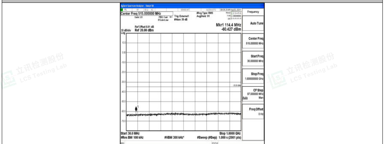
Band41-15MHz-QPSK-41515-1RB#0-30~1000-PASS
