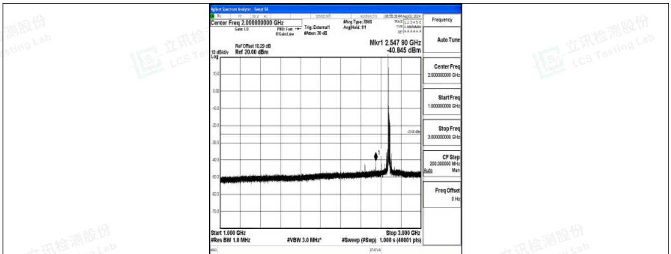
Band41-20MHz-QPSK-41490-1RB#0-1000~3000-PASS
