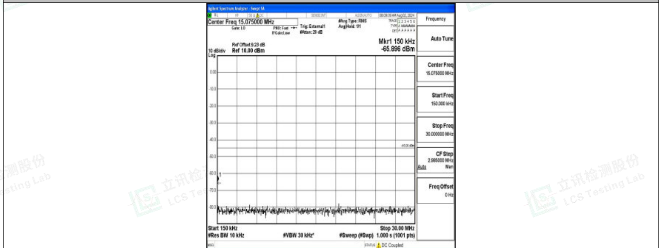
Band41-15MHz-QPSK-41515-1RB#0-0.15~30-PASS
