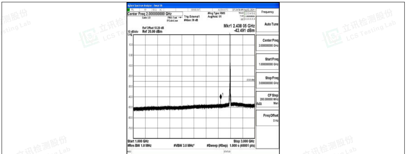
Band41-10MHz-QPSK-40620-1RB#0-1000~3000-PASS
