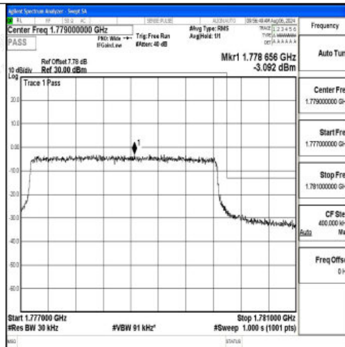
Band66_3MHz_QPSK_132657_15RB#0
