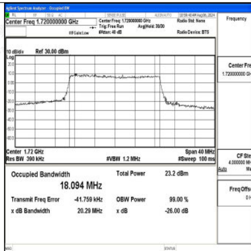
Band66-20MHz-QPSK-132072-100RB#0-PASS
