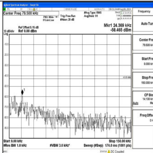
Band66_1.4MHz_QPSK_132665_1RB#0_0.009~0.15_0.009~0.15
