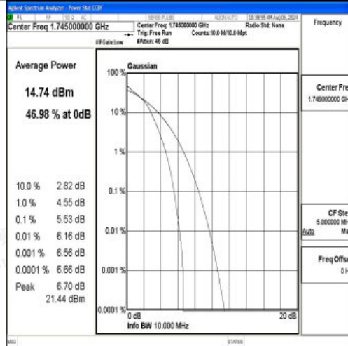
Band66-10MHz-16QAM-132322-50RB#0-PASS
