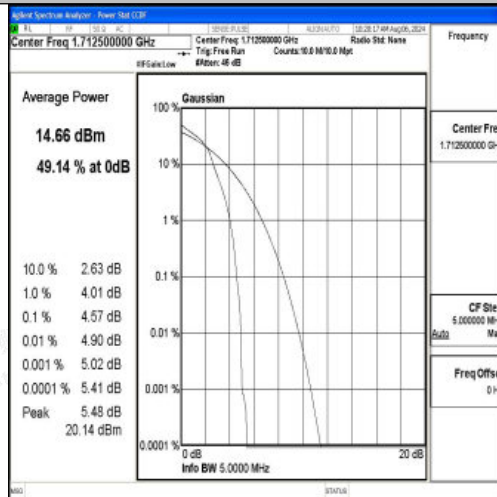
Band66-5MHz-16QAM-131997-1RB#0-PASS
