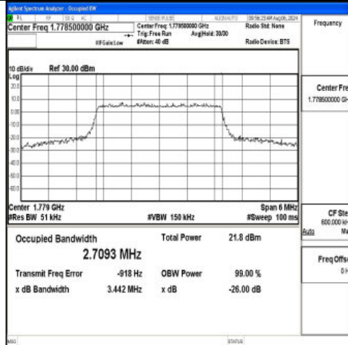
Band66-3MHz-16QAM-132657-15RB#0-PASS
