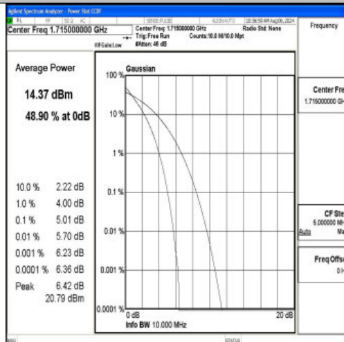
Band66-10MHz-QPSK-132022-50RB#0-PASS
