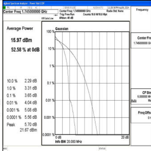
Band66-20MHz-QPSK-132322-1RB#0-PASS
