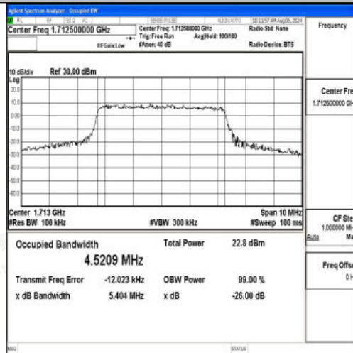
Band66-5MHz-16QAM-131997-25RB#0-PASS
