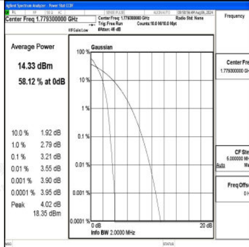
Band66-1.4MHz-QPSK-132665-6RB#0-PASS
