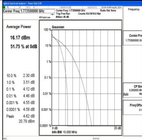
Band66-15MHz-QPSK-132597-1RB#0-PASS
