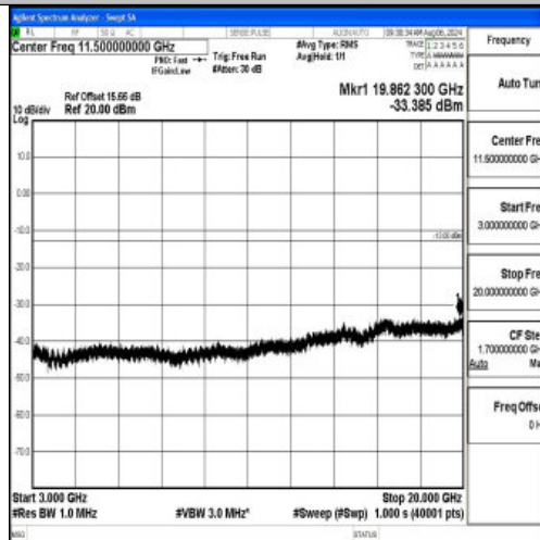
Band66_1.4MHz_QPSK_132322_1RB#0_3000~20000_3000~20000
