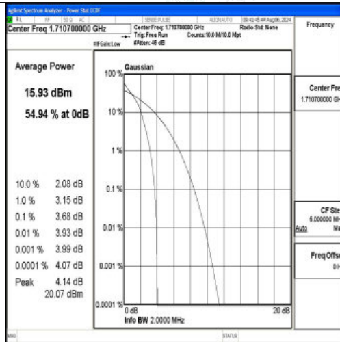
Band66-1.4MHz-QPSK-131979-1RB#0-PASS
