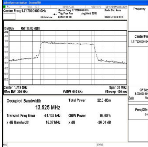
Band66-15MHz-16QAM-132047-75RB#0-PASS
