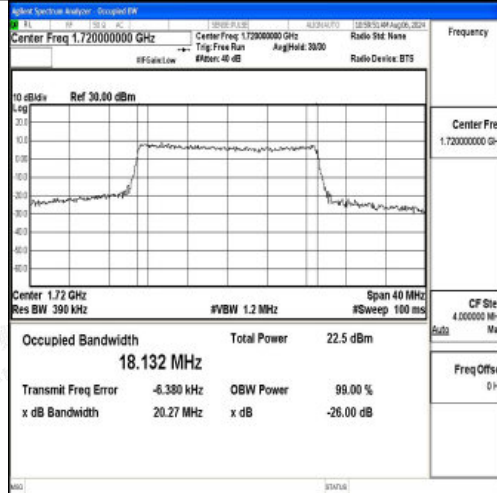
Band66-20MHz-16QAM-132072-100RB#0-PASS
