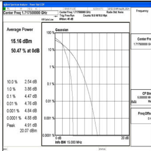
Band66-15MHz-16QAM-132047-1RB#0-PASS
