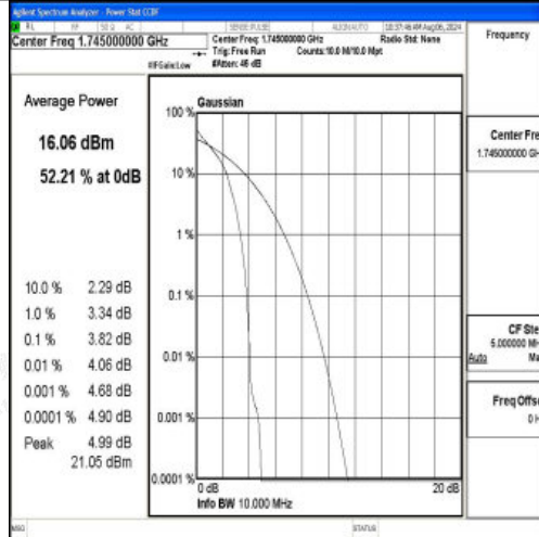
Band66-10MHz-QPSK-132322-1RB#0-PASS
