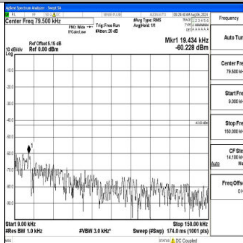
Band66_1.4MHz_16QAM_131979_1RB#0_0.009~0.15_0.009~0.15
