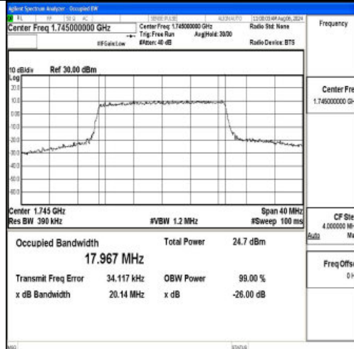
Band66-20MHz-QPSK-132322-100RB#0-PASS
