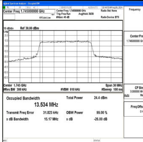
Band66-15MHz-QPSK-132322-75RB#0-PASS
