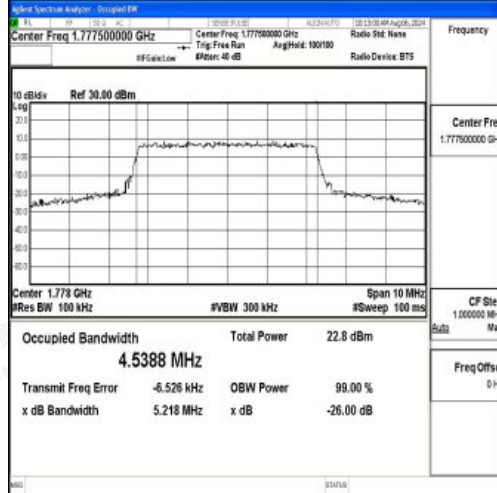
Band66-5MHz-QPSK-132647-25RB#0-PASS
