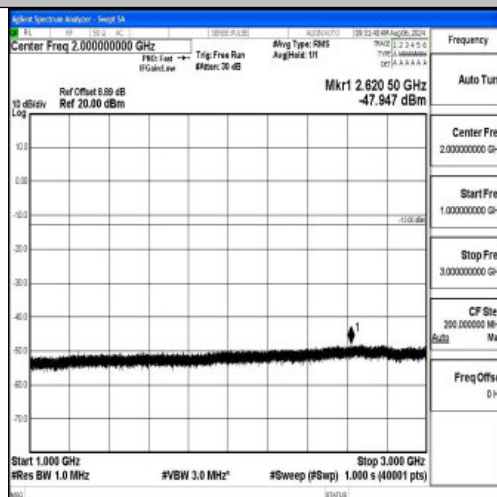
Band66_1.4MHz_QPSK_132665_1RB#0_1000~3000_1000~3000
