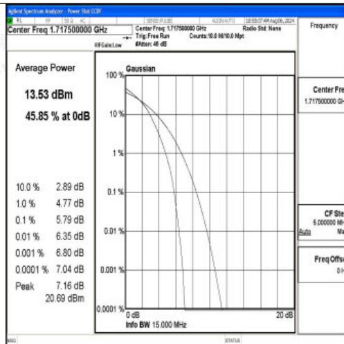
Band66-15MHz-16QAM-132047-75RB#0-PASS
