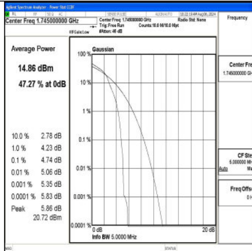
Band66-5MHz-16QAM-132322-1RB#0-PASS
