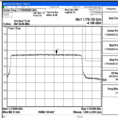
Band66_5MHz_16QAM_132647_25RB#0
