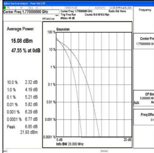
Band66-20MHz-QPSK-132572-100RB#0-PASS
