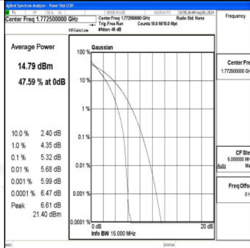
Band66-15MHz-QPSK-132597-75RB#0-PASS
