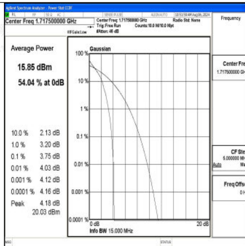
Band66-15MHz-QPSK-132047-1RB#0-PASS
