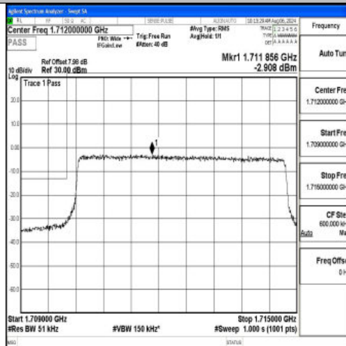
Band66_5MHz_QPSK_131997_25RB#0
