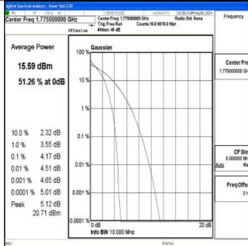
Band66-10MHz-QPSK-132622-1RB#0-PASS
