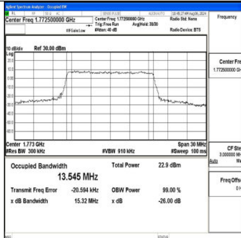
Band66-15MHz-16QAM-132597-75RB#0-PASS
