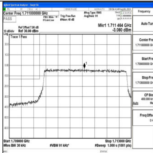
Band66_3MHz_16QAM_131987_15RB#0
