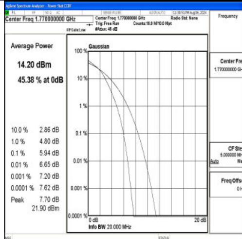
Band66-20MHz-16QAM-132572-100RB#0-PASS
