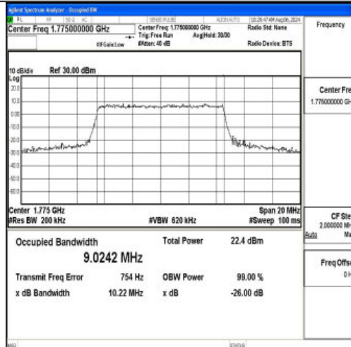
Band66-10MHz-16QAM-132622-50RB#0-PASS
