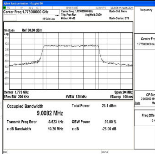
Band66-10MHz-QPSK-132622-50RB#0-PASS
