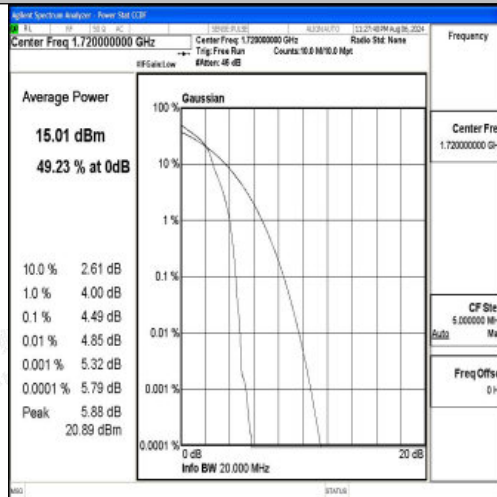
Band66-20MHz-16QAM-132072-1RB#0-PASS
