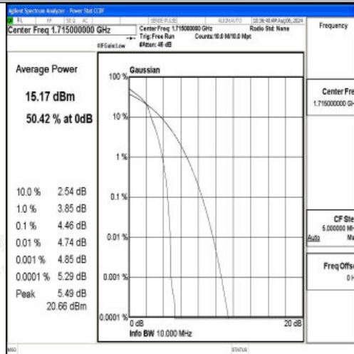
Band66-10MHz-16QAM-132022-1RB#0-PASS
