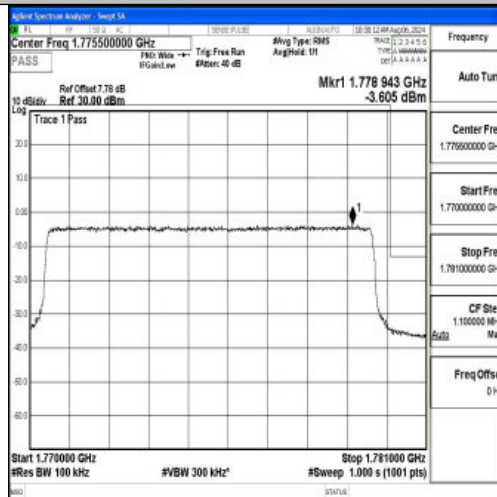
Band66_10MHz_QPSK_132622_50RB#0
