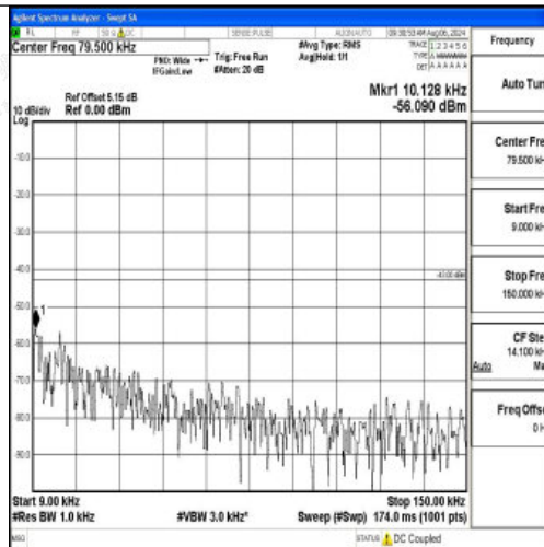
Band66_1.4MHz_16QAM_132322_1RB#0_0.009~0.15_0.009~0.15
