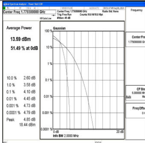
Band66-1.4MHz-16QAM-132665-6RB#0-PASS
