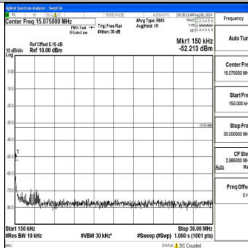
Band66_1.4MHz_QPSK_132322_1RB#0_0.15~30_0.15~30
