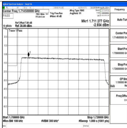
Band66_10MHz_QPSK_132022_50RB#0
