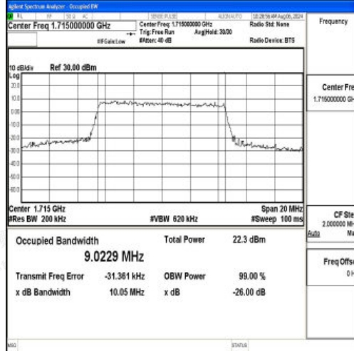
Band66-10MHz-16QAM-132022-50RB#0-PASS
