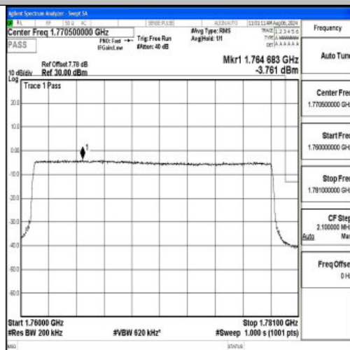
Band66 20MHz 16QAM 132572 100RB#0
