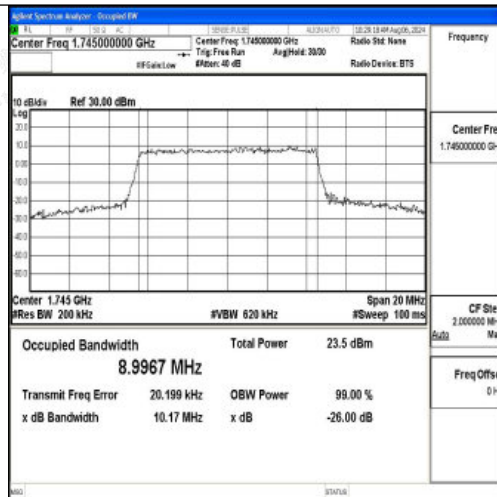
Band66-10MHz-16QAM-132322-50RB#0-PASS
