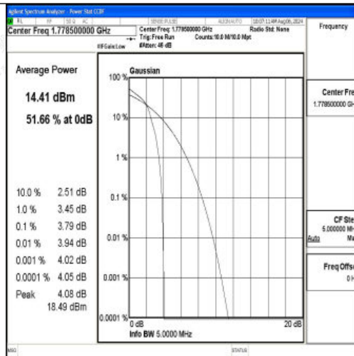
Band66-3MHz-16QAM-132657-1RB#0-PASS
