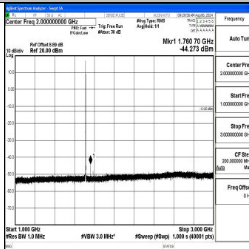
Band66_1.4MHz_16QAM_131979_1RB#0_1000~3000_1000~3000
