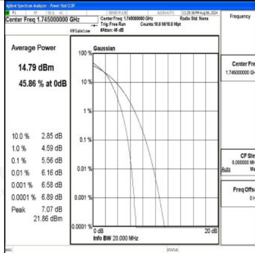
Band66-20MHz-16QAM-132322-100RB#0-PASS
