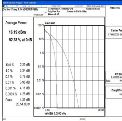
Band66-5MHz-QPSK-132322-1RB#0-PASS
