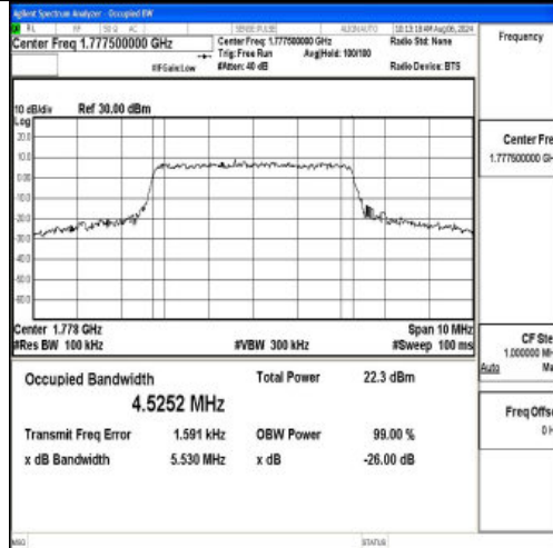
Band66-5MHz-16QAM-132647-25RB#0-PASS
