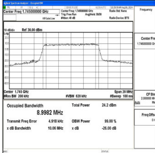
Band66-10MHz-QPSK-132322-50RB#0-PASS
