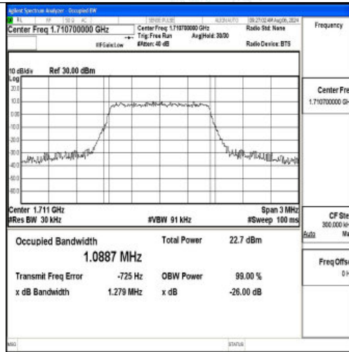
Band66-1.4MHz-QPSK-131979-6RB#0-PASS
