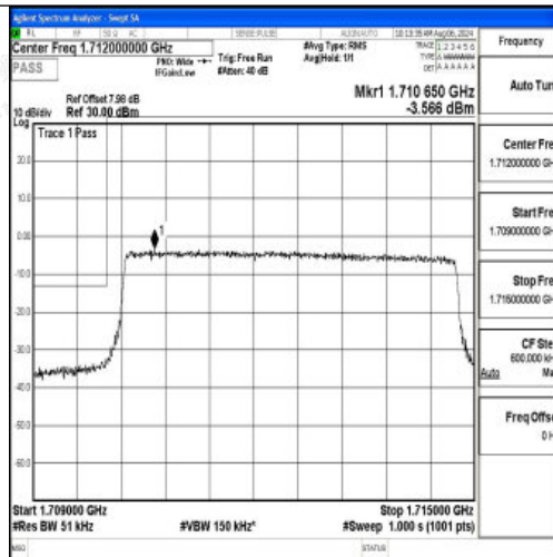
Band66_5MHz_16QAM_131997_25RB#0
