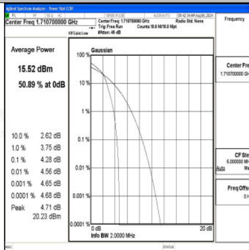
Band66-1.4MHz-16QAM-131979-1RB#0-PASS
