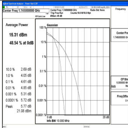
Band66-10MHz-16QAM-132322-1RB#0-PASS
