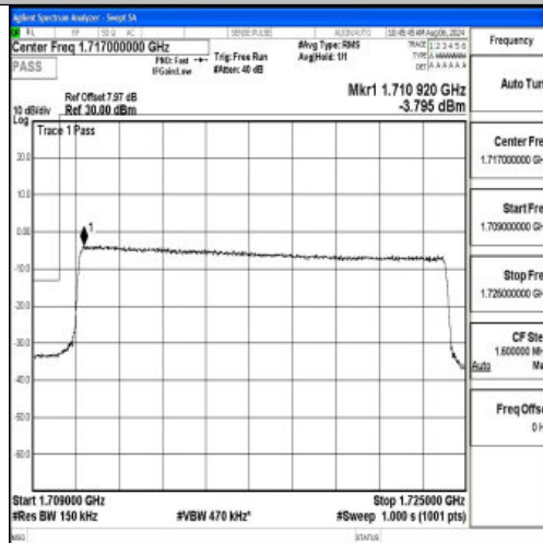
Band66_15MHz_16QAM_132047_75RB#0
