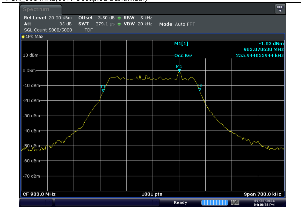
FSK 903 MHz(99% Occupied Bandwidth)
