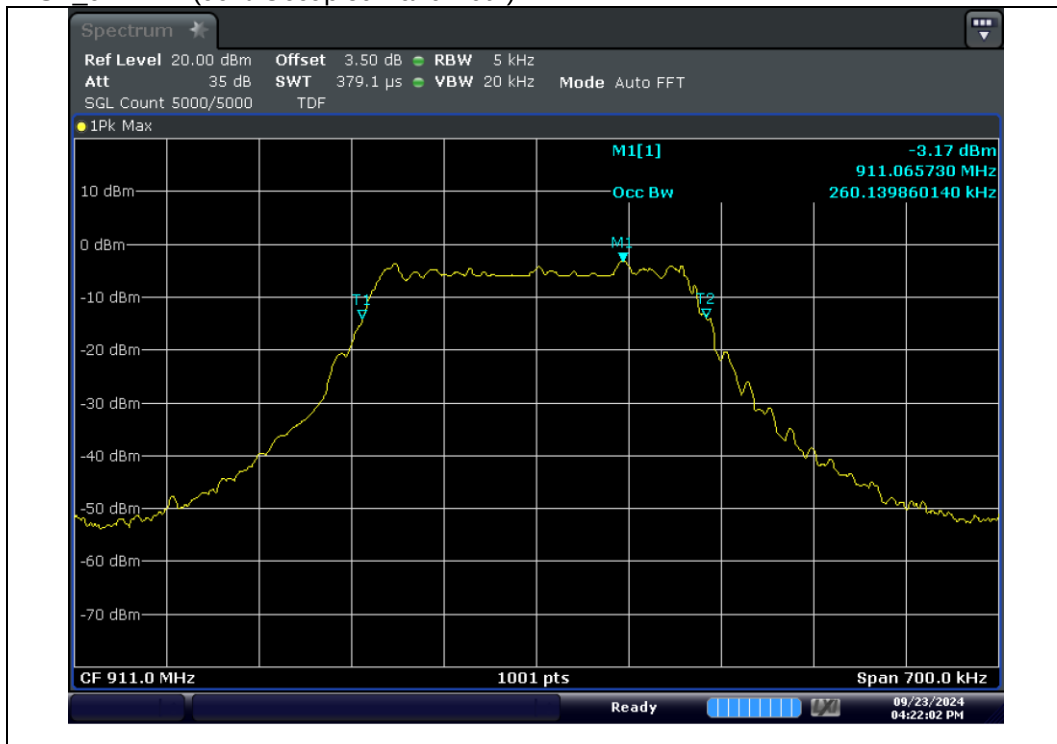
FSK 911 MHz(99% Occupied Bandwidth)
