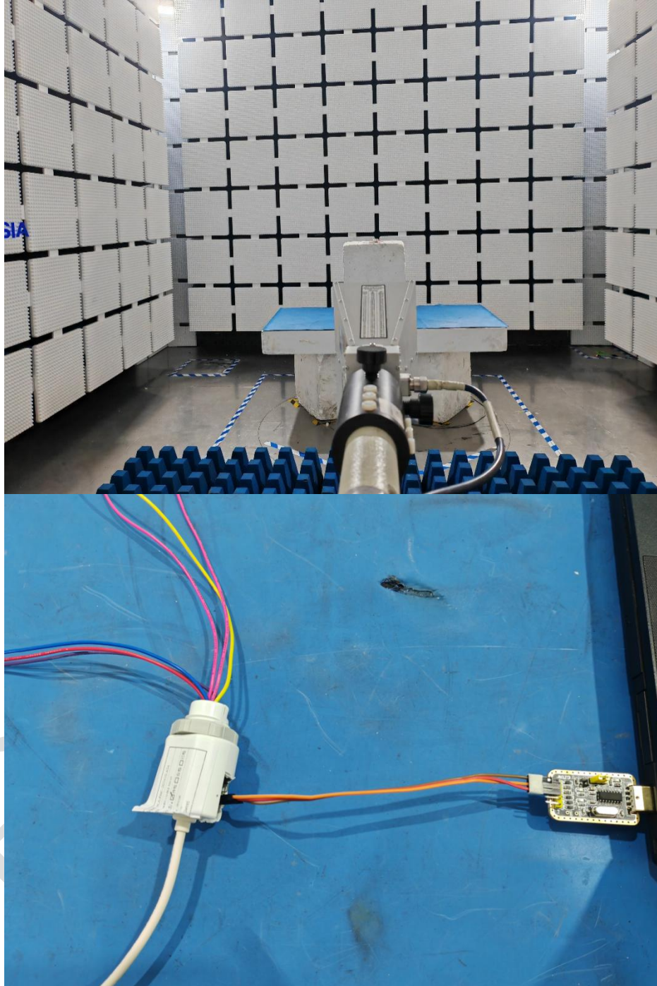
Radiated Emissions (above 1GHz)
