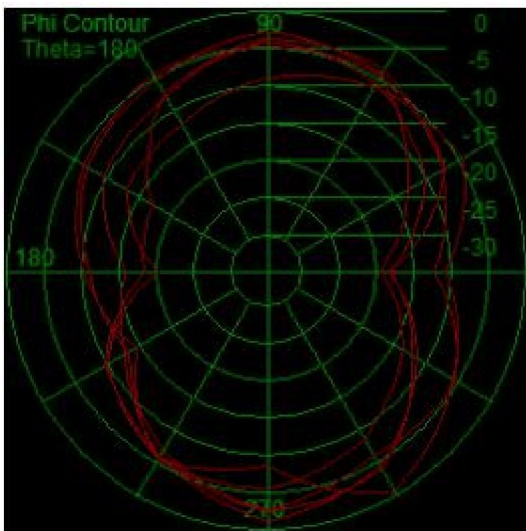
Passive -Freq2460.00MHz
