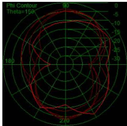
Passive -Freq2480.00MHz
