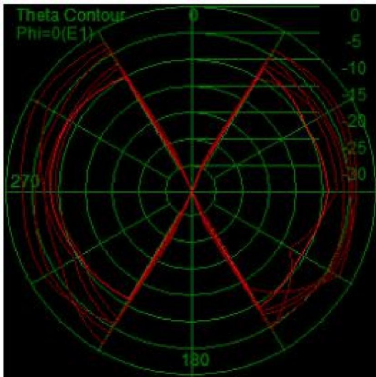
Passive -Freq2400.00MHz
