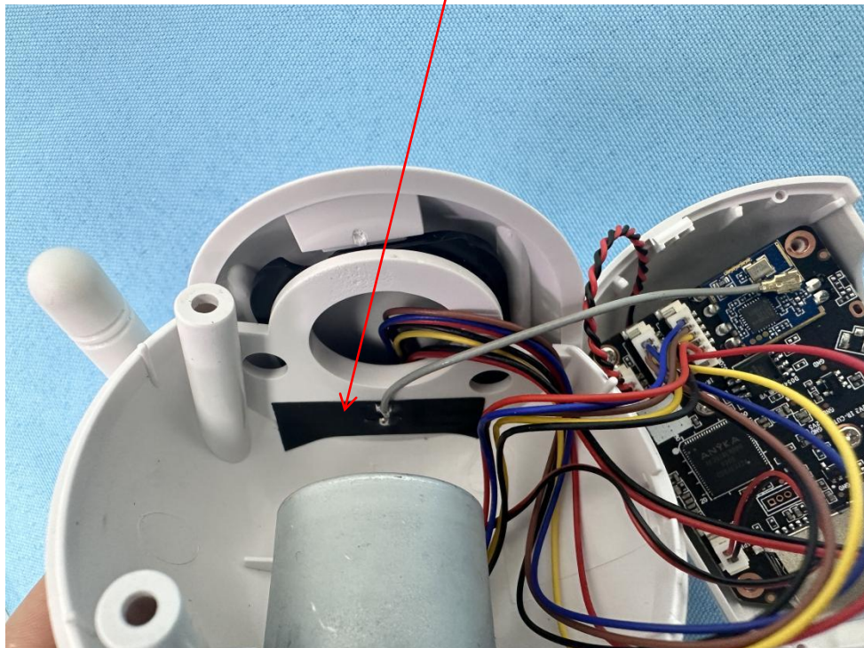
BT&WLAN ANT
