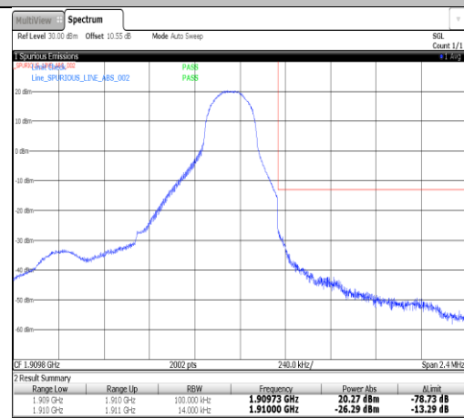
Band2-1.4MHz-QPSK-19193-1RB#5-PASS
