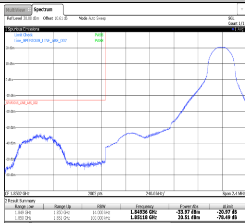
Band2-1.4MHz-QPSK-18607-1RB#5-PASS
