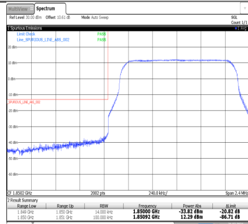
Band2-1.4MHz-QPSK-18607-6RB#0-PASS
