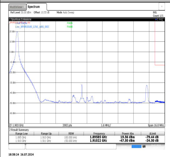
Band2-15MHz-QPSK-19125-1RB#74-PASS
