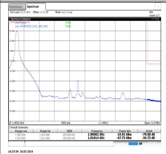
Band2-10MHz-QPSK-19150-1RB#49-PASS
