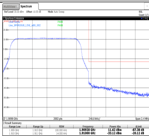
Band2-1.4MHz-QPSK-19193-6RB#0-PASS
