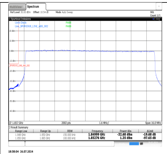
Band2-15MHz-QPSK-19125-1RB#0-PASS
