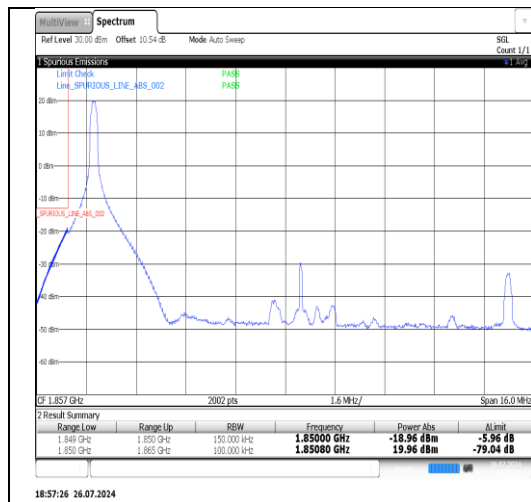
Band2-15MHz-QPSK-18675-1RB#74-PASS
