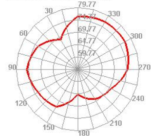
Wifi 161 TIS Phi=45
