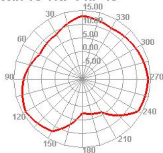
Wifi 60 TRP Phi=45
