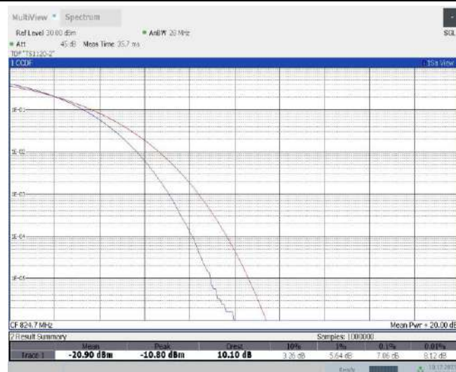
Band5-1.4MHz-QPSK-20525-1RB#0
