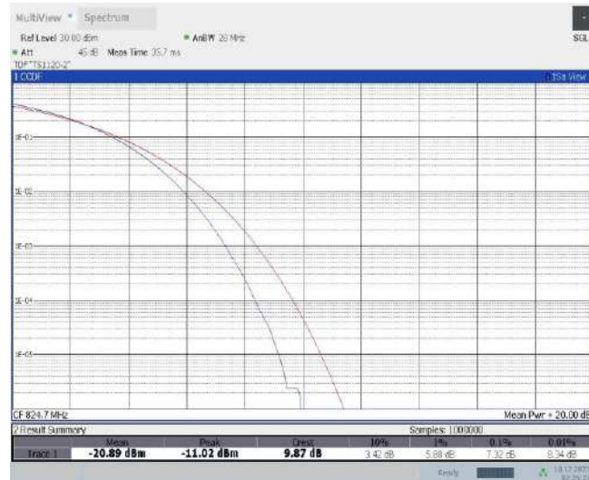
Band5-1.4MHz-16QAM-20525-1RB#0
