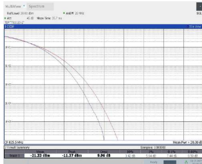
Band5-3MHz-16QAM-20415-15RB#0
