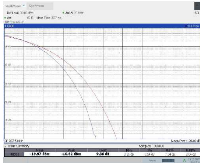
Band12-3MHz-QPSK-23095-15RB#0
