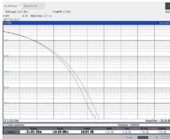
Band7-5MHz-16QAM-21100-25RB#0
