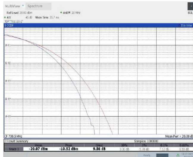
Band12-3MHz-QPSK-23025-15RB#0
