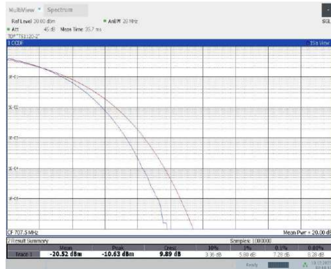
Band12-5MHz-QPSK-23095-25RB#0
