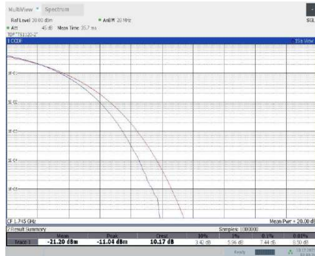
Band66-1.4MHz-QPSK-132322-6RB#0
