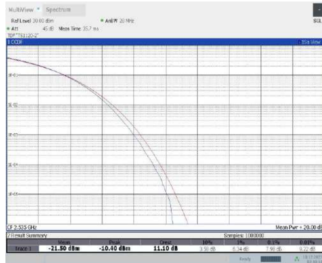
Band7-20MHz-16QAM-21100-100RB#0
