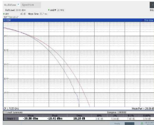
Band66-5MHz-QPSK-131997-25RB#0
