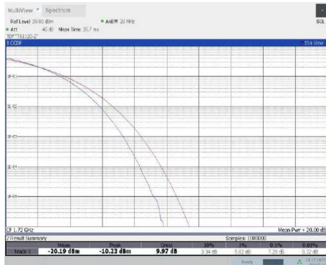
Band66-20MHz-QPSK-132072-100RB#0
