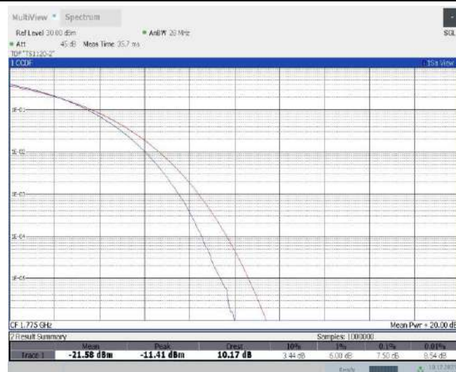
Band66-10MHz-QPSK-132622-50RB#0
