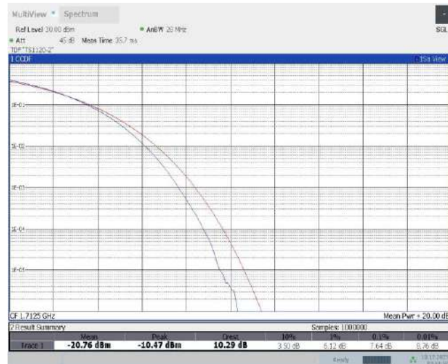
Band66-5MHz-16QAM-131997-25RB#0
