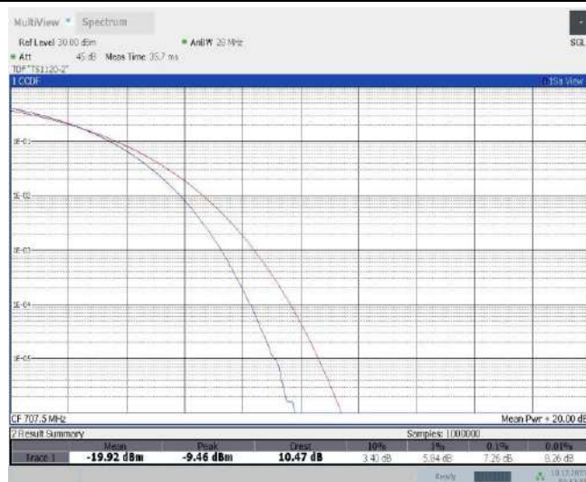
Band12-3MHz-16QAM-23095-15RB#0
