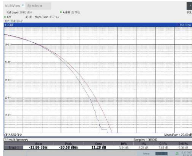
Band7-15MHz-QPSK-21100-75RB#0
