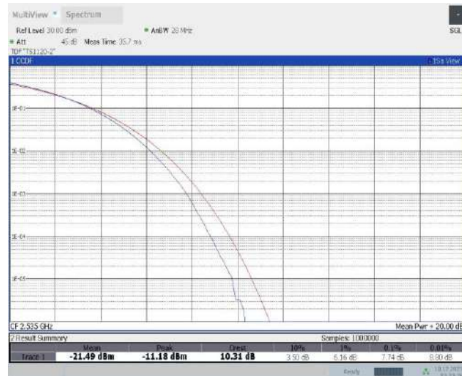
Band7-5MHz-QPSK-21425-1RB#0
