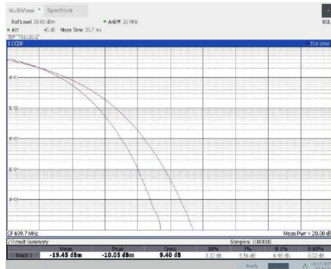
Band12-1.4MHz-QPSK-23017-6RB#0
