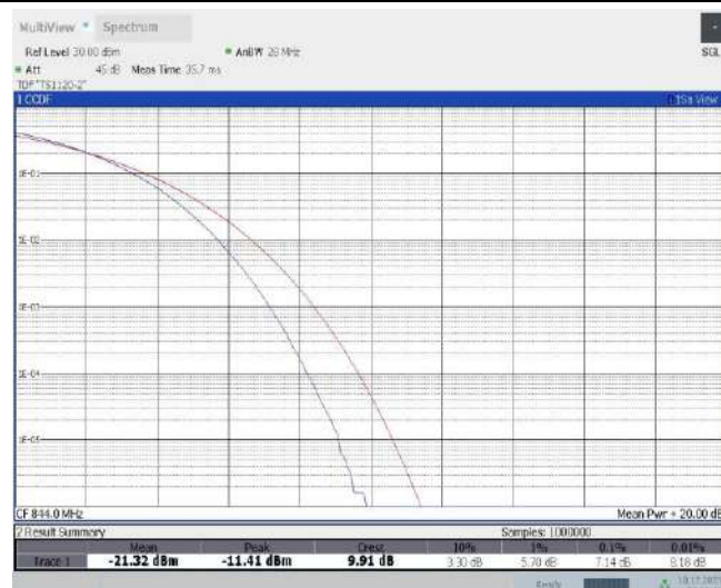
Band5-10MHz-QPSK-20600-50RB#0
