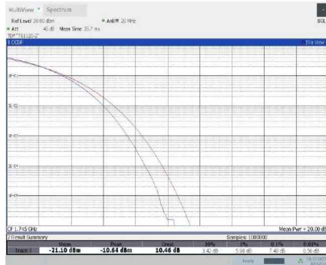
Band66-5MHz-QPSK-132322-25RB#0
