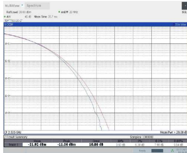
Band7-10MHz-16QAM-21100-50RB#0
