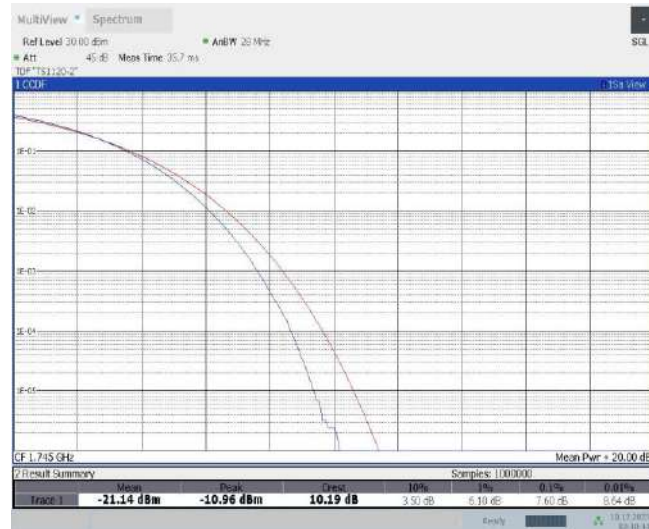
Band66-1.4MHz-16QAM-132322-6RB#0
