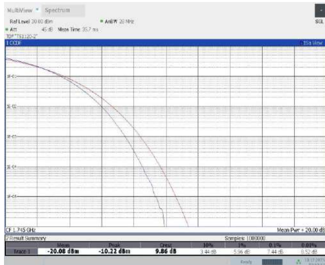
Band66-3MHz-16QAM-132657-1RB#0
