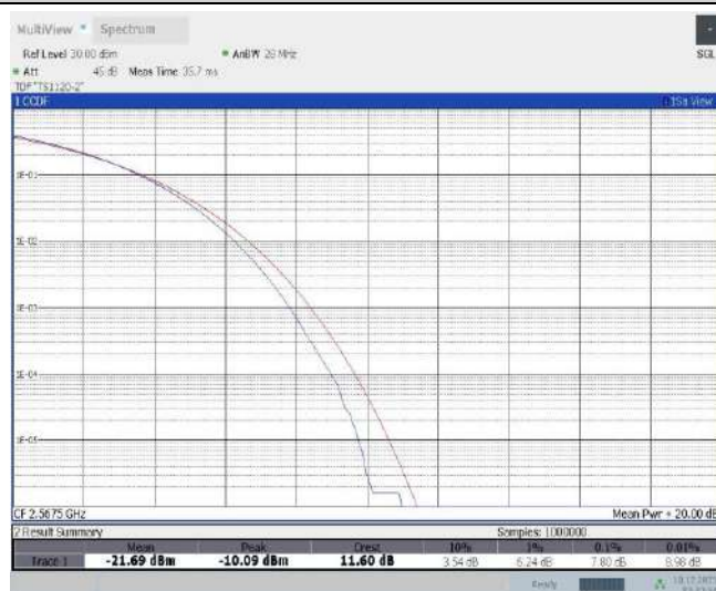
Band7-5MHz-16QAM-21425-25RB#0
