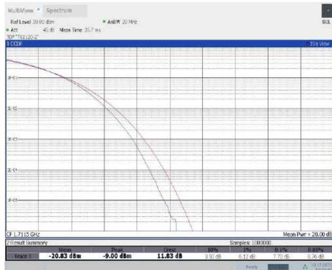
Band66-3MHz-16QAM-131987-15RB#0
