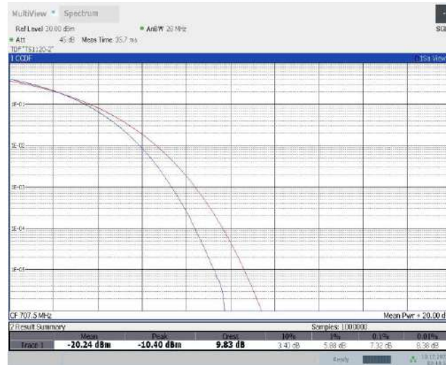
Band12-5MHz-16QAM-23095-25RB#0
