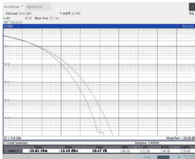
Band66-3MHz-16QAM-132322-15RB#0
