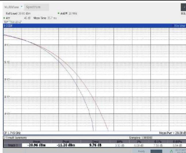
Band66-10MHz-16QAM-132322-50RB#0
