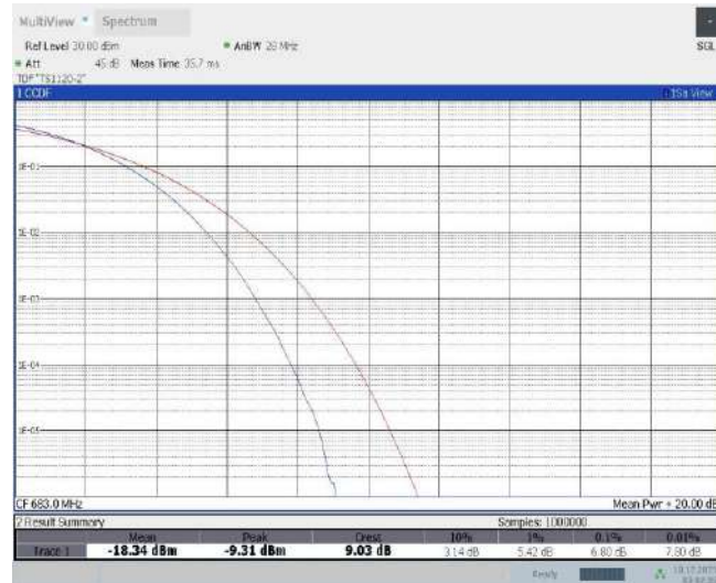
Band71-20MHz-QPSK-133322-100RB#0
