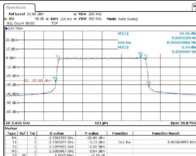
Band7-10MHz-QPSK-21400-50RB#0
