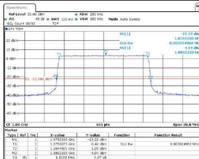
Band2-10MHz-QPSK-19150-50RB#0
