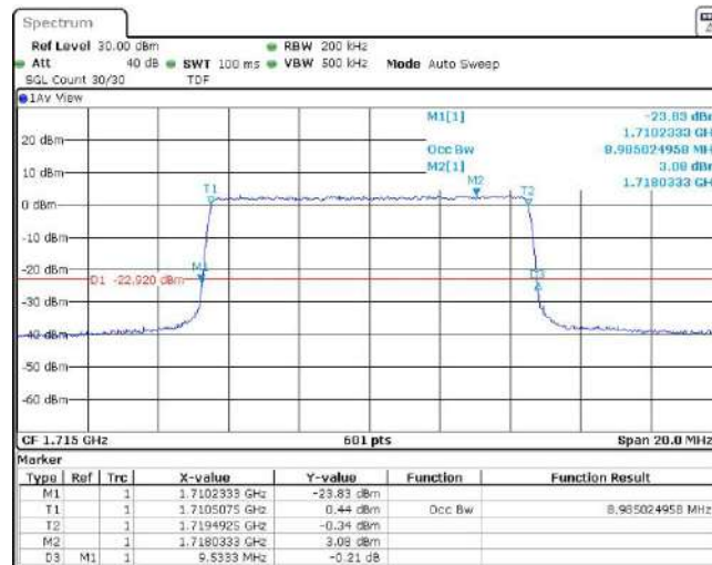
Band4-10MHz-QPSK-20175-50RB#0
