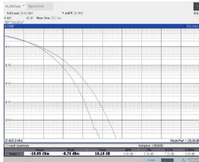
Band71-5MHz-16QAM-133147-25RB#0
