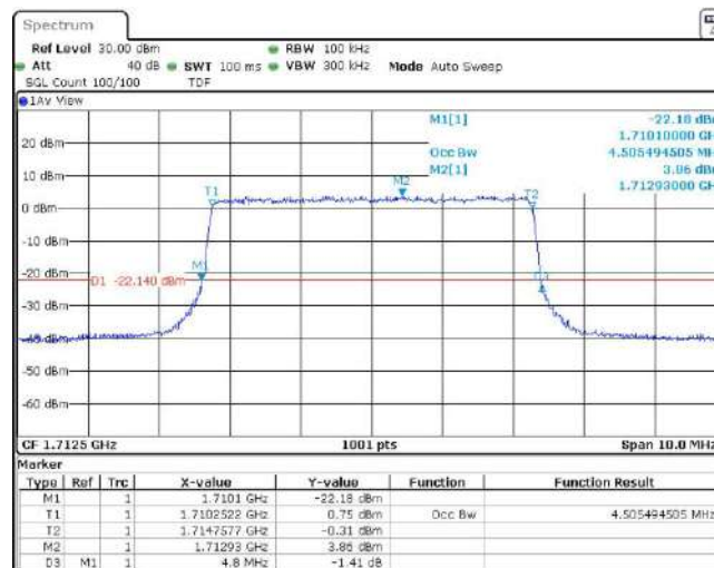
Band4-5MHz-QPSK-20175-25RB#0
