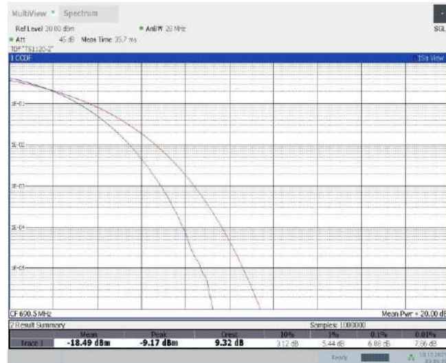
Band71-15MHz-16QAM-133197-1RB#0
