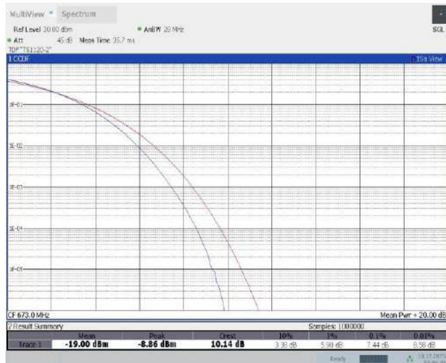
Band71-20MHz-16QAM-133222-100RB#0
