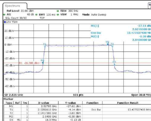
Band7-15MHz-QPSK-21375-75RB#0
