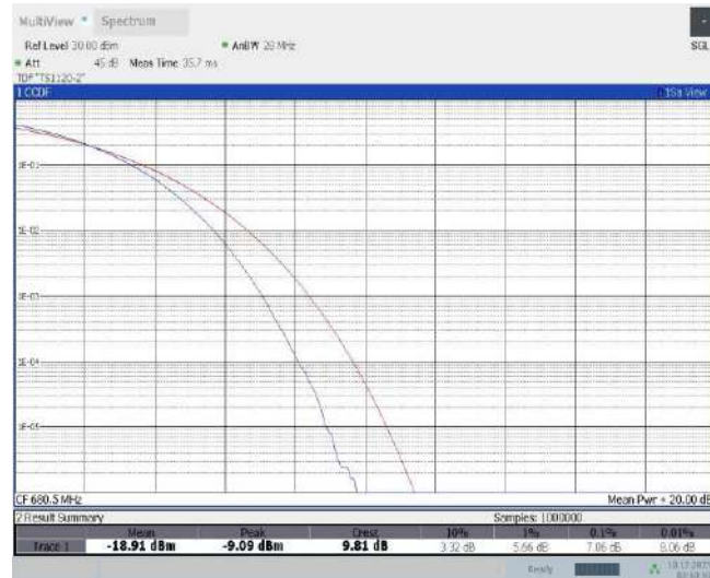
Band71-5MHz-16QAM-133297-25RB#0
