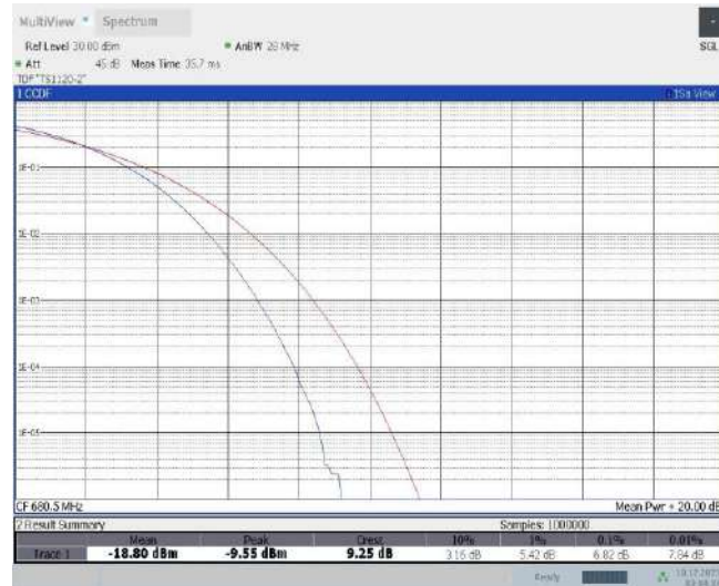
Band71-15MHz-QPSK-133297-75RB#0
