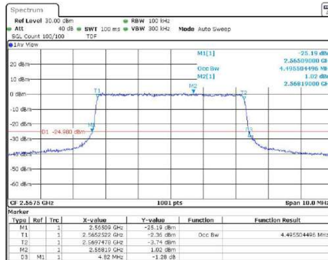
Band7-5MHz-16QAM-20775-25RB#0
