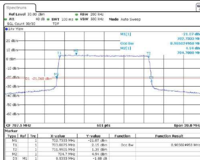
Band12-10MHz-QPSK-23130-50RB#0
