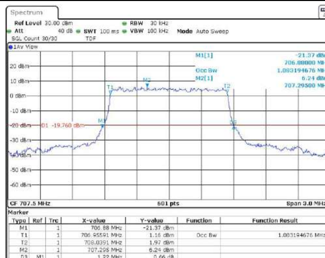
Band12-1.4MHz-16QAM-23173-6RB#0
