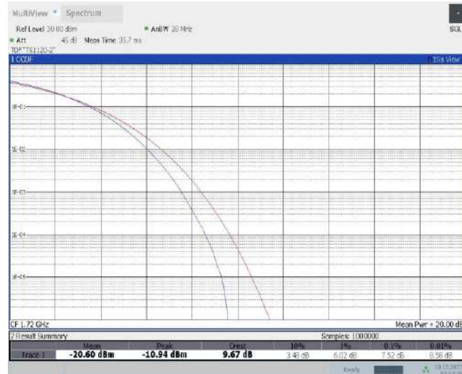
Band66-20MHz-16QAM-132072-100RB#0
