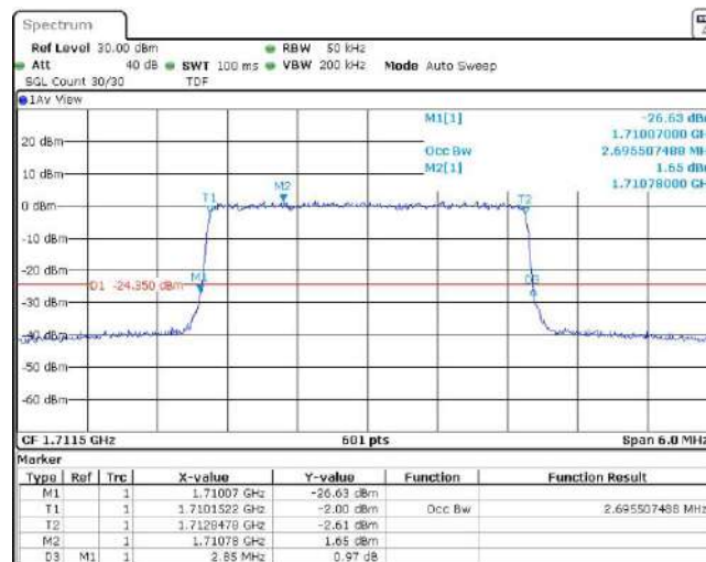
Band4-3MHz-16QAM-20175-15RB#0
