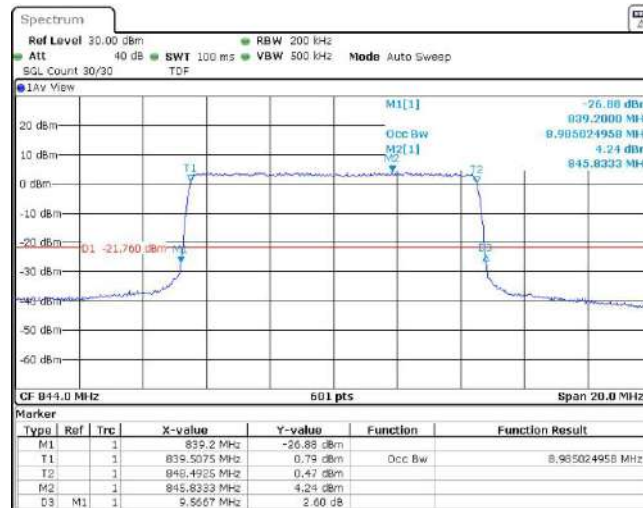
Band5-10MHz-16QAM-20450-50RB#0
