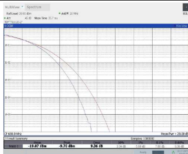
Band71-20MHz-16QAM-133372-100RB#0
