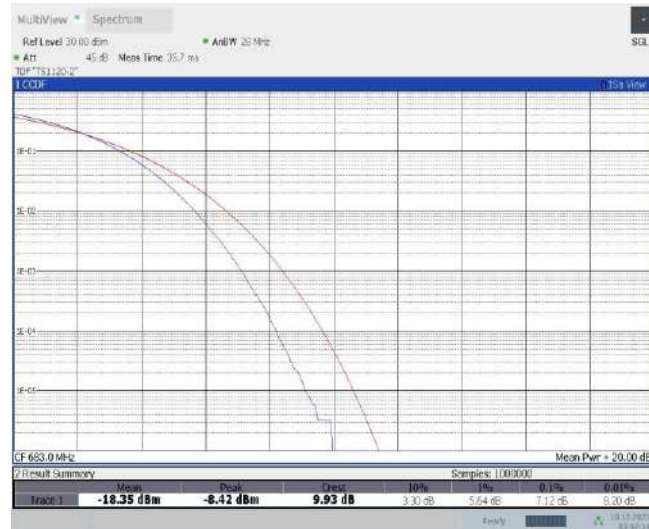
Band71-20MHz-16QAM-133322-100RB#0
