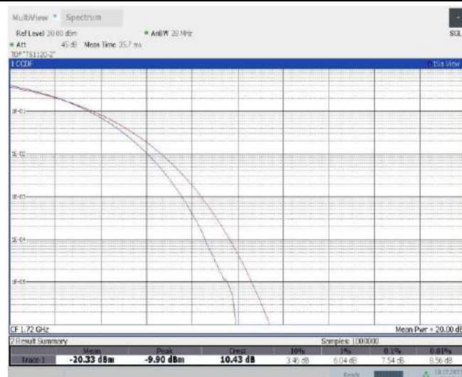
Band66-20MHz-16QAM-132322-1RB#0
