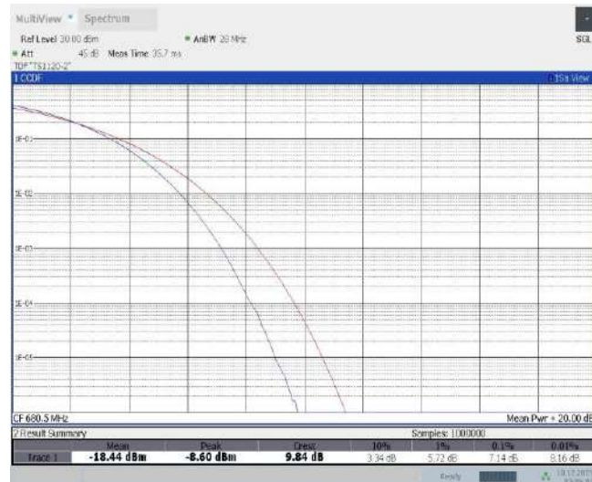
Band71-15MHz-16QAM-133397-1RB#0
