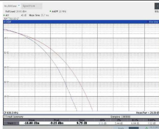
Band71-15MHz-QPSK-133397-75RB#0
