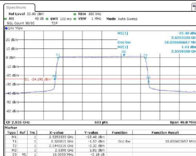
Band7-20MHz-QPSK-21350-100RB#0
