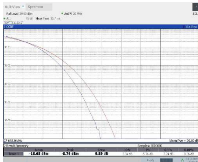
Band71-10MHz-16QAM-133172-50RB#0
