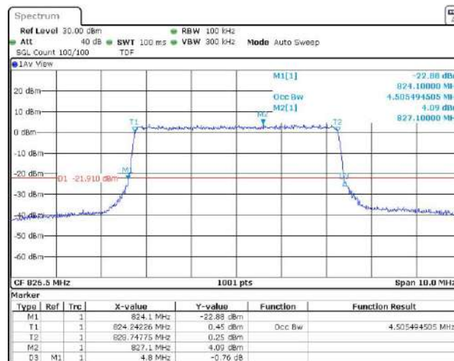
Band5-5MHz-16QAM-20525-25RB#0
