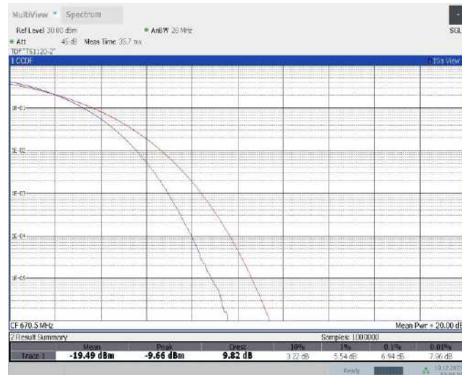
Band71-15MHz-QPSK-133197-75RB#0
