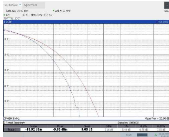
Band71-10MHz-QPSK-133297-50RB#0
