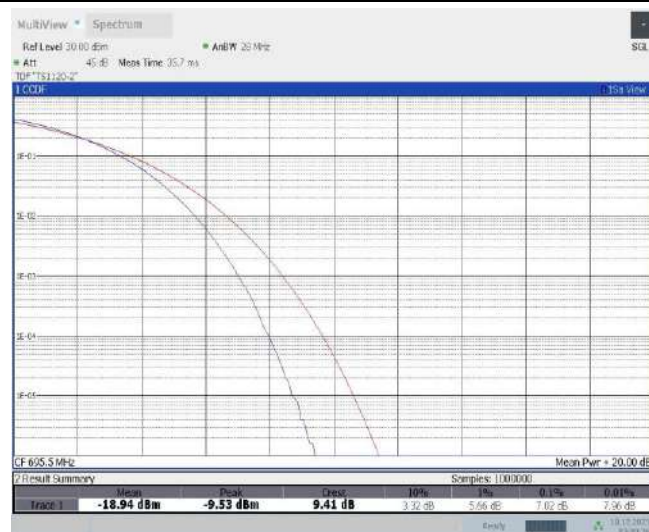
Band71-5MHz-16QAM-133447-25RB#0
