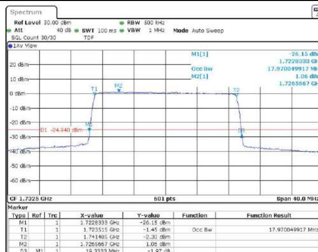
Band4-20MHz-16QAM-20300-100RB#0
