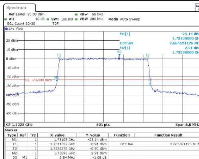
Band4-3MHz-16QAM-20385-15RB#0
