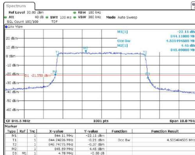
Band5-5MHz-16QAM-20425-25RB#0
