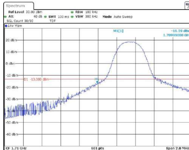
Band4-5MHz-QPSK-19975-1RB#24
