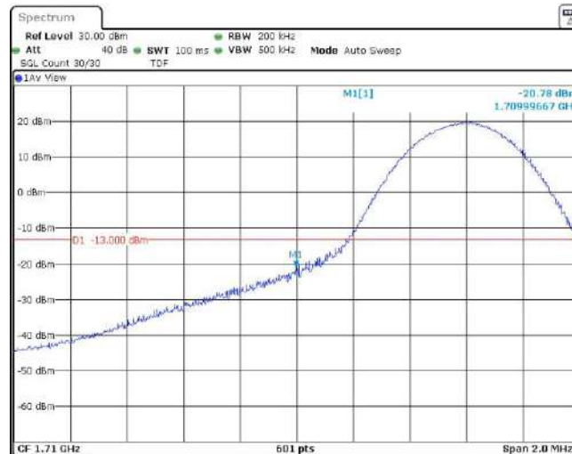
Band4-10MHz-16QAM-20000-1RB#49
