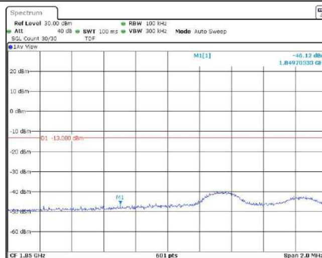
Band2-5MHz-16QAM-18625-25RB#0
