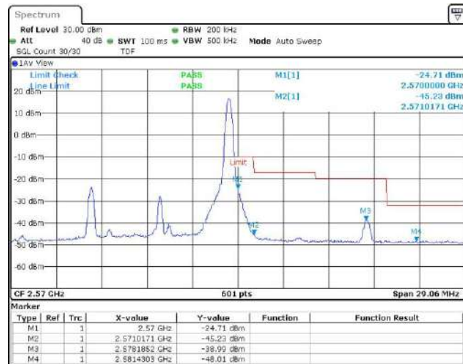
Band7-10MHz-QPSK-21400-50RB#0
