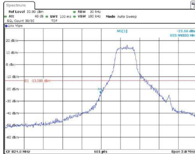
Band5-1.4MHz-16QAM-20407-1RB#5
