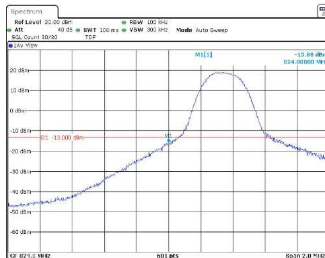
Band5-5MHz-QPSK-20425-1RB#24
