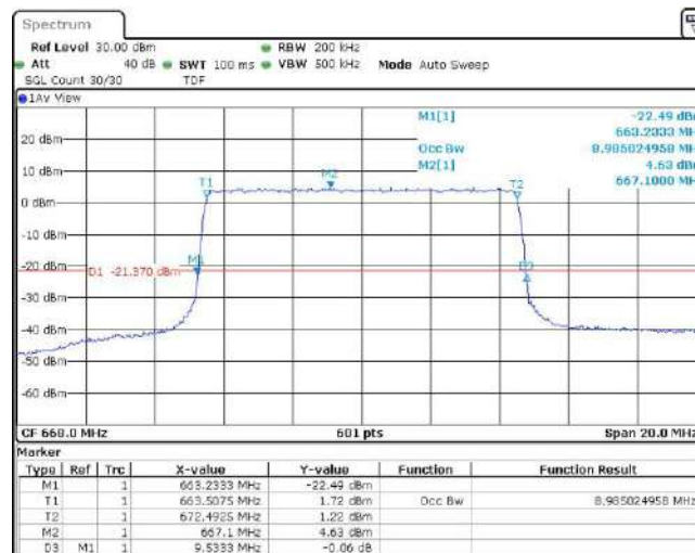
Band71-10MHz-QPSK-133297-50RB#0
