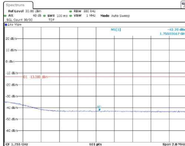
Band4-20MHz-16QAM-20300-1RB#99
