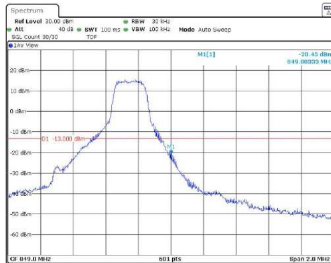
Band5-1.4MHz-QPSK-20643-6RB#0
