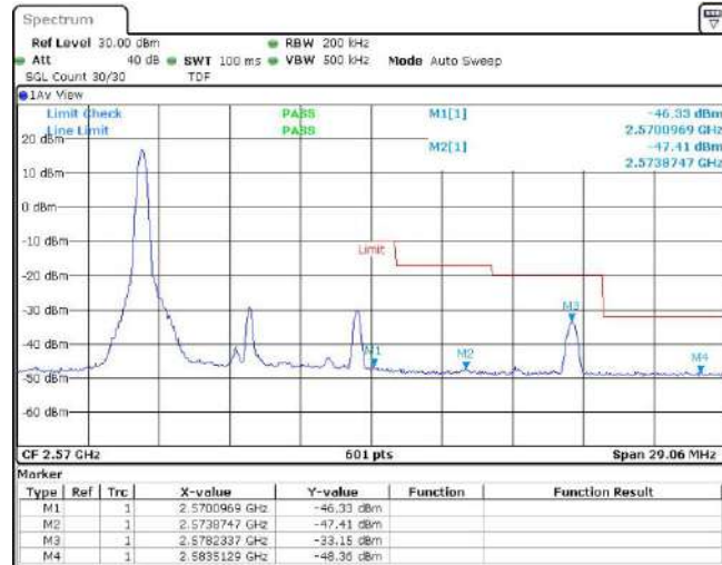
Band7-10MHz-QPSK-21400-1RB#49
