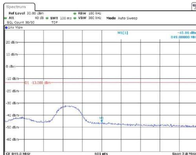
Band5-5MHz-QPSK-20625-1RB#24
