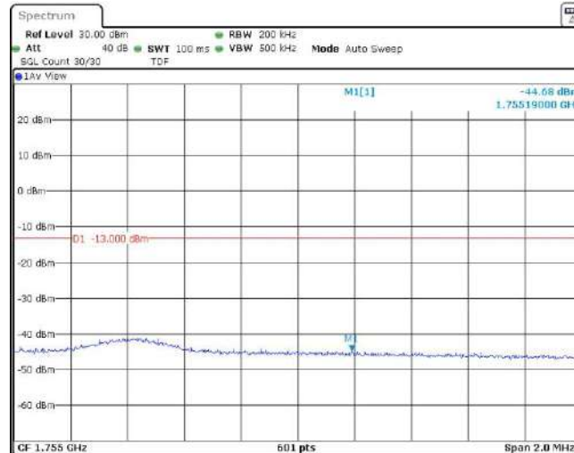
Band4-10MHz-16QAM-20350-1RB#49
