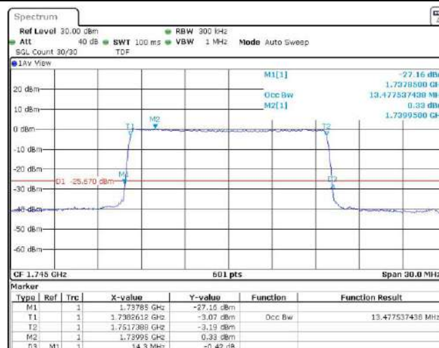
Band66-15MHz-16QAM-132597-75RB#0
