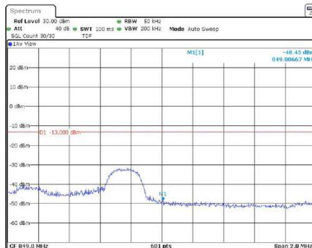
Band5-3MHz-16QAM-20635-1RB#14
