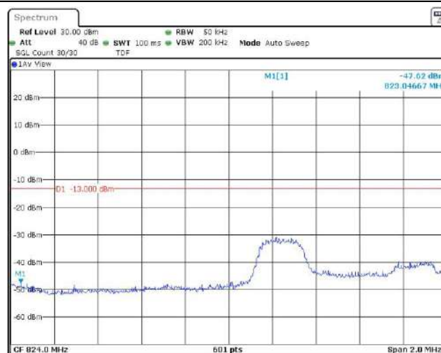
Band5-3MHz-16QAM-20415-15RB#0
