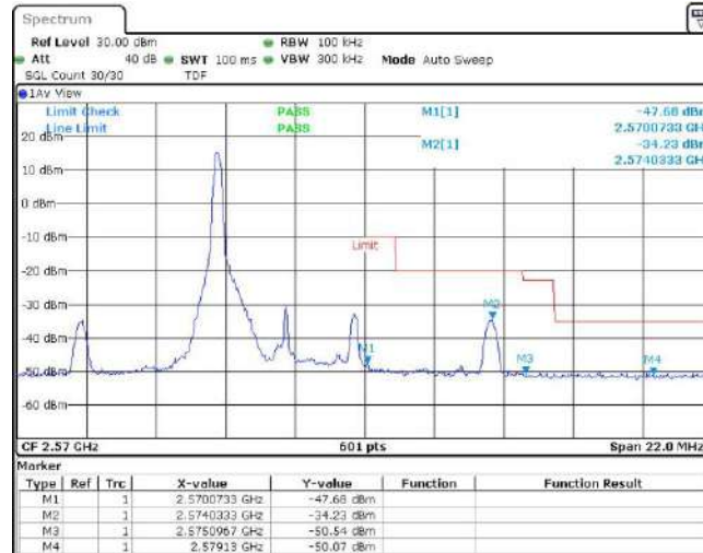
Band7-5MHz-QPSK-21425-1RB#24
