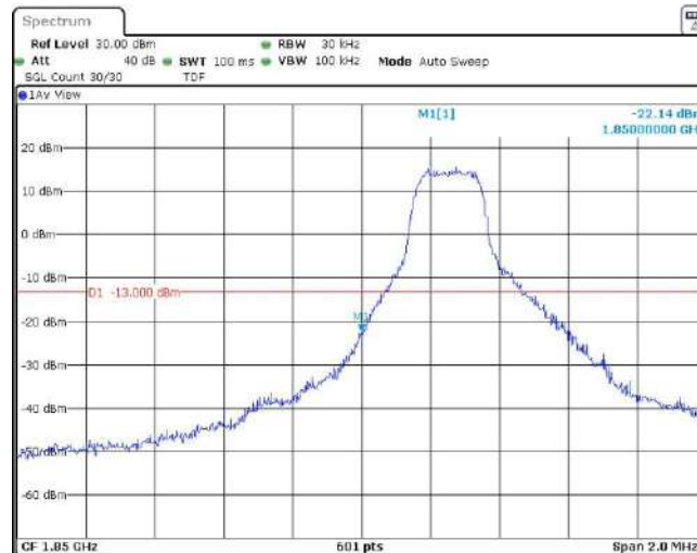
Band2-1.4MHz-QPSK-18607-1RB#5
