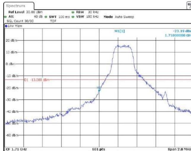
Band4-1.4MHz-QPSK-19957-1RB#5
