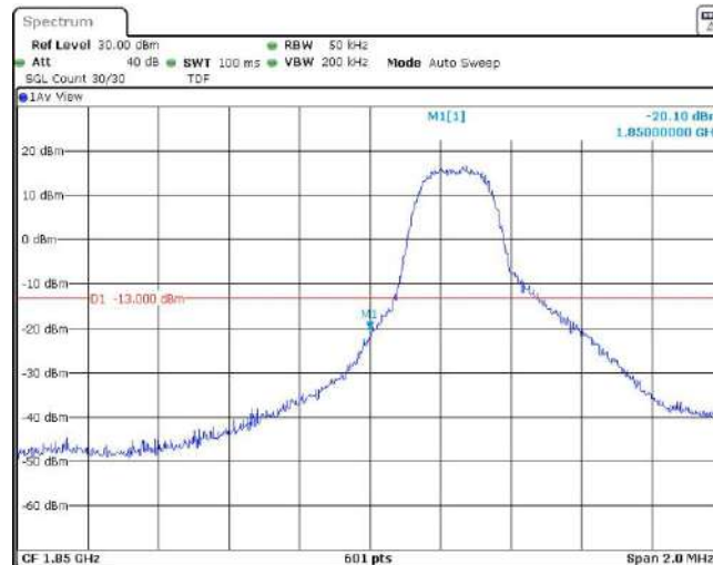
Band2-3MHz-16QAM-18615-1RB#14
