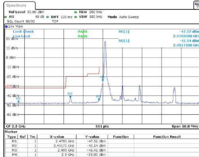
Band7-10MHz-QPSK-20800-1RB#49
