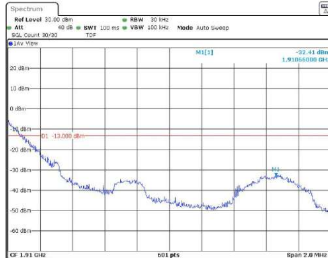
Band2-1.4MHz-QPSK-19193-1RB#5
