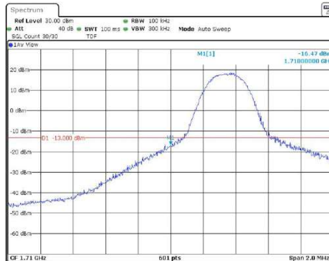
Band4-5MHz-16QAM-19975-1RB#24
