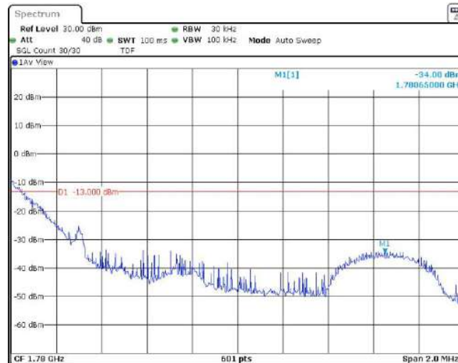
Band66-1.4MHz-16QAM-132665-1RB#5
