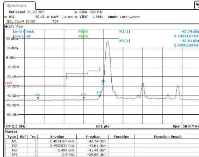
Band7-20MHz-QPSK-20850-1RB#99
