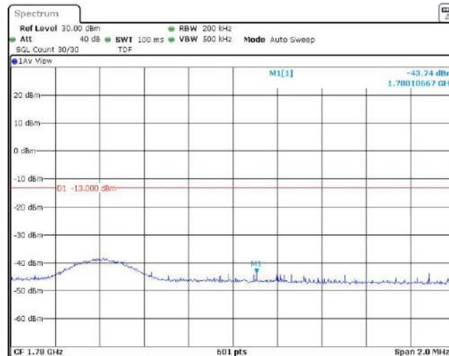
Band66-10MHz-16QAM-132622-1RB#49
