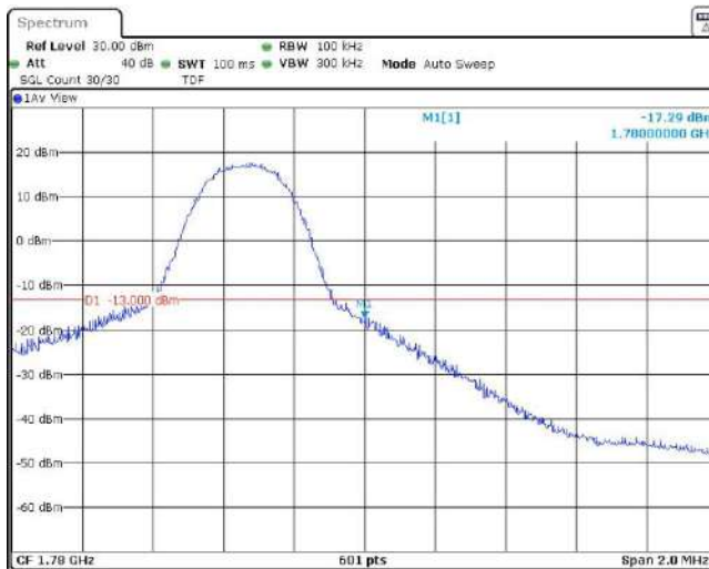
Band66-5MHz-16QAM-132647-25RB#0
