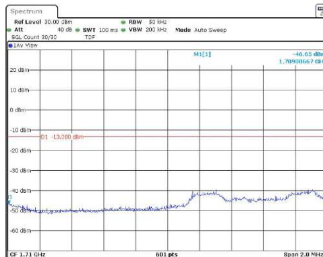
Band66-3MHz-16QAM-131987-15RB#0
