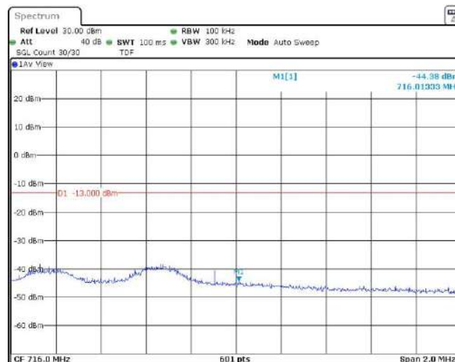
Band12-5MHz-QPSK-23155-1RB#24
