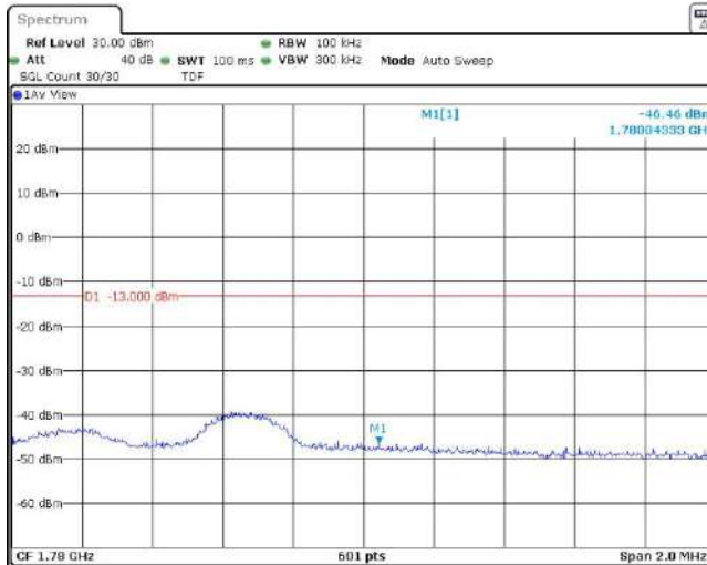
Band66-5MHz-16QAM-132647-1RB#24
