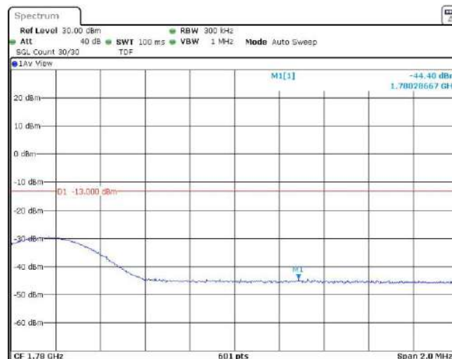
Band66-15MHz-QPSK-132597-1RB#74
