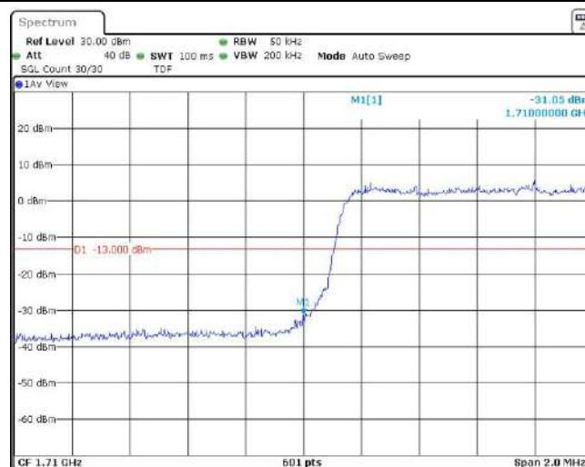
Band66-3MHz-16QAM-132657-1RB#0
