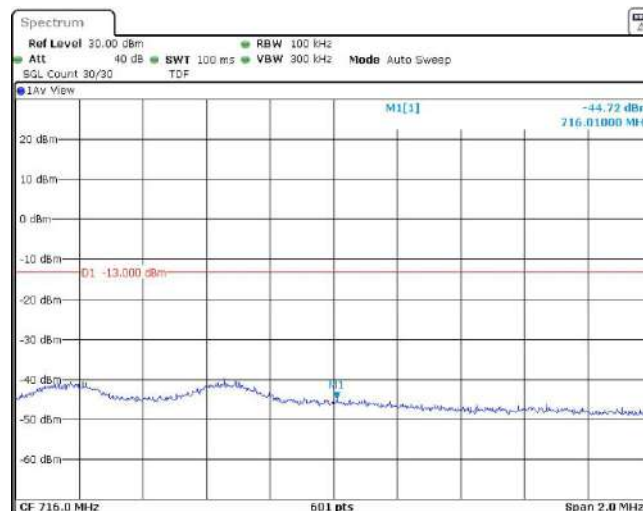
Band12-5MHz-16QAM-23155-1RB#24
