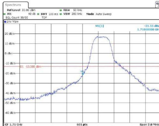
Band66-3MHz-QPSK-131987-1RB#14
