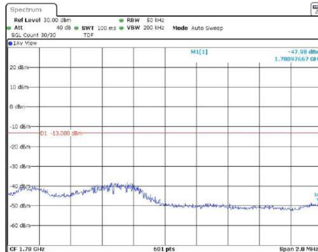
Band66-3MHz-QPSK-132657-1RB#14
