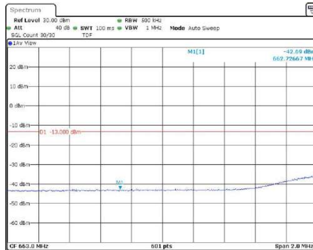
Band71-20MHz-16QAM-133222-100RB#0
