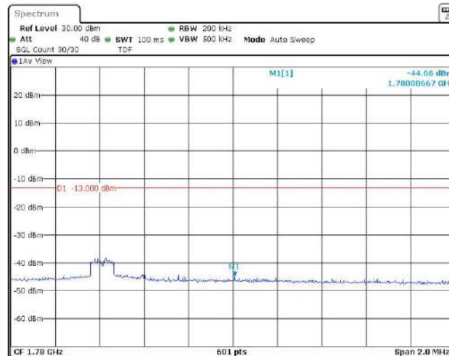
Band66-10MHz-QPSK-132622-1RB#49
