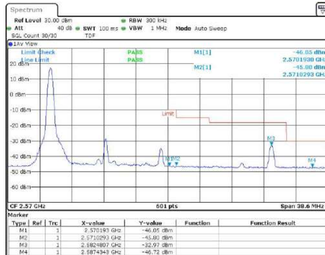
Band7-15MHz-QPSK-21375-1RB#74
