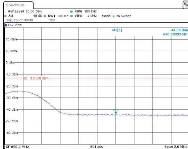
Band71-15MHz-16QAM-133397-1RB#74
