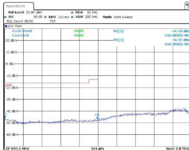
Band12-3MHz-QPSK-23025-15RB#0
