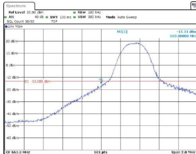
Band71-5MHz-16QAM-133147-1RB#24
