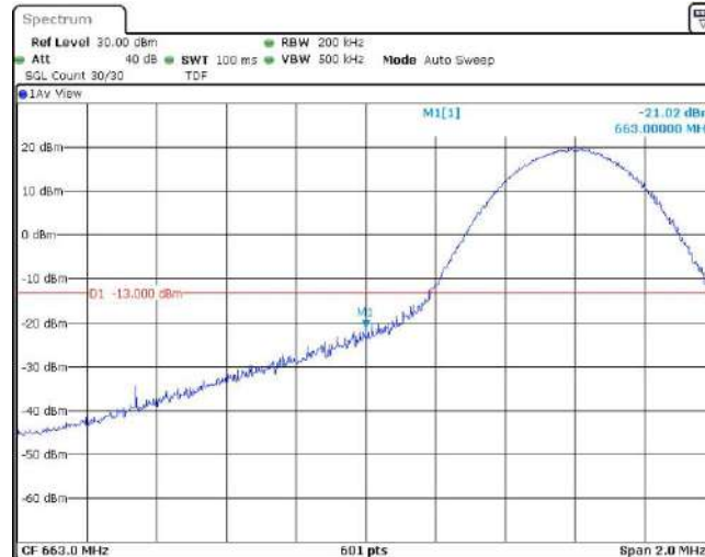
Band71-10MHz-16QAM-133172-1RB#49
