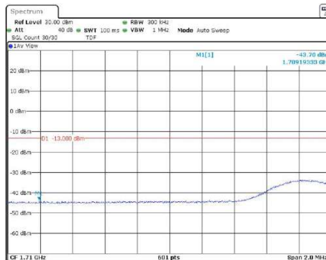
Band66-15MHz-16QAM-132047-75RB#0
