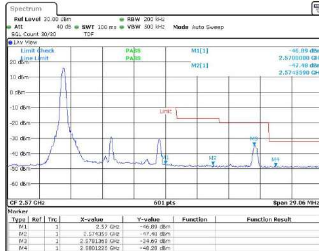
Band7-10MHz-16QAM-21400-1RB#49
