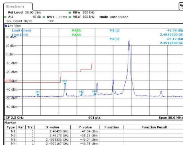
Band7-10MHz-16QAM-20800-50RB#0
