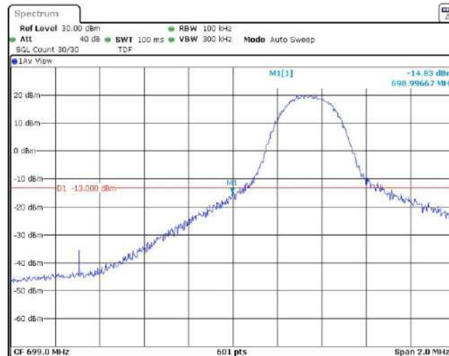
Band12-5MHz-16QAM-23035-1RB#24
