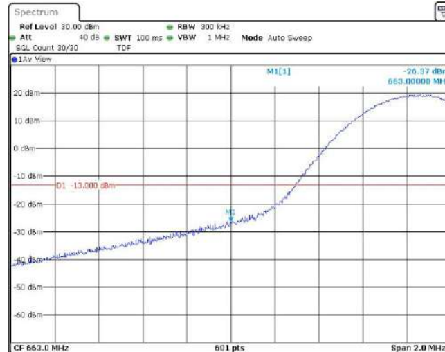
Band71-15MHz-16QAM-133197-1RB#74
