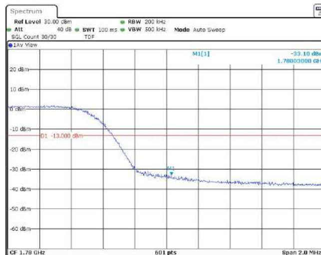
Band66-15MHz-QPSK-132047-1RB#0
