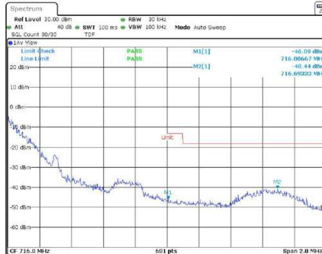
Band12-1.4MHz-16QAM-23173-1RB#5
