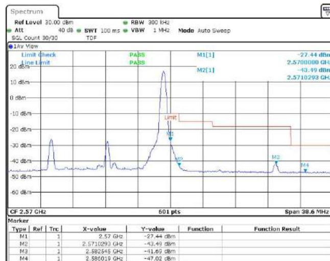
Band7-15MHz-QPSK-21375-75RB#0
