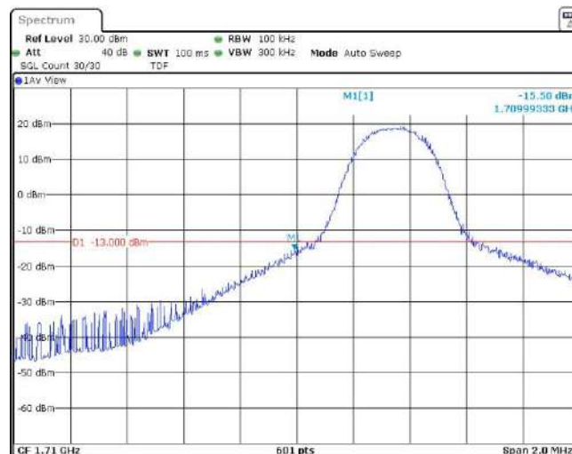
Band66-5MHz-QPSK-131997-1RB#24
