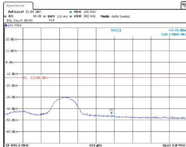
Band71-5MHz-16QAM-133447-1RB#24
