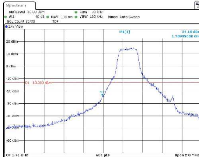
Band66-1.4MHz-16QAM-131979-1RB#5
