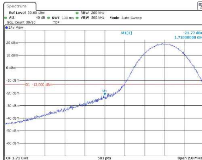
Band66-10MHz-16QAM-132022-1RB#49
