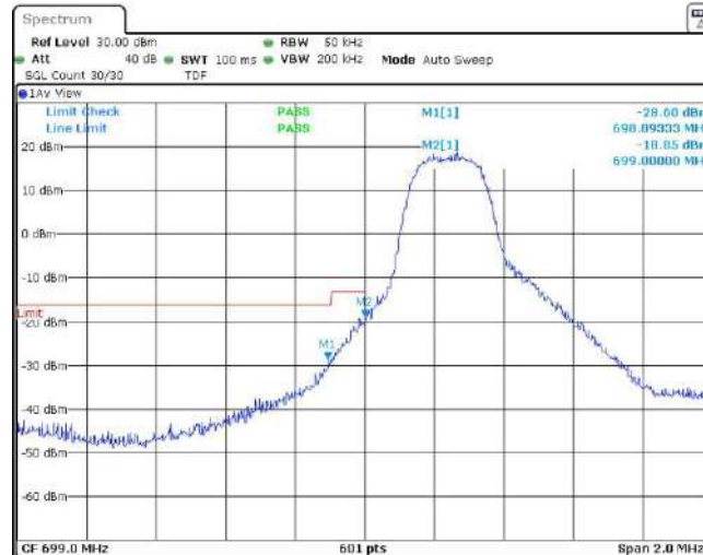
Band12-3MHz-16QAM-23025-1RB#14
