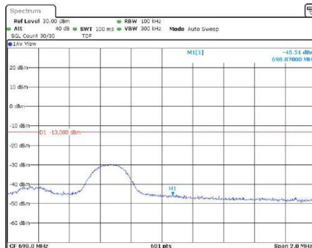
Band71-5MHz-QPSK-133447-1RB#24
