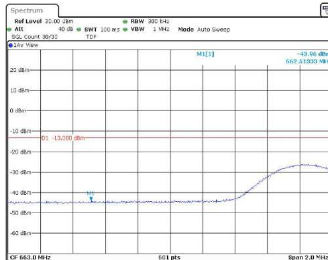
Band71-15MHz-16QAM-133197-75RB#0
