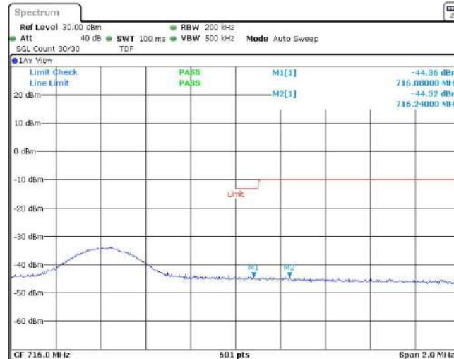
Band12-10MHz-16QAM-23130-1RB#49
