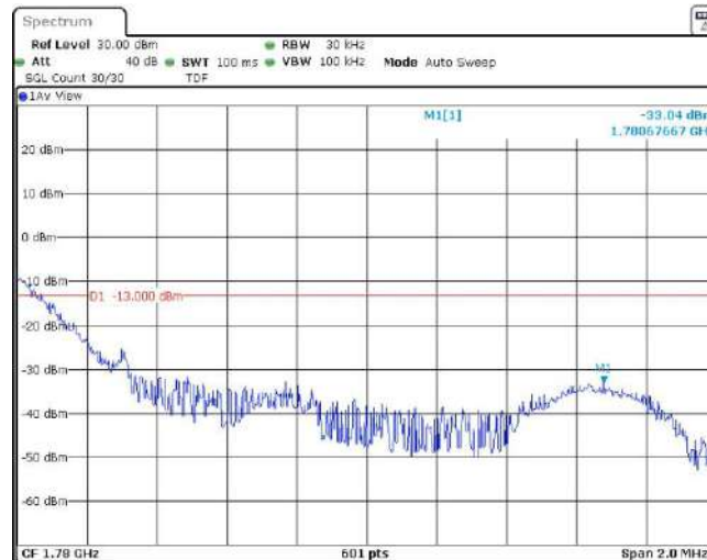
Band66-1.4MHz-QPSK-132665-1RB#5
