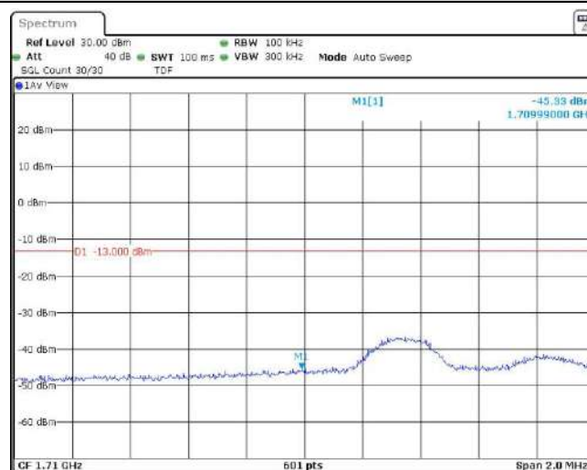
Band66-5MHz-QPSK-131997-25RB#0
