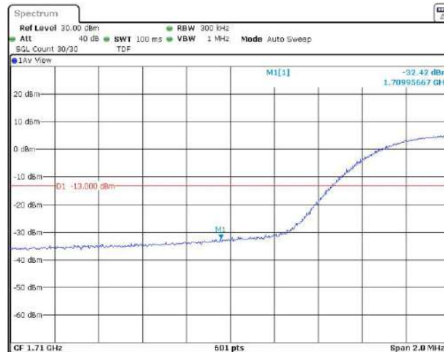
Band66-15MHz-QPSK-132047-1RB#74
