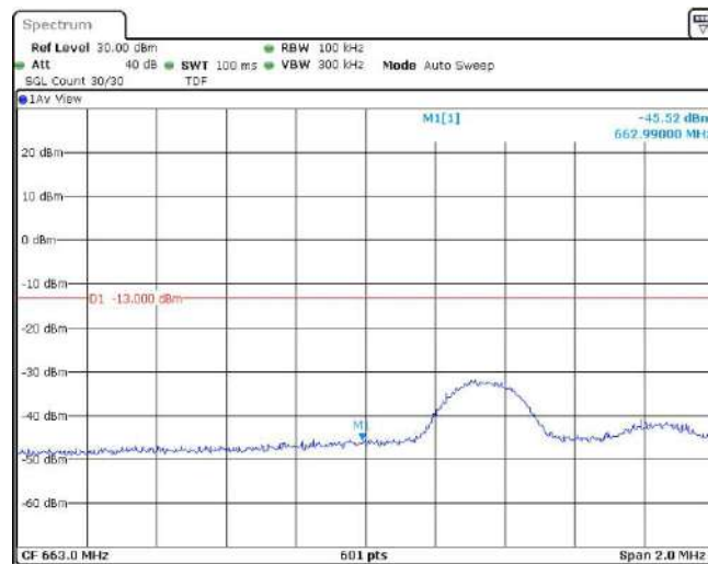
Band71-5MHz-16QAM-133147-25RB#0
