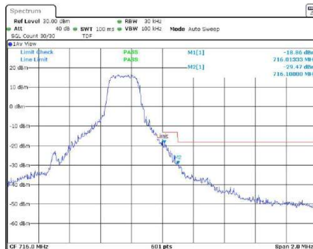
Band12-1.4MHz-QPSK-23173-6RB#0
