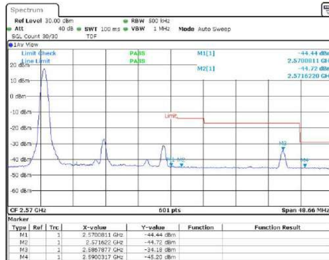
Band7-20MHz-QPSK-21350-1RB#99
