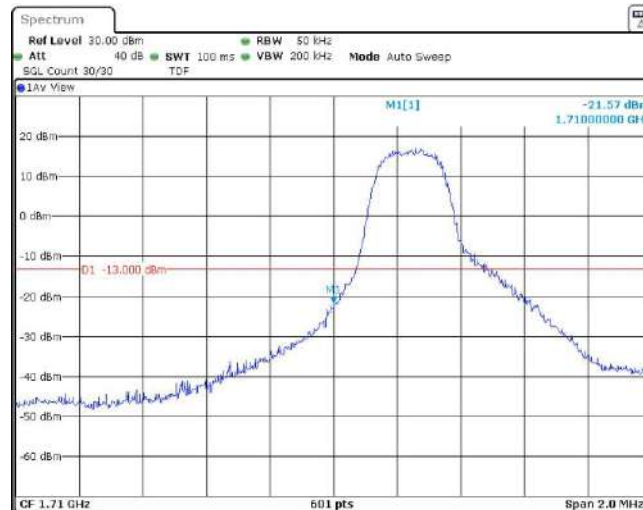
Band66-3MHz-16QAM-131987-1RB#14
