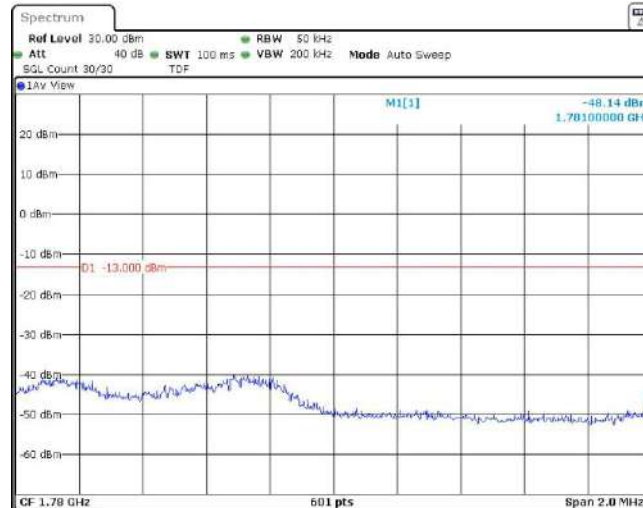
Band66-3MHz-16QAM-132657-1RB#14
