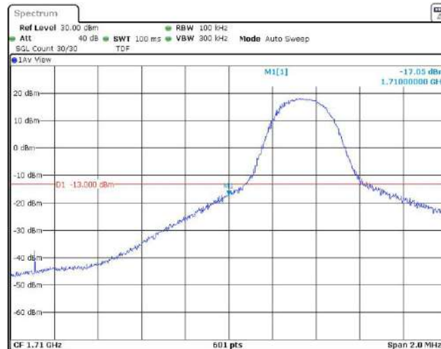
Band66-5MHz-16QAM-131997-1RB#24
