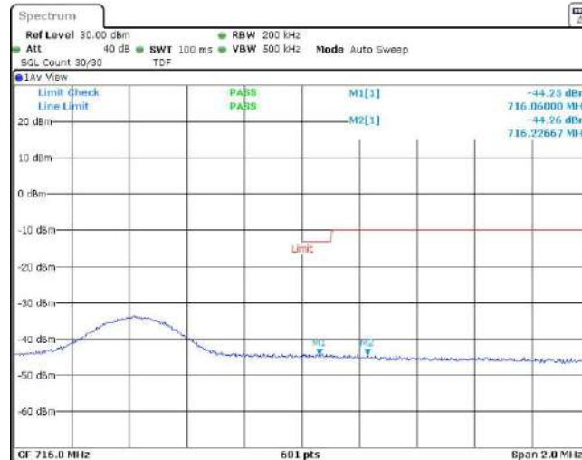
Band12-10MHz-QPSK-23130-1RB#49
