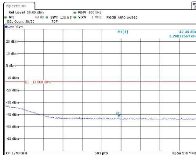
Band66-20MHz-16QAM-132572-1RB#99
