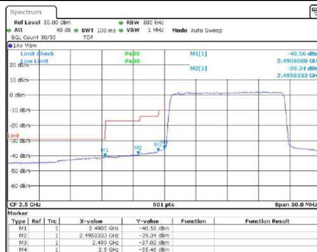
Band7-20MHz-QPSK-21350-1RB#0
