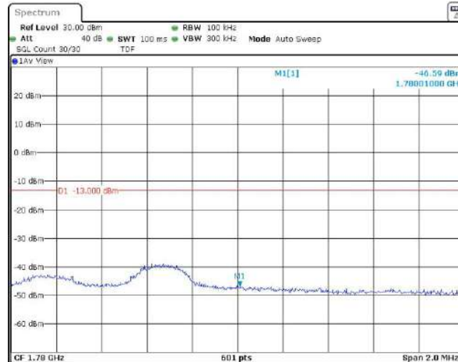
Band66-5MHz-QPSK-132647-1RB#24
