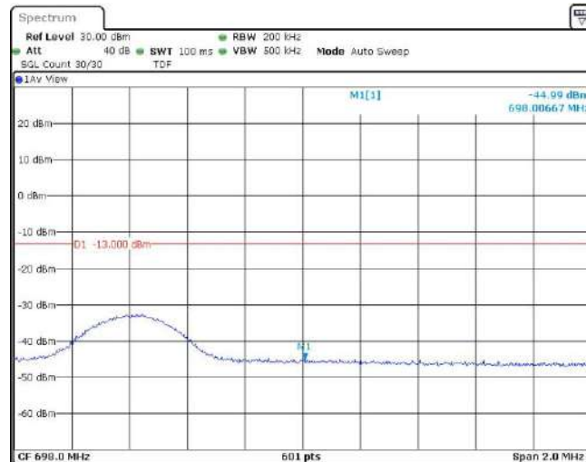
Band71-10MHz-16QAM-133422-1RB#49
