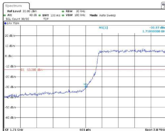
Band66-1.4MHz-16QAM-132665-1RB#0
