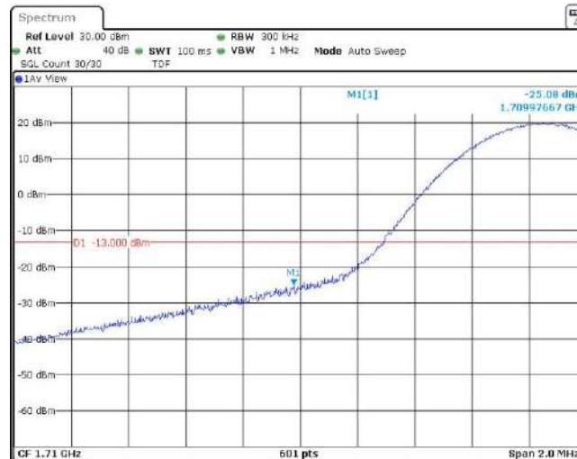
Band66-15MHz-16QAM-132047-1RB#74
