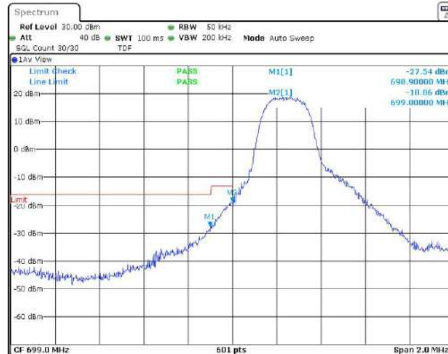
Band12-3MHz-QPSK-23025-1RB#14
