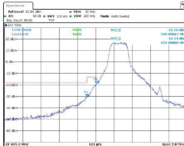
Band12-1.4MHz-QPSK-23017-1RB#5
