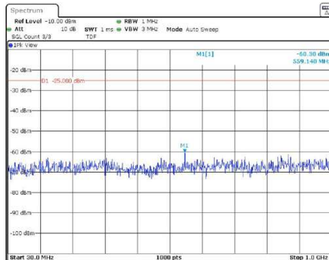
Band7-20MHz-16QAM-21100-1RB#0-Range2:1000~3000MHz
