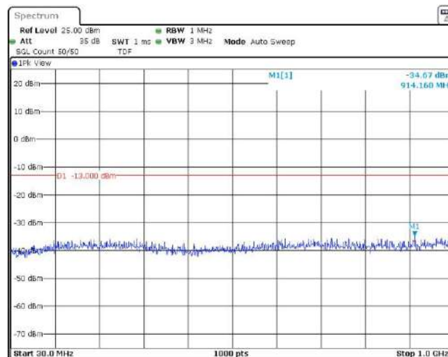
Band4-1.4MHz-16QAM-20175-1RB#0-Range2:1000~2000MHz
