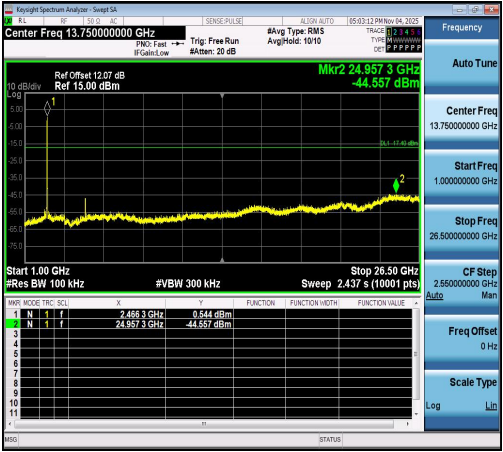
11G-Ant1-2462-1000~26500-PASS
