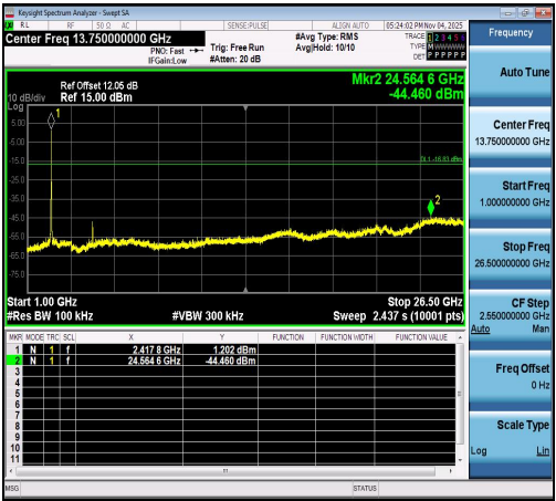
11N20SISO-Ant1-2412-1000~26500-PASS
