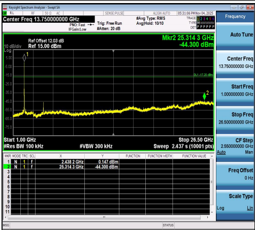
11N20SISO-Ant1-2437-1000~26500-PASS
