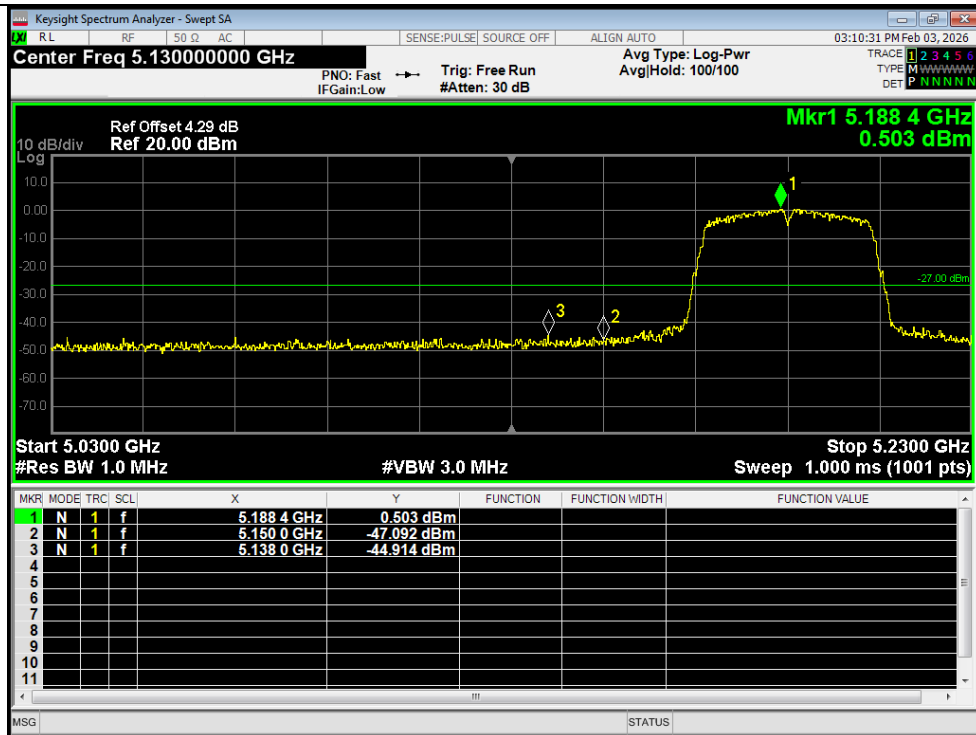
Bandedge_NVNT_ANT1_802_11ac(VHT40) 5230
