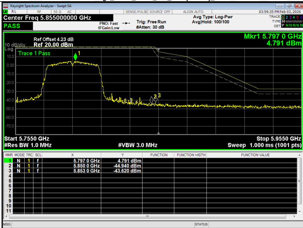
Bandedge_NVNT_ANT1_802_11ac(VHT80) 5775
