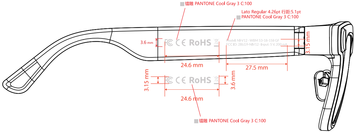
L边-内壳
