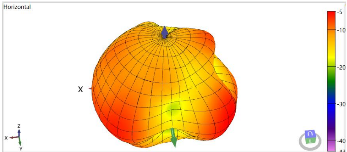
antenna天线 2440MHz 3D-Horizontal Pattern
