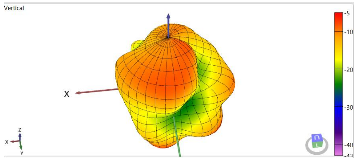
antenna天线 2440MHz 3D-Vertical Pattern
