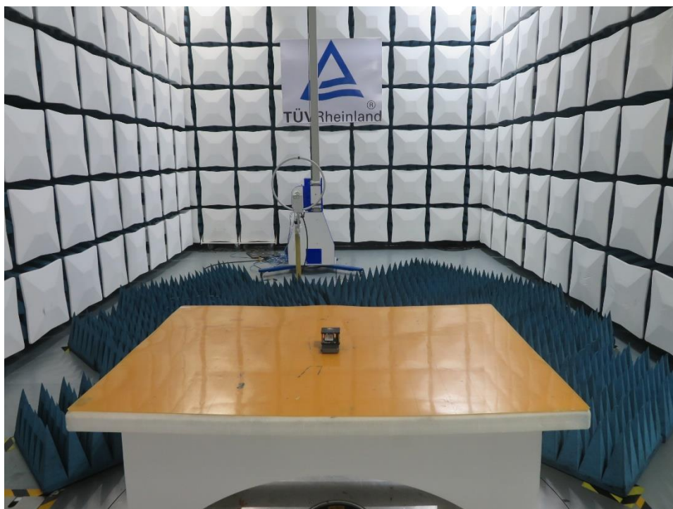
Photograph 2: Set-up photo for Radiated Emission, Below 30MHz
