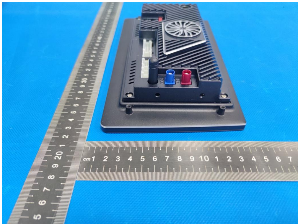
Photo 8 (2G/3G/4G Antenna)
