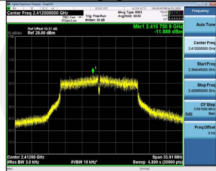
11G Ant2 2412
