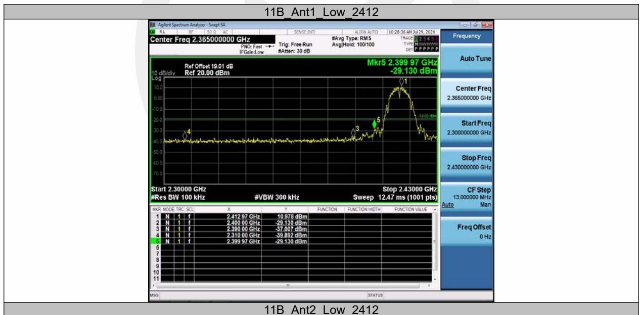
Band Edge Test Graph
