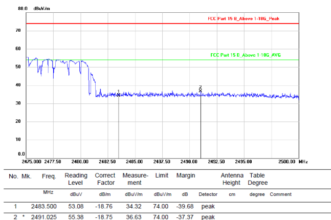
Test Mode: GFSK-High Hopping-on
