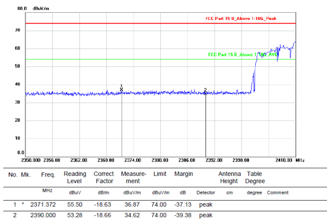
Test Mode: GFSK-Low Hopping-on
