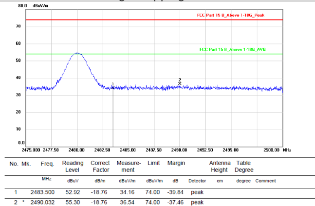
Test Mode: GFSK-High Hopping-off
