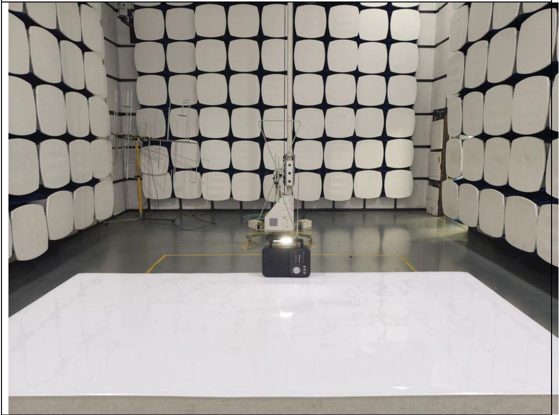
Radiated Emission
