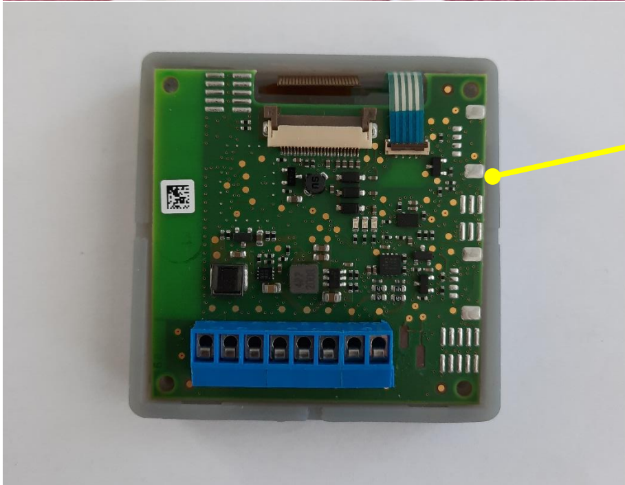
PCBA inserted in the housing (plastic part)
