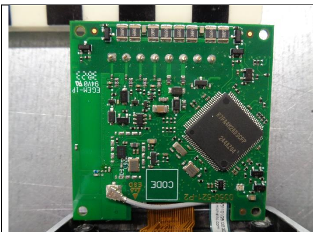
Antenna side with antenna connection
