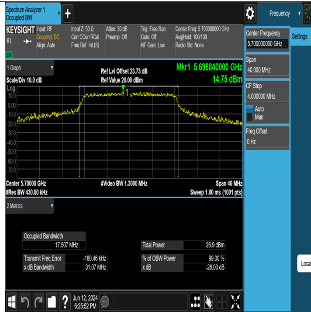
11A-Ant3-5700
