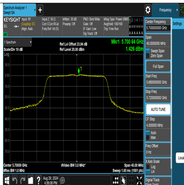
11N20MIMO-Ant3-5700-PASS
