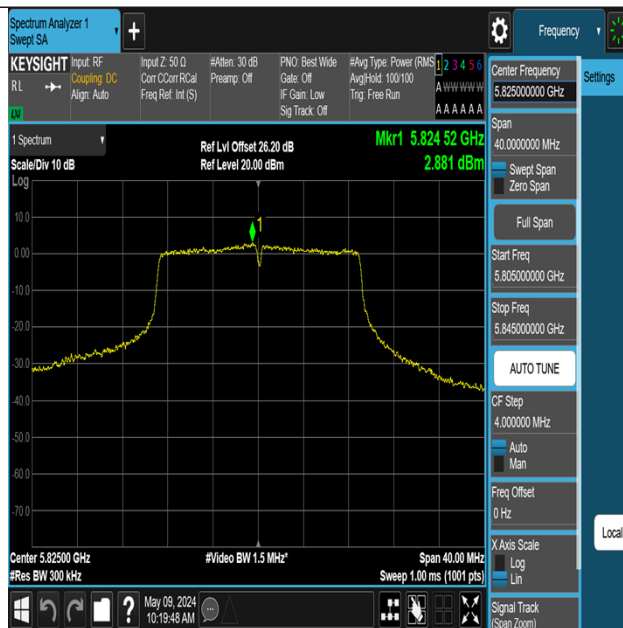
11N20MIMO-Ant2-5825-PASS
