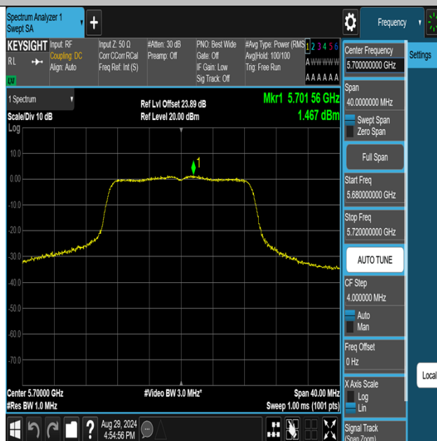
11N20MIMO-Ant2-5700-PASS
