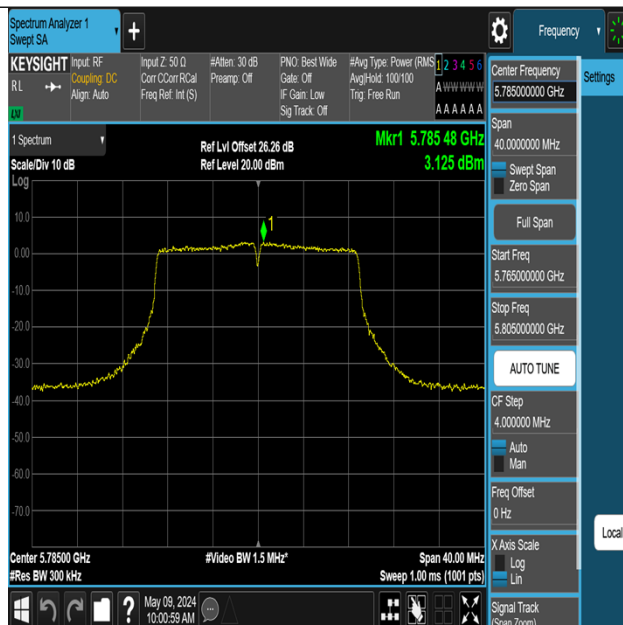
11N20MIMO-Ant3-5785-PASS
