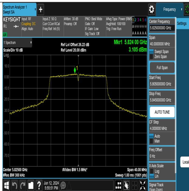
11A-Ant2-5825-PASS
