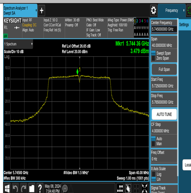
11N20MIMO-Ant3-5745-PASS
