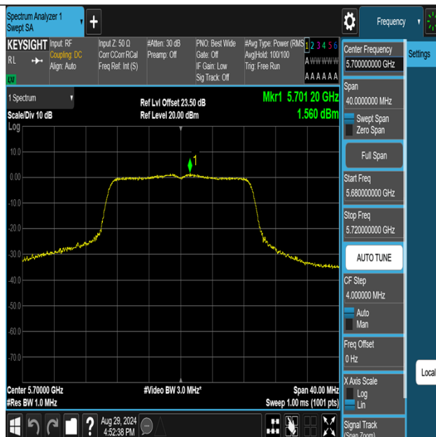
11N20MIMO-Ant1-5700-PASS
