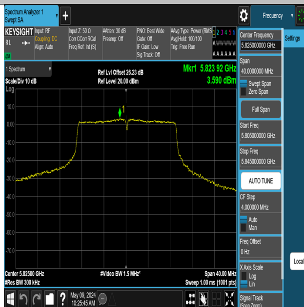
11N20MIMO-Ant3-5825-PASS
