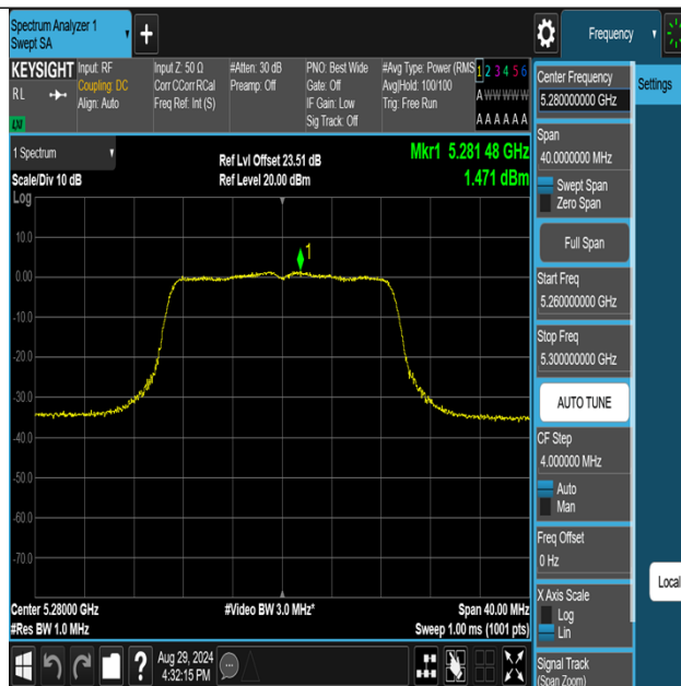
11N20MIMO-Ant1-5280-PASS
