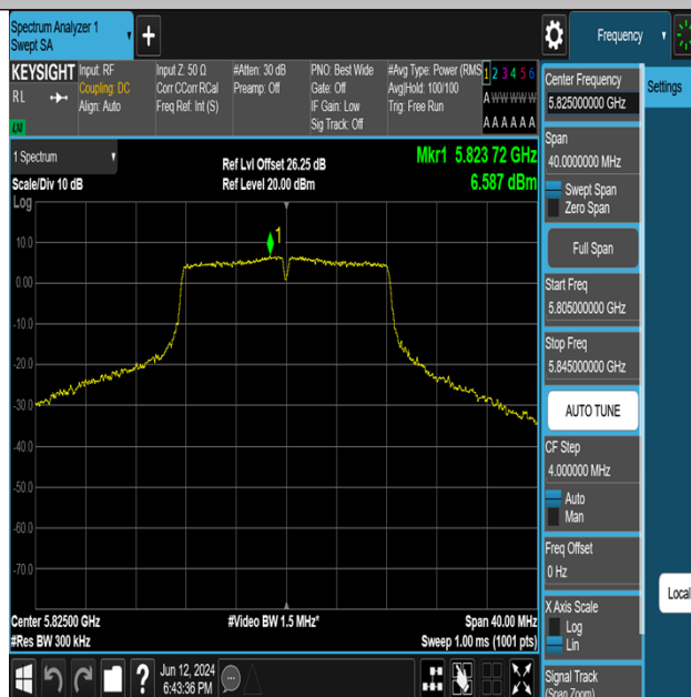
11A-Ant3-5825-PASS
