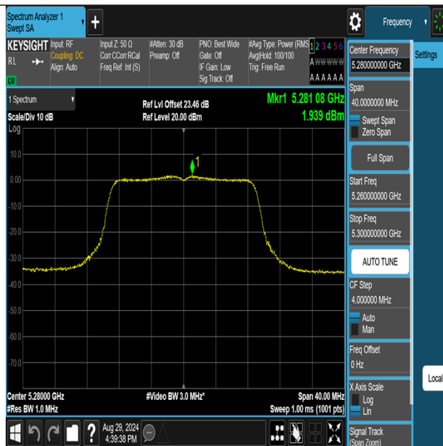
11N20MIMO-Ant3-5280-PASS
