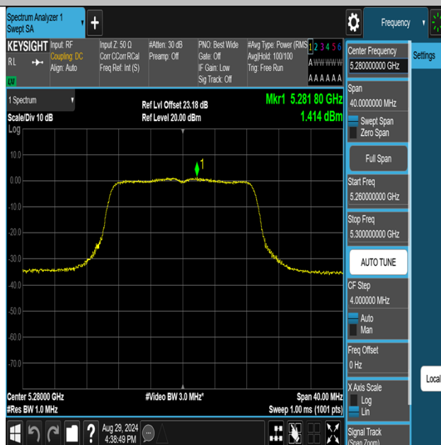
11N20MIMO-Ant2-5280-PASS
