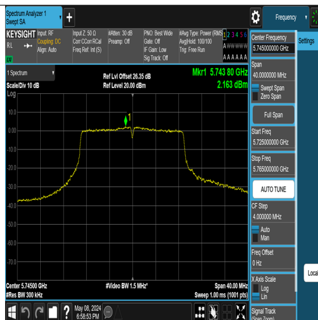
11N20MIMO-Ant2-5745-PASS
