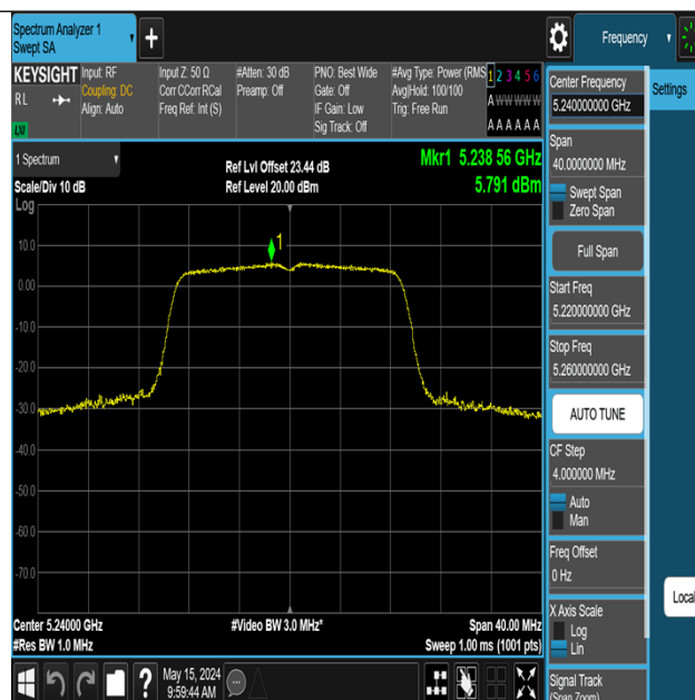
11N20MIMO-Ant3-5240-PASS
