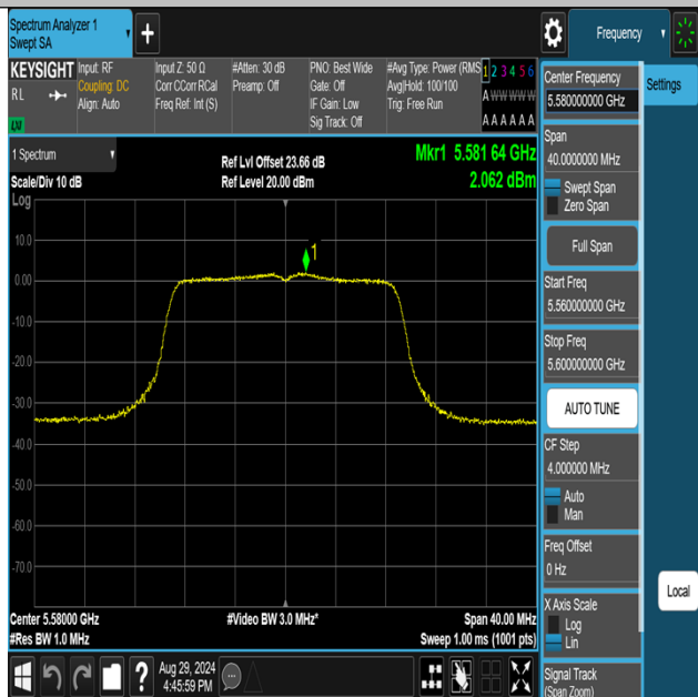
11N20MIMO-Ant1-5580-PASS
