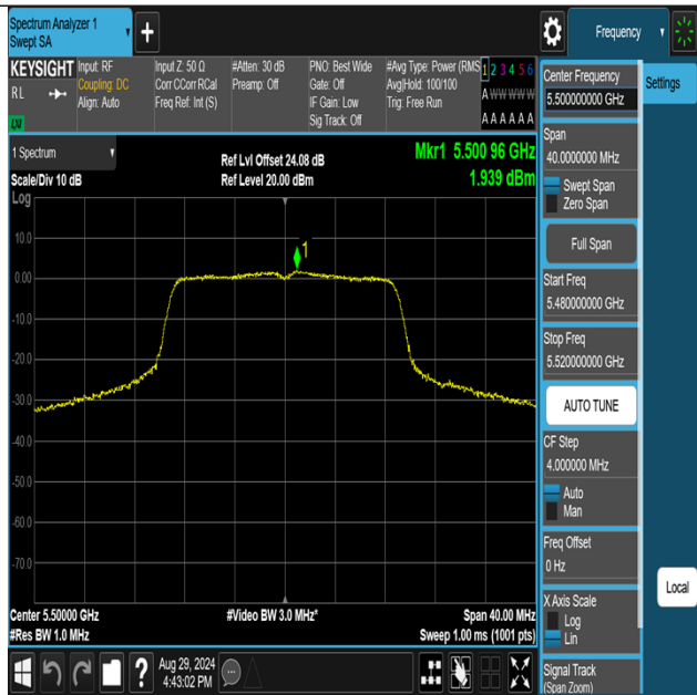
11N20MIMO-Ant1-5500-PASS
