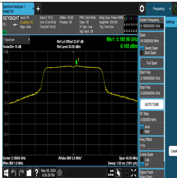
11N20MIMO-Ant3-5180-PASS
