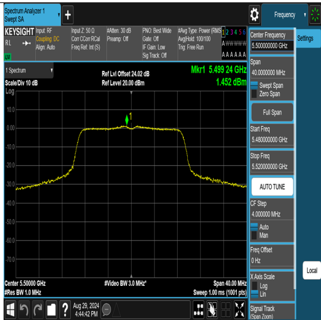
11N20MIMO-Ant3-5500-PASS
