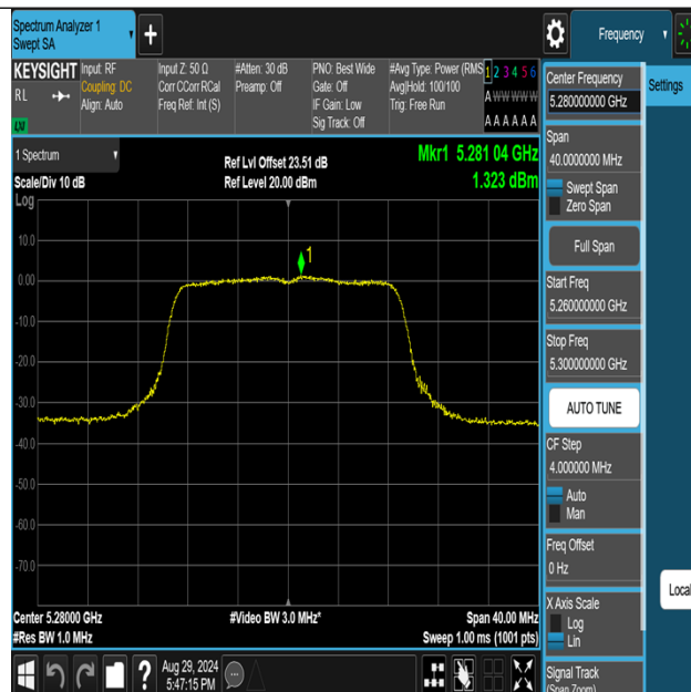
11AC20MIMO-Ant2-5280-PASS
