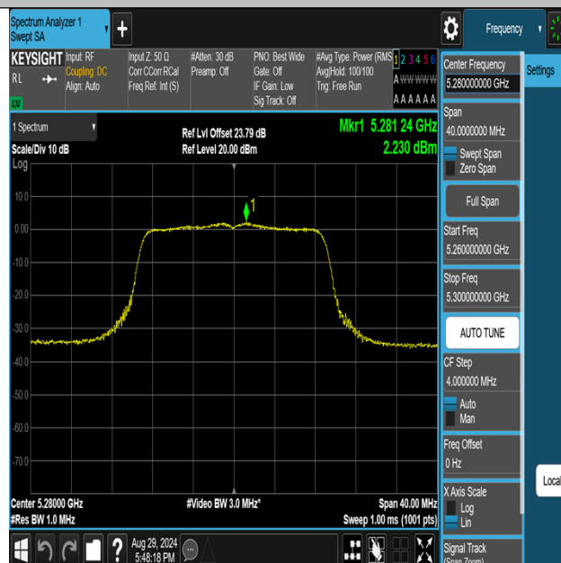
11AC20MIMO-Ant3-5280-PASS
