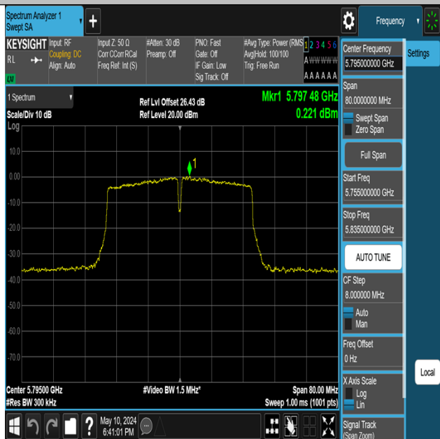
11N40MIMO-Ant2-5795-PASS
