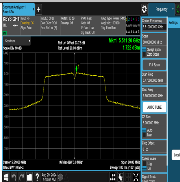
11N40MIMO-Ant2-5510-PASS
