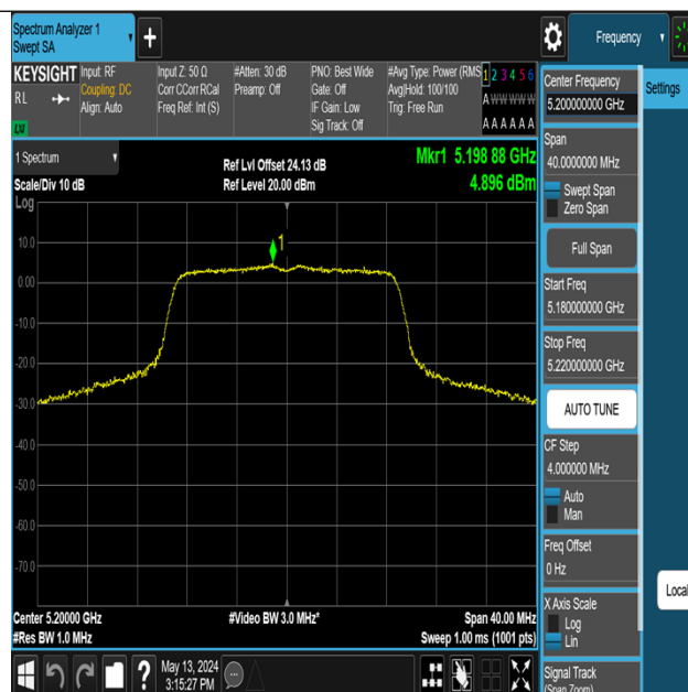
11AC20MIMO-Ant1-5200-PASS
