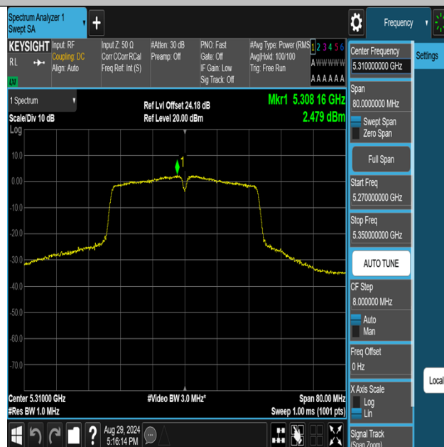
11N40MIMO-Ant3-5310-PASS
