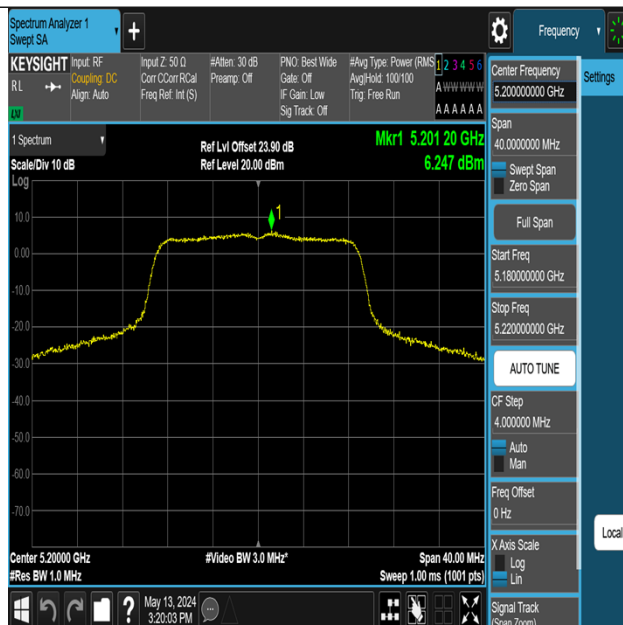
11AC20MIMO-Ant3-5200-PASS
