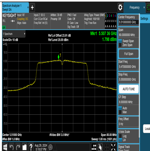
11N40MIMO-Ant1-5510-PASS
