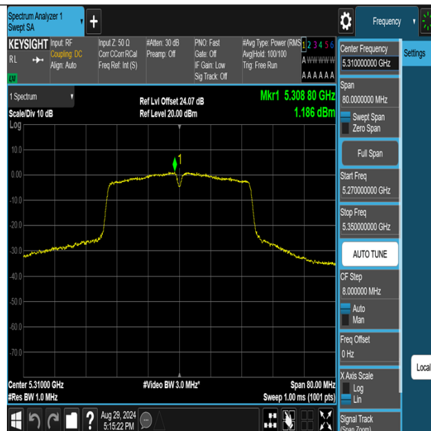
11N40MIMO-Ant2-5310-PASS
