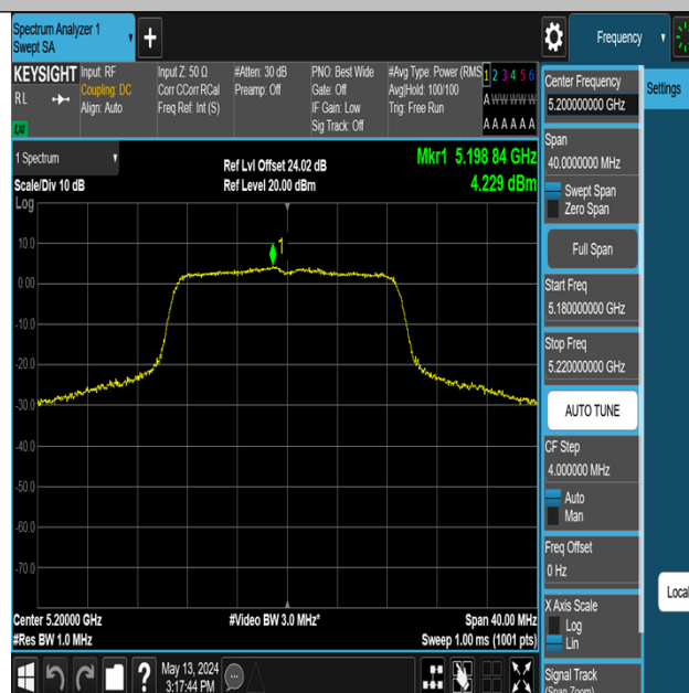
11AC20MIMO-Ant2-5200-PASS
