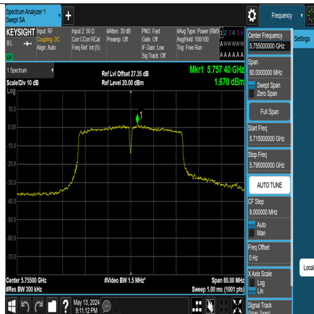
11AC40MIMO-Ant3-5755-PASS
