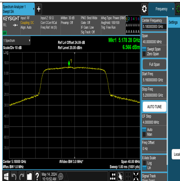
11AX20MIMO-Ant3-5180-PASS
