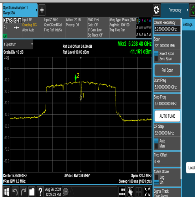
11AC160MIMO-Ant3-5250_UNII-1-PASS
