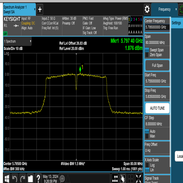
11AC40MIMO-Ant3-5795-PASS
