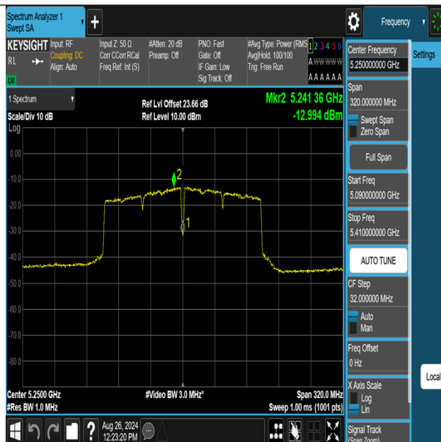
11AC160MIMO-Ant2-5250_UNII-1-PASS
