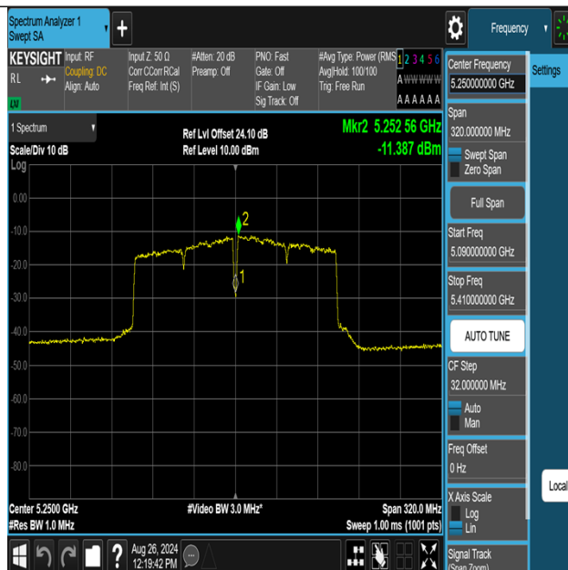
11AC160MIMO-Ant1-5250_UNII-2A-PASS
