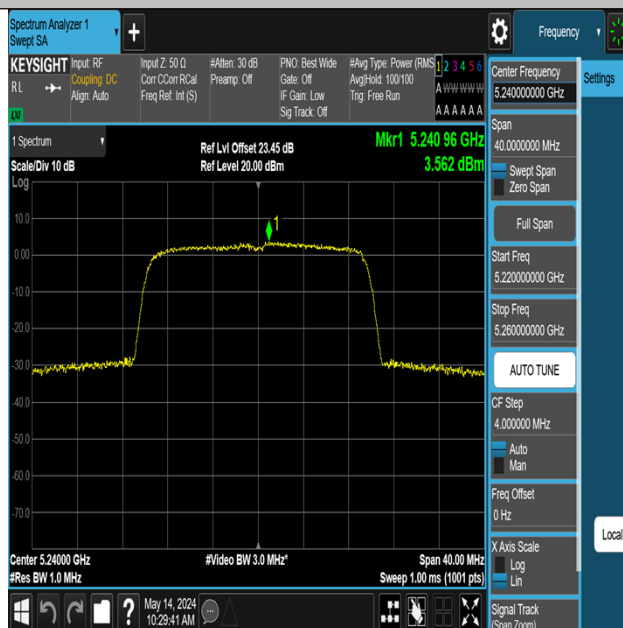
11AX20MIMO-Ant2-5240-PASS
