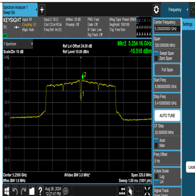
11AC160MIMO-Ant3-5250_UNII-2A-PASS
