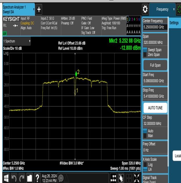
11AC160MIMO-Ant2-5250_UNII-2A-PASS
