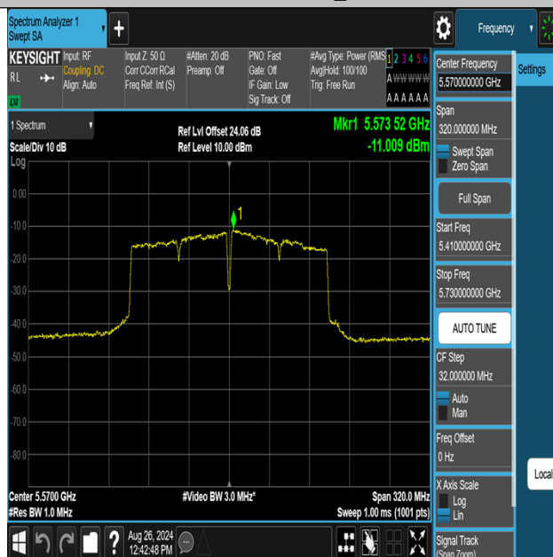
11AC160MIMO-Ant1-5570-PASS
