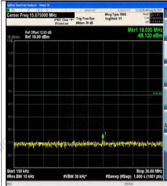
Band2-10MHz-16QAM-19150-1RB#49-0.15~30-P ASS
