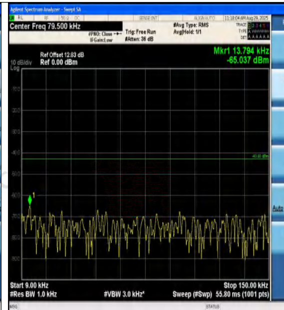
Band2-10MHz-16QAM-18650-1RB#49-0.009~0.15 -PASS
