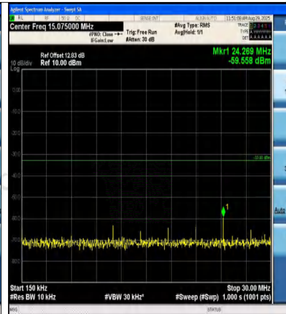
Band2-5MHz-16QAM-19175-1RB#24-0.15~30-PA SS
