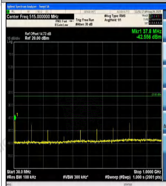
Band2-5MHz-16QAM-19175-1RB#24-30~1000-P ASS
