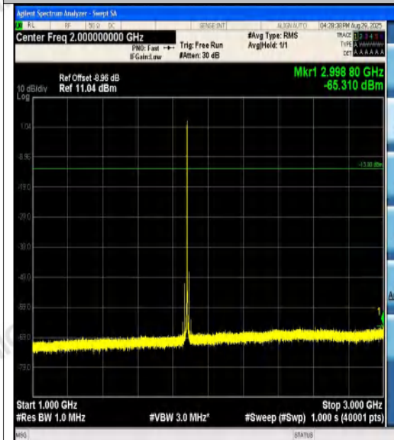
Band2-1.4MHz-QPSK-18900-1RB#0-1000~3000- PASS
