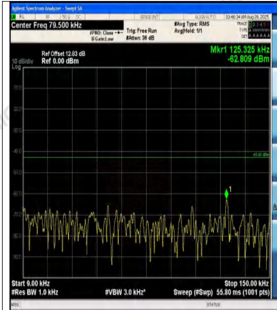
Band2-1.4MHz-16QAM-19193-1RB#0-0.009~0.1 5-PASS
