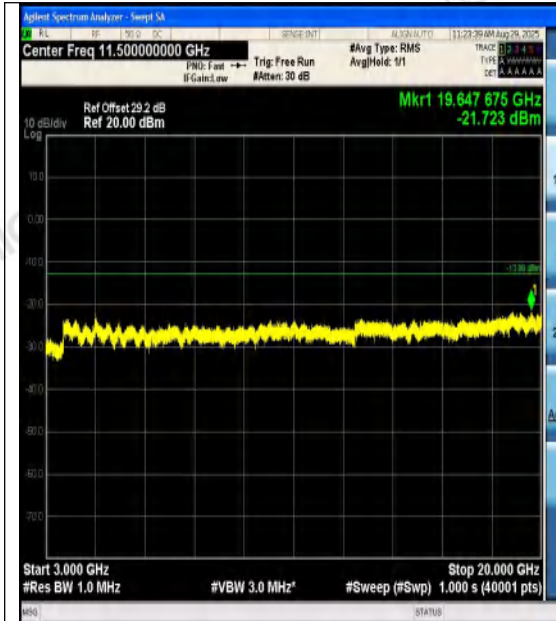
Band2-10MHz-QPSK-19150-1RB#49-3000~2000 0-PASS
