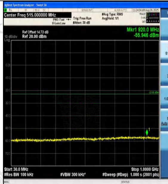
Band2-10MHz-16QAM-19150-1RB#49-30~1000-P ASS
