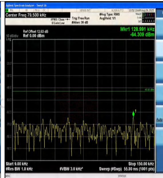
Band2-3MHz-16QAM-18615-1RB#14-0.009~0.15- PASS
