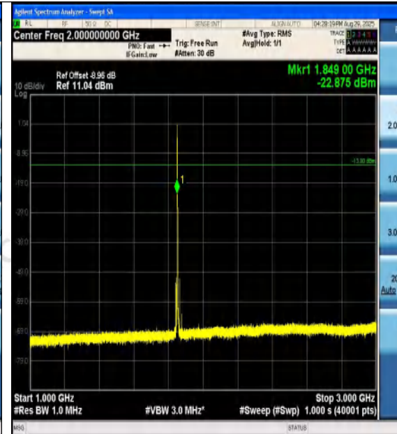
Band2-1.4MHz-16QAM-18607-6RB#0-1000~3000- PASS
