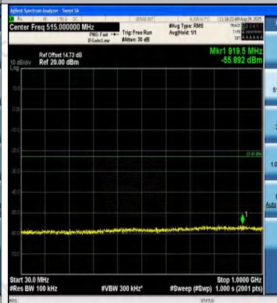
Band2-10MHz-16QAM-18650-1RB#49-30~1000-P ASS
