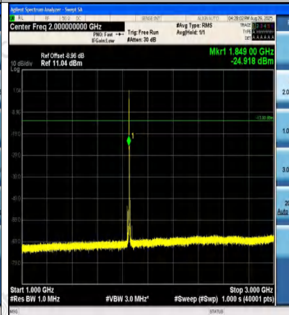
Band2-1.4MHz-QPSK-18607-6RB#0-1000~3000-P
