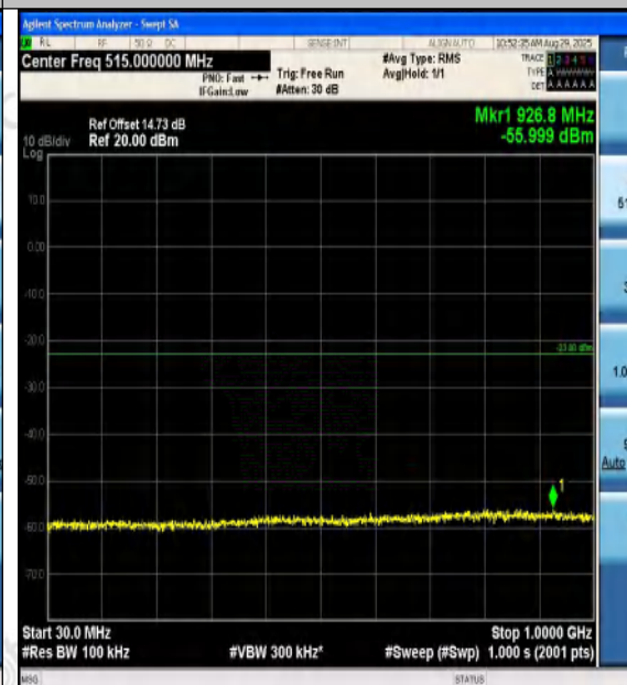
Band2-3MHz-16QAM-18615-1RB#14-30~1000-PA SS
