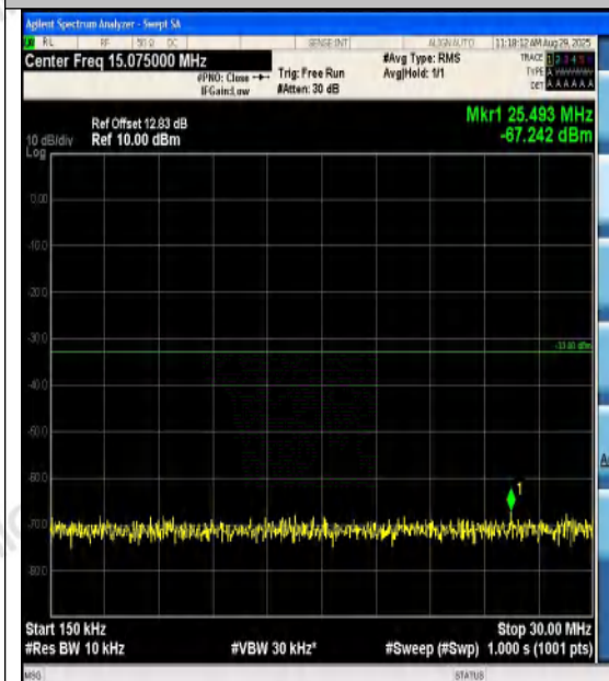
Band2-10MHz-16QAM-18650-1RB#49-0.15~30-P ASS
