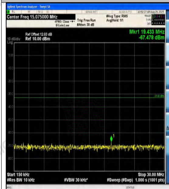
Band2-3MHz-16QAM-18615-1RB#14-0.15~30-PA SS
