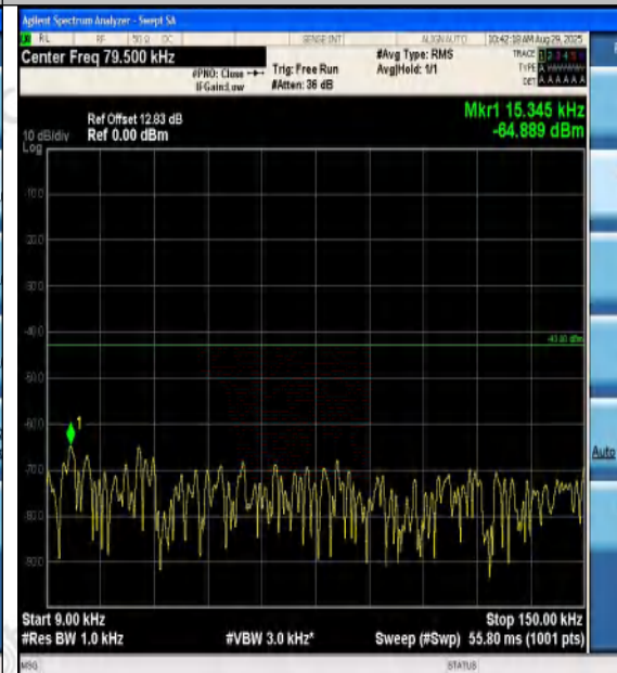
Band2-1.4MHz-16QAM-18900-1RB#0-0.009~0.15- PASS
