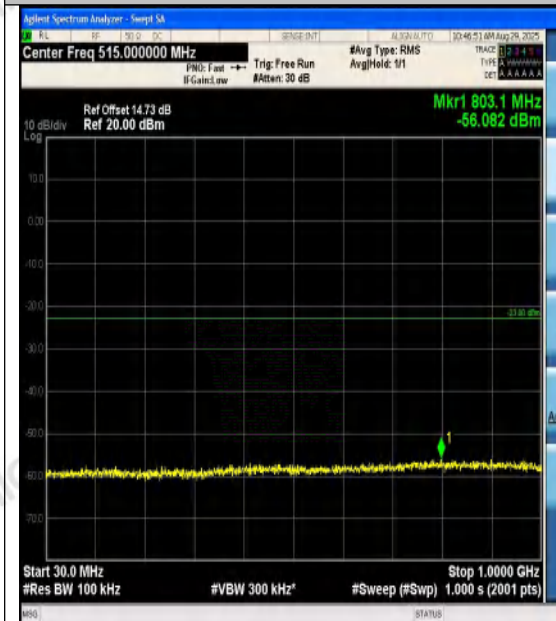
Band2-1.4MHz-16QAM-19193-1RB#0-30~1000-P ASS
