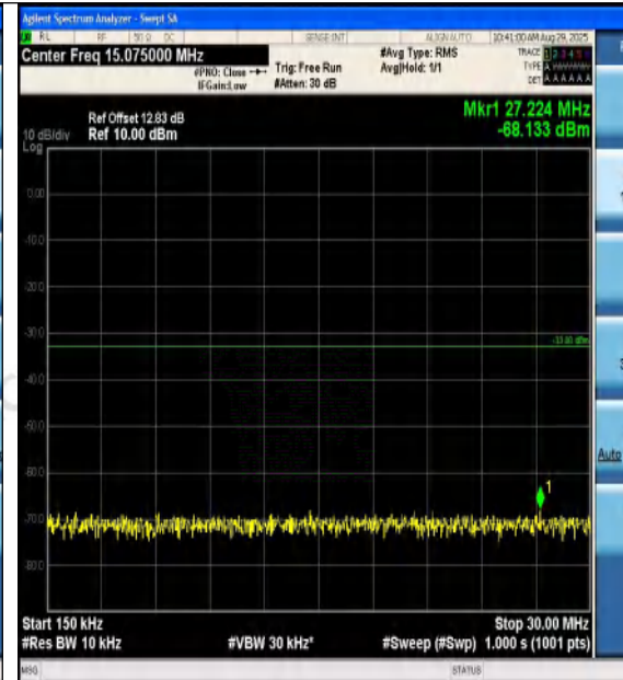
Band2-1.4MHz-16QAM-18607-6RB#0-0.15~30-PA
