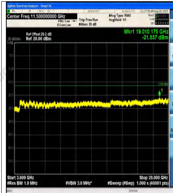
Band2-10MHz-QPSK-18650-1RB#49-3000~2000 0-PASS
