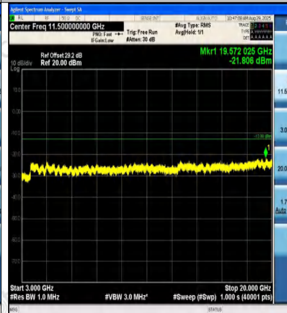
Band2-1.4MHz-16QAM-19193-1RB#0-3000~2000 0-PASS
