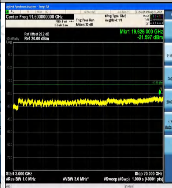
Band2-5MHz-16QAM-19175-1RB#24-3000~20000 -PASS
