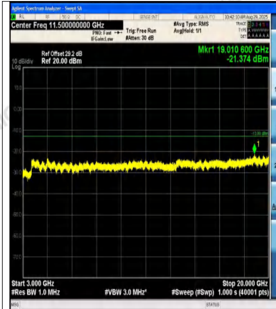
Band2-1.4MHz-QPSK-18900-1RB#0-3000~20000 -PASS
