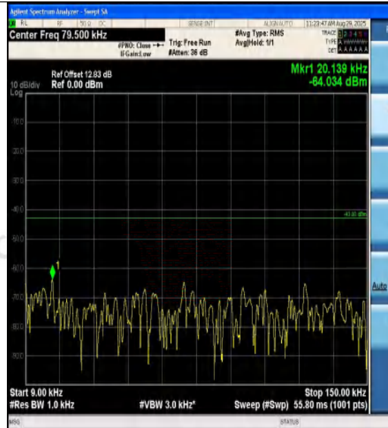
Band2-10MHz-16QAM-19150-1RB#49-0.009~0.15 -PASS
