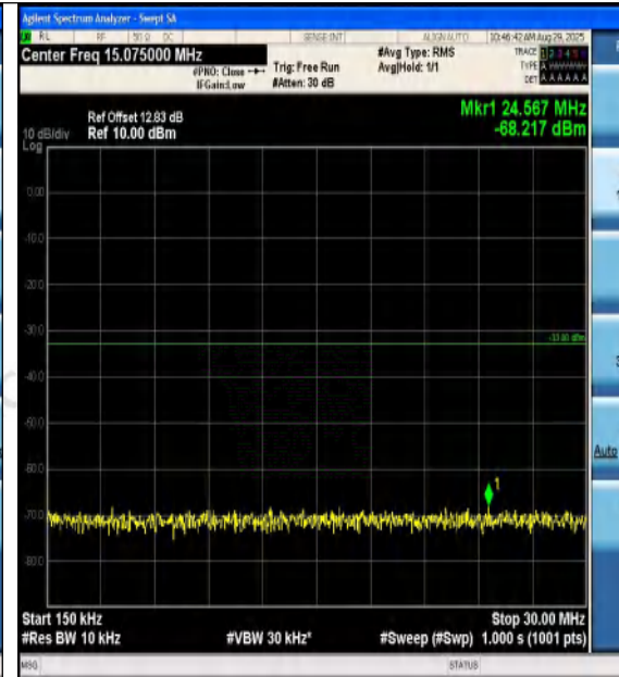
Band2-1.4MHz-16QAM-19193-1RB#0-0.15~30-PA SS
