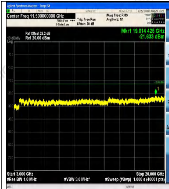
Band2-3MHz-QPSK-18615-1RB#14-3000~20000 -PASS
