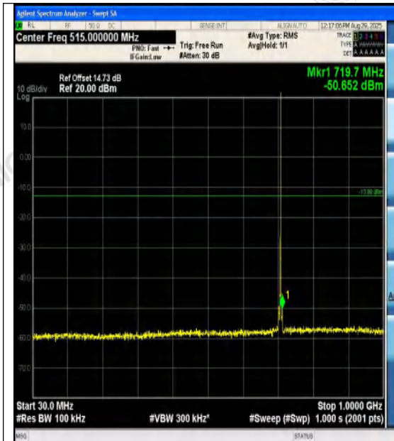
Band12-1.4MHz-QPSK-23173-1RB#0-30~1000-P ASS
