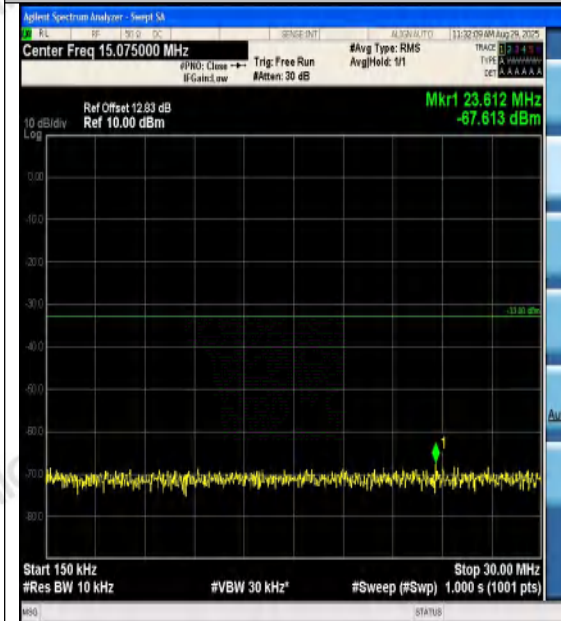
Band2-15MHz-16QAM-18900-1RB#74-0.15~30-P ASS
