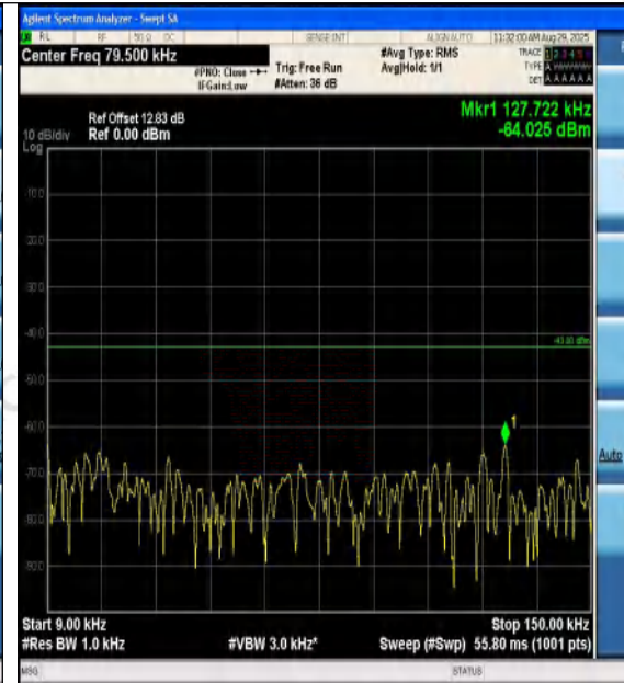
Band2-15MHz-16QAM-18900-1RB#74-0.009~0.15 -PASS
