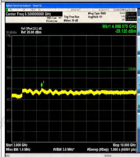
Band12-1.4MHz-QPSK-23017-6RB#0-3000~1000 0-PASS
