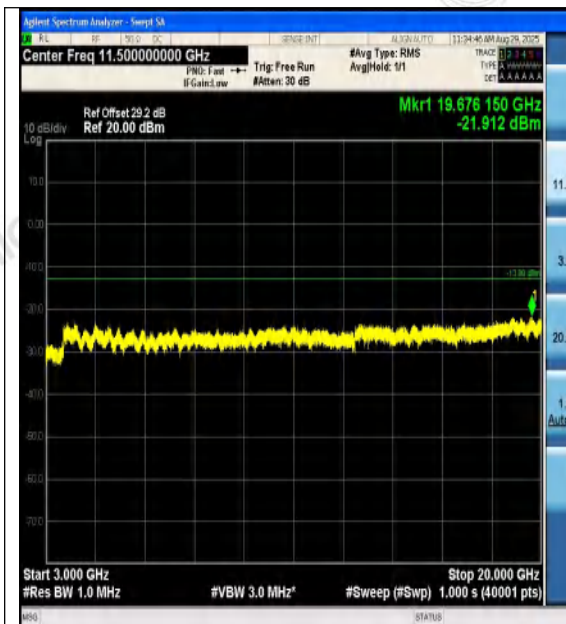
Band2-15MHz-QPSK-19125-1RB#74-3000~2000 0-PASS
