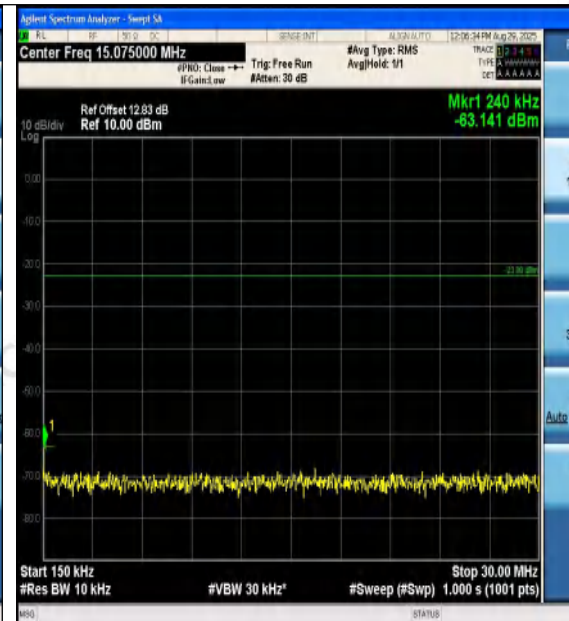
Band12-1.4MHz-QPSK-23017-1RB#5-0.15~30-PA SS
