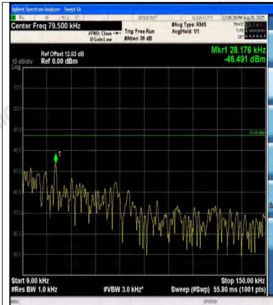
Band12-1.4MHz-QPSK-23017-1RB#5-0.009~0.15 -PASS
