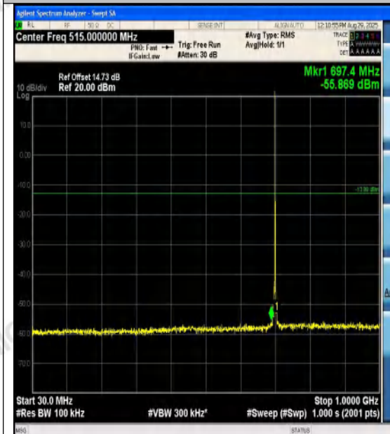
Band12-1.4MHz-QPSK-23095-1RB#0-30~1000-P ASS
