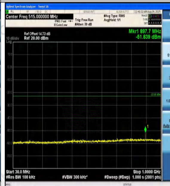
Band2-20MHz-16QAM-18700-1RB#99-30~1000-P ASS
