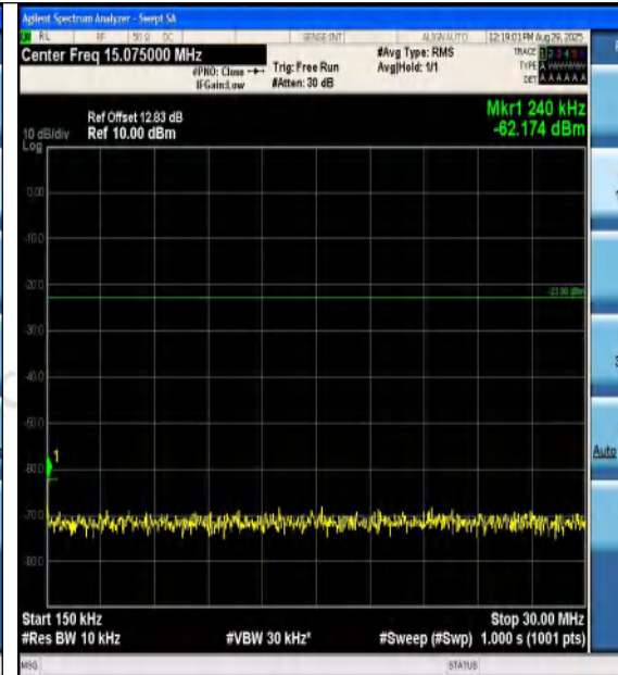
Band12-1.4MHz-QPSK-23173-1RB#5-0.15~30-PA SS
