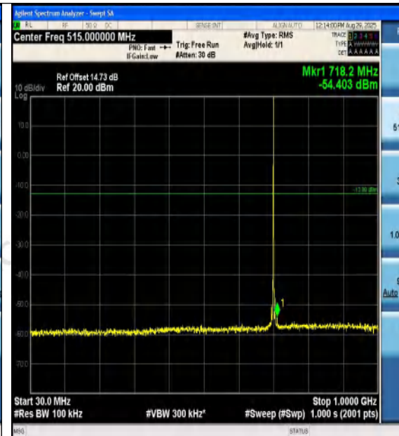
Band12-1.4MHz-16QAM-23095-1RB#5-30~1000-P ASS
