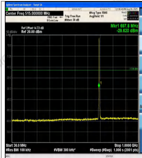
Band12-1.4MHz-QPSK-23017-6RB#0-30~1000-P ASS
