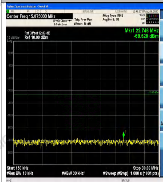
Band2-20MHz-QPSK-19100-100RB#0-0.15~30-P ASS
