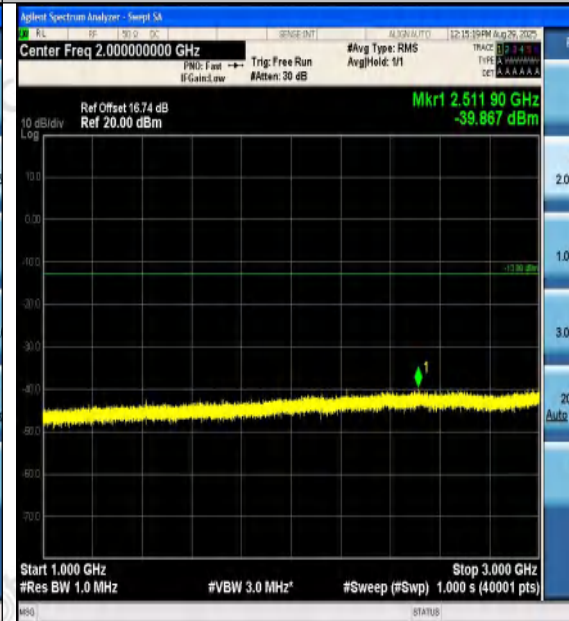
Band12-1.4MHz-QPSK-23095-6RB#0-1000~3000- PASS
