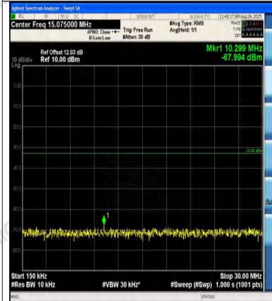
Band2-20MHz-16QAM-18900-1RB#99-0.15~30-P ASS
