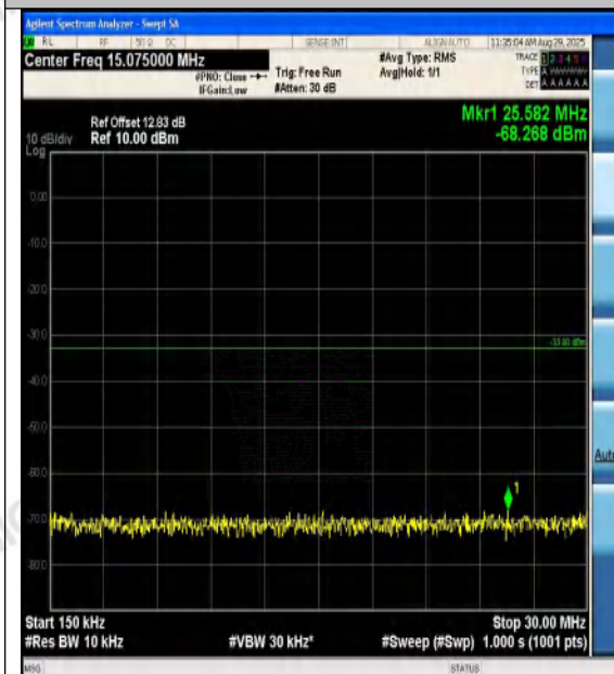
Band2-15MHz-16QAM-19125-1RB#74-0.15~30-P ASS
