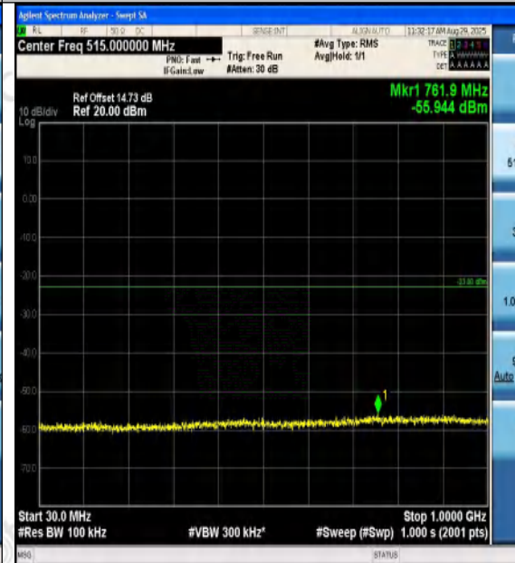
Band2-15MHz-16QAM-18900-1RB#74-30~1000-P ASS
