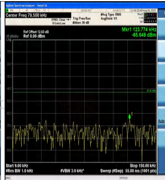
Band2-20MHz-16QAM-18700-1RB#99-0.009~0.15 -PASS
