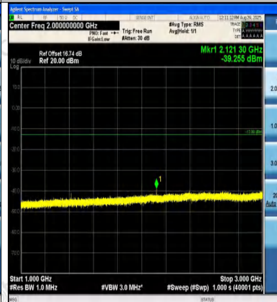
Band12-1.4MHz-QPSK-23095-1RB#0-1000~3000- PASS
