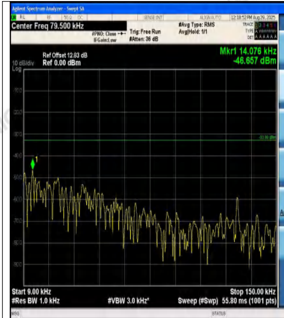
Band12-1.4MHz-QPSK-23173-1RB#5-0.009~0.15 -PASS
