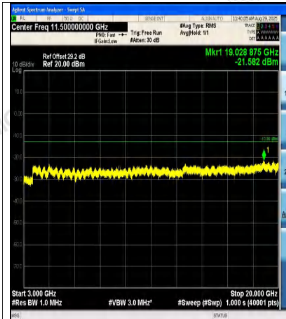
Band2-20MHz-QPSK-18700-1RB#99-3000~2000 0-PASS
