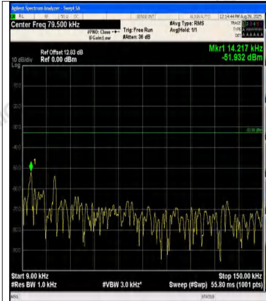
Band12-1.4MHz-QPSK-23095-6RB#0-0.009~0.15 -PASS
