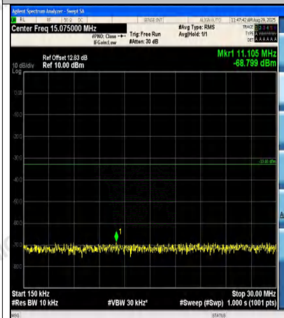
Band2-20MHz-QPSK-18900-100RB#0-0.15~30-P ASS
