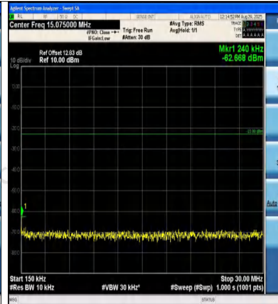
Band12-1.4MHz-QPSK-23095-6RB#0-0.15~30-PA SS
