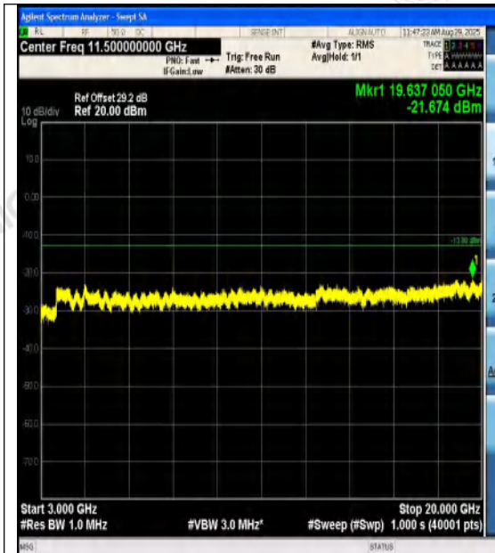
Band2-20MHz-QPSK-18700-100RB#0-3000~200 00-PASS
