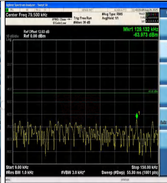
Band2-20MHz-16QAM-18900-1RB#99-0.009~0.15 -PASS
