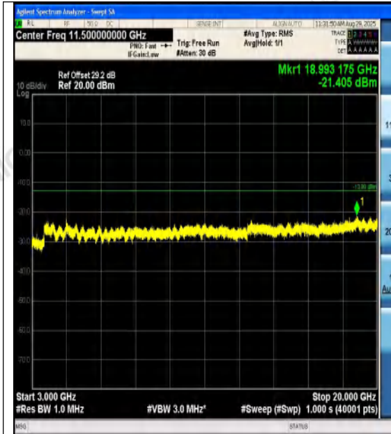
Band2-15MHz-QPSK-18900-1RB#74-3000~2000 0-PASS
