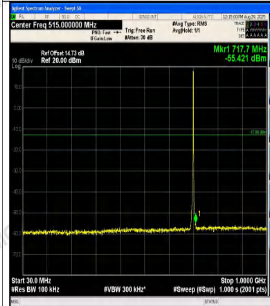
Band12-1.4MHz-QPSK-23095-6RB#0-30~1000-P ASS
