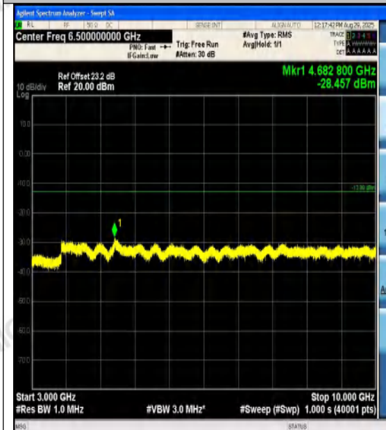
Band12-1.4MHz-QPSK-23173-1RB#0-3000~1000 0-PASS
