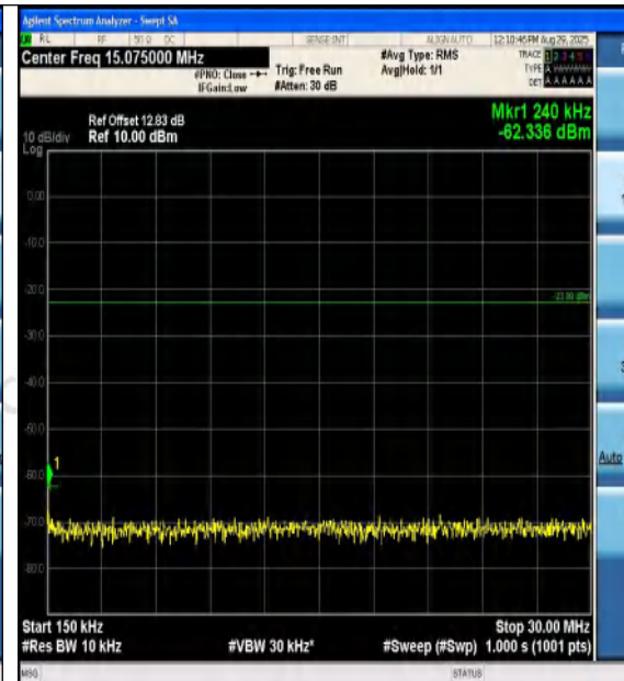
Band12-1.4MHz-QPSK-23095-1RB#0-0.15~30-PA SS
