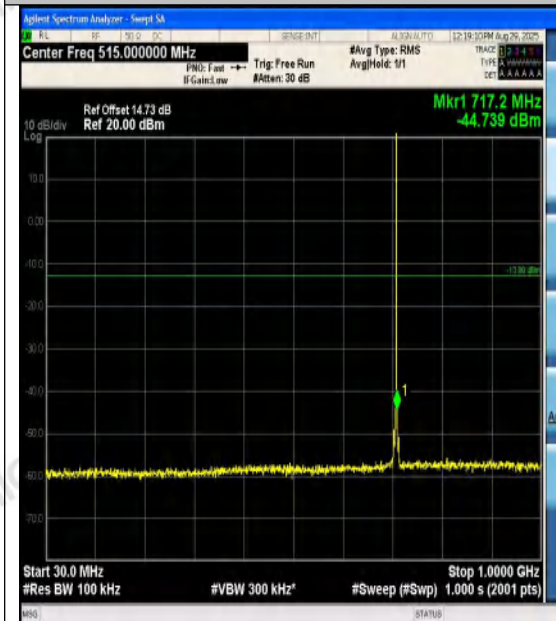
Band12-1.4MHz-QPSK-23173-1RB#5-30~1000-P ASS
