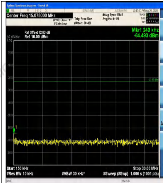
Band12-1.4MHz-16QAM-23095-1RB#5-0.15~30- PASS
