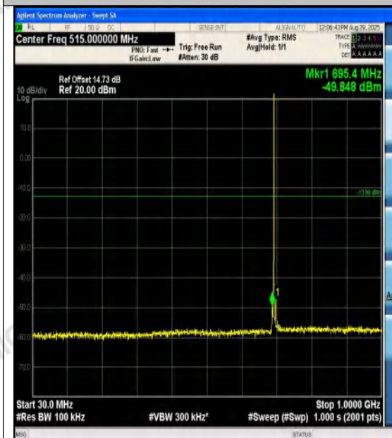
Band12-1.4MHz-QPSK-23017-1RB#5-30~1000-P ASS
