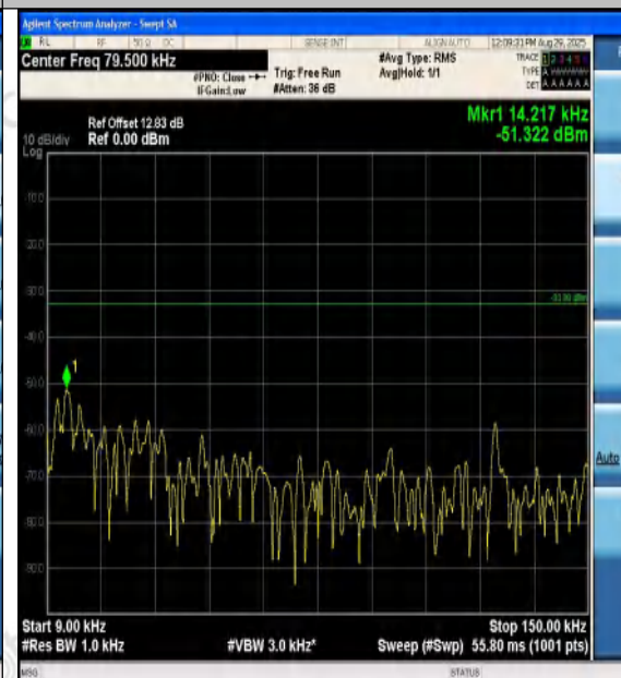
Band12-1.4MHz-16QAM-23017-6RB#0-0.009~0.1 5-PASS
