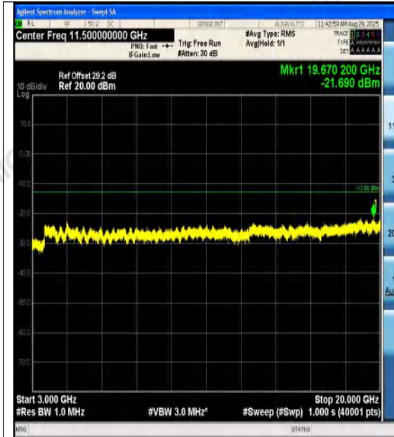
Band2-20MHz-QPSK-18900-1RB#99-3000~2000 0-PASS
