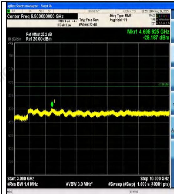
Band12-5MHz-QPSK-23095-25RB#0-3000~1000 0-PASS
