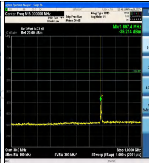
Band12-5MHz-16QAM-23035-1RB#0-30~1000-PA
