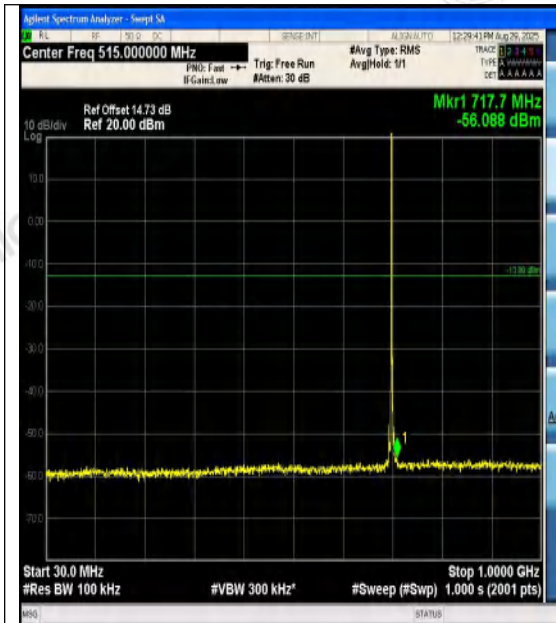
Band12-3MHz-QPSK-23095-1RB#0-30~1000-PA
