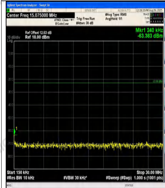
Band12-3MHz-16QAM-23025-15RB#0-0.15~30-P ASS
