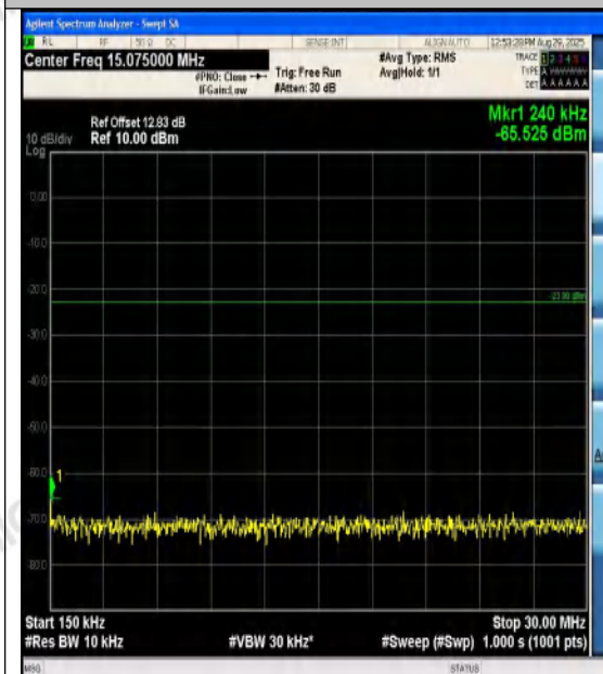
Band12-5MHz-16QAM-23095-25RB#0-0.15~30-P ASS
