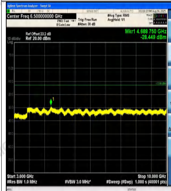
Band12-10MHz-QPSK-23060-1RB#49-3000~10000-PASS
