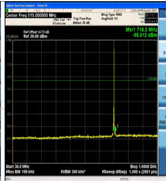
Band12-5MHz-16QAM-23095-1RB#24-30~1000-P
