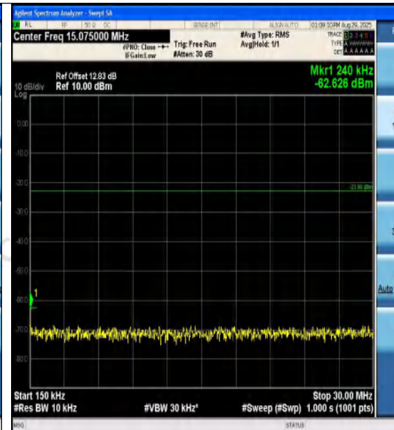
Band12-10MHz-QPSK-23130-1RB#0-0.15~30-PA SS
