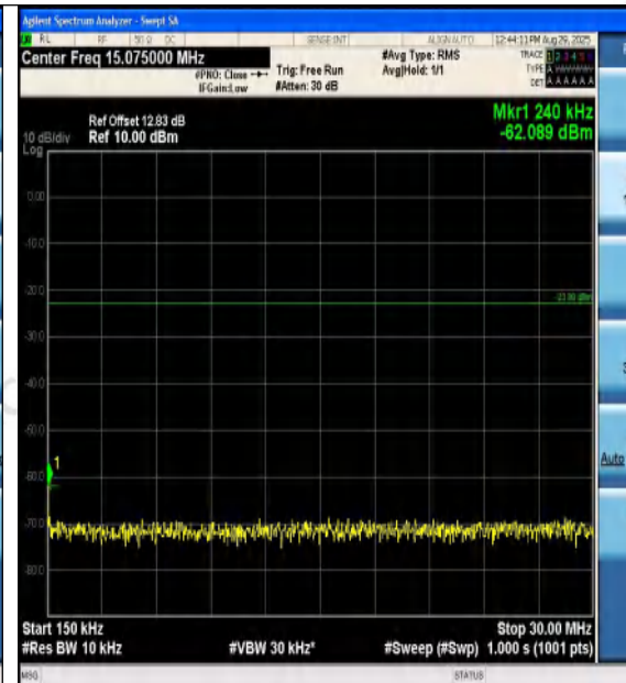
Band12-5MHz-QPSK-23035-1RB#24-0.15~30-PA SS
