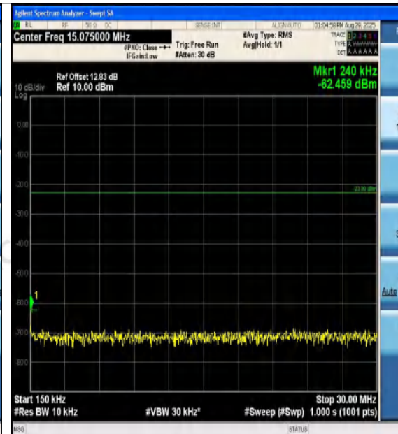
Band12-10MHz-QPSK-23095-1RB#0-0.15~30-PA SS
