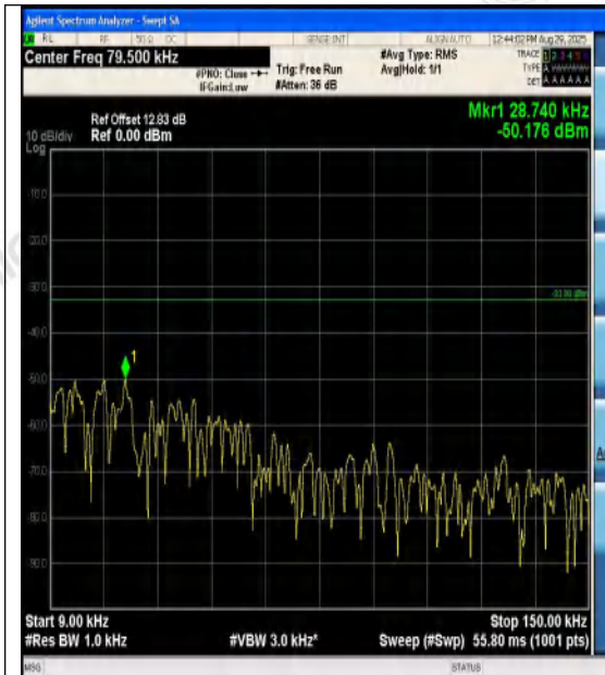
Band12-5MHz-QPSK-23035-1RB#24-0.009~0.15 -PASS
