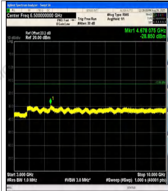
Band12-3MHz-QPSK-23025-15RB#0-3000~1000 0-PASS
