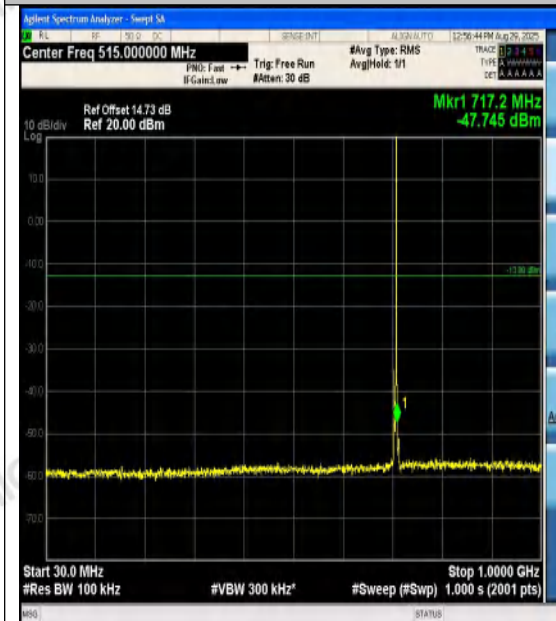
Band12-5MHz-QPSK-23155-1RB#24-30~1000-P ASS
