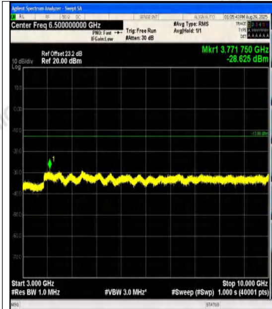
Band12-10MHz-QPSK-23095-1RB#0-3000~1000 0-PASS
