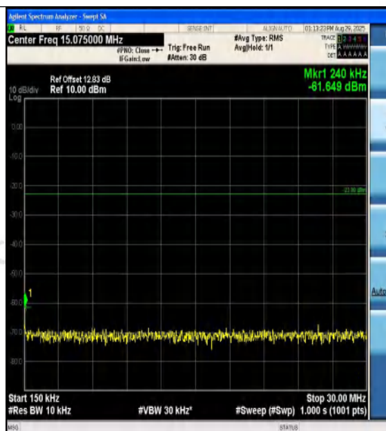
Band12-10MHz-QPSK-23060-50RB#0-0.15~30-PA SS
