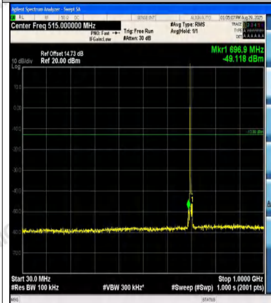
Band12-10MHz-QPSK-23095-1RB#0-30~1000-P ASS
