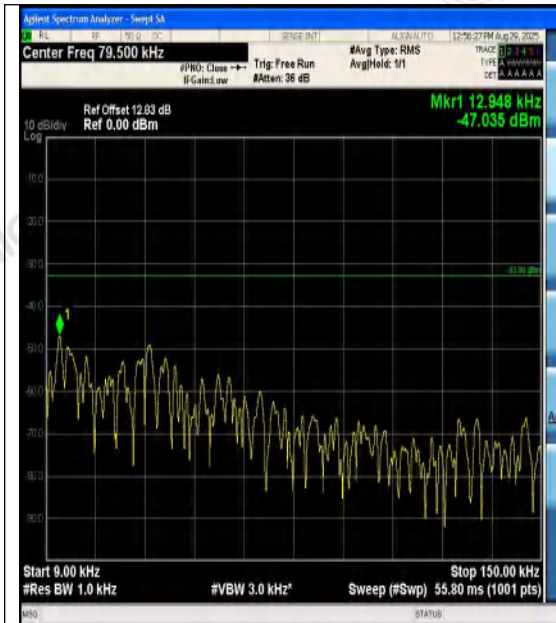
Band12-5MHz-QPSK-23155-1RB#24-0.009~0.15 -PASS
