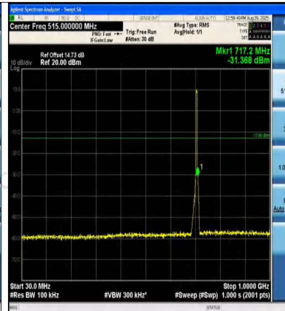
Band12-5MHz-16QAM-23155-25RB#0-30~1000-P ASS
