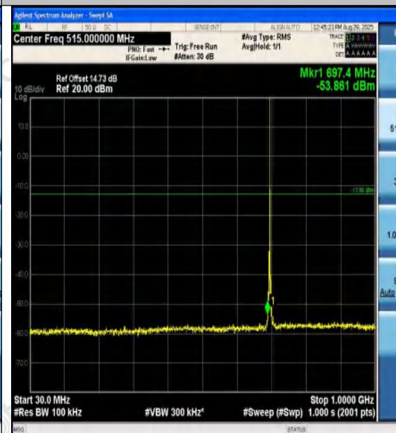
Band12-5MHz-16QAM-23035-1RB#24-30~1000-P ASS
