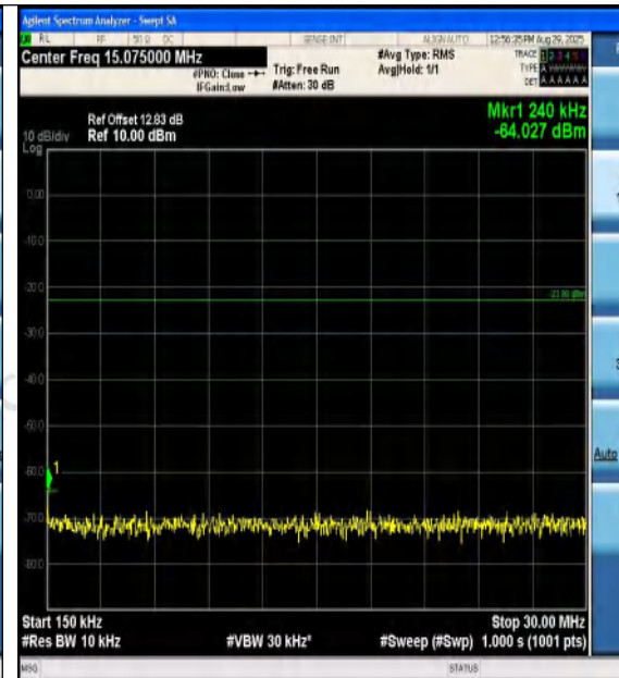
Band12-5MHz-QPSK-23155-1RB#24-0.15~30-PA SS
