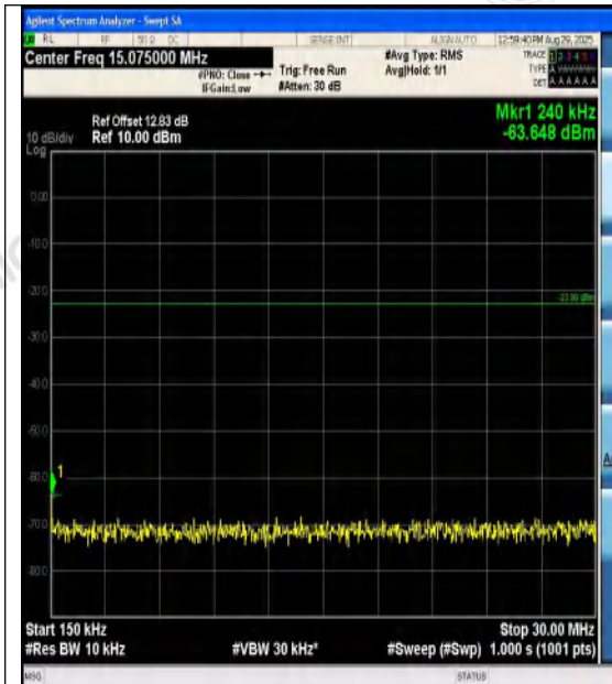
Band12-5MHz-16QAM-23155-25RB#0-0.15~30-P ASS
