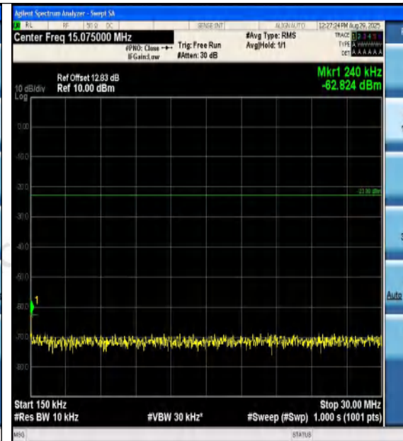
Band12-3MHz-QPSK-23025-15RB#0-0.15~30-PA SS
