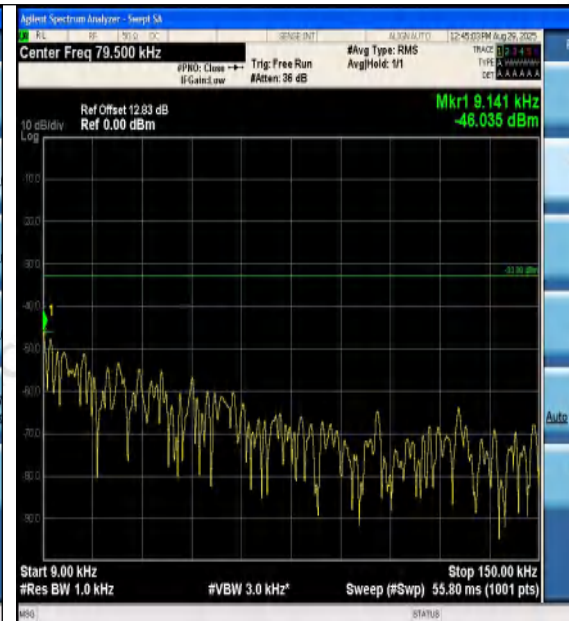
Band12-5MHz-16QAM-23035-1RB#24-0.009~0.15 -PASS
