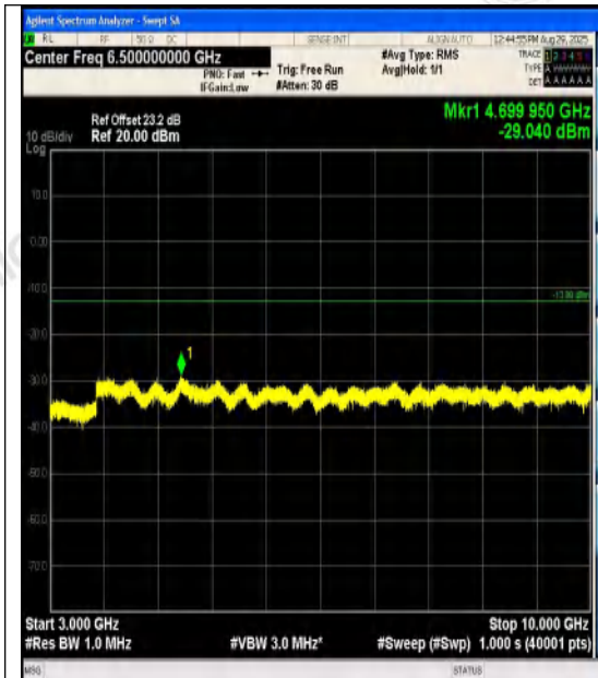
Band12-5MHz-QPSK-23035-1RB#24-3000~1000 0-PASS
