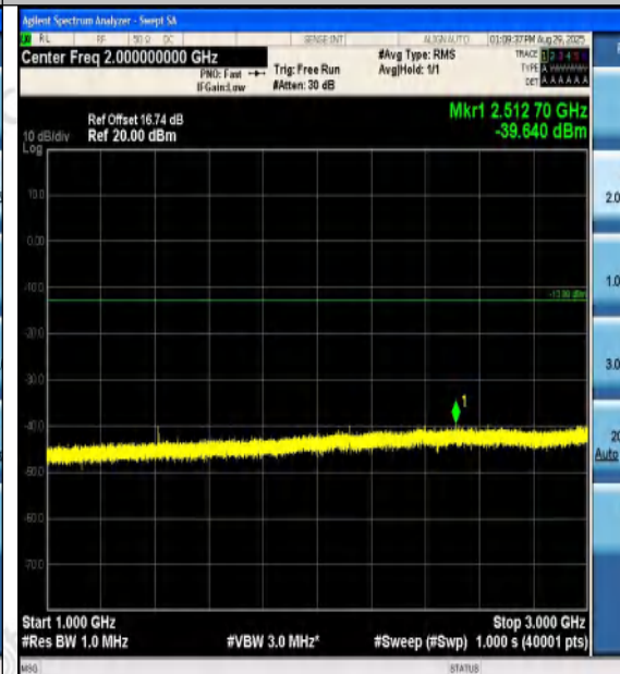
Band12-10MHz-QPSK-23130-1RB#0-1000~3000- PASS
