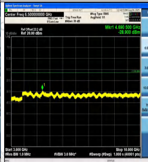
Band12-5MHz-16QAM-23035-1RB#0-3000~10000
