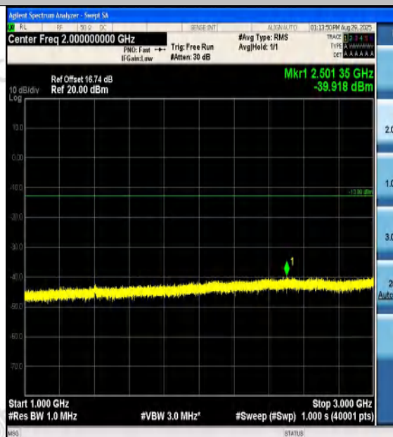
Band12-10MHz-QPSK-23060-50RB#0-1000~3000 -PASS
