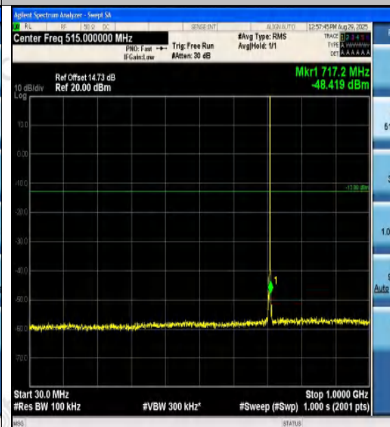
Band12-5MHz-16QAM-23155-1RB#24-30~1000-P ASS
