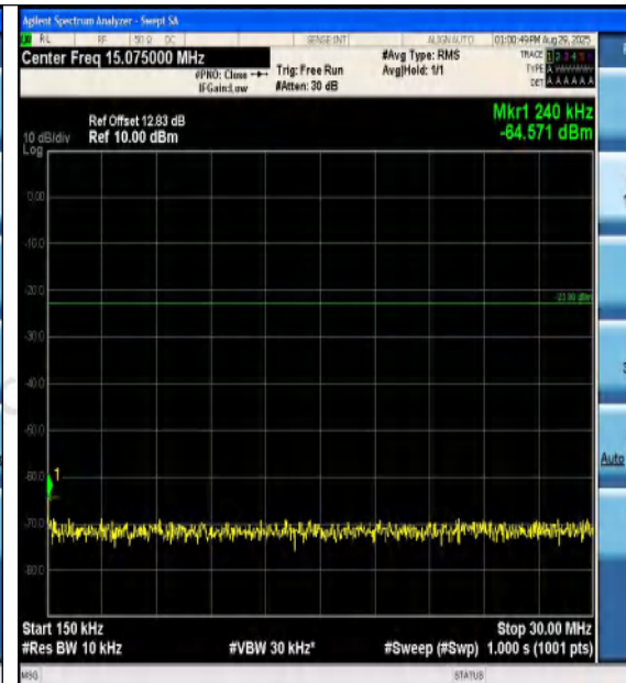
Band12-10MHz-QPSK-23060-1RB#0-0.15~30-PA SS
