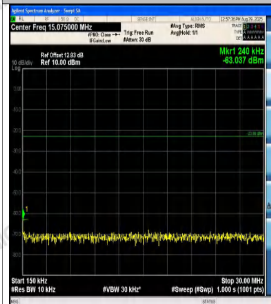
Band12-5MHz-16QAM-23155-1RB#24-0.15~30-P ASS
