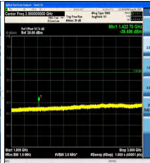
Band12-5MHz-QPSK-23155-1RB#0-1000~3000-P
