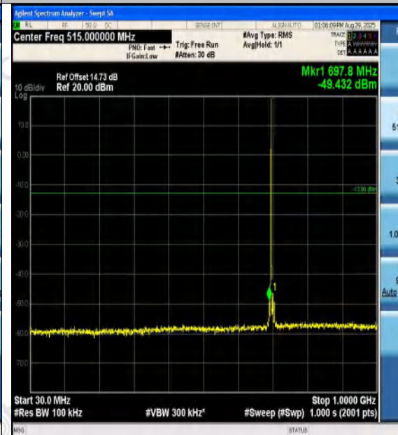
Band12-10MHz-16QAM-23095-1RB#0-30~1000-P ASS
