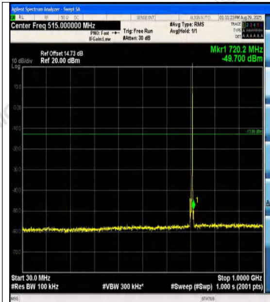
Band12-10MHz-QPSK-23130-1RB#49-30~1000- PASS
