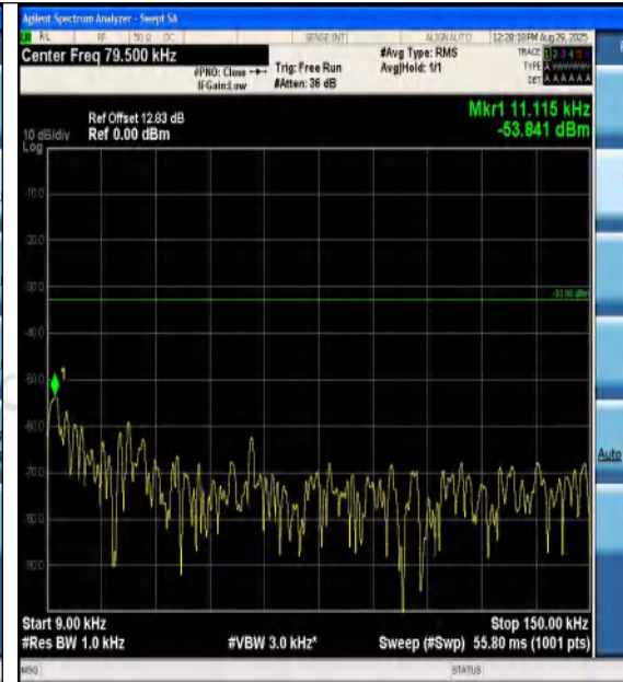
Band12-3MHz-16QAM-23025-15RB#0-0.009~0.15 -PASS
