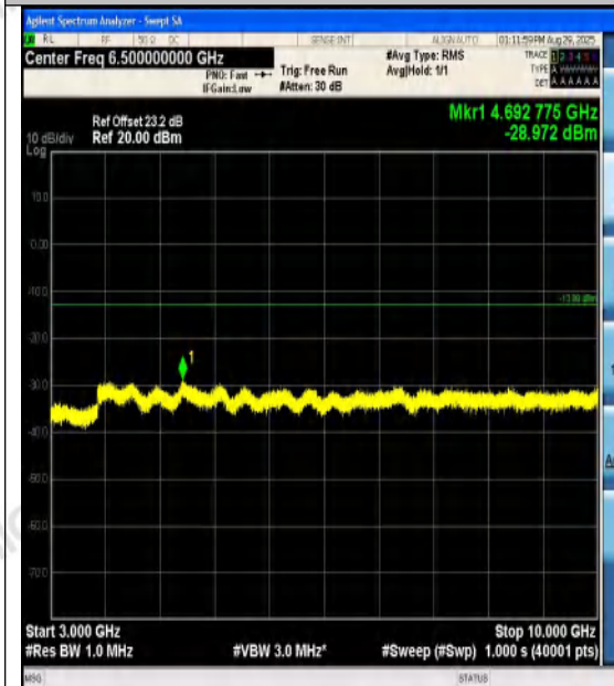
Band12-10MHz-QPSK-23130-1RB#49-3000~100 00-PASS
