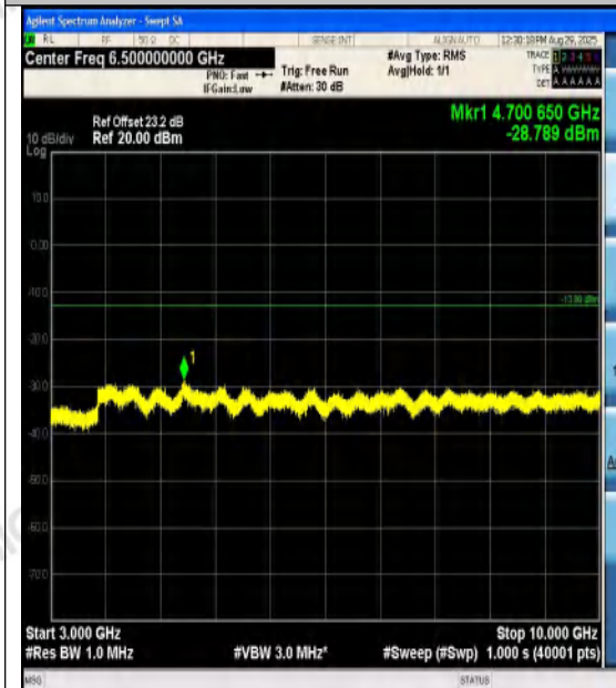
Band12-3MHz-QPSK-23095-1RB#0-3000~10000
