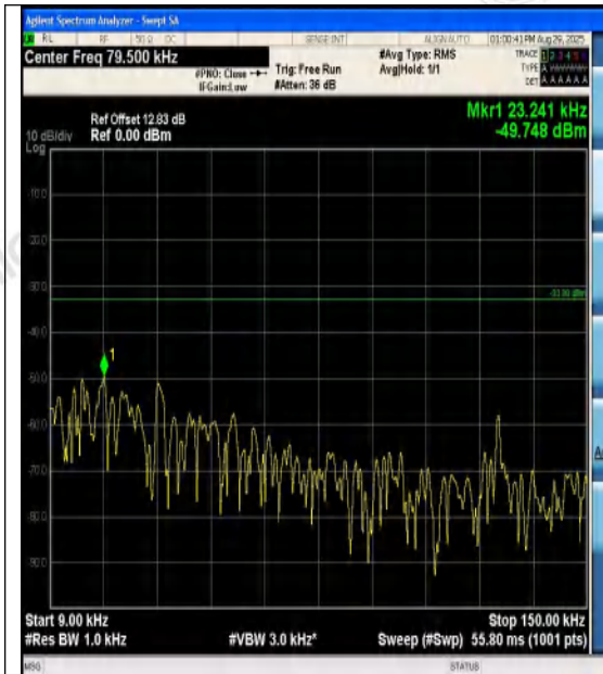
Band12-10MHz-QPSK-23060-1RB#0-0.009~0.15 -PASS
