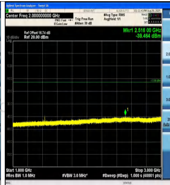
Band12-10MHz-QPSK-23130-1RB#49-1000~3000 -PASS
