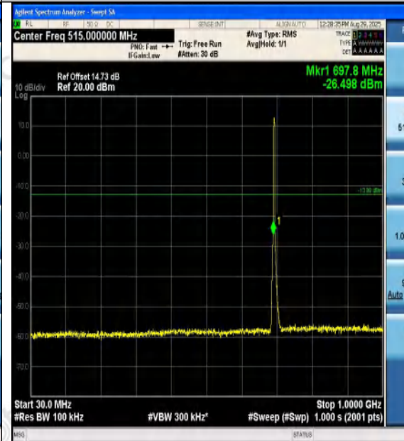
Band12-3MHz-16QAM-23025-15RB#0-30~1000-P ASS
