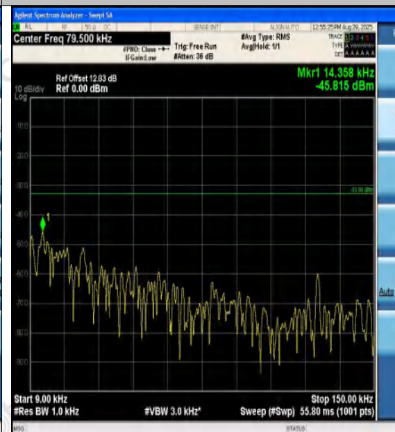
Band12-5MHz-16QAM-23155-1RB#0-0.009~0.15-
