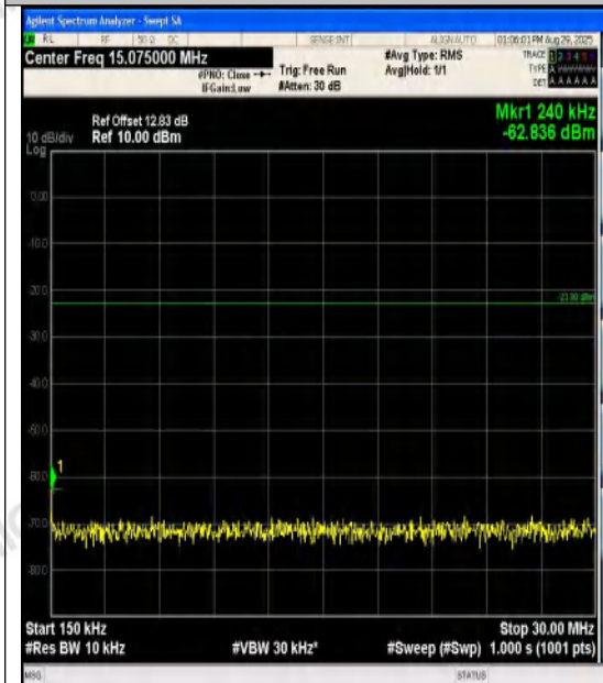
Band12-10MHz-16QAM-23095-1RB#0-0.15~30-P ASS
