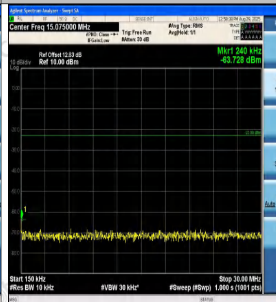
Band12-5MHz-QPSK-23155-25RB#0-0.15~30-PA SS
