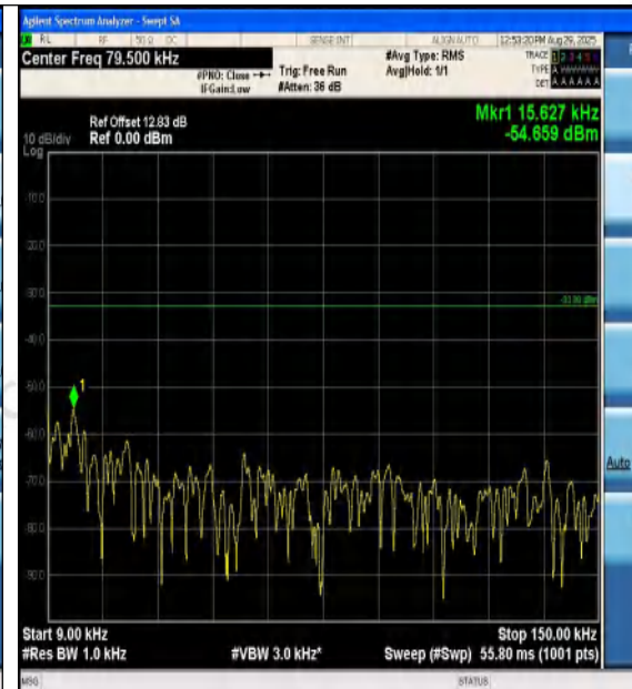
Band12-5MHz-16QAM-23095-25RB#0-0.009~0.15 -PASS
