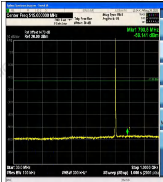
Band12-5MHz-QPSK-23155-1RB#0-30~1000-PA
