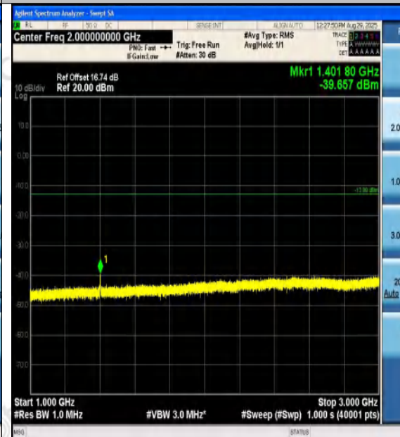
Band12-3MHz-QPSK-23025-15RB#0-1000~3000- PASS
