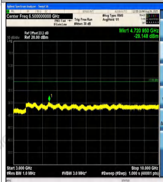
Band12-5MHz-QPSK-23155-1RB#0-3000~10000
