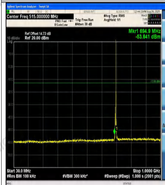
Band12-5MHz-QPSK-23035-1RB#24-30~1000-P ASS
