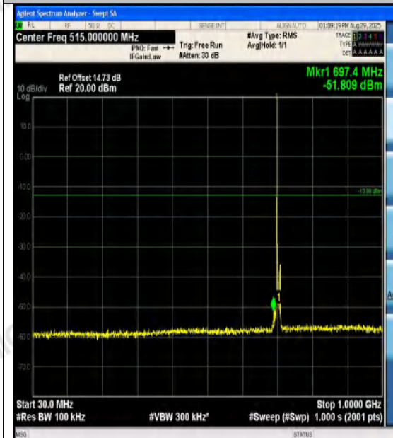
Band12-10MHz-QPSK-23130-1RB#0-30~1000-P ASS
