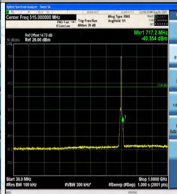
Band12-5MHz-16QAM-23095-25RB#0-30~1000-P ASS
