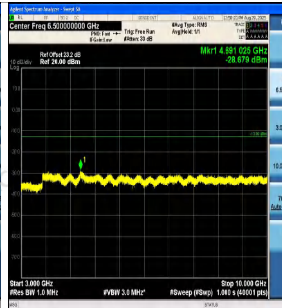
Band12-5MHz-16QAM-23155-1RB#24-3000~1000 0-PASS
