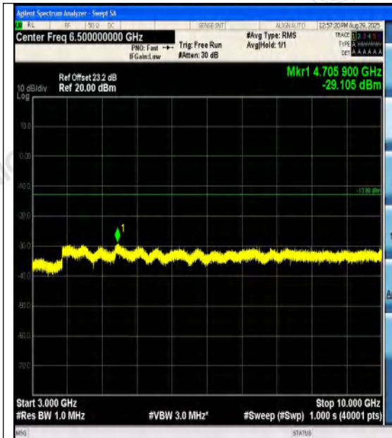
Band12-5MHz-QPSK-23155-1RB#24-3000~1000 0-PASS
