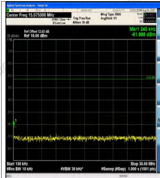
Band12-5MHz-16QAM-23095-1RB#24-0.15~30-P
