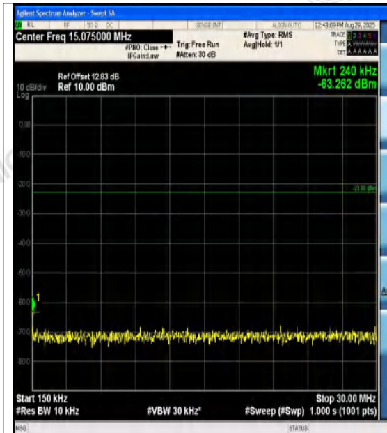
Band12-5MHz-16QAM-23035-1RB#0-0.15~30-PA
