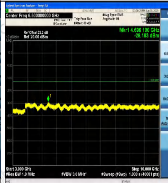
Band12-5MHz-16QAM-23155-25RB#0-3000~1000 0-PASS
