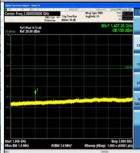
Band12-5MHz-QPSK-23035-1RB#24-1000~3000- PASS
