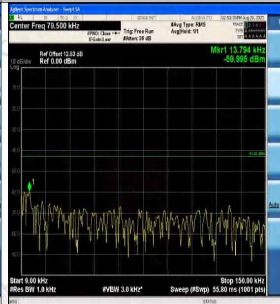
Band4-3MHz-16QAM-19965-15RB#0-0.009~0.15- PASS
