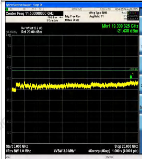
Band4-1.4MHz-16QAM-20393-1RB#0-3000~200
