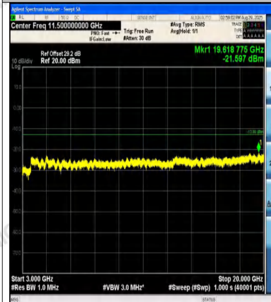
Band4-3MHz-QPSK-20385-1RB#0-3000~20000-
