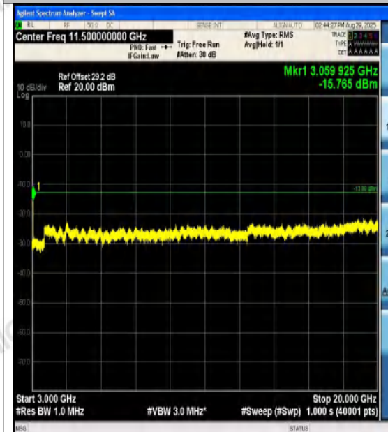
Band4-1.4MHz-QPSK-20175-6RB#0-3000~20000 -PASS
