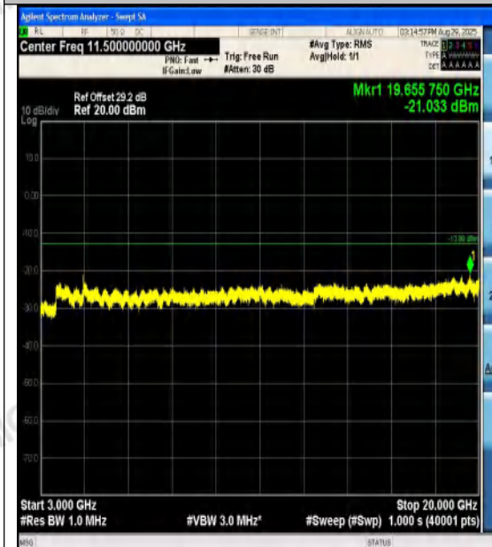
Band4-5MHz-QPSK-20375-25RB#0-3000~20000
