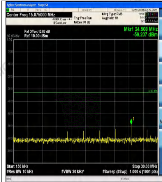
Band4-3MHz-16QAM-20385-1RB#0-0.15~30-PA
