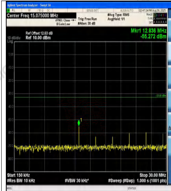
Band4-1.4MHz-16QAM-20393-1RB#5-0.15~30-P
