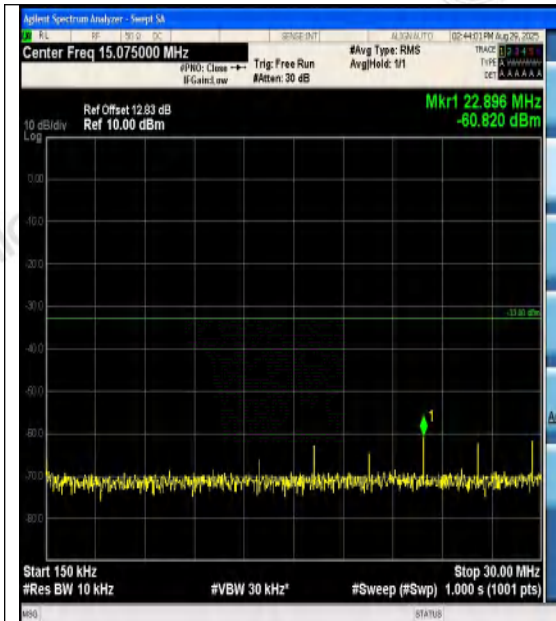
Band4-1.4MHz-QPSK-20175-6RB#0-0.15~30-PA SS
