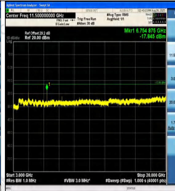
Band4-1.4MHz-QPSK-20175-1RB#5-3000~20000- PASS
