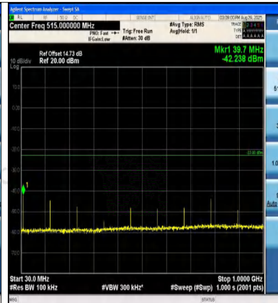
Band4-5MHz-QPSK-20175-1RB#24-30~1000-PAS
