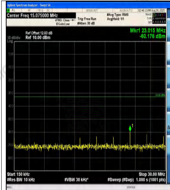
Band4-1.4MHz-16QAM-20393-1RB#0-0.15~30-P
