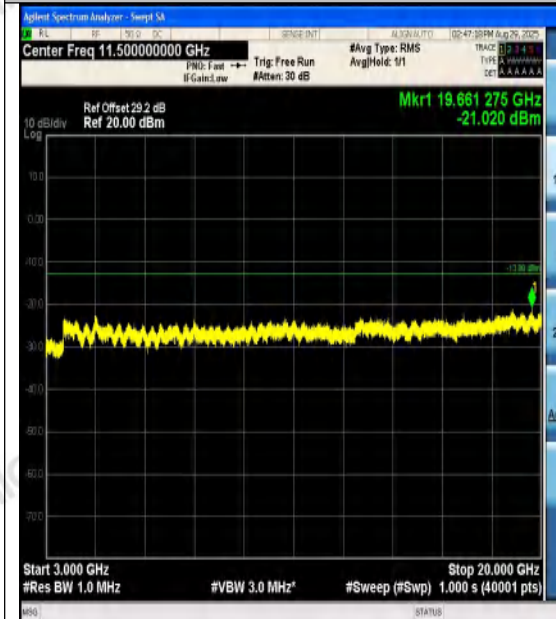
Band4-1.4MHz-QPSK-20393-1RB#5-3000~20000 -PASS
