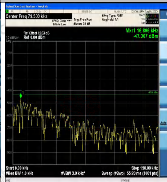
Band4-1.4MHz-16QAM-20175-1RB#0-0.009~0.15-
