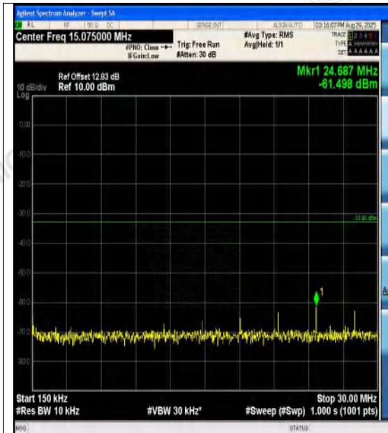
Band4-10MHz-QPSK-20000-1RB#0-0.15~30-PA
