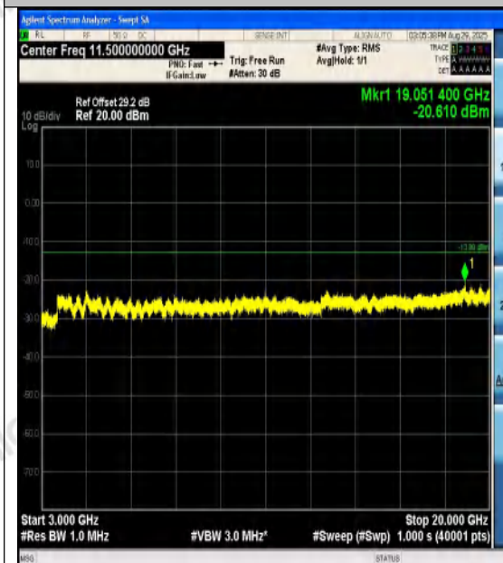
Band4-5MHz-16QAM-19975-1RB#24-3000~2000
