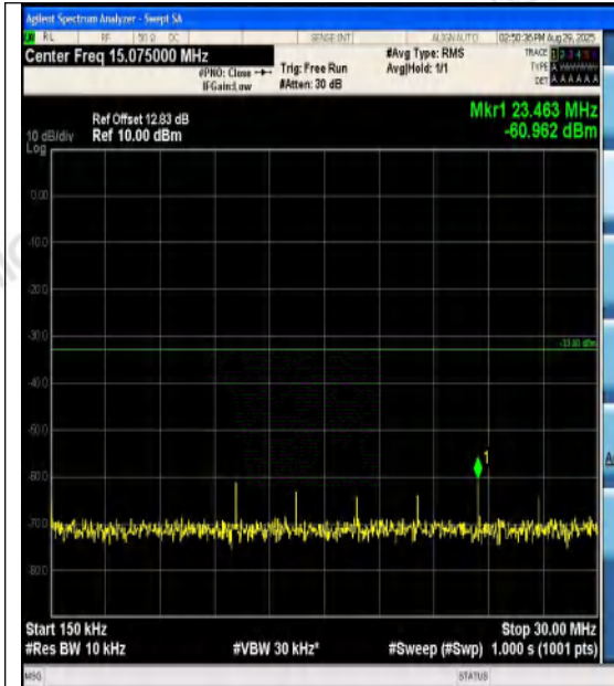
Band4-3MHz-16QAM-19965-1RB#0-0.15~30-PA
