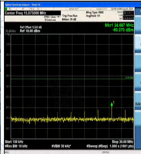
Band4-3MHz-QPSK-20175-1RB#14-0.15~30-PAS
