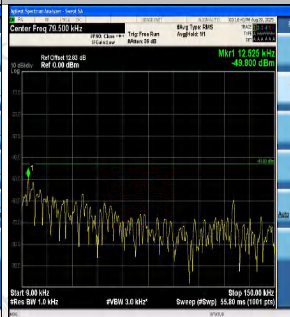
Band4-10MHz-16QAM-20000-1RB#0-0.009~0.15-
