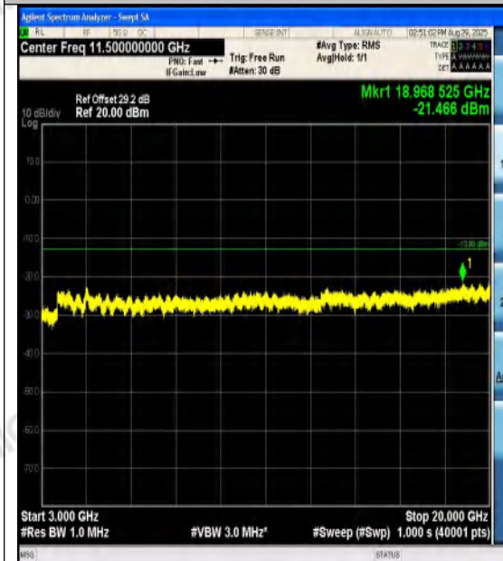
Band4-3MHz-16QAM-19965-1RB#0-3000~20000
