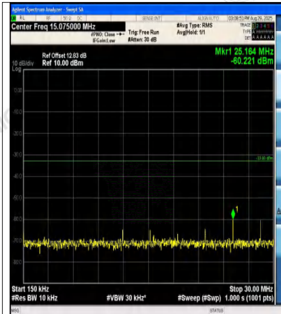
Band4-5MHz-QPSK-20175-1RB#24-0.15~30-PA
