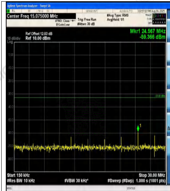
Band4-3MHz-QPSK-20175-1RB#0-0.15~30-PAS
