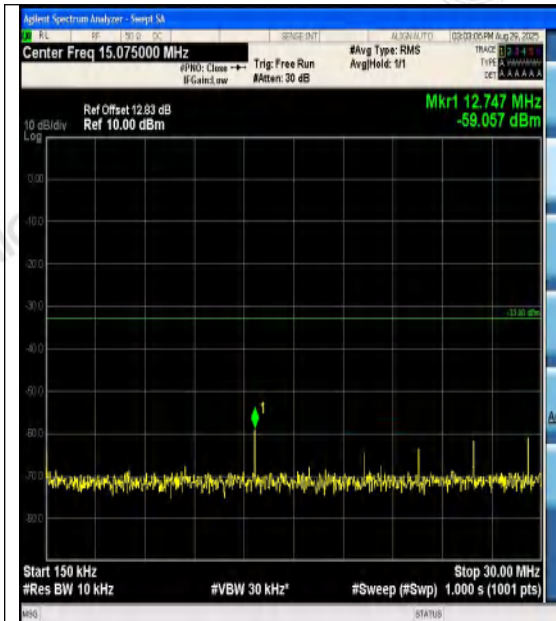
Band4-5MHz-QPSK-19975-1RB#0-0.15~30-PAS
