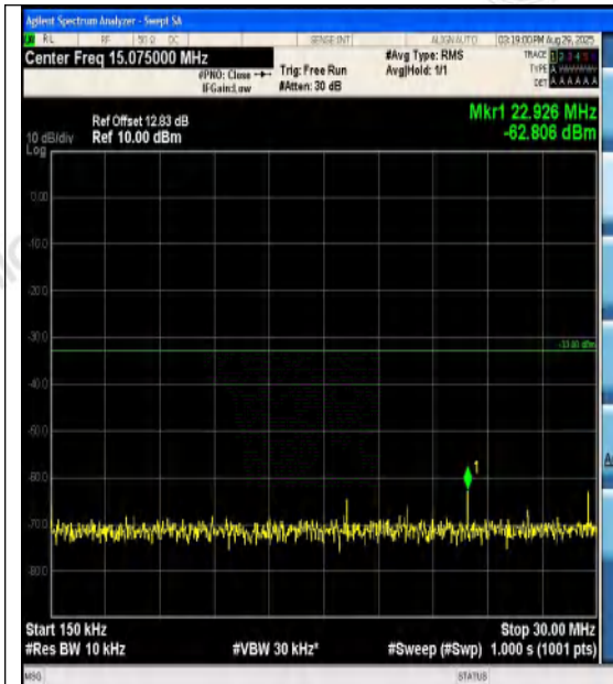
Band4-10MHz-QPSK-20175-1RB#0-0.15~30-PA
