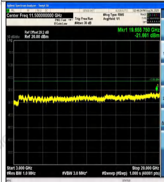
Band4-1.4MHz-16QAM-20393-6RB#0-3000~200 00-PASS
