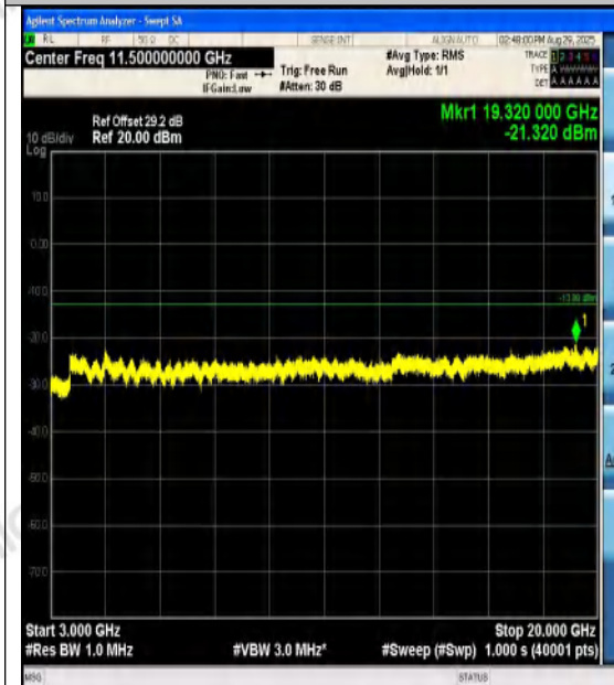
Band4-1.4MHz-16QAM-20393-1RB#5-3000~200
