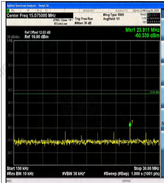
Band4-1.4MHz-QPSK-20175-1RB#0-0.15~30-PA
