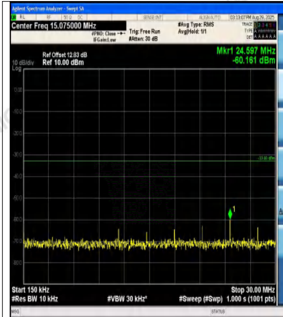
Band4-5MHz-QPSK-20375-1RB#24-0.15~30-PA
