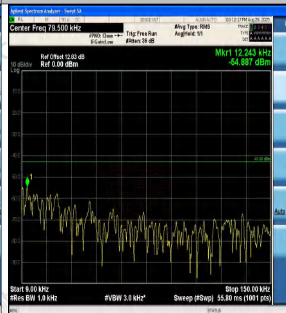
Band4-5MHz-16QAM-20375-1RB#0-0.009~0.15-P
