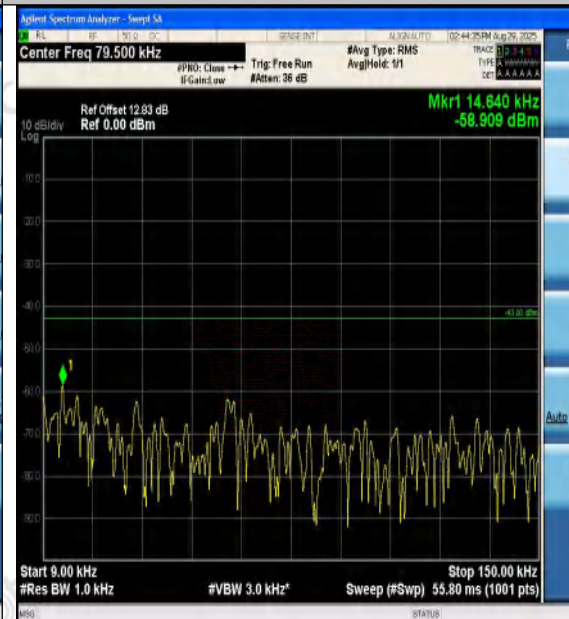
Band4-1.4MHz-16QAM-20175-6RB#0-0.009~0.15- PASS
