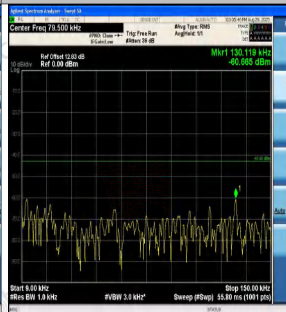
Band4-5MHz-QPSK-19975-25RB#0-0.009~0.15-P
