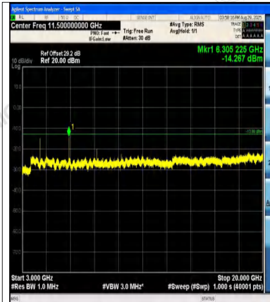
Band4-3MHz-16QAM-20175-1RB#0-3000~20000 -PASS
