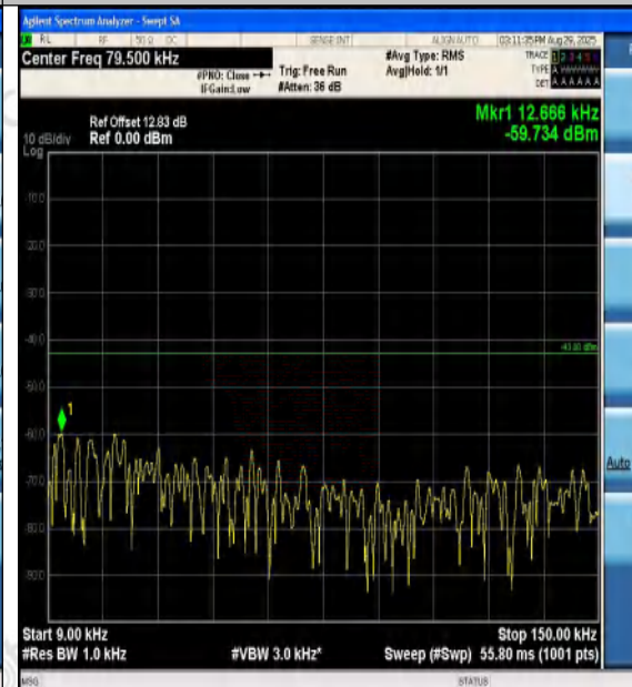
Band4-5MHz-QPSK-20375-1RB#0-0.009~0.15-PA
