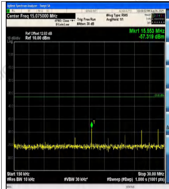
Band4-3MHz-QPSK-20385-1RB#14-0.15~30-PA SS
