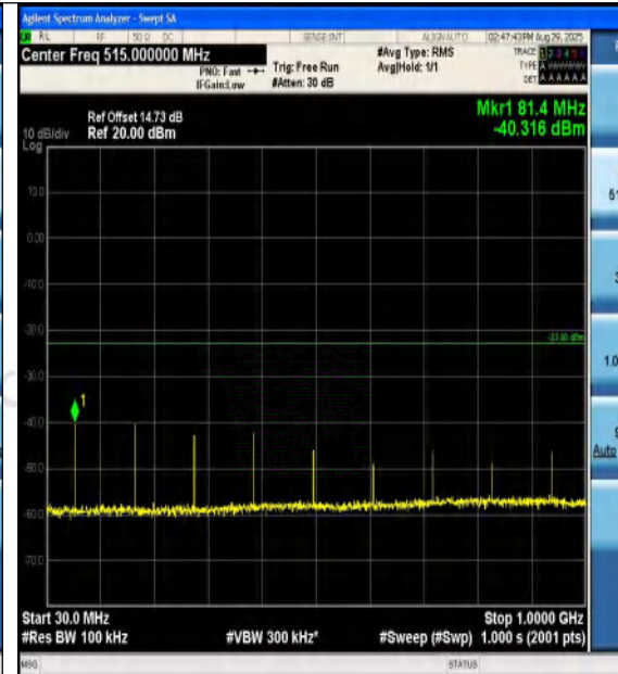
Band4-1.4MHz-16QAM-20393-1RB#5-30~1000-P
