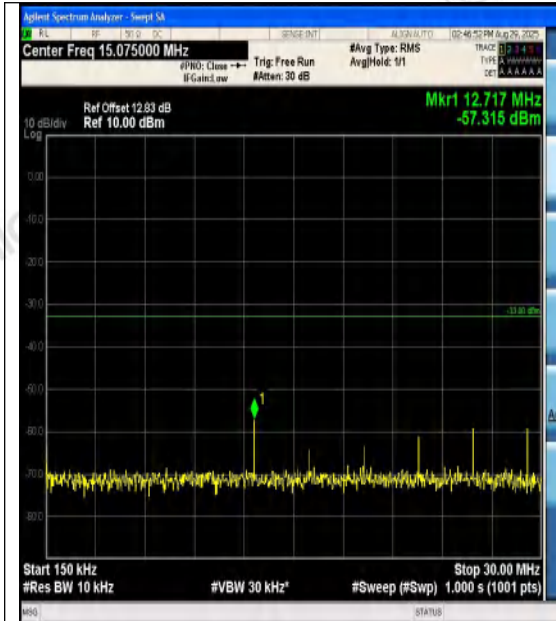
Band4-1.4MHz-QPSK-20393-1RB#5-0.15~30-PA SS
