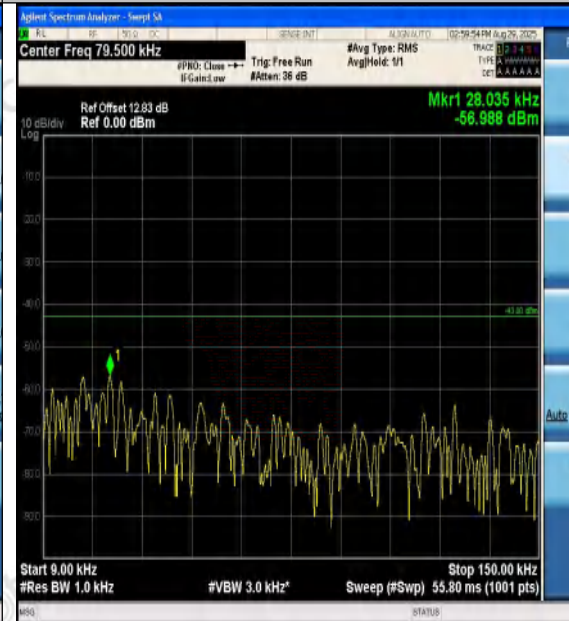
Band4-3MHz-QPSK-20385-1RB#14-0.009~0.15-P
