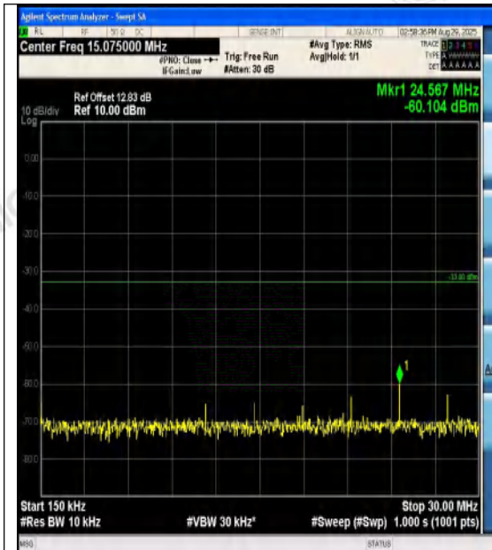
Band4-3MHz-QPSK-20385-1RB#0-0.15~30-PAS
