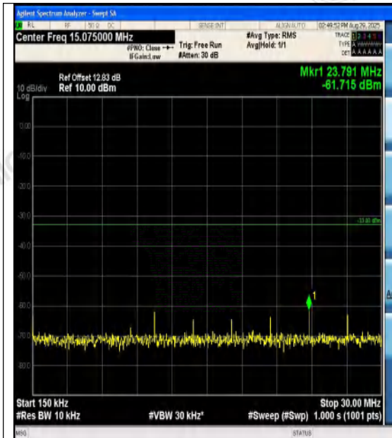
Band4-3MHz-QPSK-19965-1RB#0-0.15~30-PAS
