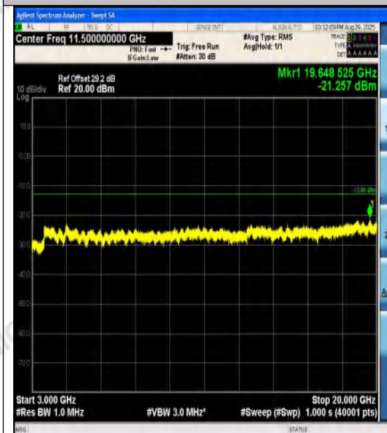
Band4-5MHz-QPSK-20375-1RB#0-3000~20000-
