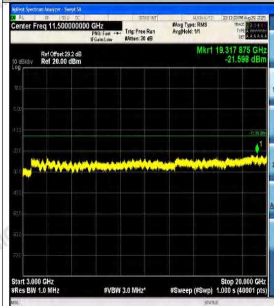
Band4-5MHz-QPSK-20375-1RB#24-3000~20000
