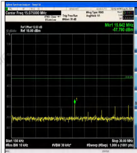
Band4-3MHz-QPSK-19965-15RB#0-0.15~30-PA SS
