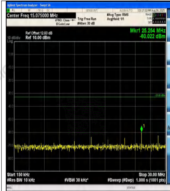
Band4-10MHz-QPSK-20000-1RB#49-0.15~30-PA
