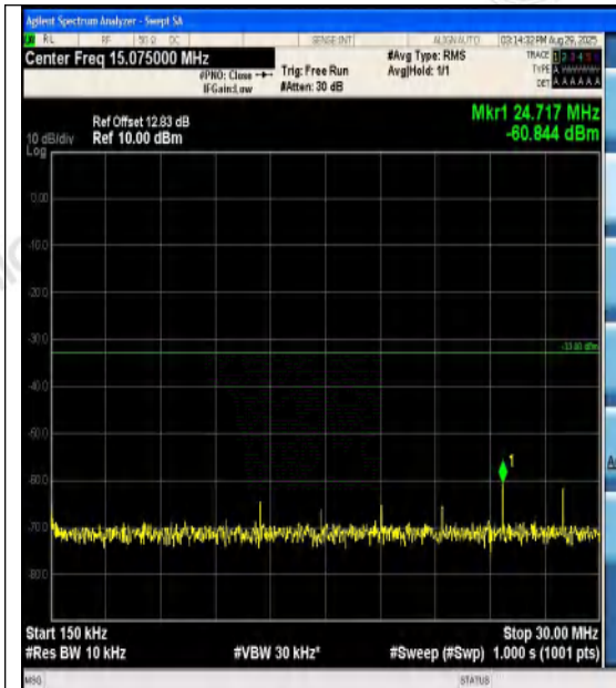
Band4-5MHz-QPSK-20375-25RB#0-0.15~30-PA
