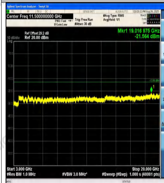
Band4-5MHz-QPSK-19975-1RB#0-3000~20000-
