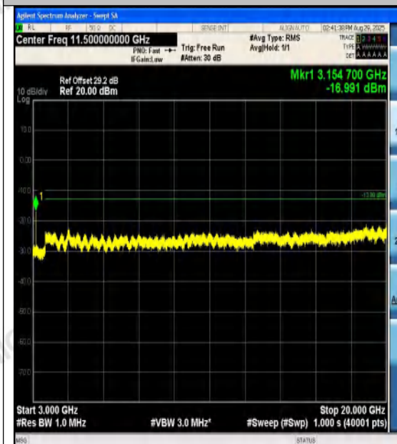
Band4-1.4MHz-QPSK-20175-1RB#0-3000~20000
