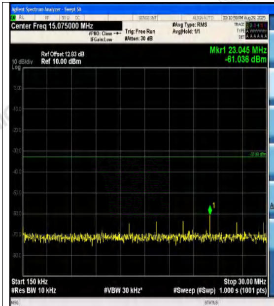
Band4-5MHz-16QAM-20175-25RB#0-0.15~30-PA
