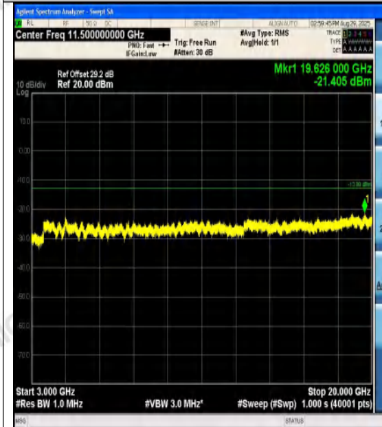
Band4-3MHz-16QAM-20385-1RB#0-3000~20000
