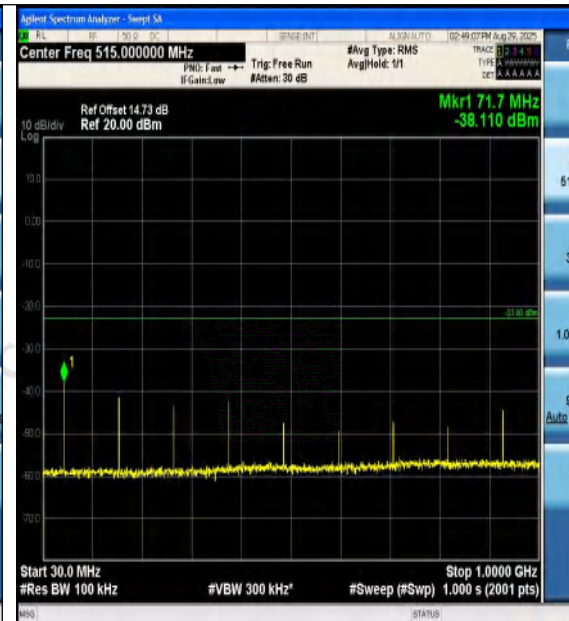
Band4-1.4MHz-16QAM-20393-6RB#0-30~1000-P ASS
