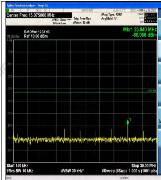
Band4-5MHz-QPSK-20375-1RB#0-0.15~30-PAS
