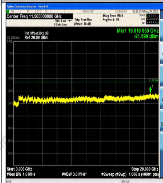
Band4-10MHz-QPSK-20000-1RB#0-3000~20000
