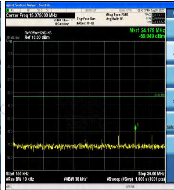
Band4-1.4MHz-QPSK-20175-1RB#5-0.15~30-PAS S
