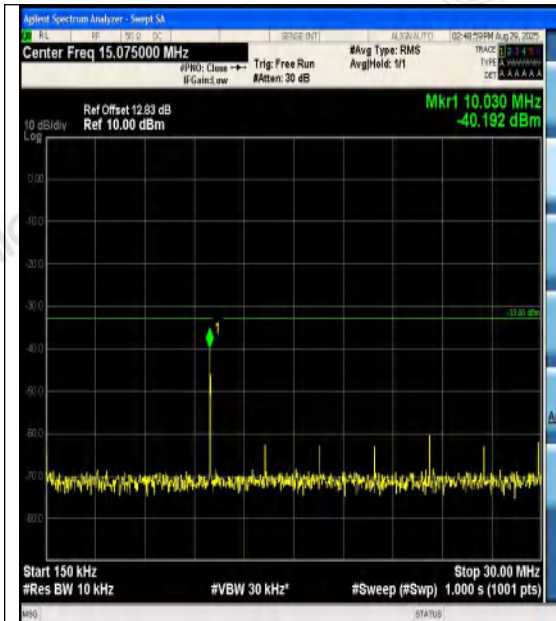
Band4-1.4MHz-16QAM-20393-6RB#0-0.15~30-P ASS
