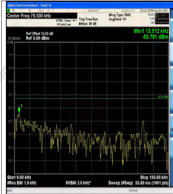
Band4-1.4MHz-QPSK-20175-1RB#5-0.009~0.15- PASS
