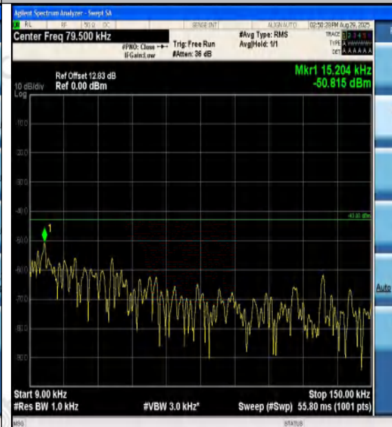
Band4-3MHz-16QAM-19965-1RB#0-0.009~0.15-P
