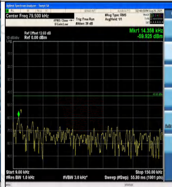
Band4-1.4MHz-QPSK-20393-6RB#0-0.009~0.15-P
