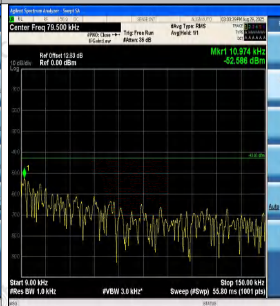
Band4-5MHz-16QAM-19975-1RB#0-0.009~0.15-P
