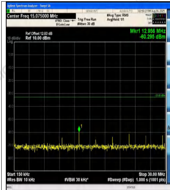
Band4-3MHz-16QAM-19965-15RB#0-0.15~30-PA
