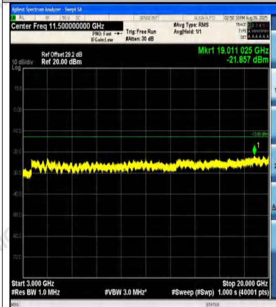
Band4-3MHz-QPSK-19965-1RB#0-3000~20000-
