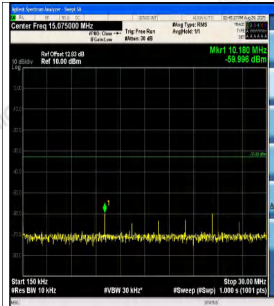
Band4-1.4MHz-QPSK-20393-1RB#0-0.15~30-PA SS
