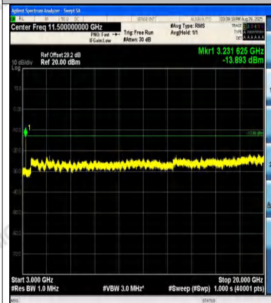
Band4-5MHz-QPSK-20175-1RB#24-3000~20000
