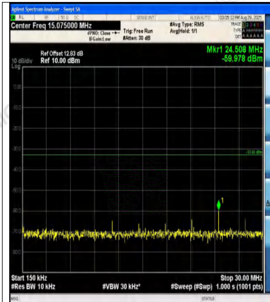
Band4-5MHz-16QAM-19975-1RB#24-0.15~30-PA
