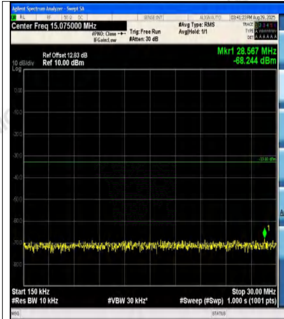
Band4-20MHz-QPSK-20050-1RB#0-0.15~30-PA
