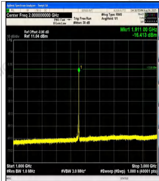
Band2-1.4MHz-QPSK-19193-1RB#5-1000~3000- PASS
