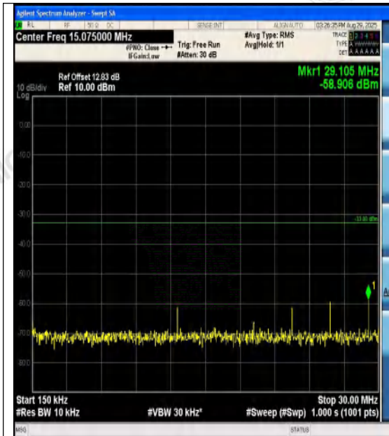
Band4-10MHz-QPSK-20350-50RB#0-0.15~30-PA
