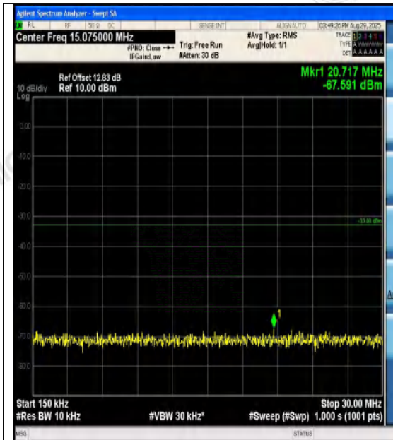
Band4-20MHz-16QAM-20300-1RB#99-0.15~30-P ASS
