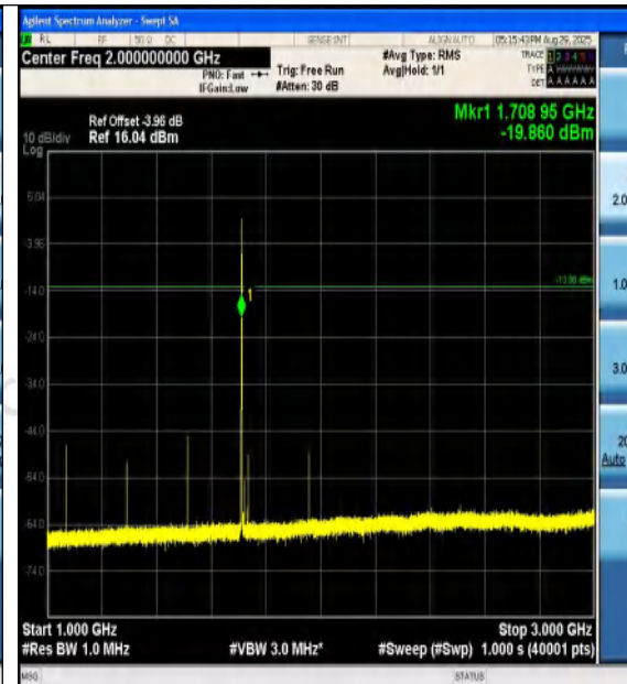
Band4-1.4MHz-16QAM-19957-1RB#0-1000~3000- PASS
