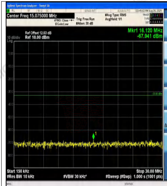
Band4-20MHz-16QAM-20175-1RB#0-0.15~30-PA SS
