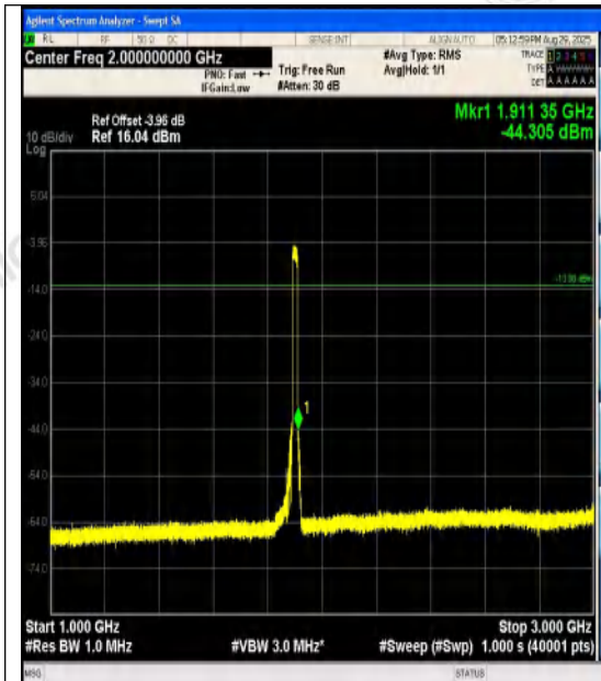
Band2-20MHz-QPSK-19100-100RB#0-1000~300 0-PASS
