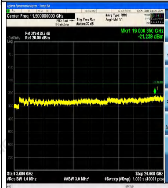
Band4-15MHz-QPSK-20325-1RB#74-3000~2000
