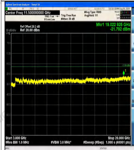
Band4-15MHz-QPSK-20175-1RB#74-3000~2000
