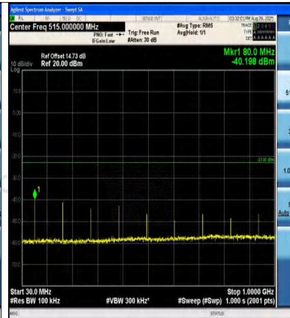
Band4-15MHz-QPSK-20175-1RB#74-30~1000-PA
