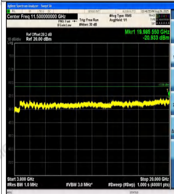
Band4-20MHz-16QAM-20175-1RB#99-3000~200 00-PASS
