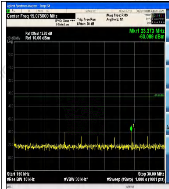
Band4-15MHz-QPSK-20325-1RB#74-0.15~30-PA
