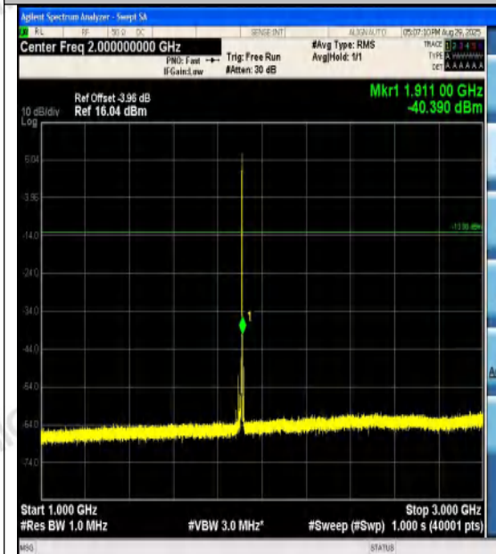
Band2-15MHz-16QAM-19125-1RB#74-1000~300 0-PASS
