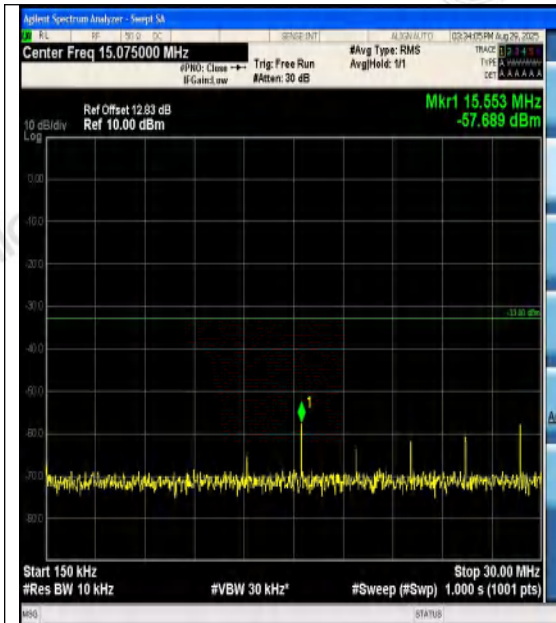
Band4-15MHz-16QAM-20325-1RB#0-0.15~30-PA
