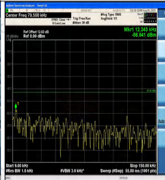
Band4-15MHz-QPSK-20175-1RB#0-0.009~0.15-P
