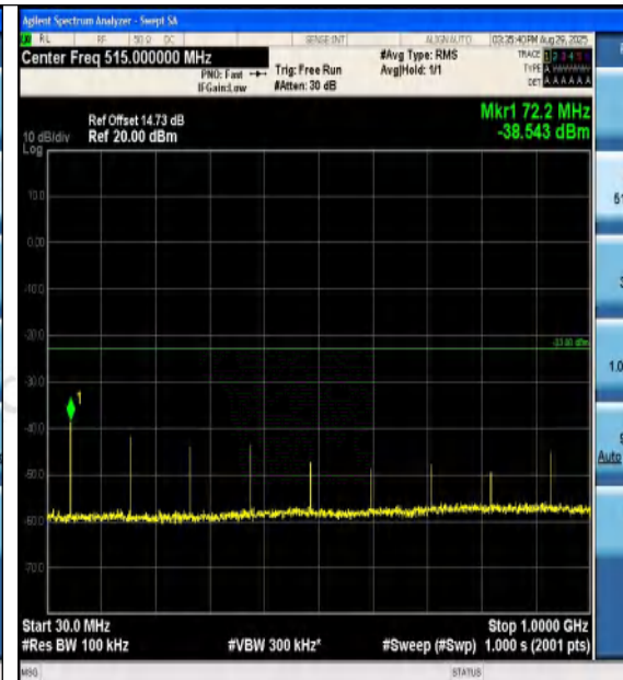
Band4-15MHz-16QAM-20325-1RB#74-30~1000-P ASS
