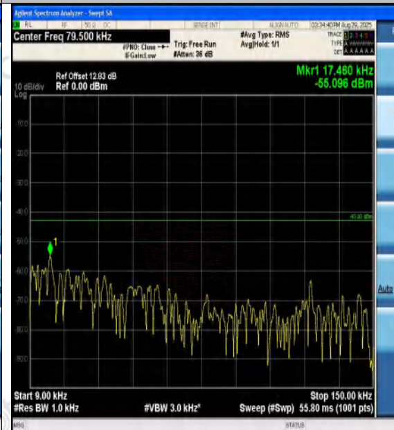
Band4-15MHz-QPSK-20325-1RB#74-0.009~0.15-
