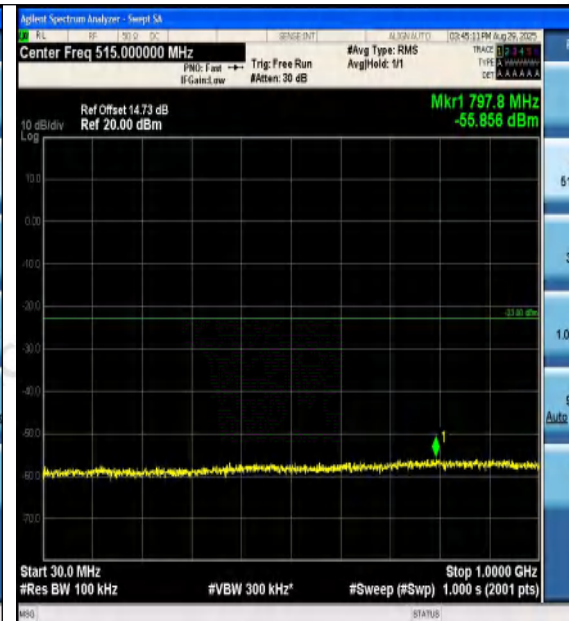
Band4-20MHz-16QAM-20175-1RB#0-30~1000-PA SS
