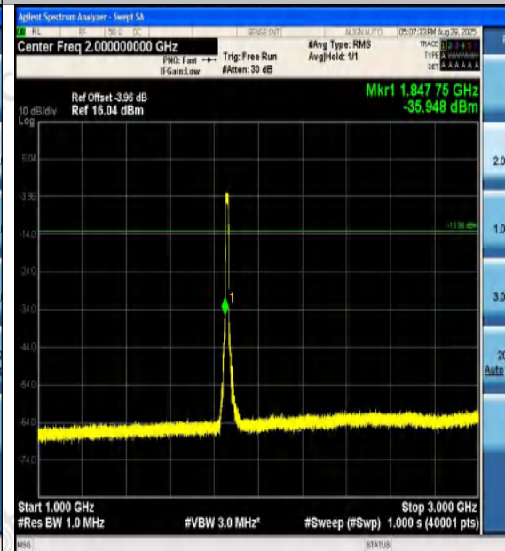
Band2-15MHz-QPSK-18675-75RB#0-1000~3000- PASS
