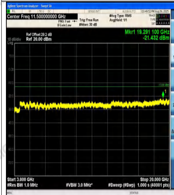
Band4-20MHz-16QAM-20300-1RB#99-3000~200 00-PASS
