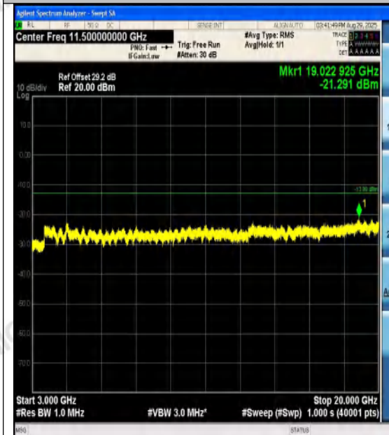
Band4-20MHz-QPSK-20050-1RB#0-3000~20000
