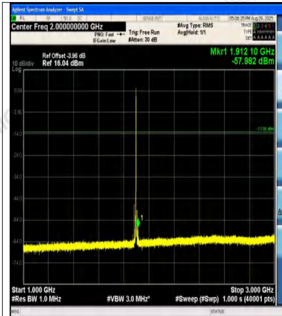
Band2-15MHz-16QAM-19125-1RB#0-1000~3000 -PASS
