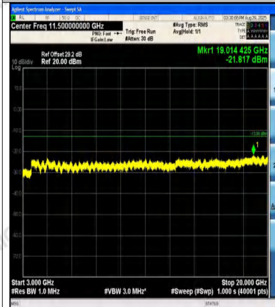
Band4-15MHz-16QAM-20025-1RB#74-3000~200
