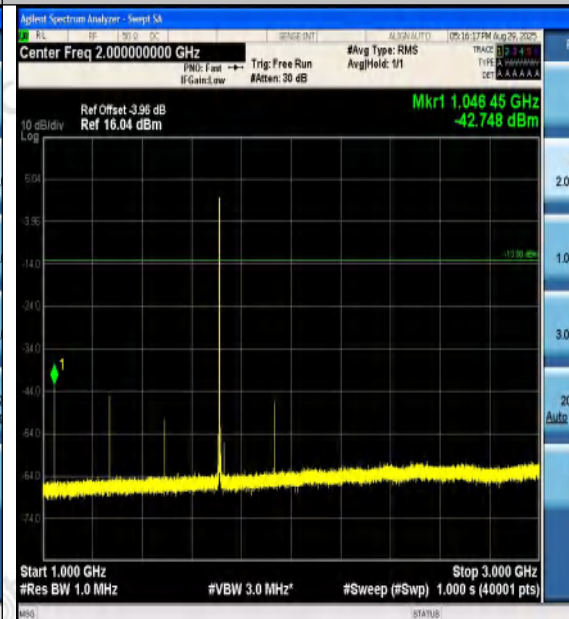
Band4-1.4MHz-16QAM-19957-1RB#5-1000~3000- PASS
