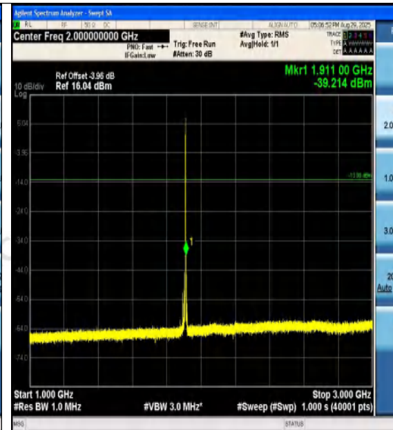
Band2-15MHz-QPSK-19125-1RB#74-1000~3000- PASS
