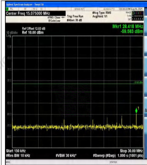
Band4-15MHz-QPSK-20325-1RB#0-0.15~30-PA
