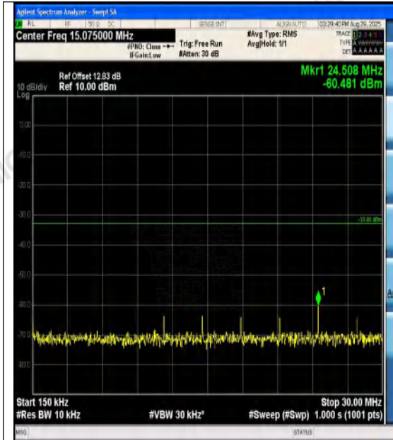
Band4-15MHz-16QAM-20025-1RB#74-0.15~30-P
