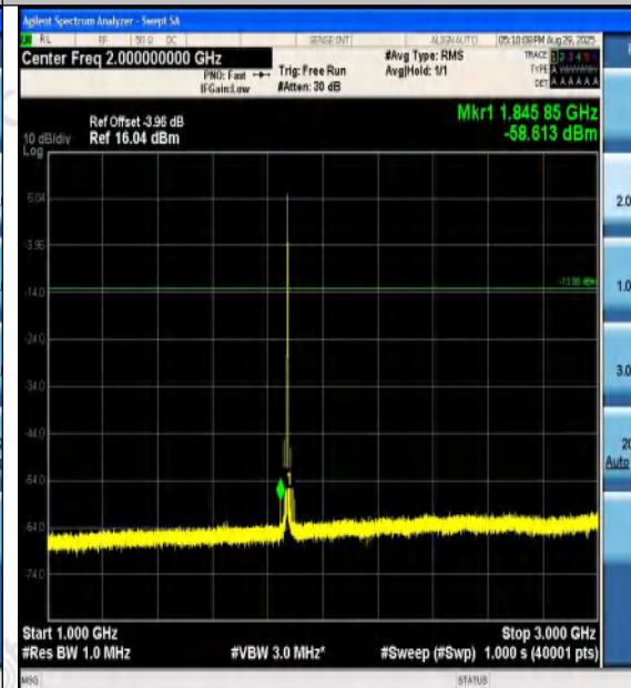
Band2-20MHz-16QAM-18900-1RB#0-1000~3000- PASS
