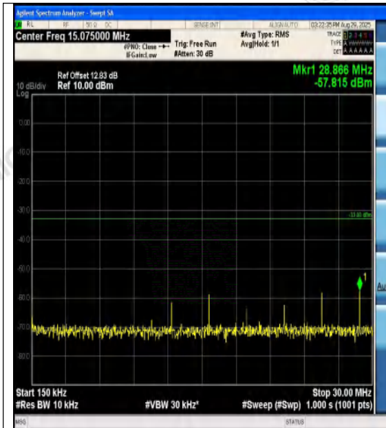
Band4-10MHz-16QAM-20350-1RB#0-0.15~30-PA SS
