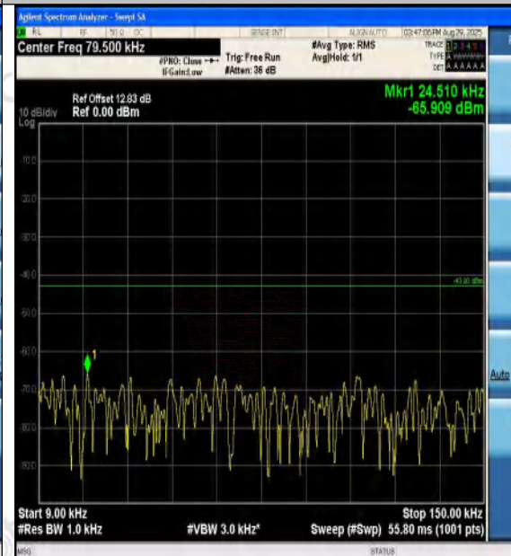
Band4-20MHz-QPSK-20300-1RB#0-0.009~0.15-P ASS
