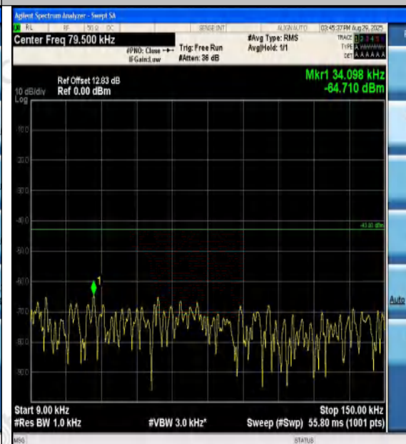
Band4-20MHz-QPSK-20175-1RB#99-0.009~0.15- PASS
