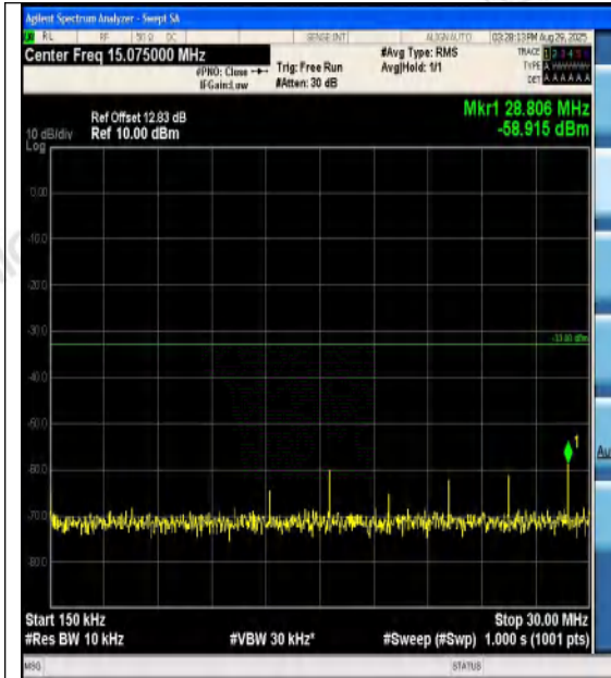
Band4-15MHz-16QAM-20025-1RB#0-0.15~30-PA
