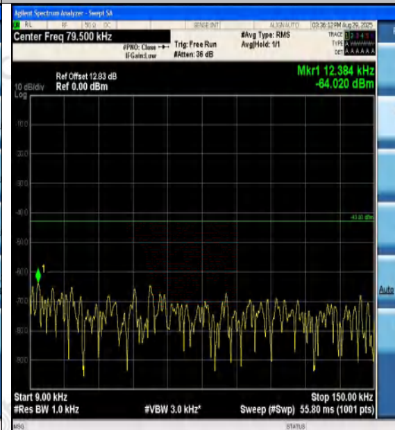
Band4-15MHz-QPSK-20025-75RB#0-0.009~0.15- PASS
