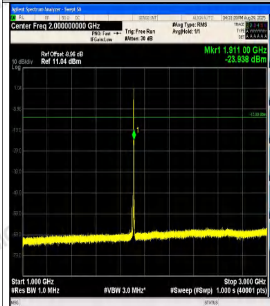
Band2-1.4MHz-QPSK-19193-6RB#0-1000~3000- PASS
