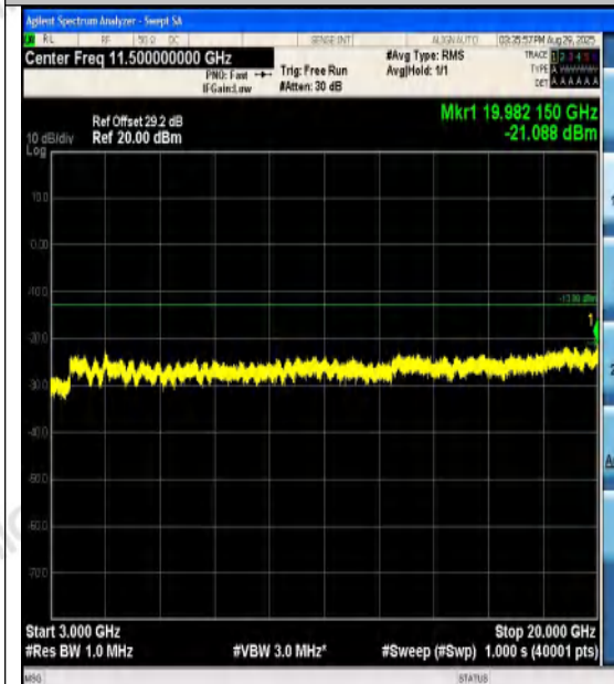
Band4-15MHz-16QAM-20325-1RB#74-3000~200 00-PASS
