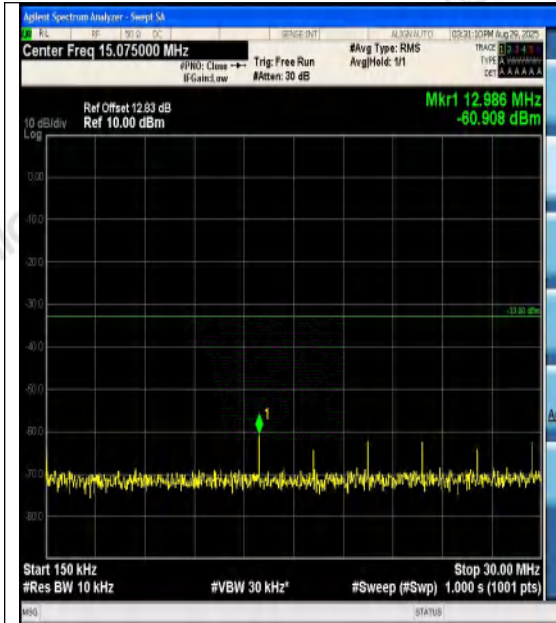
Band4-15MHz-16QAM-20175-1RB#0-0.15~30-PA
