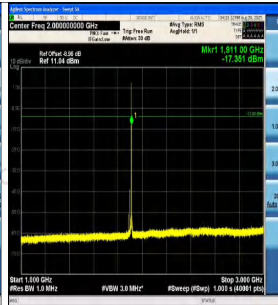
Band2-1.4MHz-16QAM-19193-1RB#5-1000~3000- PASS
