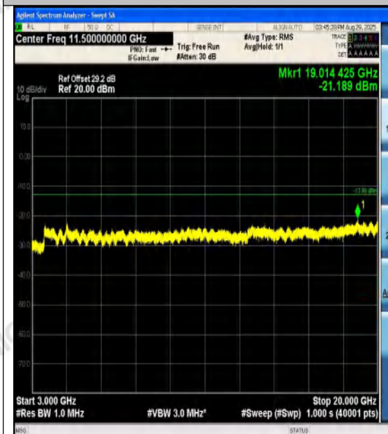
Band4-20MHz-16QAM-20175-1RB#0-3000~2000 0-PASS
