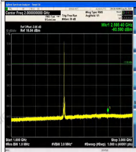
Band2-20MHz-QPSK-18900-1RB#0-1000~3000- PASS
