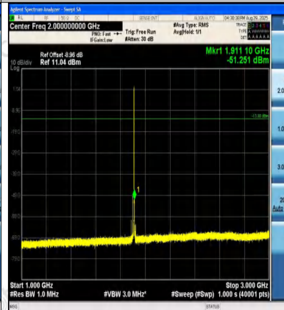
Band2-1.4MHz-16QAM-19193-1RB#0-1000~3000-
