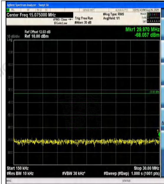
Band4-20MHz-QPSK-20300-100RB#0-0.15~30-P
