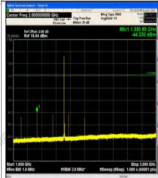
Band4-1.4MHz-QPSK-19957-1RB#5-1000~3000- PASS
