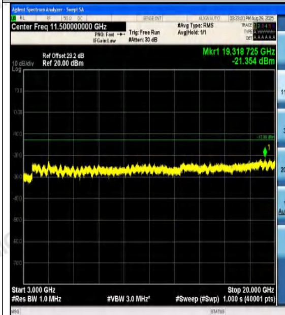
Band4-10MHz-16QAM-20350-1RB#0-3000~2000 0-PASS
