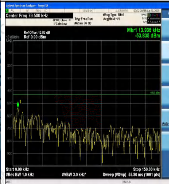
Band4-15MHz-16QAM-20175-1RB#74-0.009~0.15
