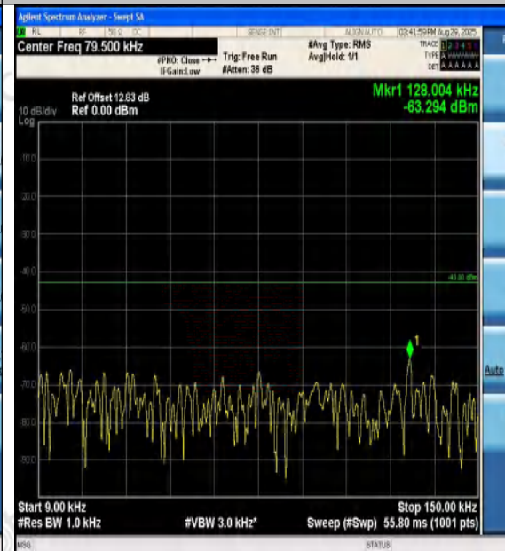
Band4-20MHz-16QAM-20050-1RB#0-0.009~0.15-
