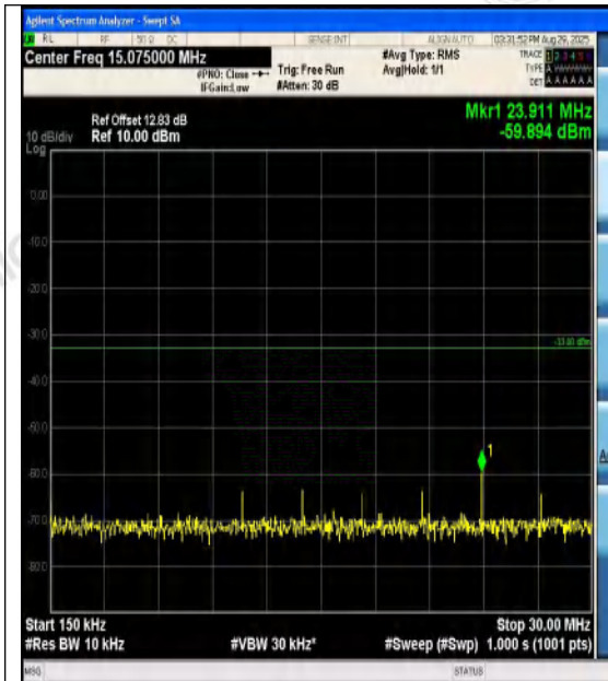
Band4-15MHz-QPSK-20175-1RB#74-0.15~30-PA
