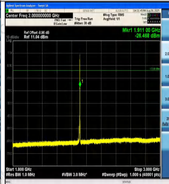
Band2-1.4MHz-16QAM-19193-6RB#0-1000~3000- PASS
