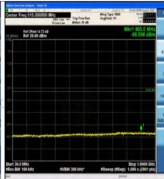
Band4-20MHz-16QAM-20300-1RB#99-30~1000-P ASS
