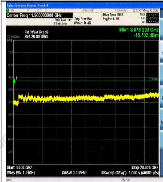
Band4-15MHz-QPSK-20325-1RB#0-3000~20000
