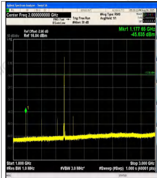
Band4-10MHz-QPSK-20000-1RB#49-1000~3000 -PASS
