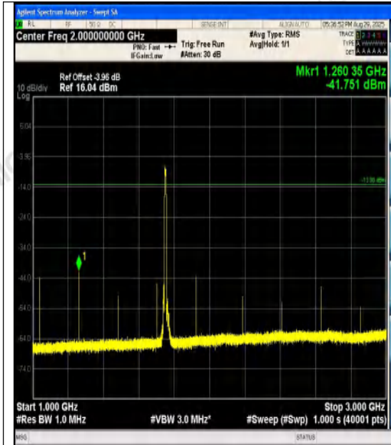
Band4-10MHz-QPSK-20350-50RB#0-1000~3000
