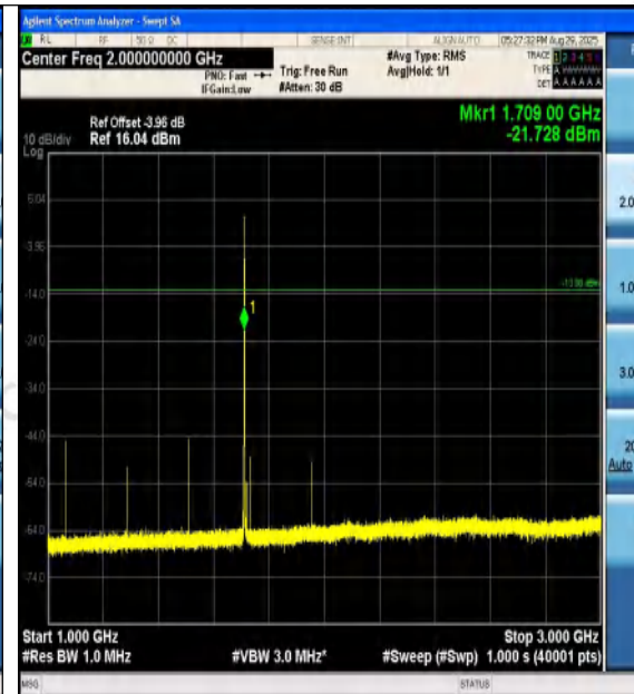
Band4-5MHz-16QAM-19975-1RB#0-1000~3000-P ASS
