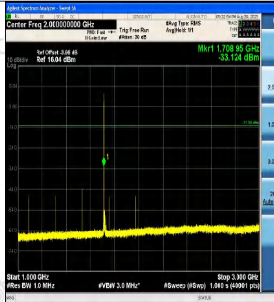
Band4-10MHz-16QAM-20000-1RB#0-1000~3000- PASS
