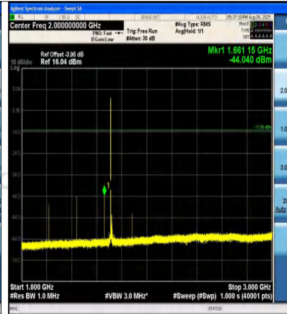
Band4-15MHz-QPSK-20025-1RB#0-1000~3000-P
