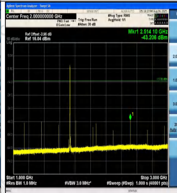
Band4-1.4MHz-16QAM-20175-6RB#0-1000~3000- PASS
