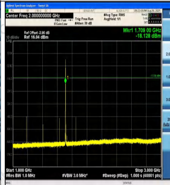
Band4-3MHz-16QAM-19965-1RB#0-1000~3000-P ASS
