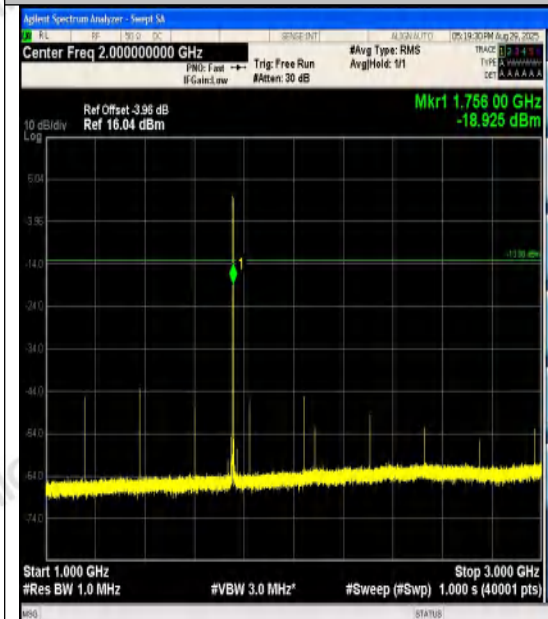
Band4-1.4MHz-QPSK-20393-1RB#5-1000~3000- PASS
