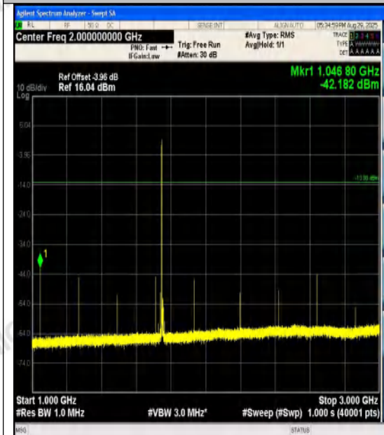
Band4-10MHz-QPSK-20350-1RB#0-1000~3000-
