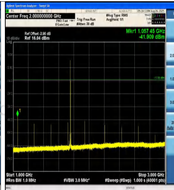
Band4-1.4MHz-16QAM-20393-1RB#0-1000~3000- PASS
