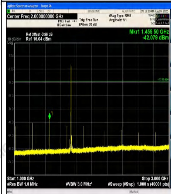
Band4-1.4MHz-QPSK-20175-6RB#0-1000~3000- PASS
