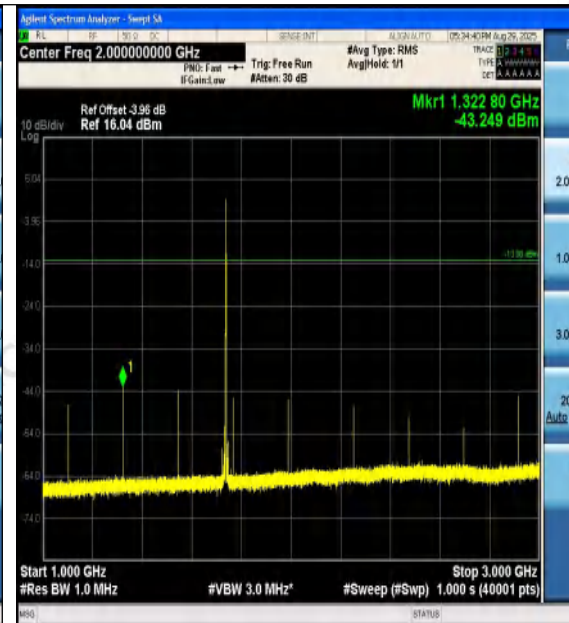
Band4-10MHz-16QAM-20175-1RB#49-1000~3000
