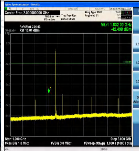
Band4-10MHz-16QAM-20350-1RB#0-1000~3000-
