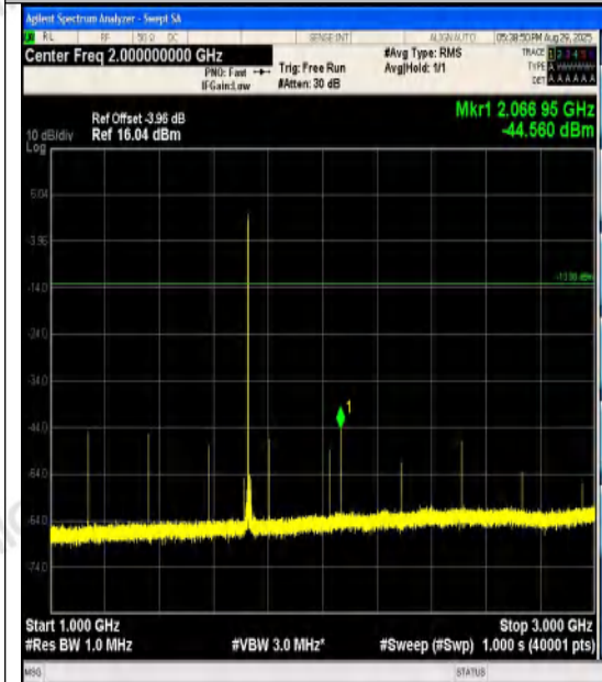
Band4-15MHz-16QAM-20175-1RB#0-1000~3000 -PASS
