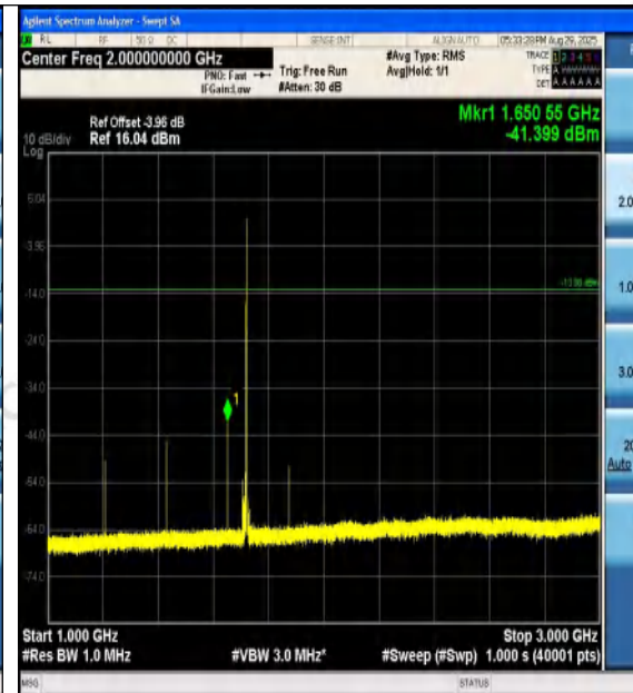
Band4-10MHz-16QAM-20000-1RB#49-1000~3000 -PASS
