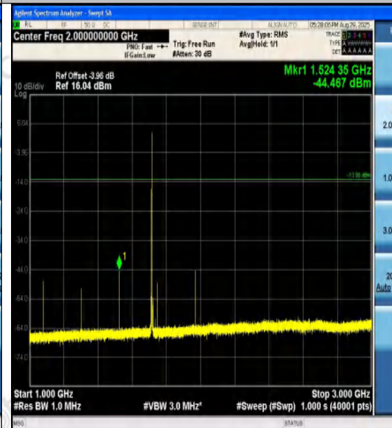
Band4-5MHz-16QAM-19975-1RB#24-1000~3000- PASS
