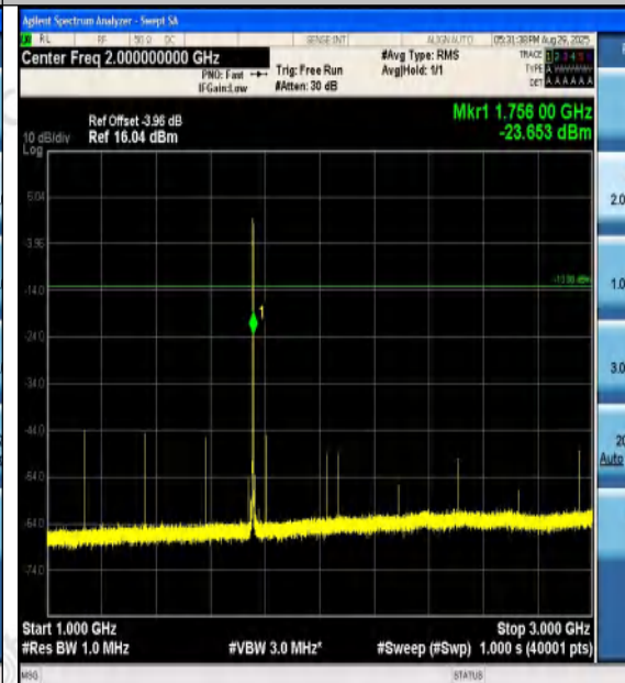
Band4-5MHz-16QAM-20375-1RB#24-1000~3000-
