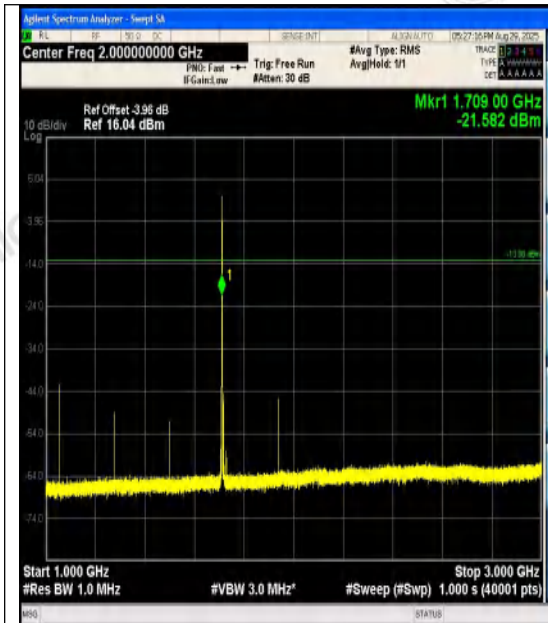
Band4-5MHz-QPSK-19975-1RB#0-1000~3000-P ASS
