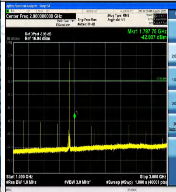
Band4-10MHz-16QAM-20175-1RB#0-1000~3000- PASS
