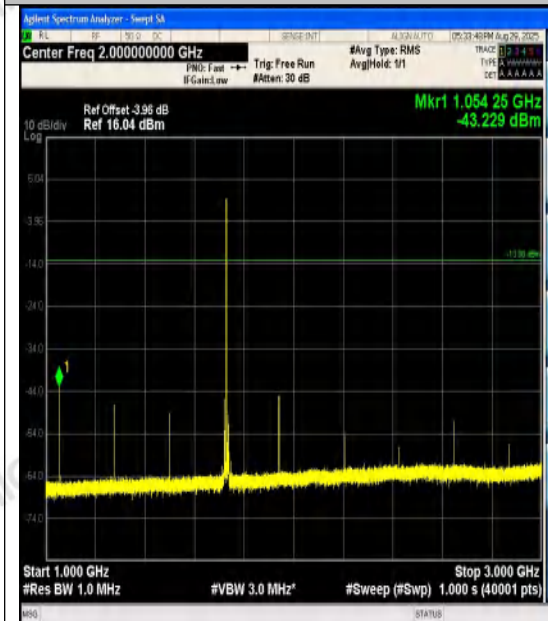
Band4-10MHz-QPSK-20175-1RB#0-1000~3000- PASS
