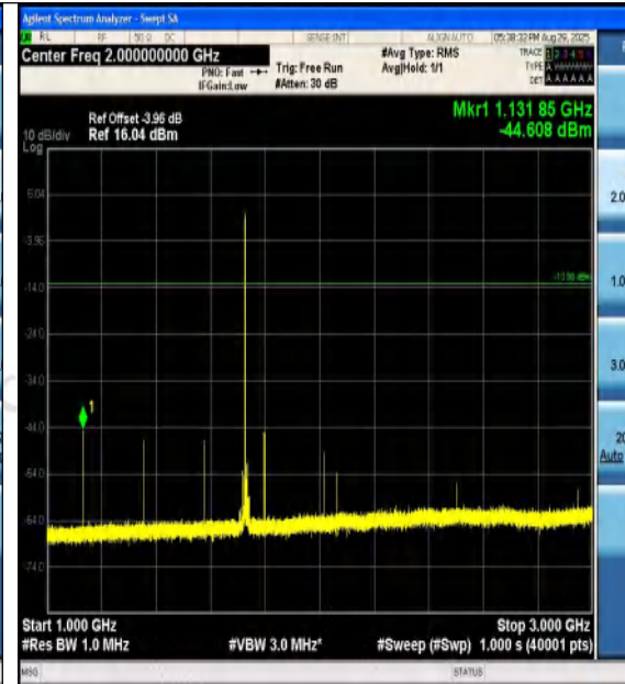
Band4-15MHz-QPSK-20175-1RB#0-1000~3000-P ASS
