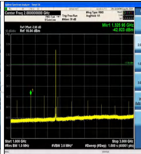
Band4-1.4MHz-16QAM-20175-1RB#5-1000~3000- PASS
