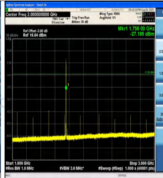
Band4-1.4MHz-16QAM-20393-6RB#0-1000~3000- PASS
