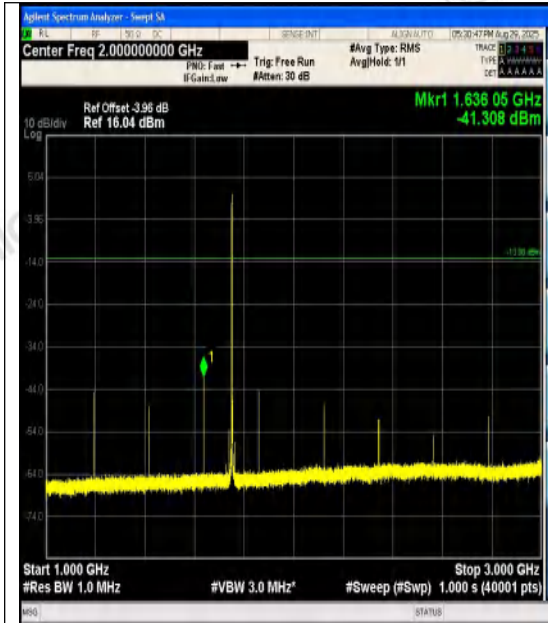
Band4-5MHz-QPSK-20375-1RB#0-1000~3000-P
