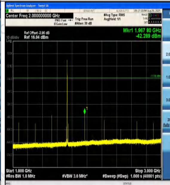
Band4-1.4MHz-16QAM-20175-1RB#0-1000~3000- PASS
