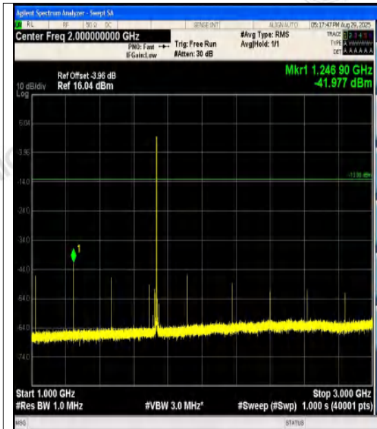
Band4-1.4MHz-QPSK-20175-1RB#5-1000~3000- PASS
