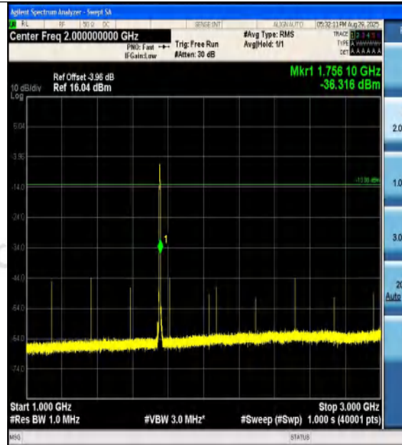
Band4-5MHz-16QAM-20375-25RB#0-1000~3000- PASS
