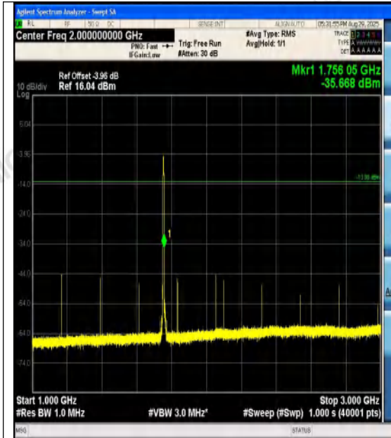
Band4-5MHz-QPSK-20375-25RB#0-1000~3000- PASS
