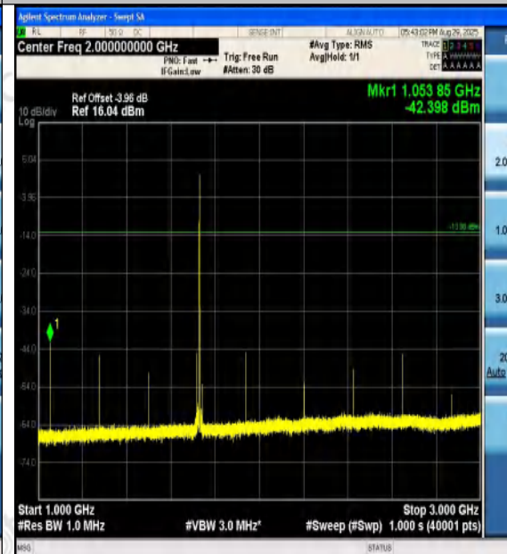
Band4-20MHz-16QAM-20050-1RB#99-1000~3000- -PASS
