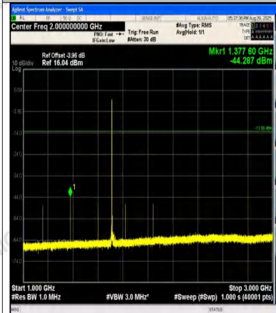
Band4-15MHz-16QAM-20025-1RB#0-1000~3000
