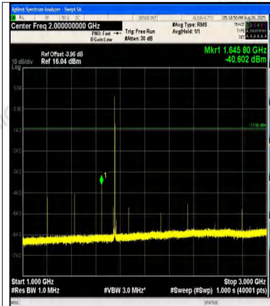
Band4-1.4MHz-QPSK-20393-1RB#0-1000~3000- PASS
