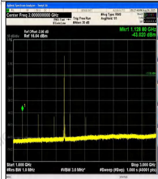
Band4-5MHz-QPSK-19975-1RB#24-1000~3000- PASS
