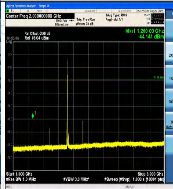
Band4-15MHz-QPSK-20025-1RB#74-1000~3000-
