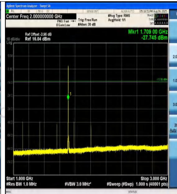
Band4-1.4MHz-16QAM-19957-6RB#0-1000~3000- PASS
