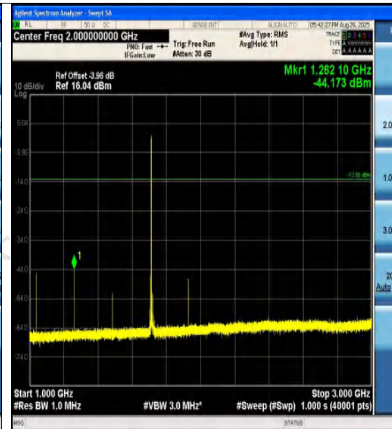
Band4-20MHz-16QAM-20050-1RB#0-1000~3000- PASS
