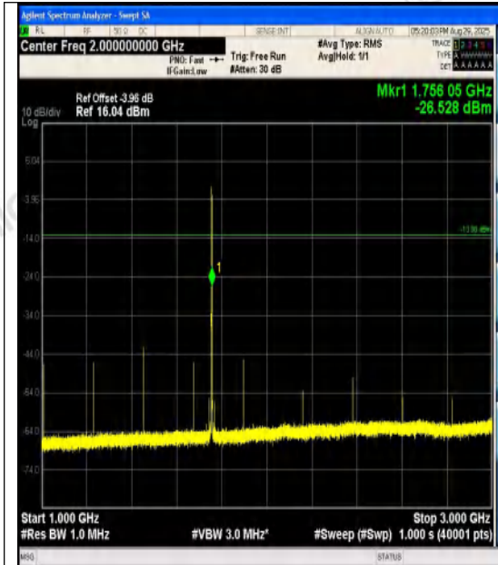
Band4-1.4MHz-QPSK-20393-6RB#0-1000~3000- PASS
