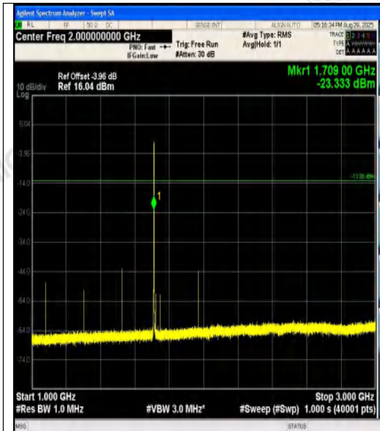
Band4-1.4MHz-QPSK-19957-6RB#0-1000~3000- PASS
