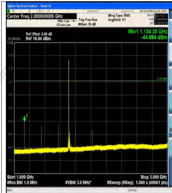
Band4-20MHz-QPSK-20050-1RB#0-1000~3000- PASS
