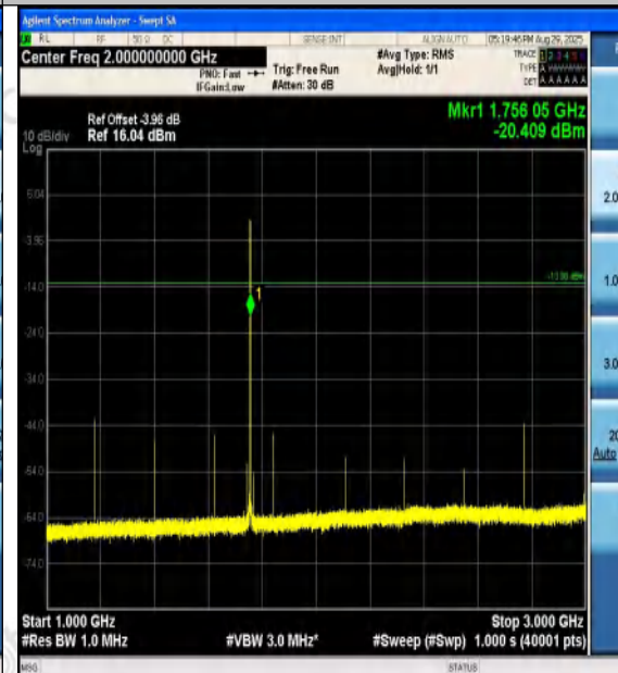
Band4-1.4MHz-16QAM-20393-1RB#5-1000~3000- PASS
