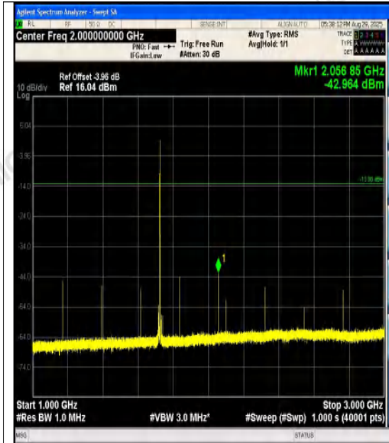
Band4-15MHz-16QAM-20025-1RB#74-1000~300 0-PASS
