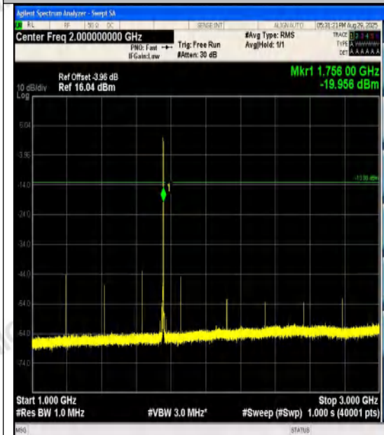
Band4-5MHz-QPSK-20375-1RB#24-1000~3000-
