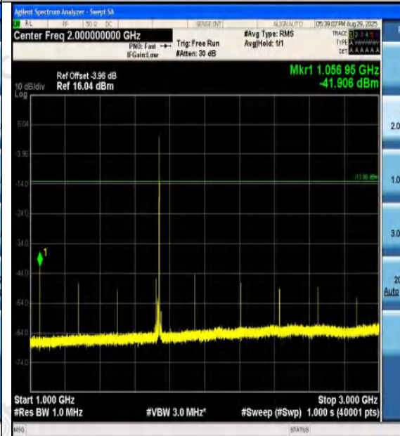
Band4-15MHz-QPSK-20175-1RB#74-1000~3000-P PASS
