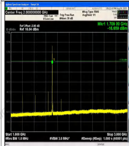
Band4-3MHz-QPSK-19965-1RB#0-1000~3000-P ASS
