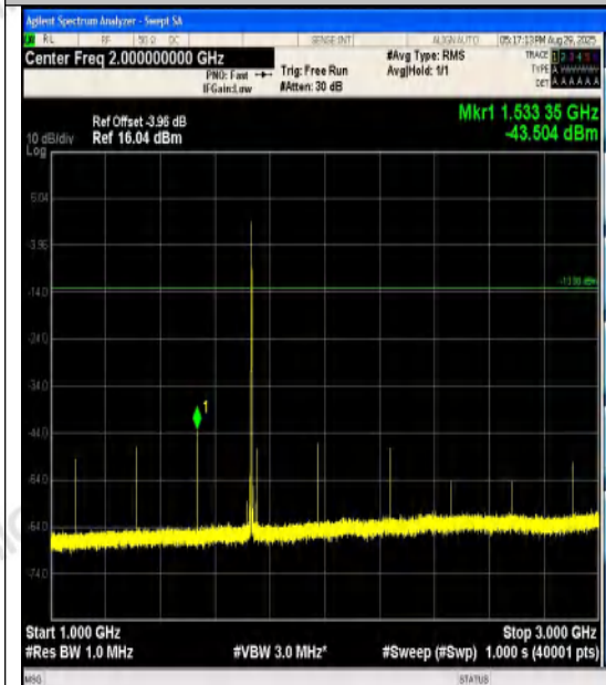
Band4-1.4MHz-QPSK-20175-1RB#0-1000~3000- PASS
