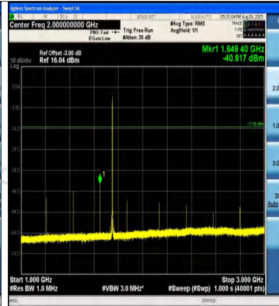
Band4-5MHz-16QAM-20375-1RB#0-1000~3000-P
