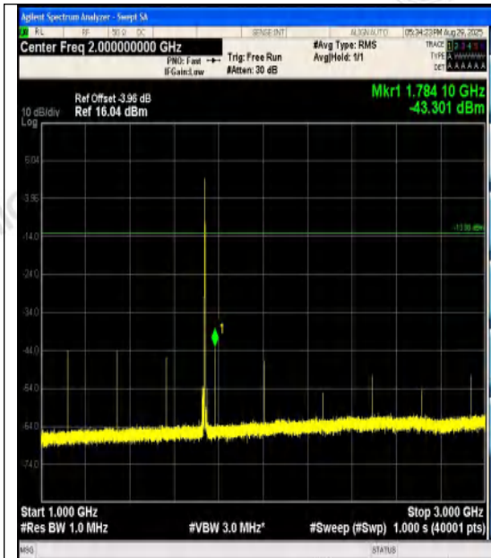
Band4-10MHz-QPSK-20175-1RB#49-1000~3000
