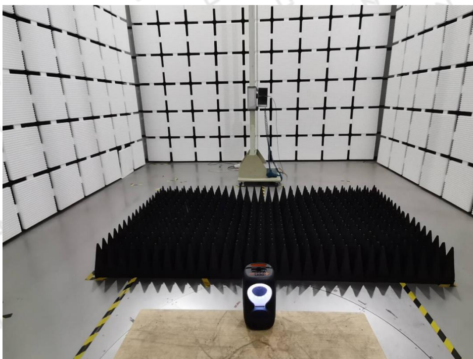
Above 1GHz
