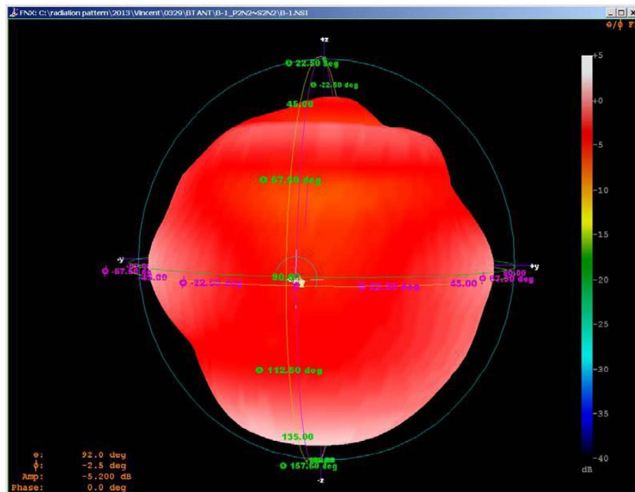
3D radiation pattern diagram
