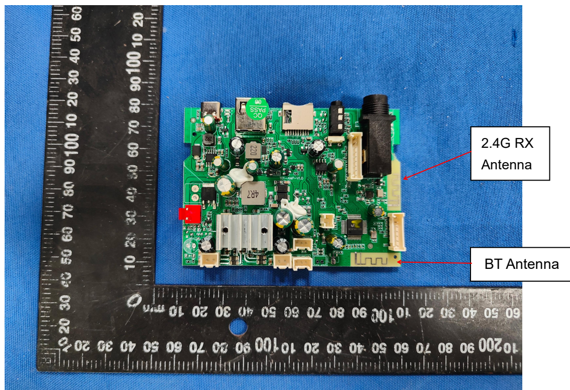
Fig.3 2.4G RX Antenna is only receiving function.
