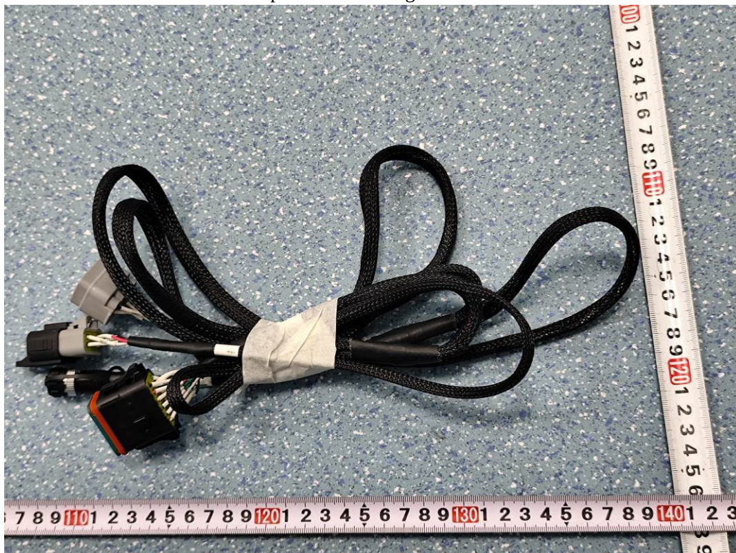
Spare Main Wiring Harness
